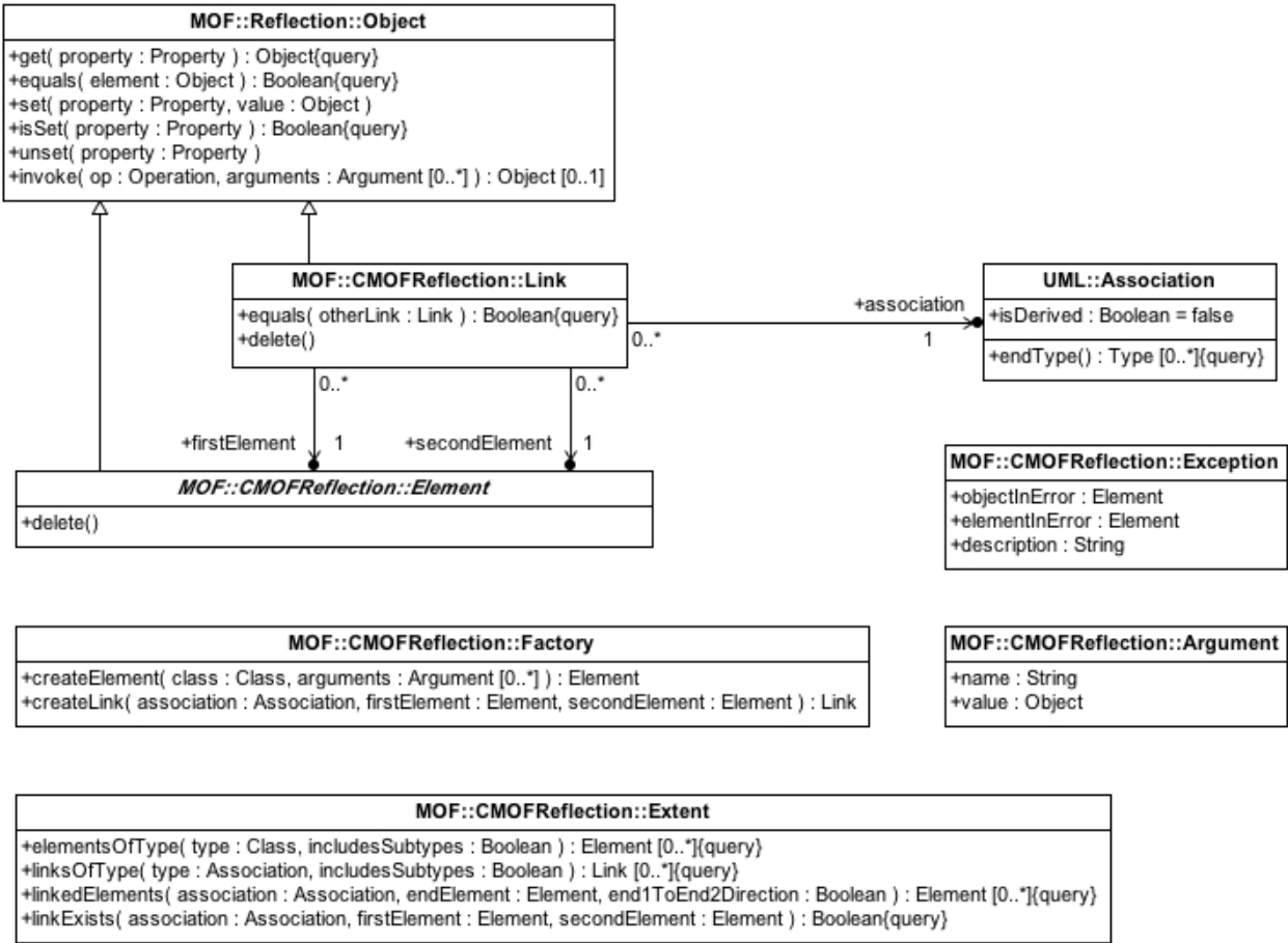
Figure 13.2 - CMOF Reflection package
