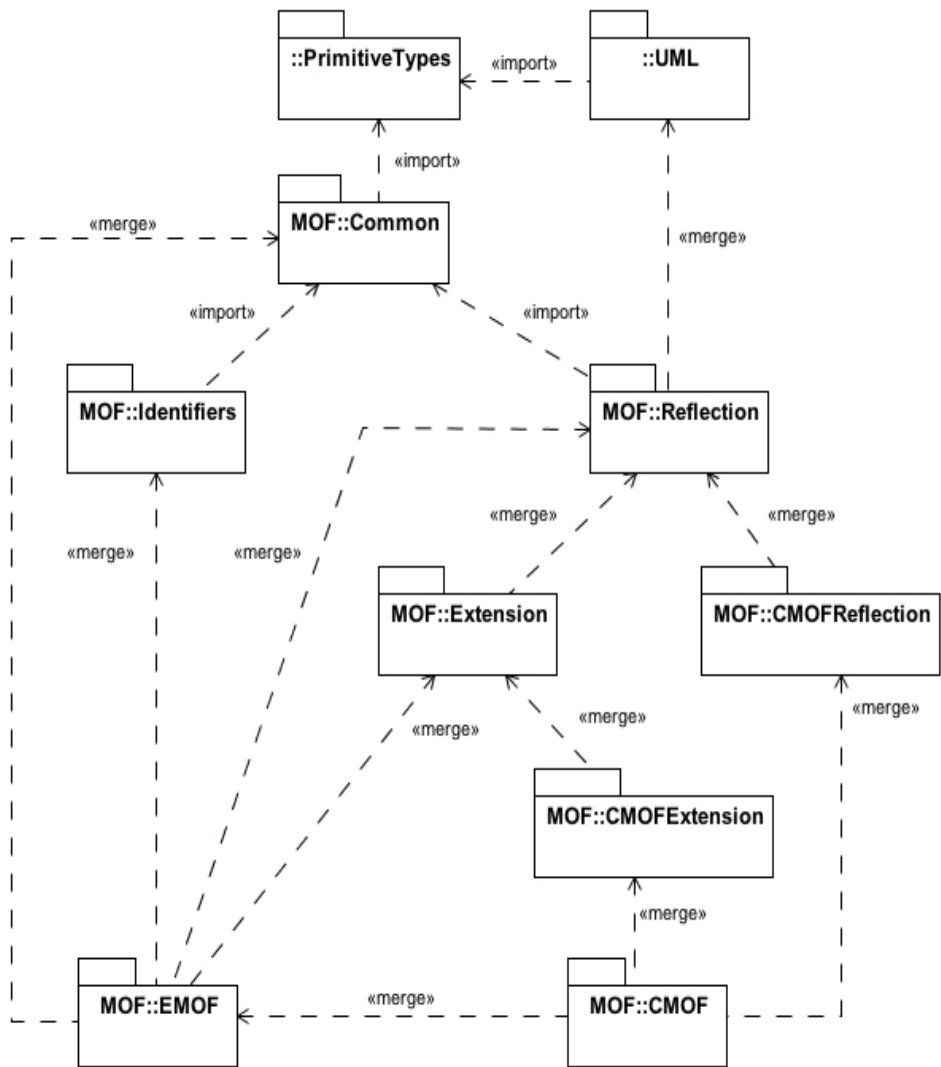
Figure 14.1 - CMOF Packages
