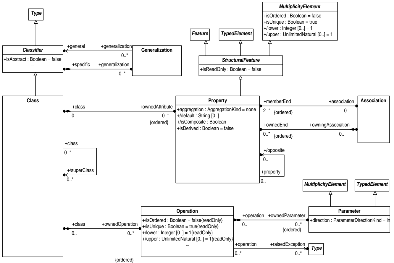
Figure 12.2 - EMOF Classes
