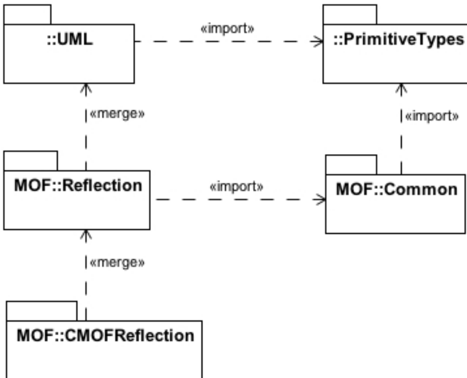
Figure 13.1 - CMOF Reflection
