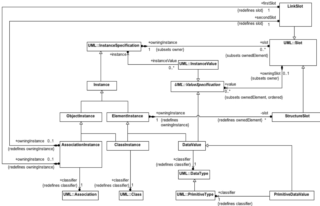
Figure 15.1 - Semantic Domain model for Constructs
