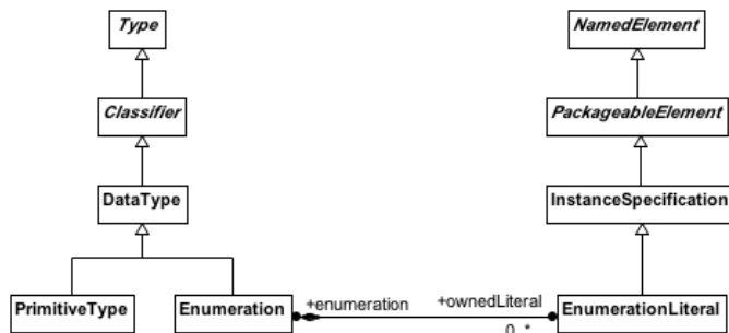
Figure 12.3 - EMOF Data Types
