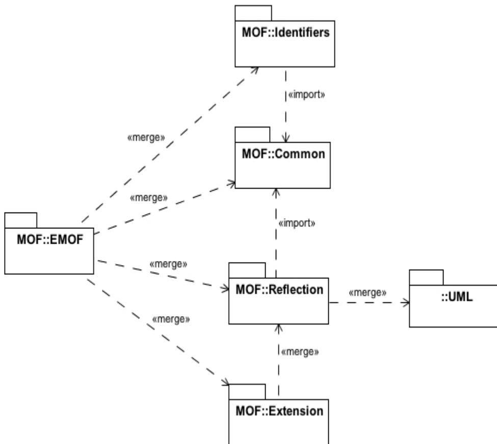
Figure 12.1- EMOF Model - Overview
