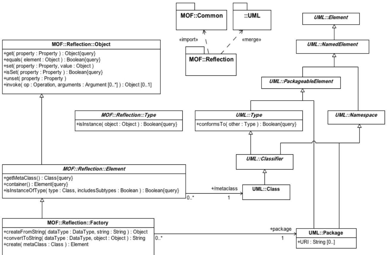
Figure 9.1- The Reflection Package
