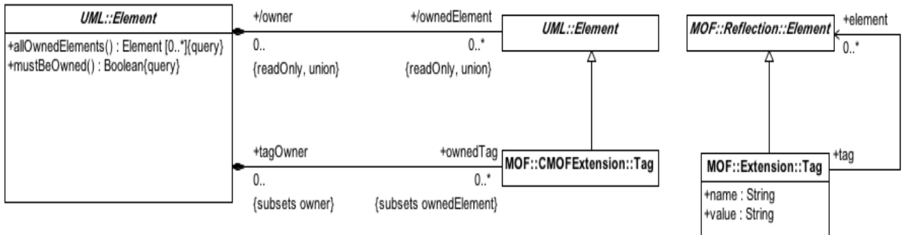
Figure 14.3 - CMOF Extension Package
