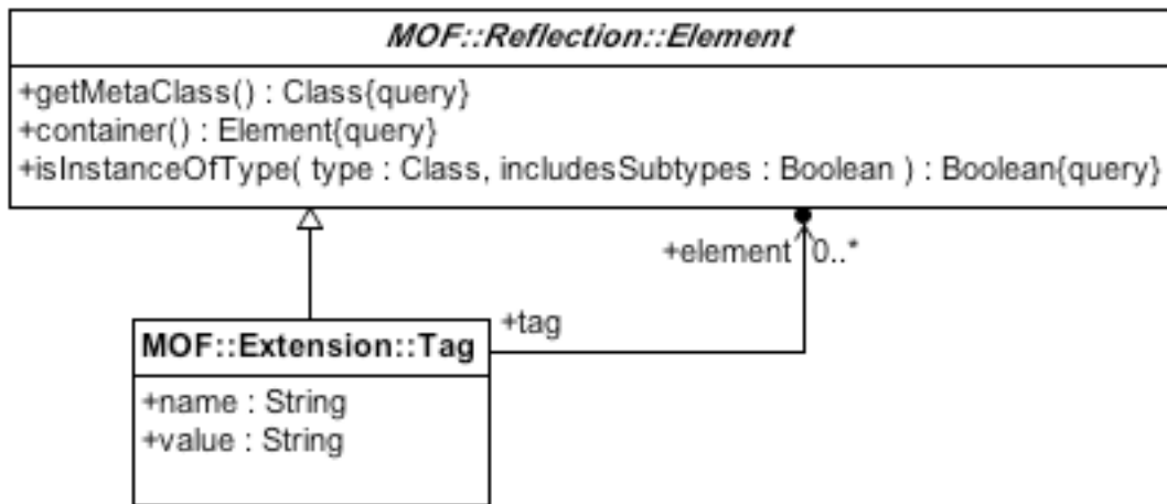
Figure 11.1 – The Extension package
