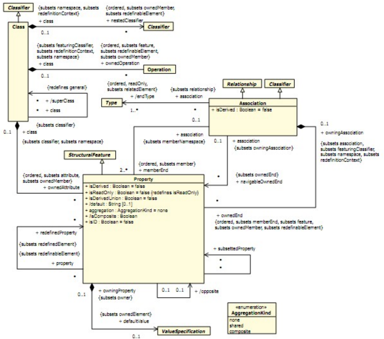
Figure 14.2 – Key concrete classes from UML2 Kernel package
