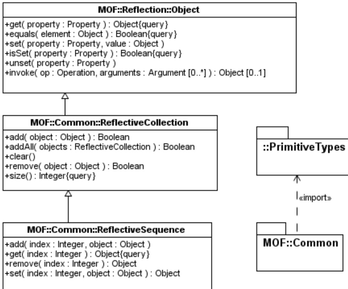
Figure 10.2 – The Common package
