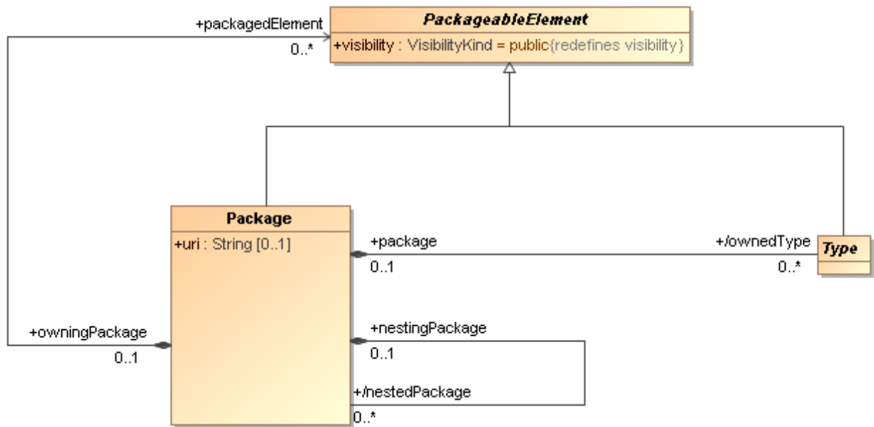
Figure 12.4 – EMOF packages
