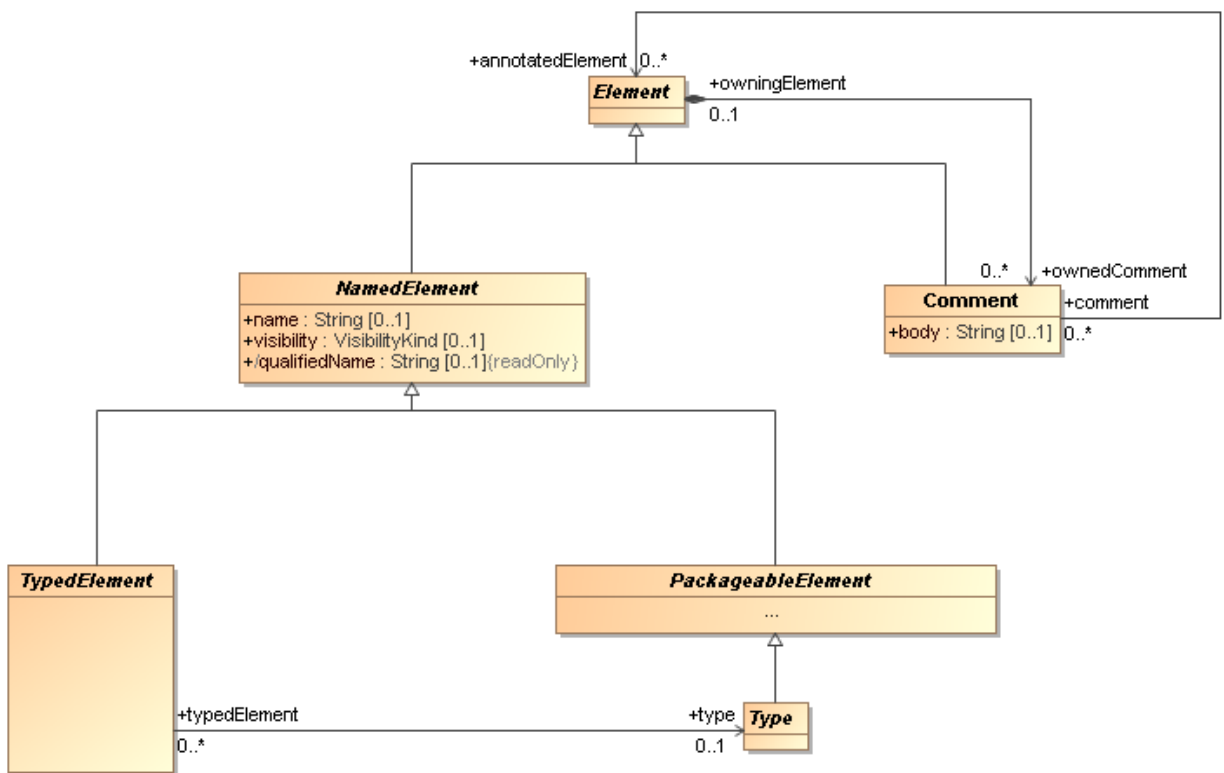
Figure 12.5 – EMOF Types
