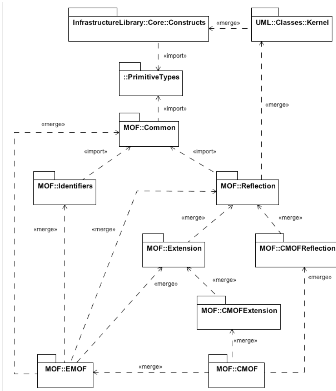
Figure 14.1 – CMOF Packages
