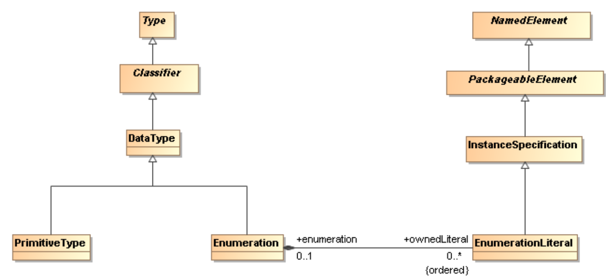
Figure 12.3 – EMOF Data Types
