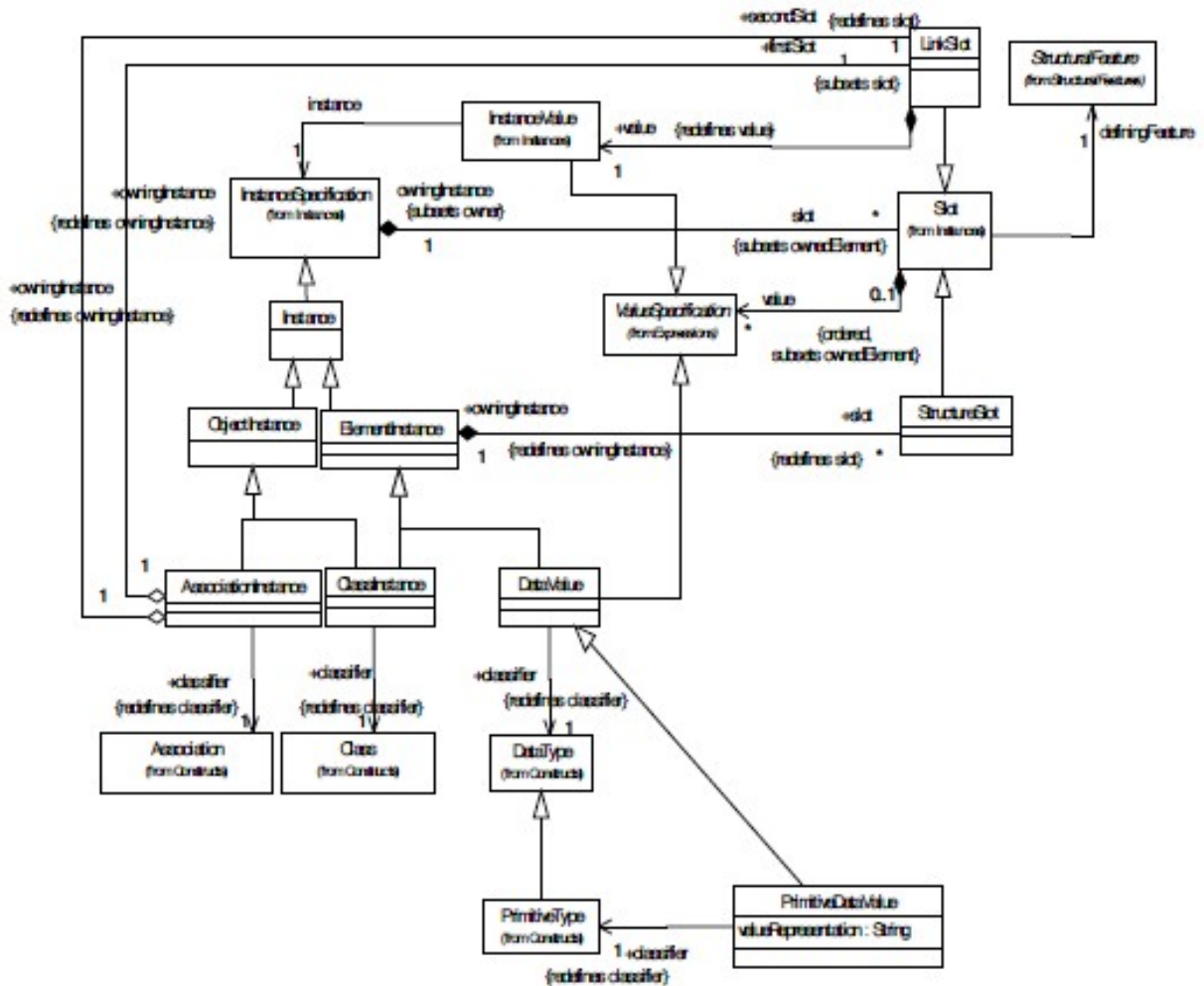
Figure 15.1 – Semantic Domain Model for Constructs
