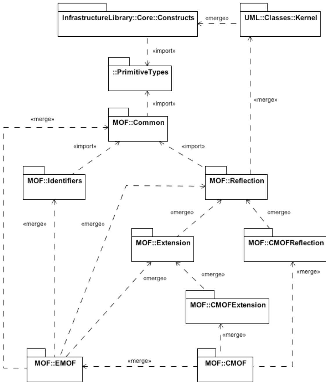
Figure 7.1 – MOF imports from the UML Core
