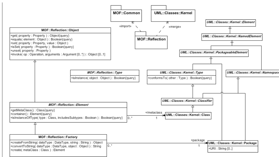
Figure 10.1 – The Reflection package
