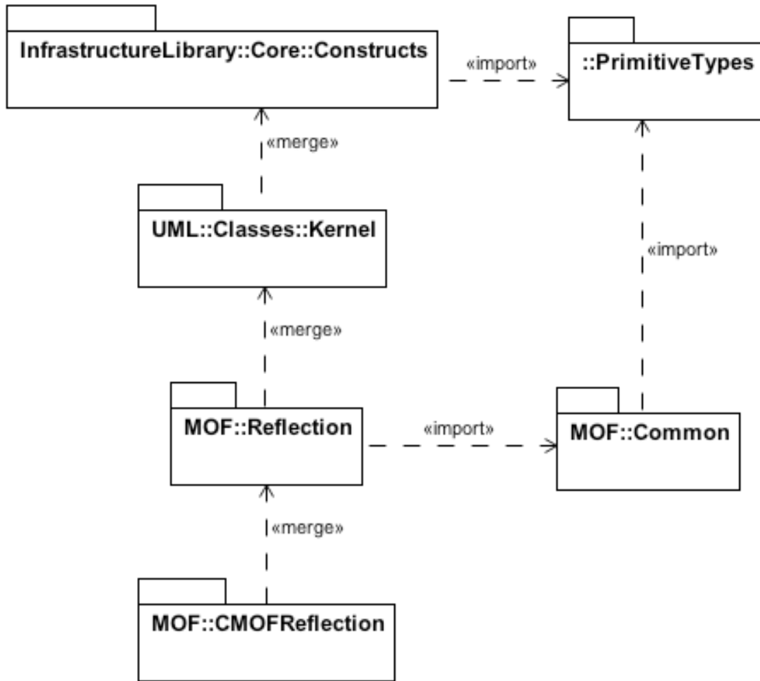
Figure 13.1 – CMOF Reflection
