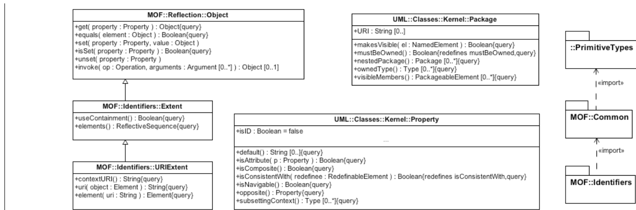
Figure 10.1 – The Identifiers package
