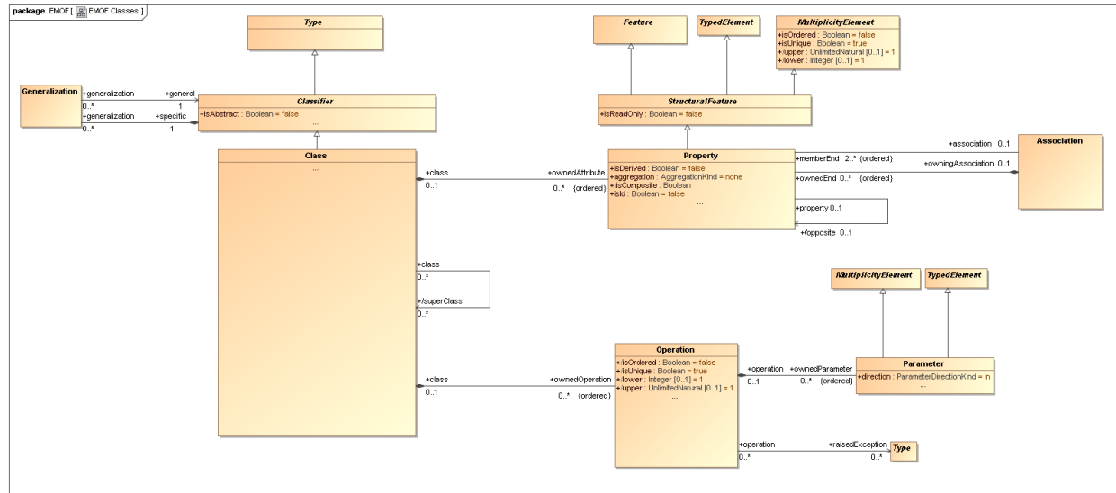
Figure 12.2 – EMOF Classes
