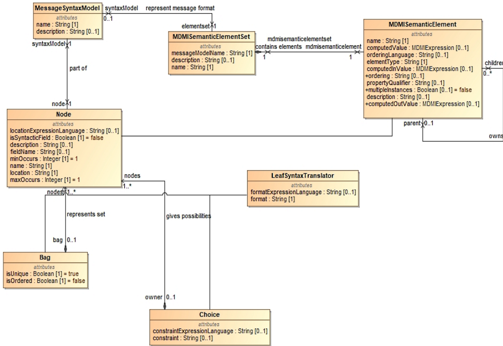
Figure 8.2 – Message Syntax Model
