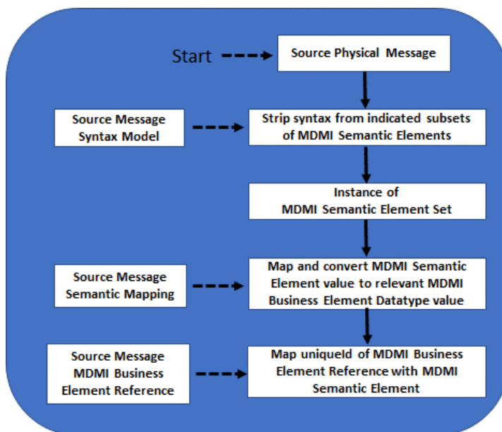
Figure 7.1 – Overview of run-time conversion methodology from Source
