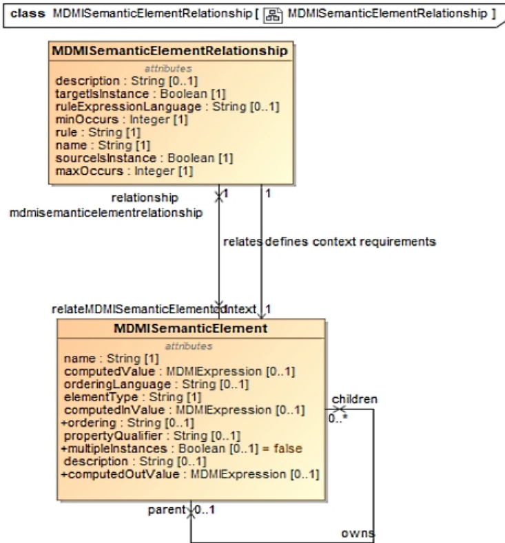
Figure 8.6 – MDMISemanticElementRelationship
