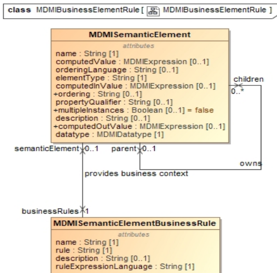
Figure 8.7 – MDMISemanticElementBusiness Rule
