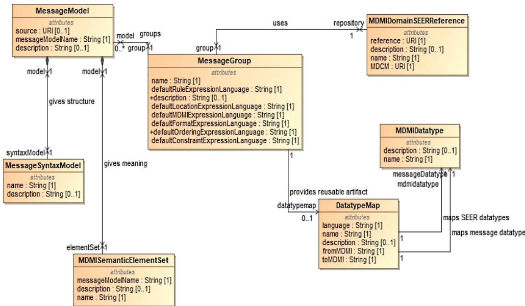
Figure 8.1 – Message Model, MessageGroup, MDMIDomainSEERReference
