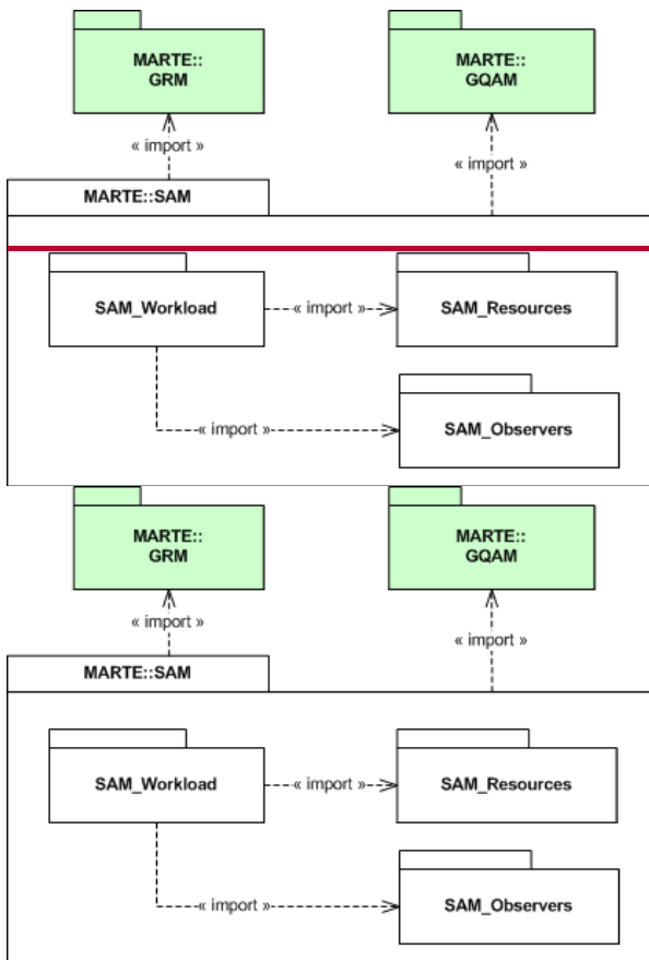
Figure 16.1 - Structure of the SAM domain model
