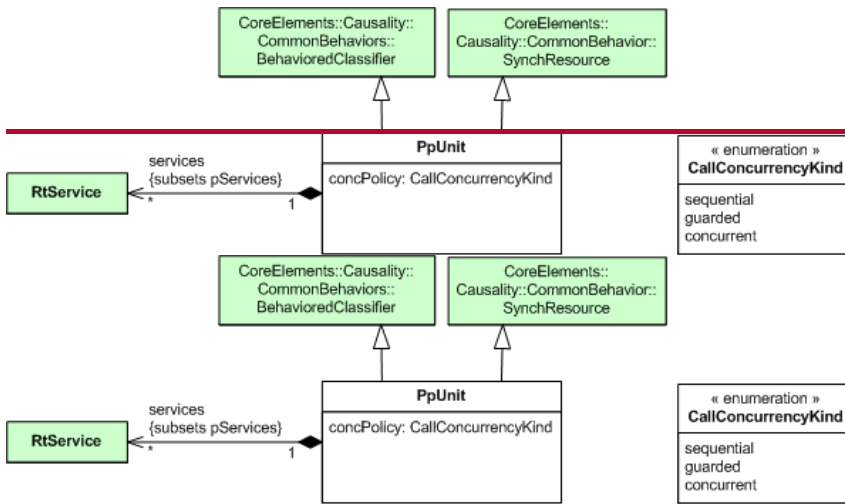
Figure 13.3 - PpUnit of the HLAM package
