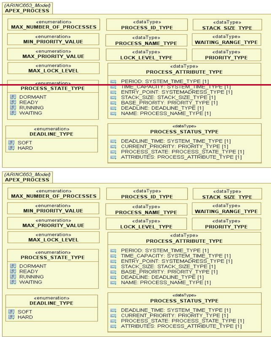
Figure D.22 - ARINC-653 APEX PROCESS Types package
