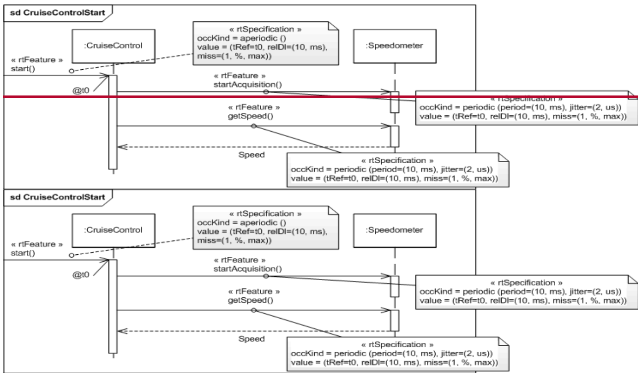
Figure 13.16 - Examples of real-time feature within sequence diagrams
