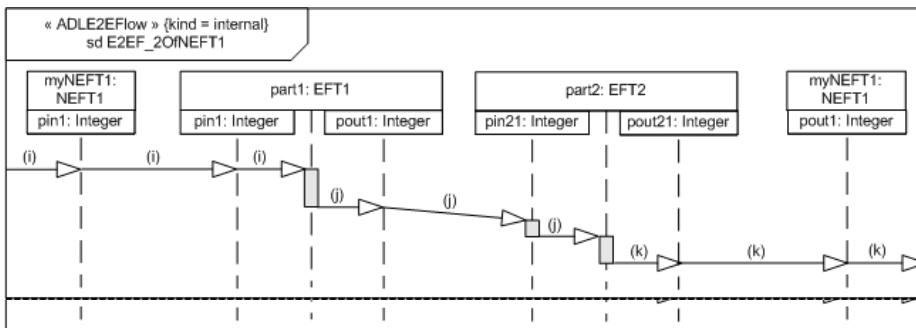
Figure A.26 - Example 1 of an internal end-to-end flow for one non-elementary function
