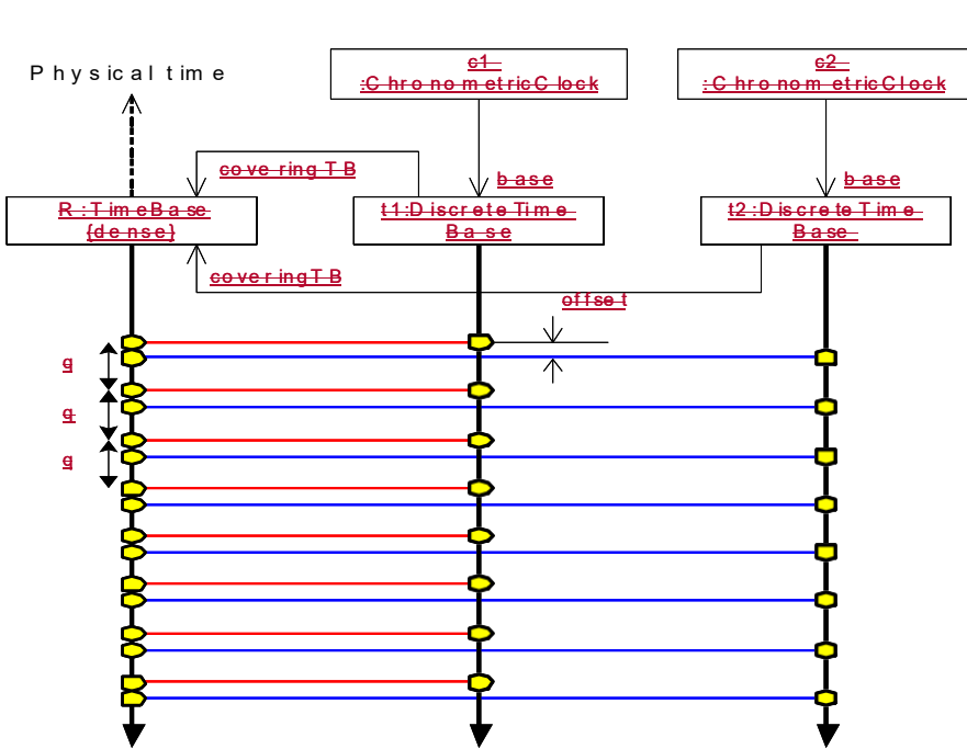
Figure 9.13 - Dependency example of chronometric clocks on physical time
