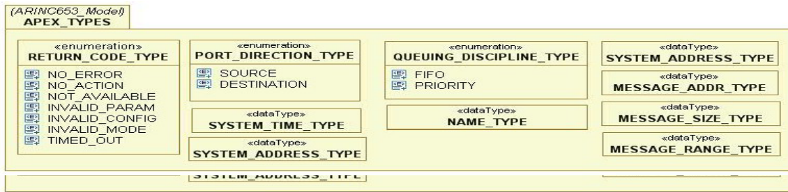
Figure D.21 - ARINC-653 Generic APEX Types package
