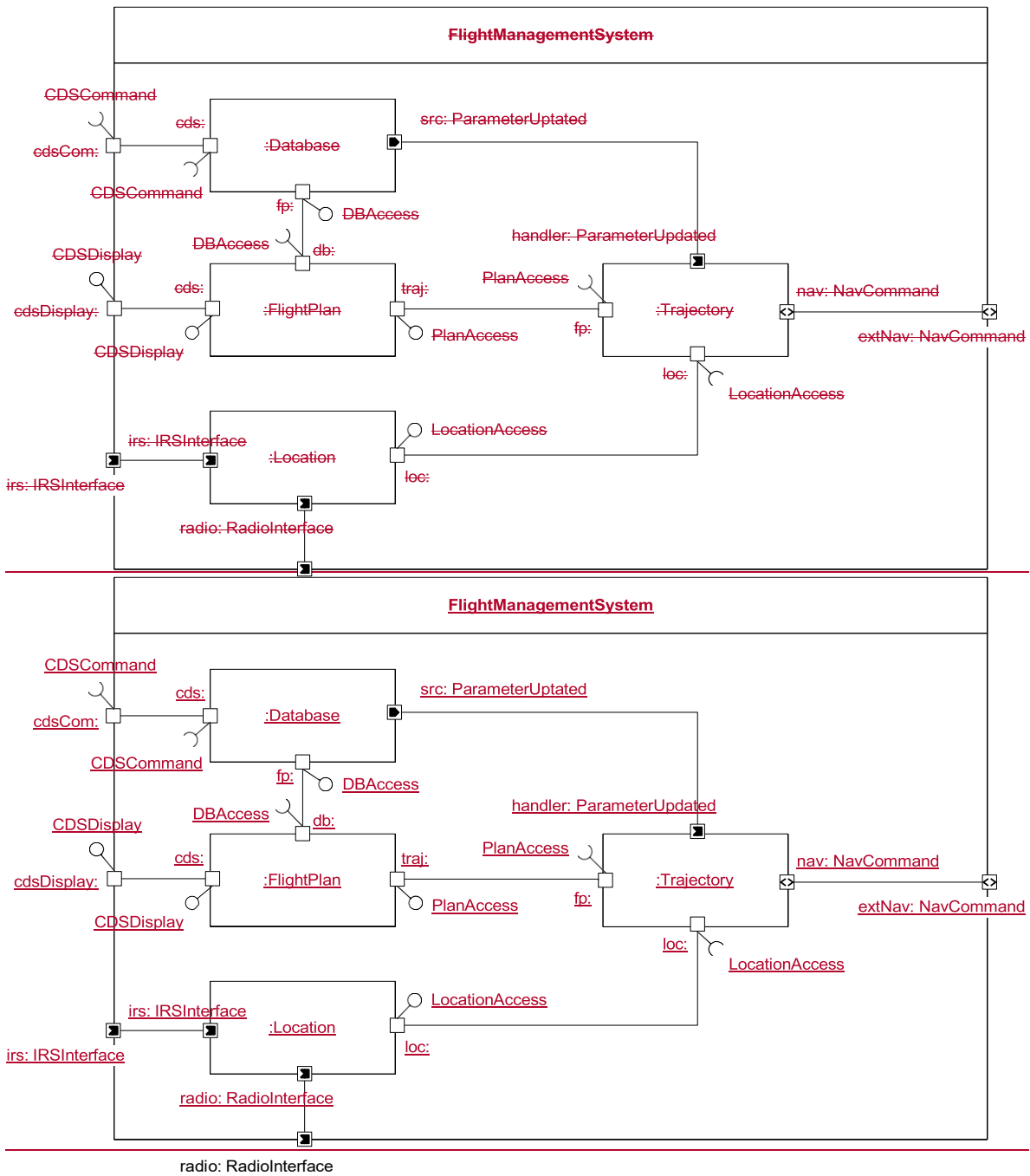
Figure 12.31 - FlightManagementSystem internal structure
