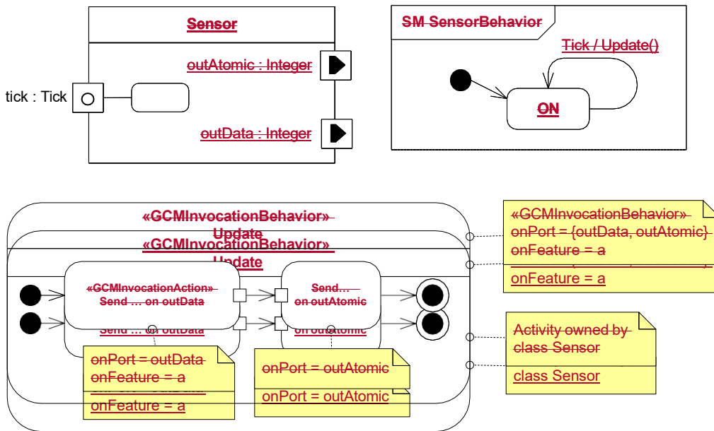
Figure 12.22 - Example 2, a sensor emitting two samples though different ports and features.
