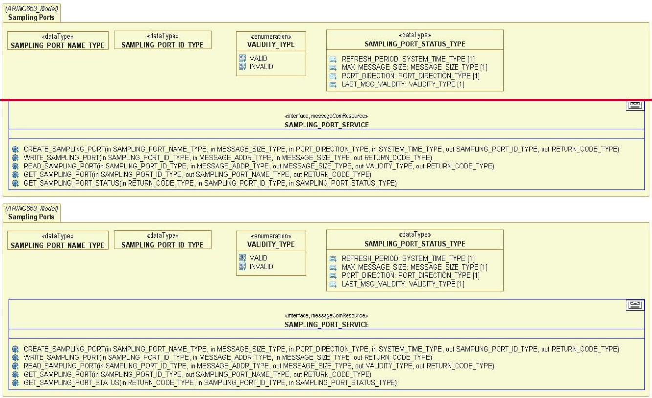
Figure D.26 - ARINC-653 Sampling Ports package
