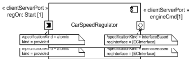
Figure 12.29 - Example of UML component with specialized MARTE ports
