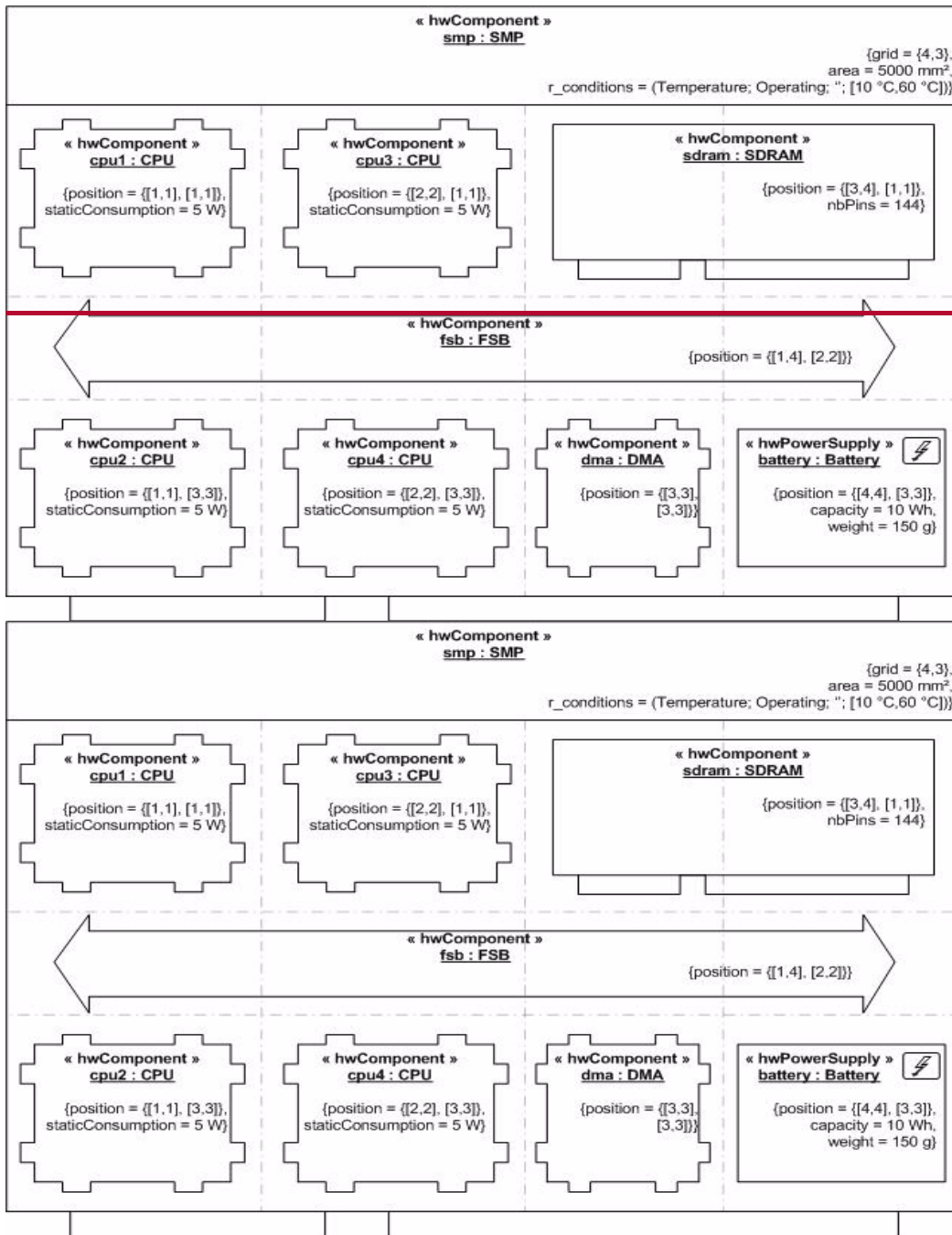
Figure 14.82 - SMP detailed physical model
