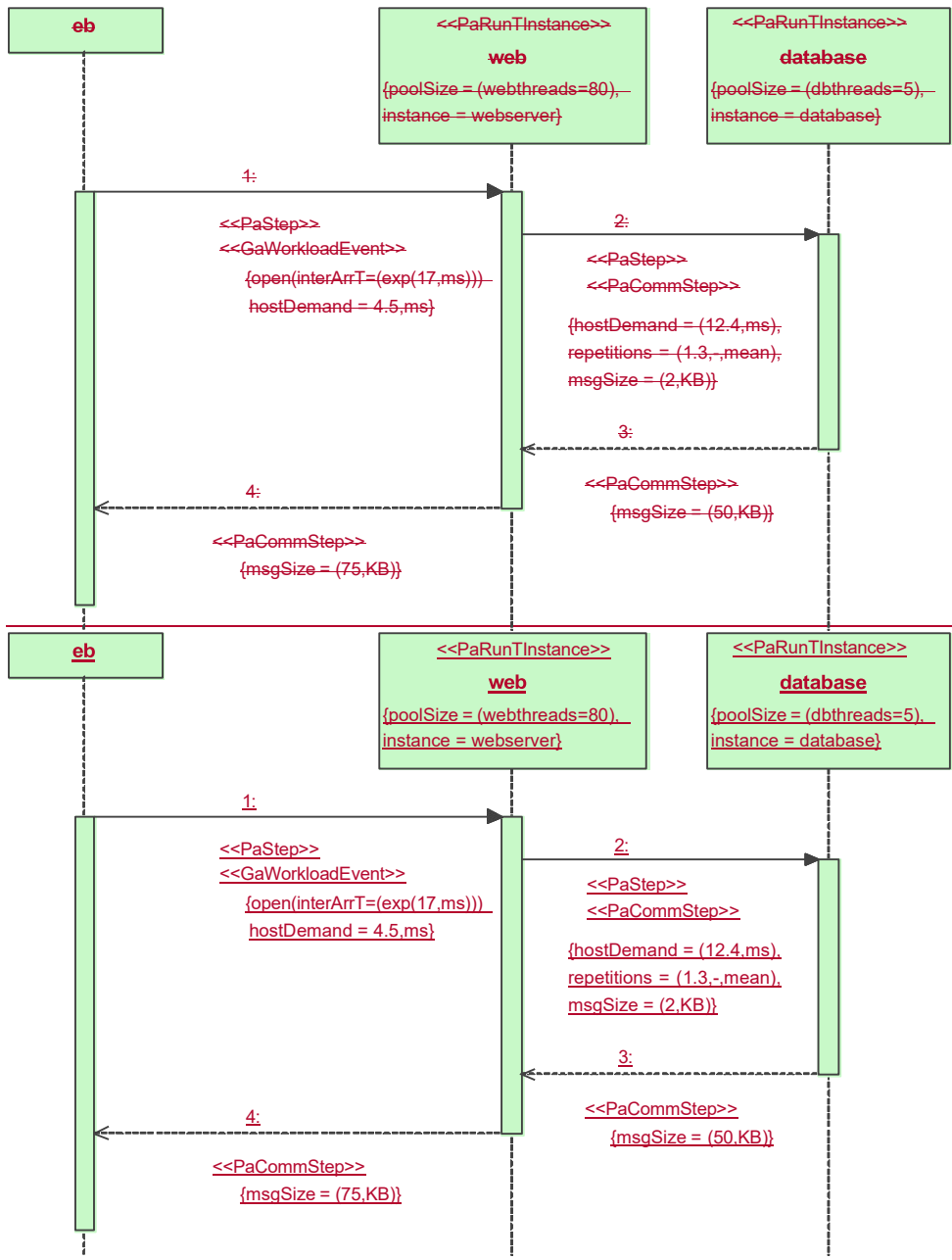
Figure 17.10 - Example of interaction performance annotations
