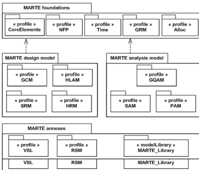
Figure 6.4 - Architecture of the MARTE Profile
