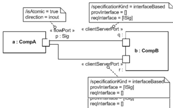
Figure 12.14 - Combined usage of atomic FlowPorts with "interfaceBased" ClientServerPorts
