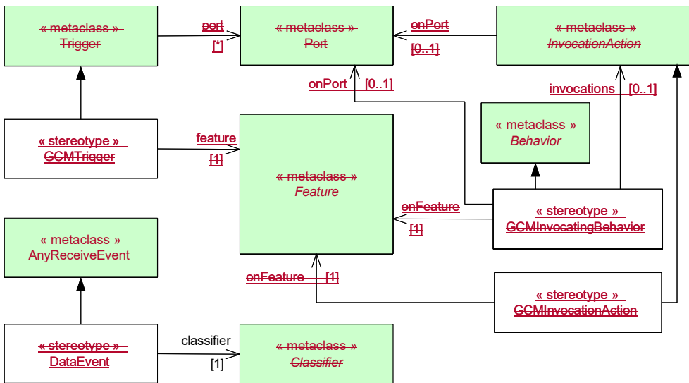
Figure 12.9 - UML profile of the MARTE GeneralComponentModel, event and communication
