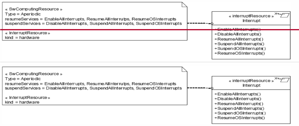
Figure 14.48 - OSEK/VDX Interrupt example
