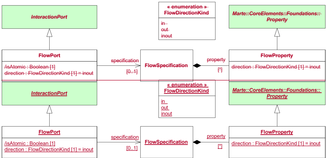
Figure 12.3 - Flow ports of the GenericComponentModel package
