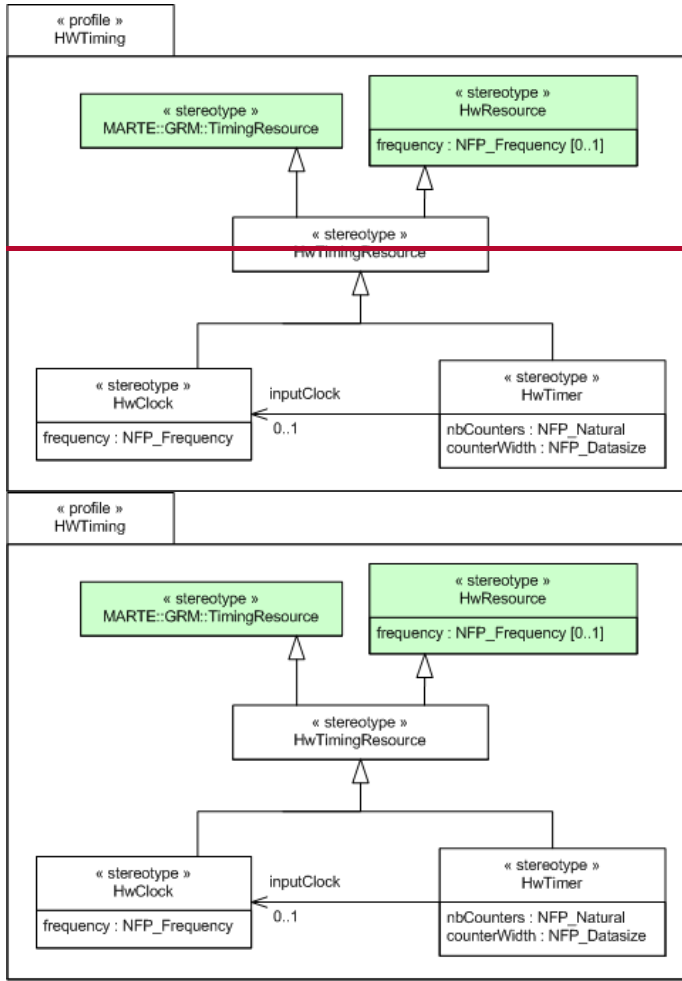
Figure 14.70 - HwTiming profile details
