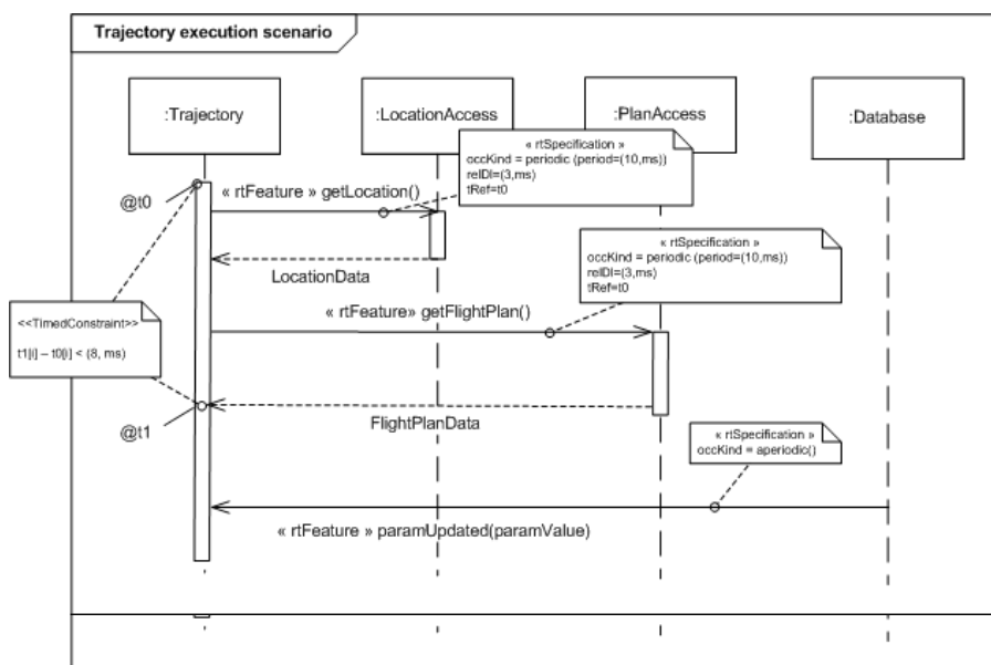
Figure 13.20 - A Trajectory execution scenario within a period
