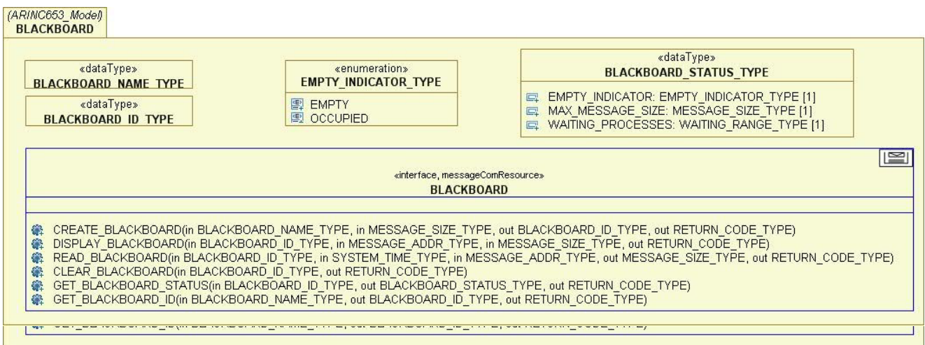
Figure D.29 - ARINC-653 Blackboard package
