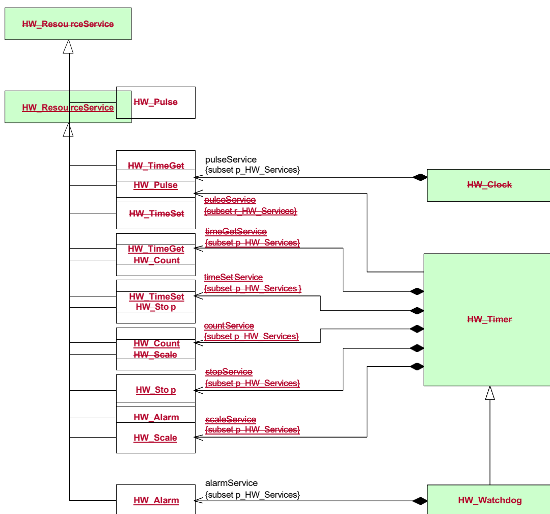
Figure 14.75 - Resource services example (HW_Timing)
