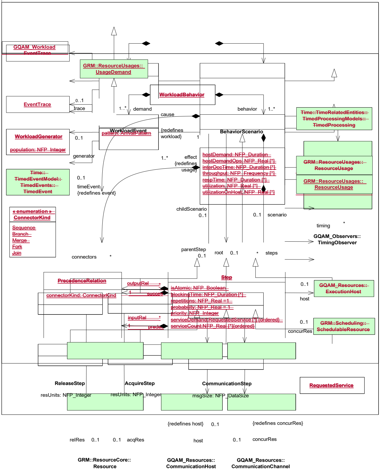
Figure 15.3 - GQAM_Workload package of the GQAM domain model
