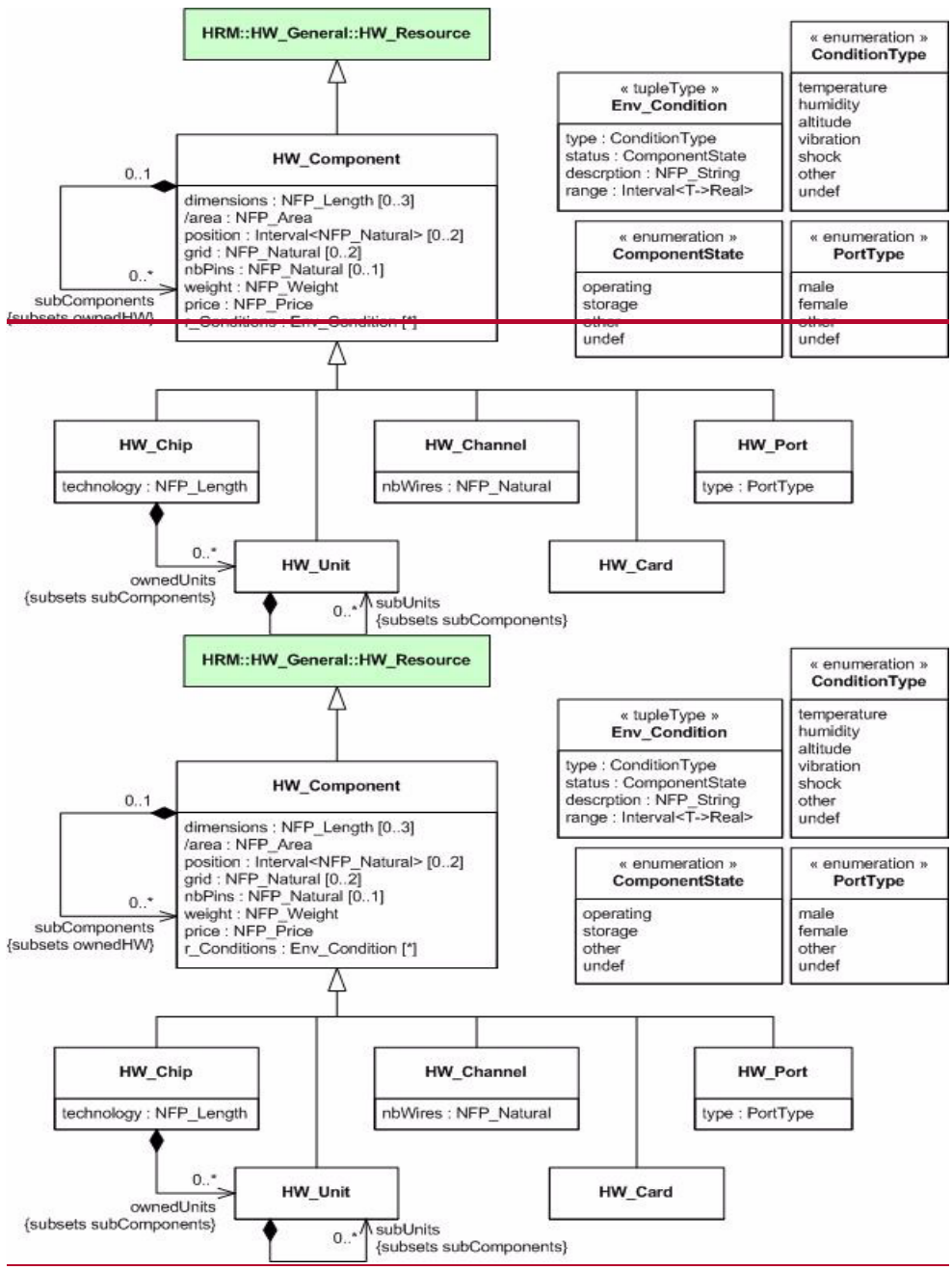
Figure 14.62 - HW_Layout package details
