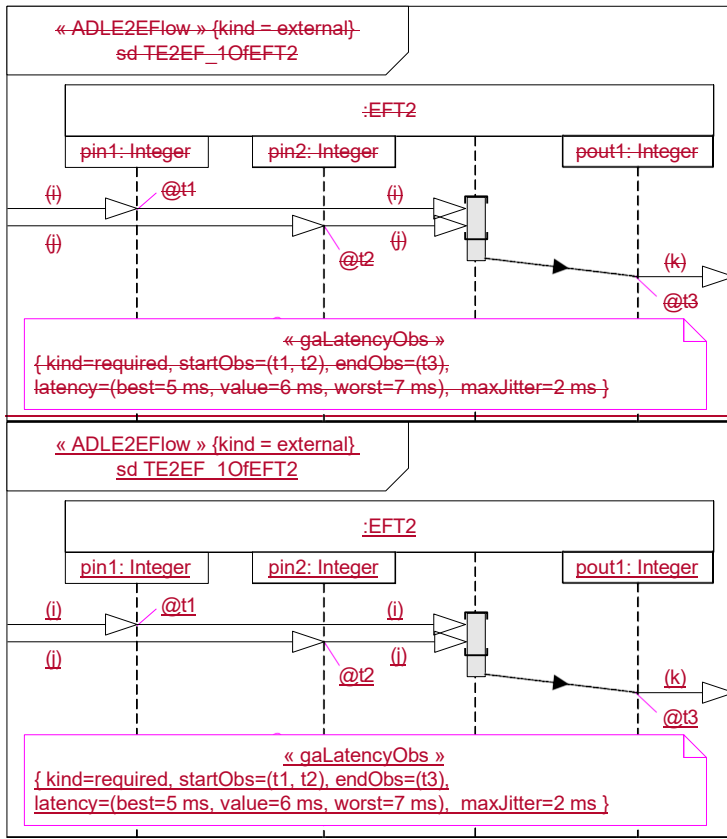
Figure A.34 - Example of latency specification with two input values
