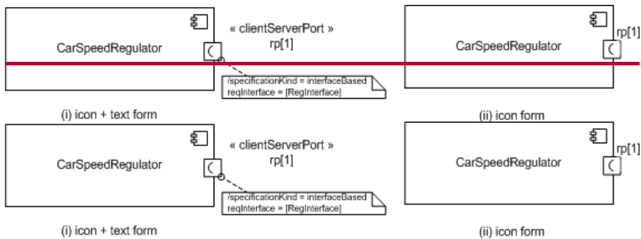
Figure 12.16 - Example of interface-based ClientServerPorts
