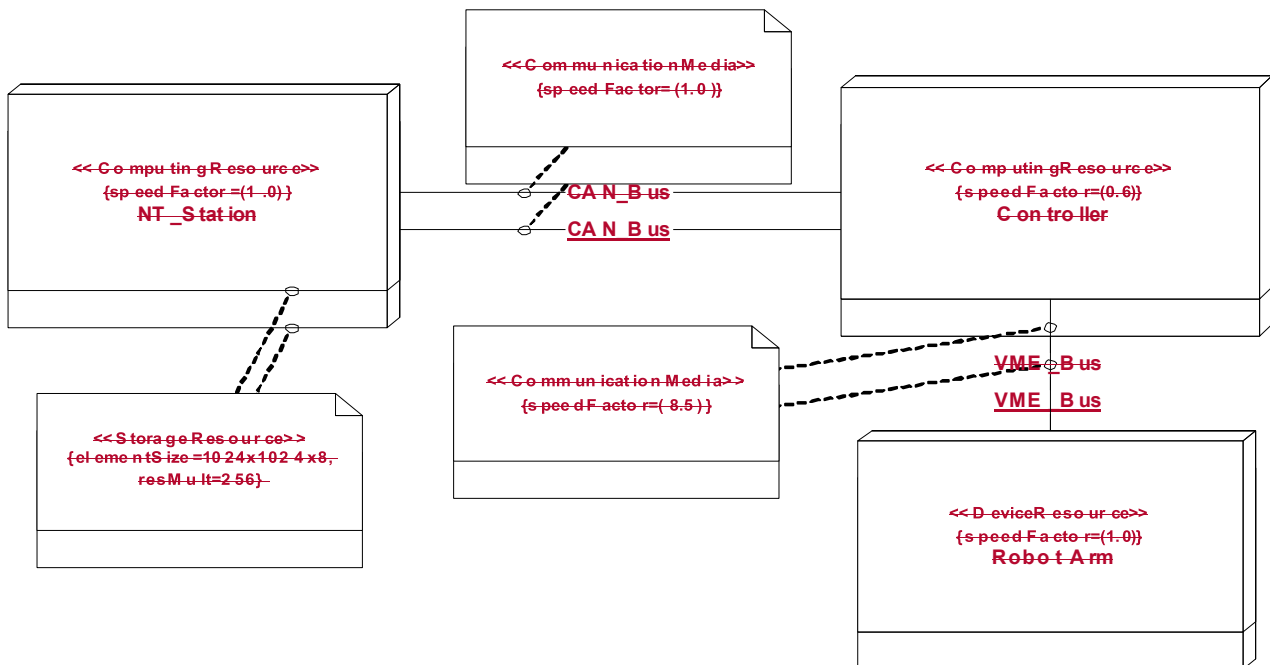
Figure 10.20 - Simple example of usage of the GRM Profile at a high architectural level
