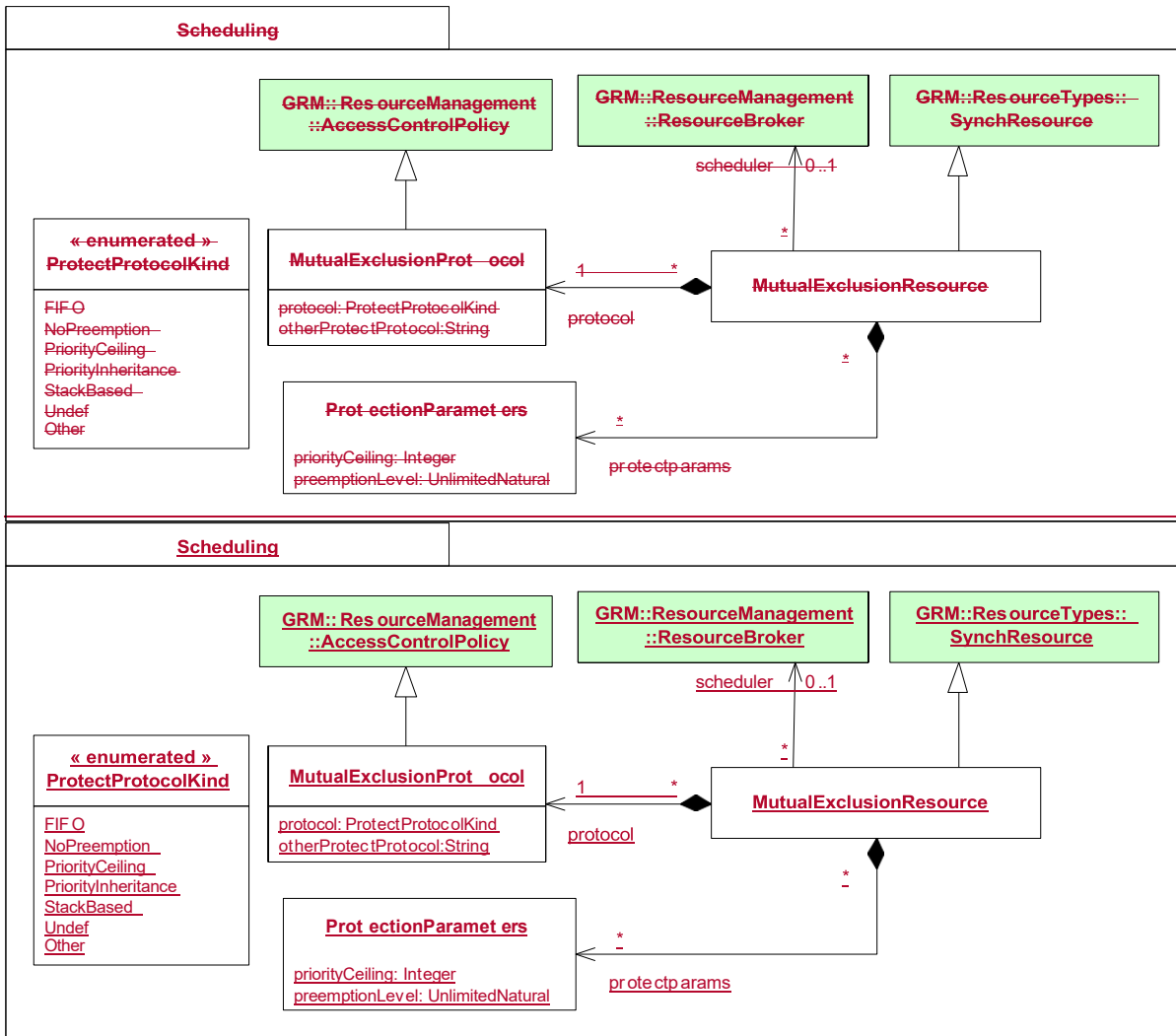
Figure 10.12 - The MutualExclusionResources in the Scheduling Package
