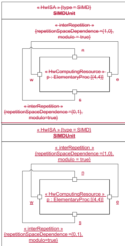
Figure E.9 - 4x4 cyclic grid of processors example
