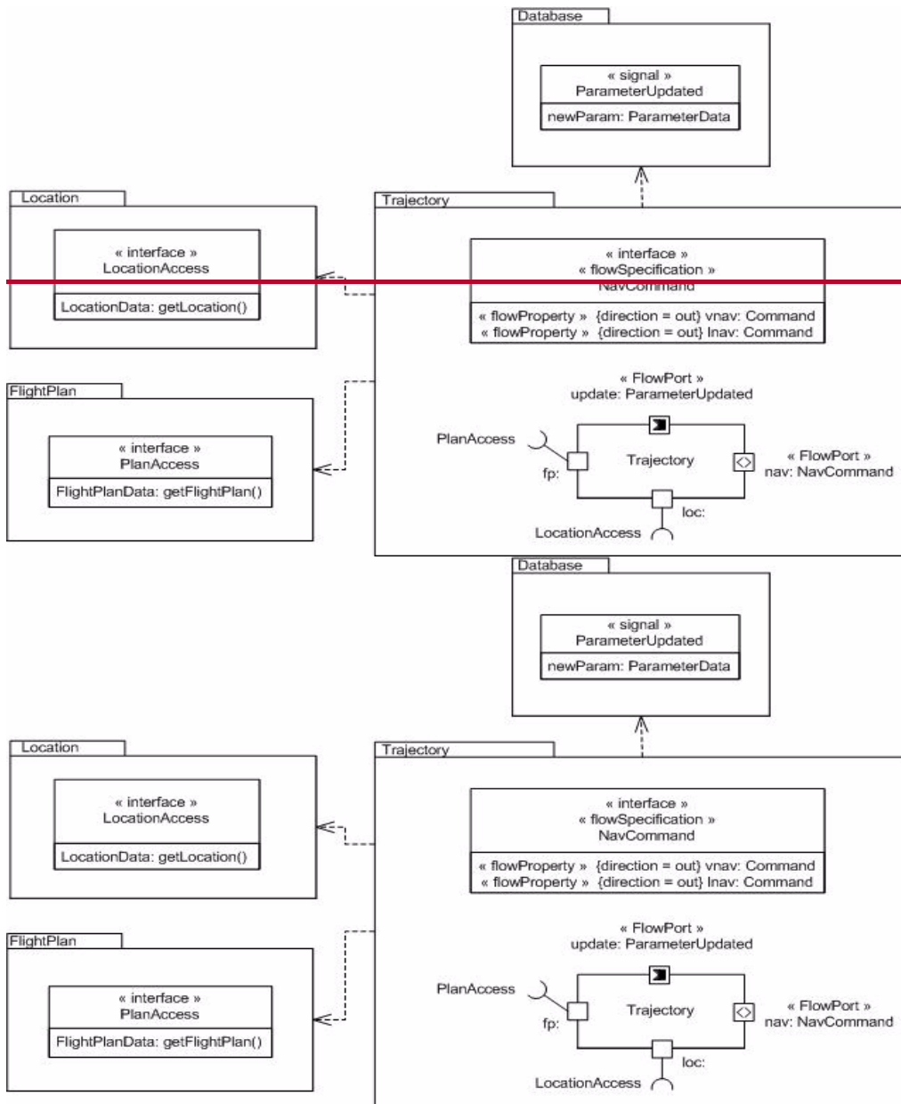
Figure 12.30 - Trajectory component definition
