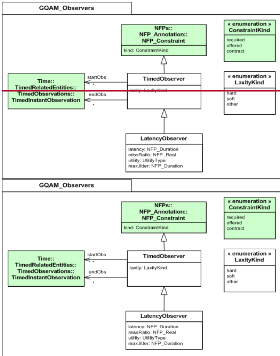
Figure 15.4 - The GQAM Observers package
