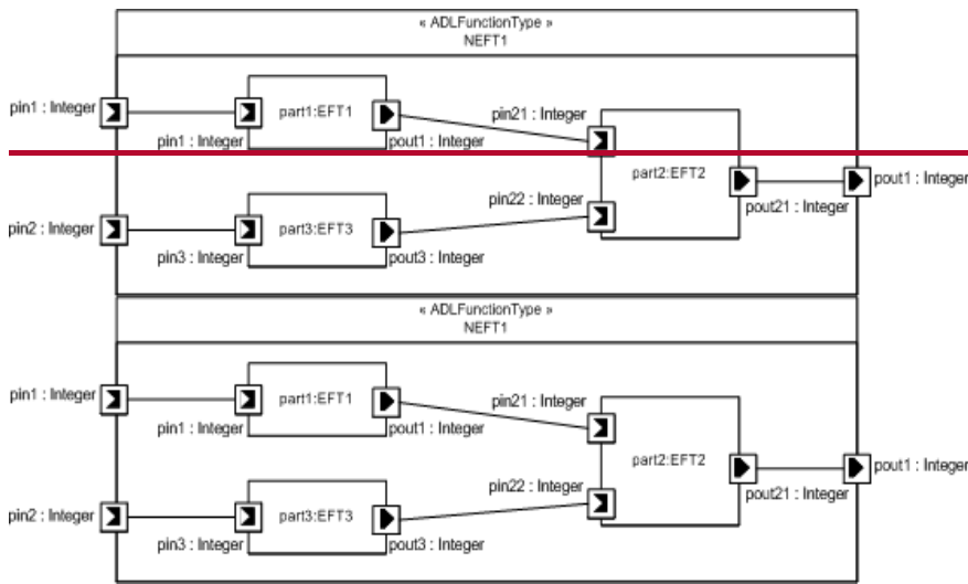
Figure A.25 - Example of a non-elementary function type owning two elementary function prototypes
