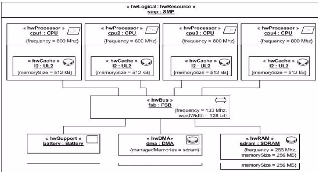
Figure 14.81 - SMP detailed logical model
