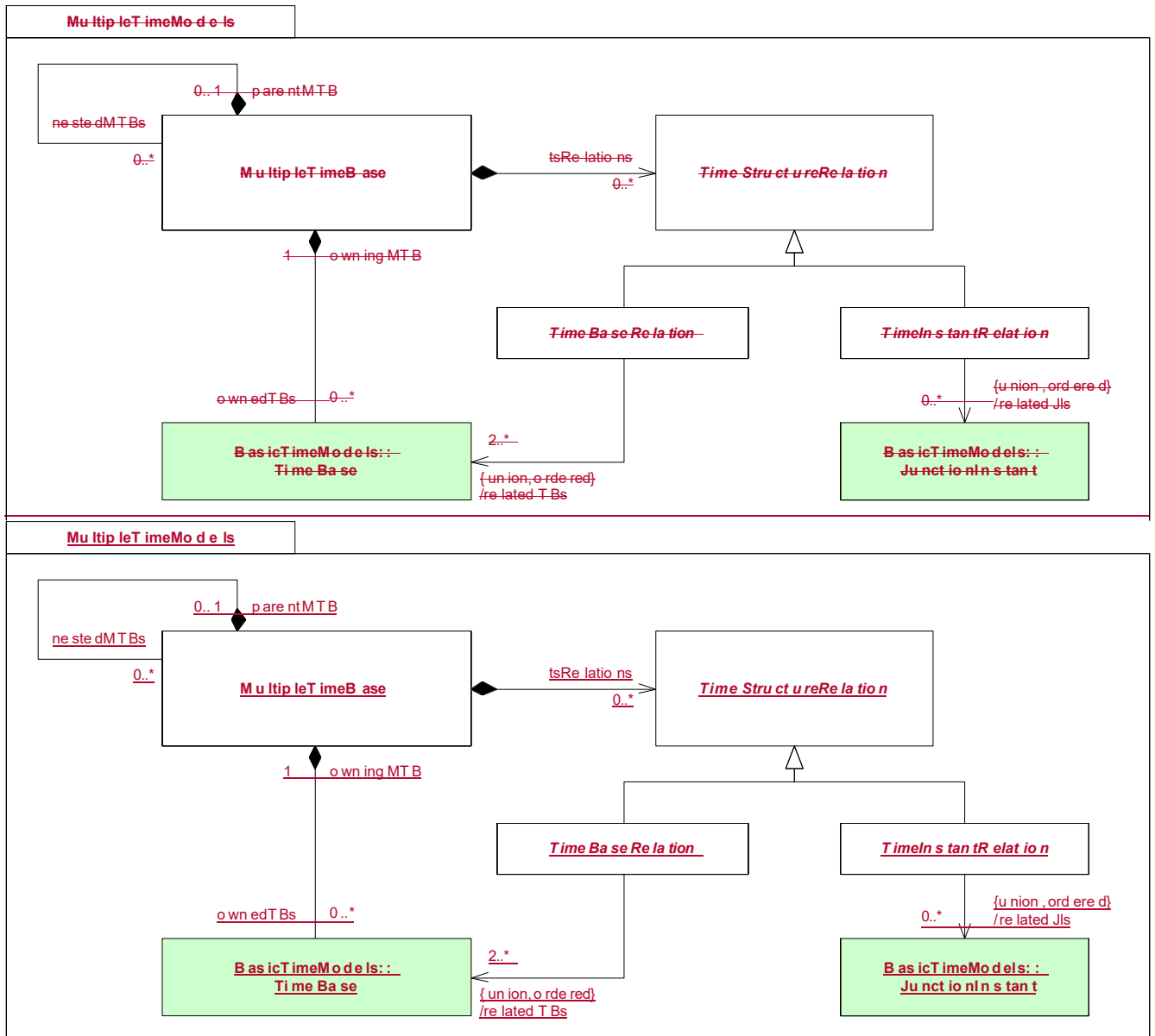
Figure 9.4 - Multiple time diagram of the time model
