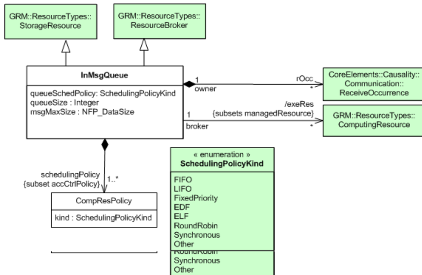
Figure 13.4 - InMsgQueue of the HLAM package
