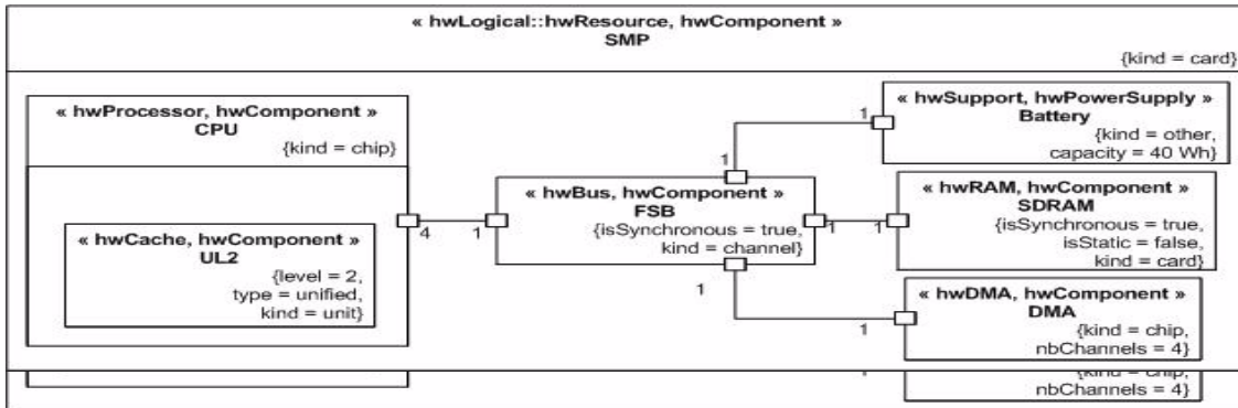
Figure 14.80 - SMP merged (logical/physical) view
