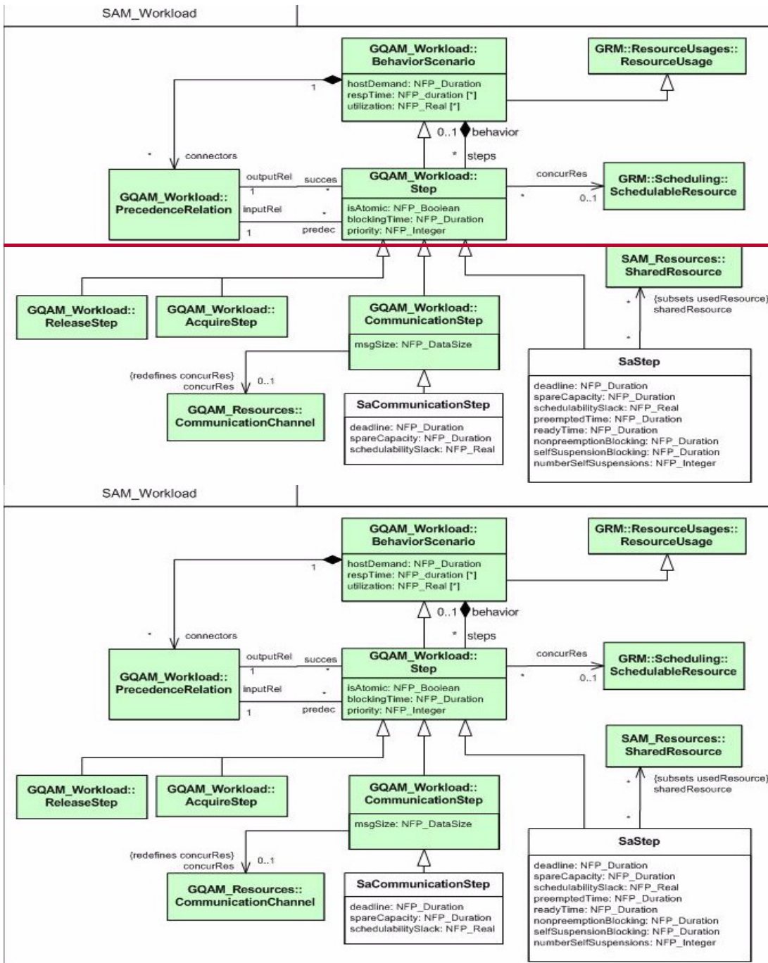
Figure 16.4 - The SAM Workload domain model: BehaviorScenario (partial view)
