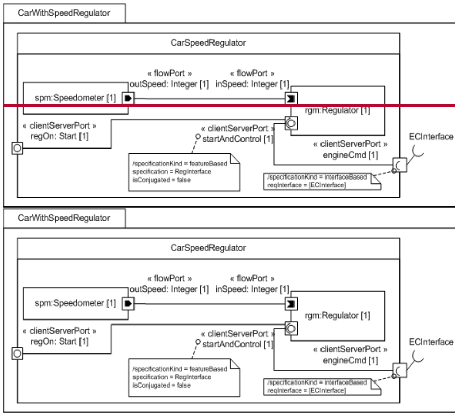
Figure 12.28 - Example of UML composite classes and parts with specialized MARTE ports
