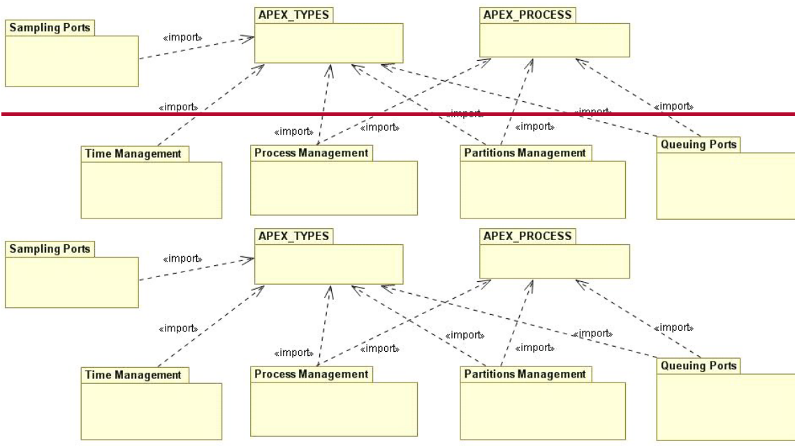
Figure D.19 - Relationship between APEX Types and ARINC-653 API services (part 1)
