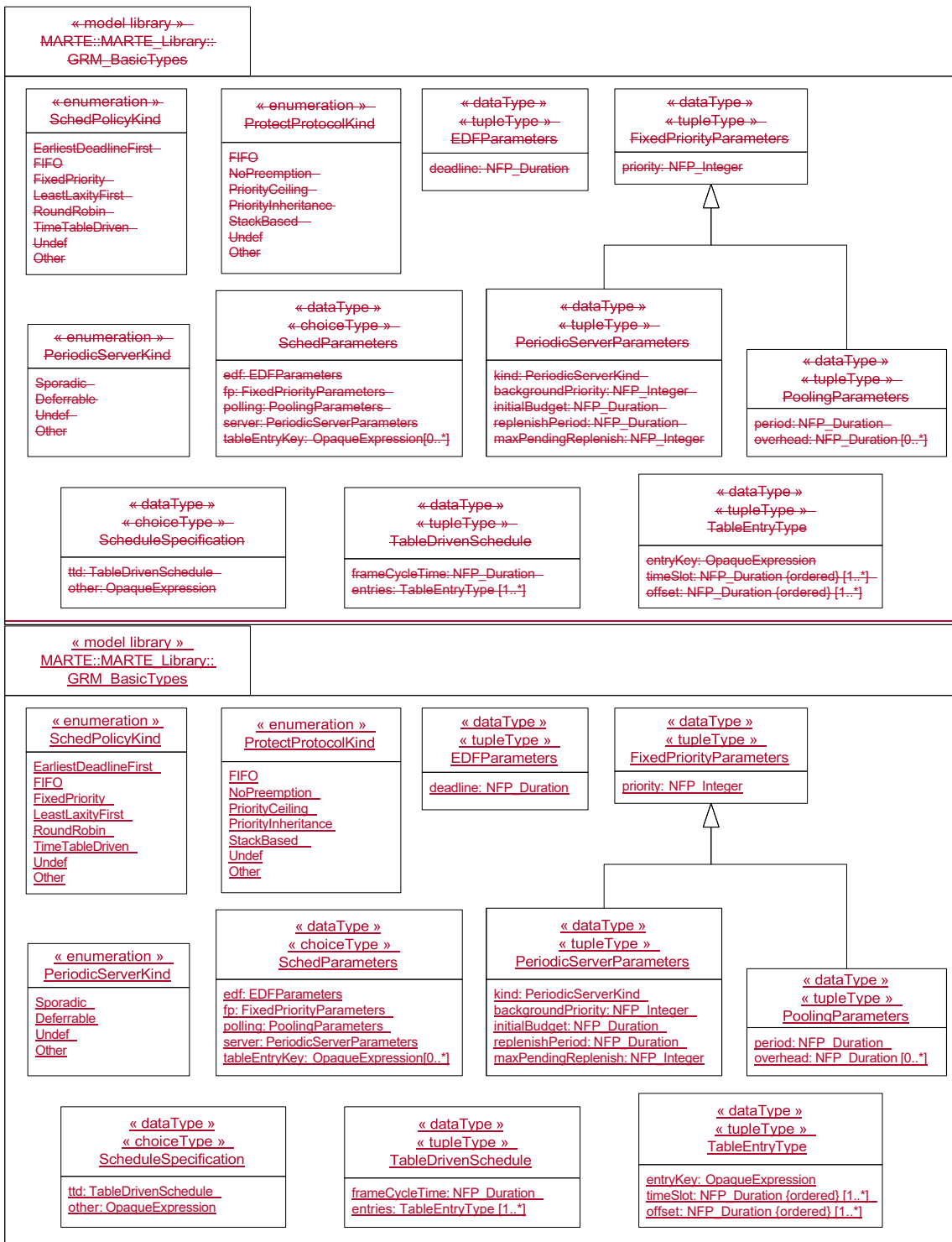
Figure 10.19 - Model library defining types used in the GRM profile (extract of Annex D)
