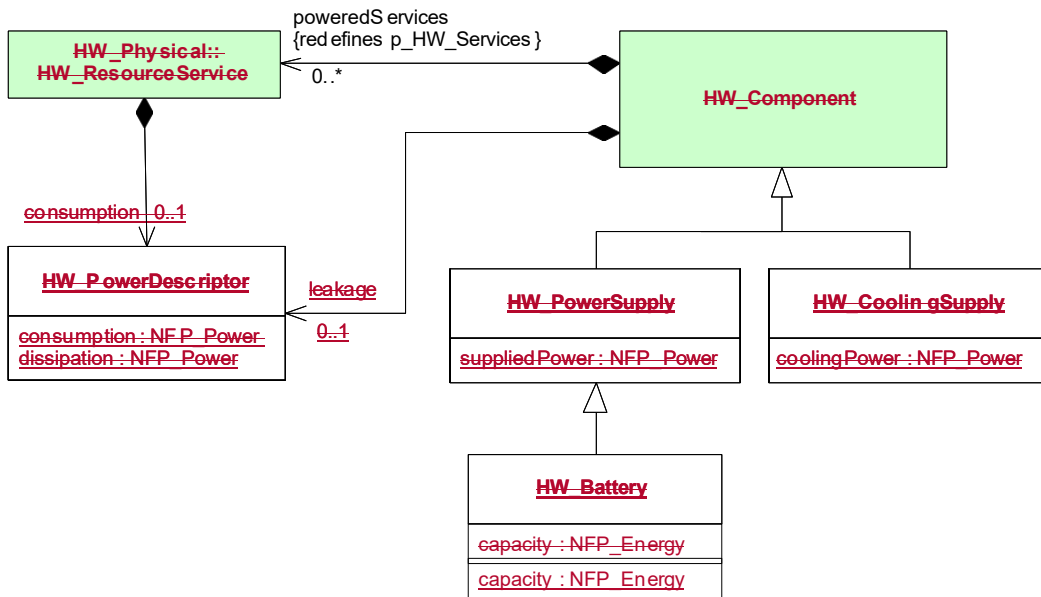
Figure 14.63 - HW_Power package details
