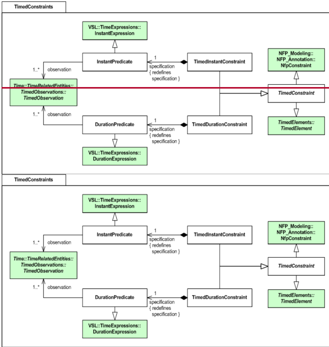
Figure 9.18 - TimedConstraints diagram of the time model
