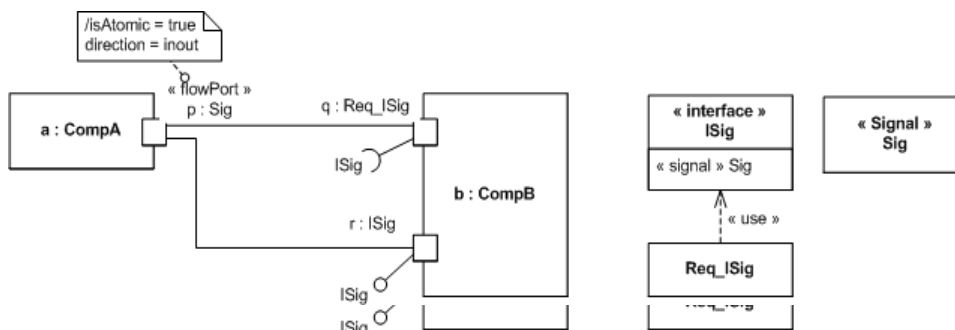
Figure 12.12 - Combined usage of atomic FlowPorts with standard UML ports
