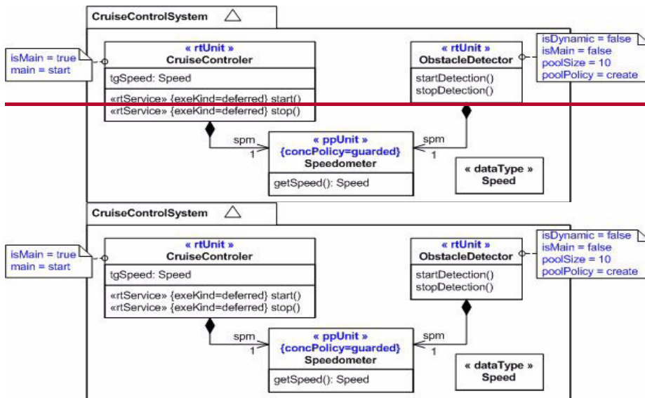
Figure 13.13 - A very simple cruise control model
