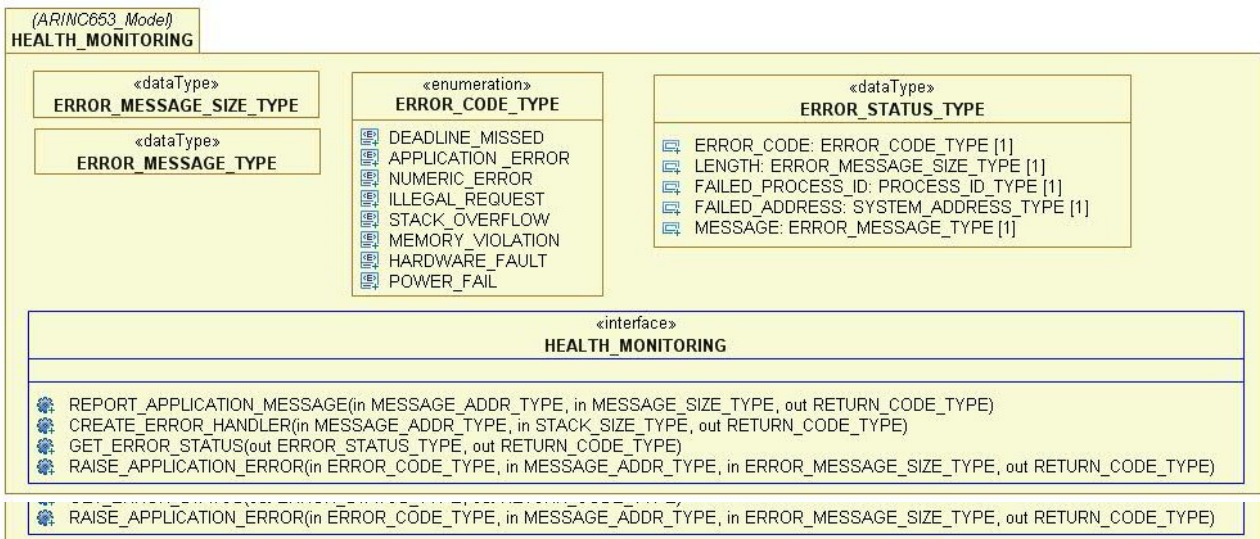
Figure D.32 - ARINC-653 Health monitoring package
