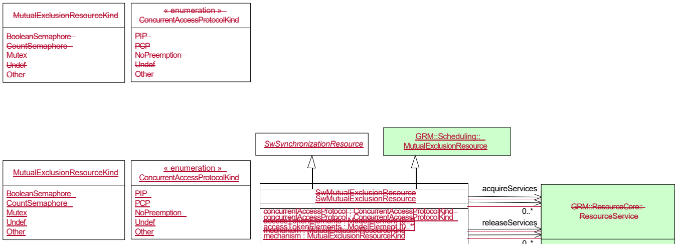
Figure 14.12 - The MutualExclusionResource Overview
