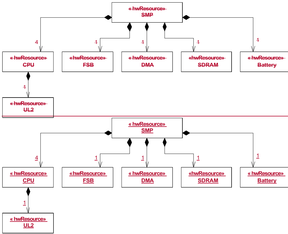
Figure 14.77 - SMP description
