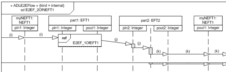
Figure A.28 - Example of reuse within one end-to-end flow description
