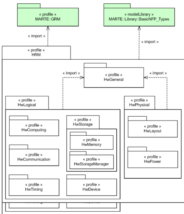
Figure 14.64 - Hardware Resource Model profile structure
