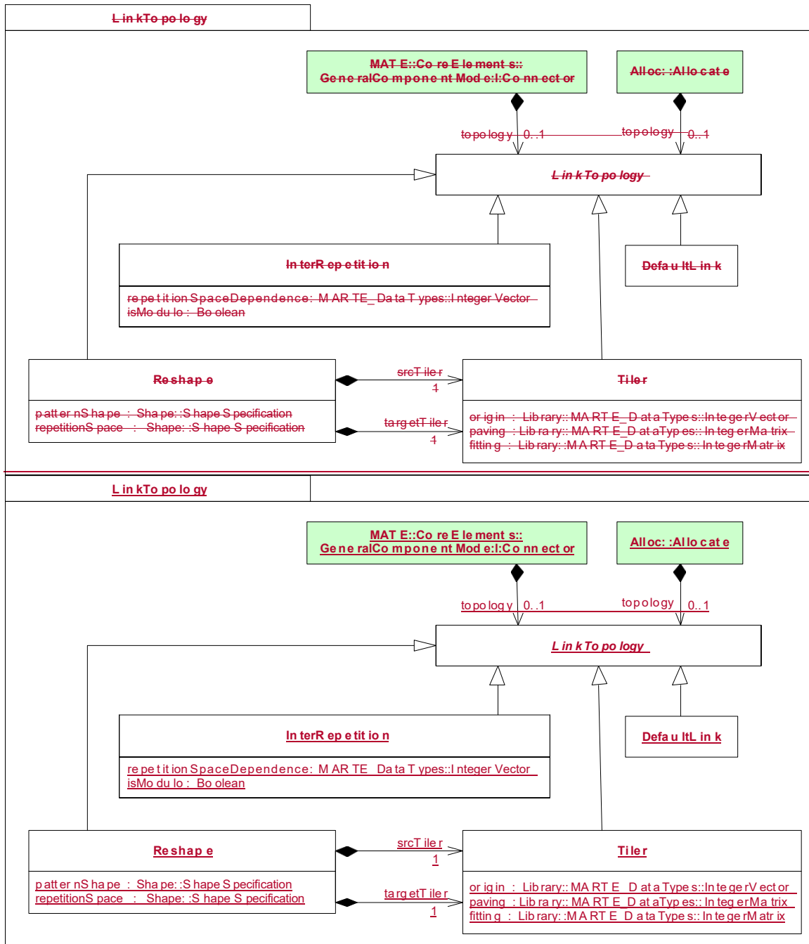
Figure E.3 - Link topology modeling concepts
