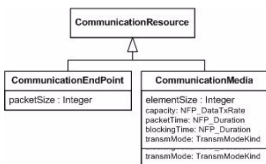
Figure 10.8 - Kinds of Communication resource in the ResourceTypeResourceTypes package
