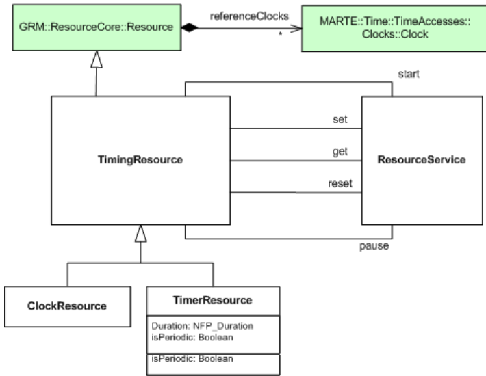
Figure 10.7 - Timing resources
