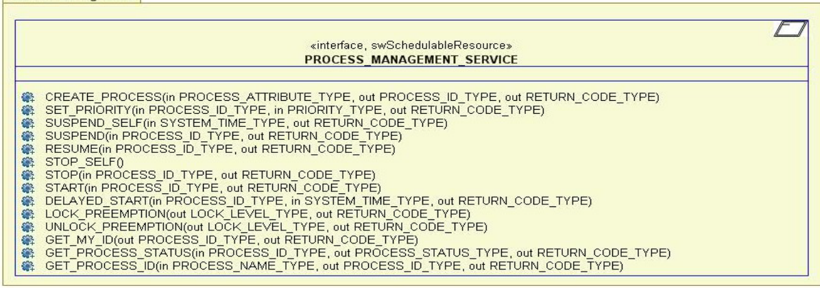
Figure D.24 - ARINC-653 PROCESS package
