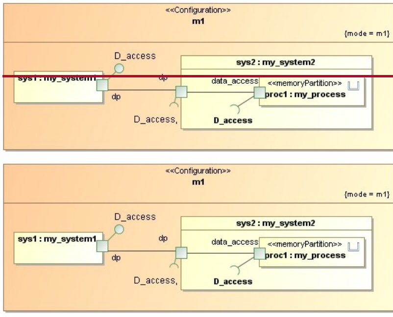
Figure A.10 - Data access mode specific example
