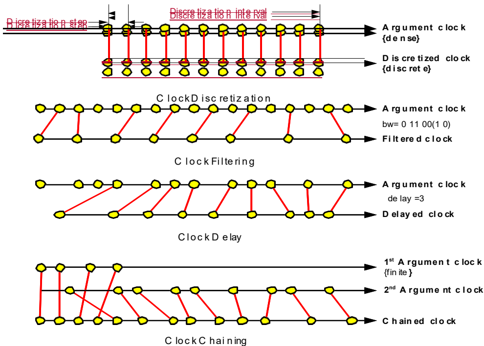
Figure C.3 - Examples of clock expressions
