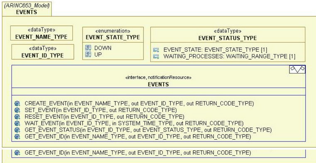
Figure D.31 - ARINC-653 Events package
