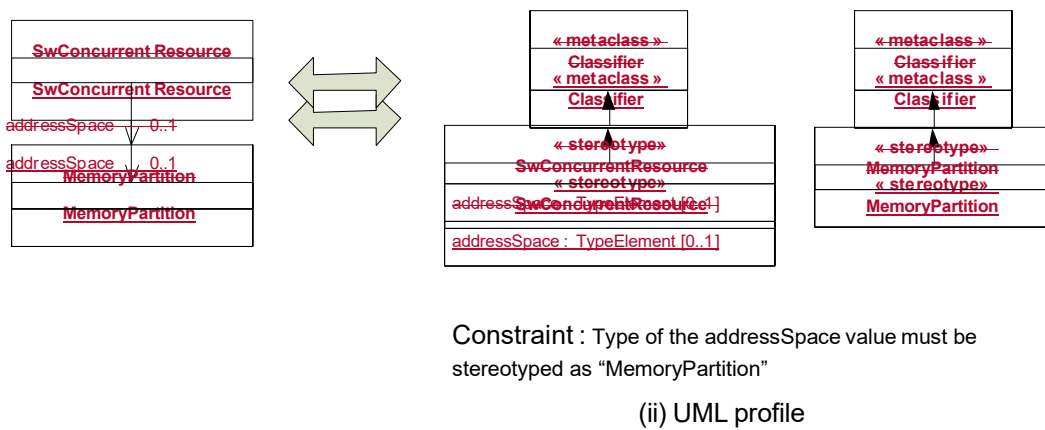
Figure 14.22 - SRM Matched rule on Associations
