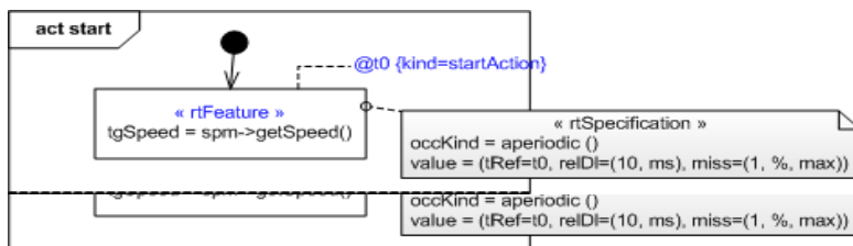
Figure 13.14 - An example of call action with a deadline real-time feature
