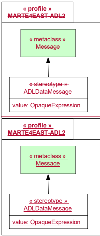
Figure A.14 - UML profile diagram for EAST-ADL2 data-based message
