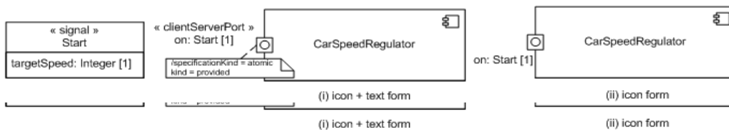
Figure 12.11 - Example of atomic client-server port
