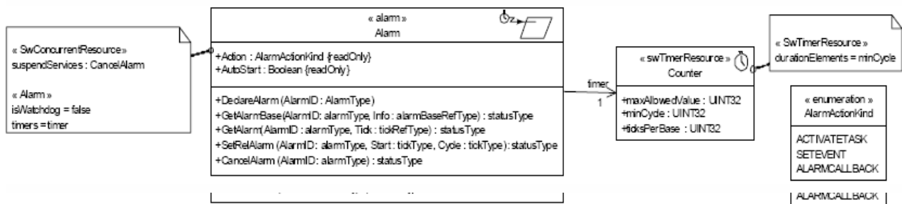
Figure 14.49 - OSEK/VDX Alarm example
