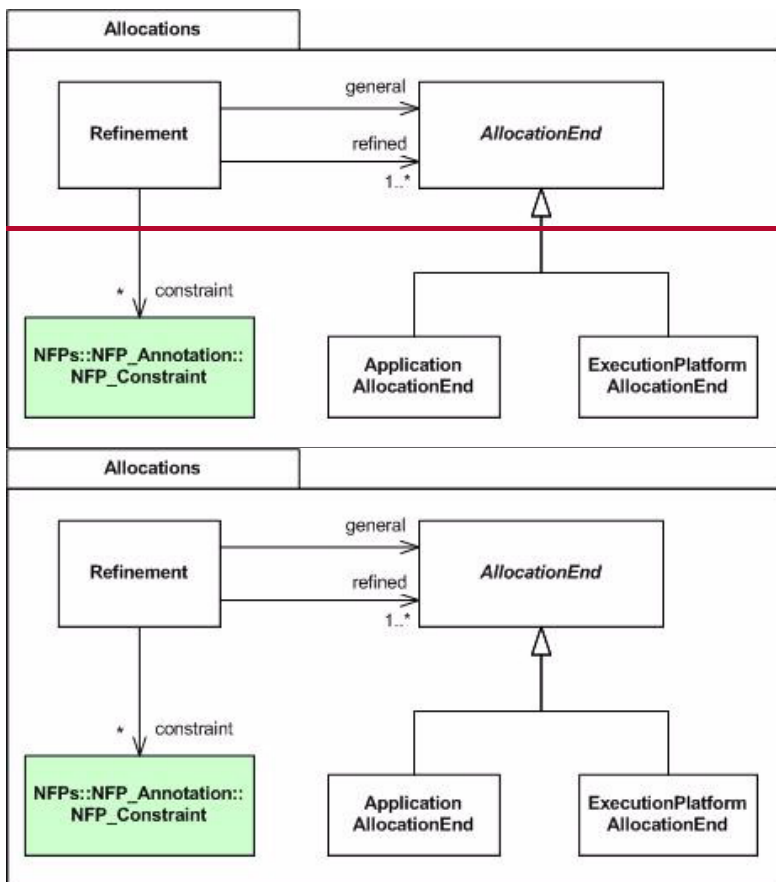
Figure 11.2 - The Refinement model
