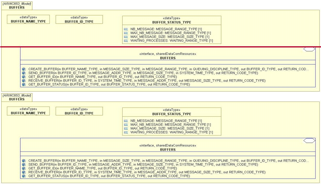
Figure D.28 - ARINC-653 Buffers package
