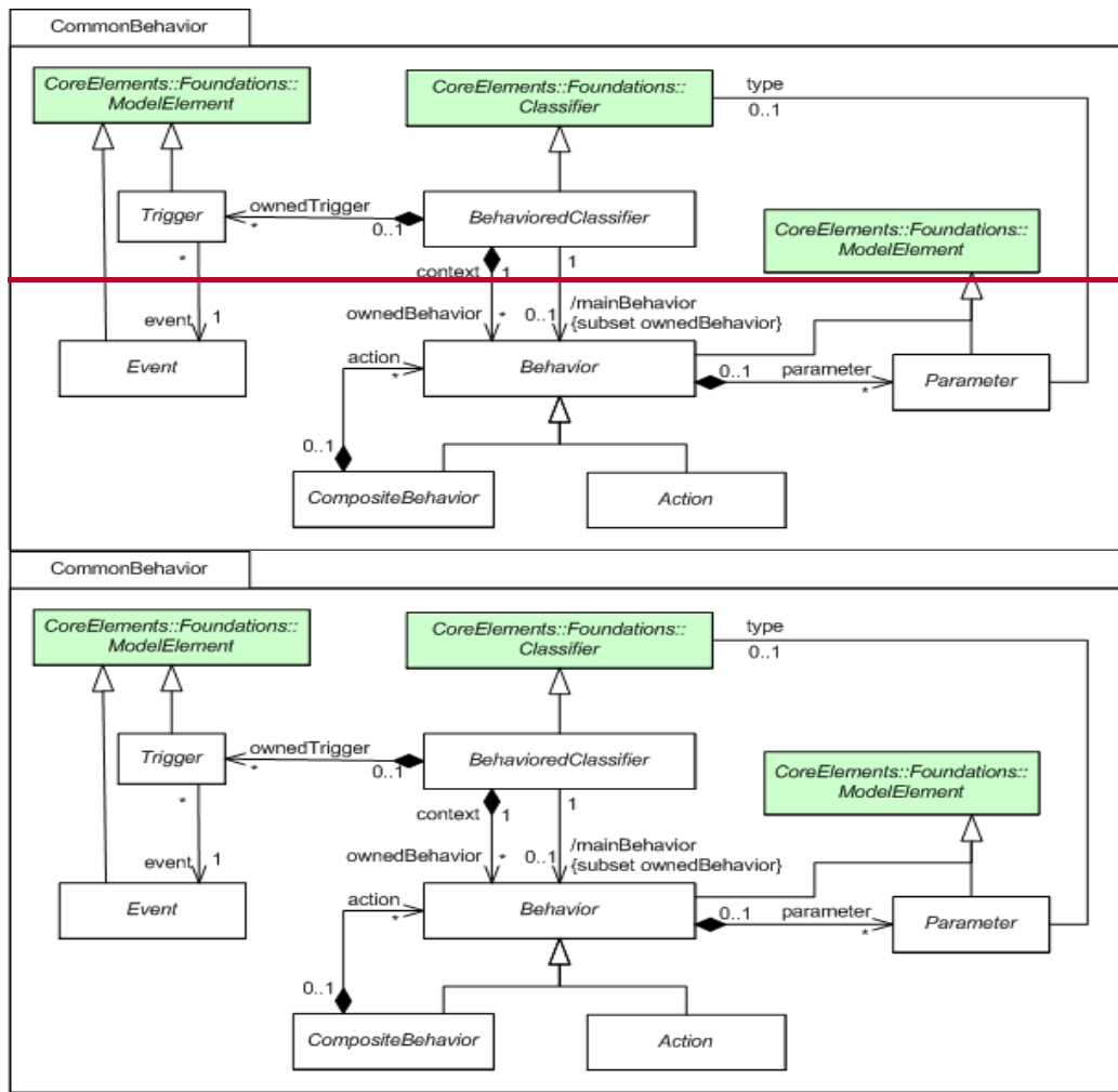
Figure 7.5 - The CommonBehavior package
