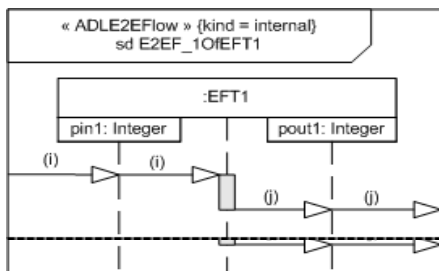
Figure A.19 - Example 1 of an EAST- ADL2 internal end-to-end flow for an elementary ADLFunctionType
