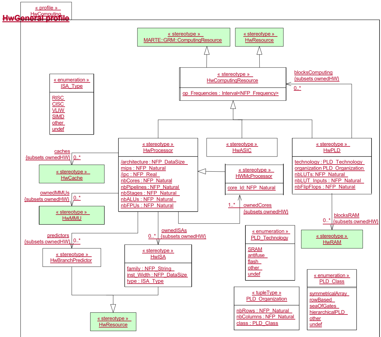
Figure 14.66 - HwComputing package details
