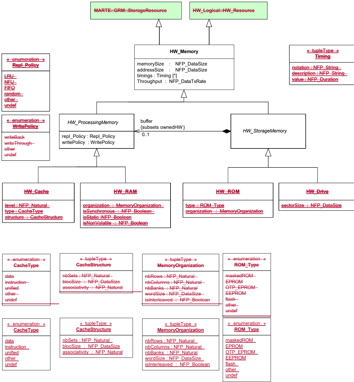
Figure 14.56 - HW_Storage package details (HW_Memory)
