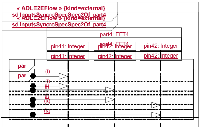
Figure A.36 - Step 1 for modeling a timed synchronization constraint
