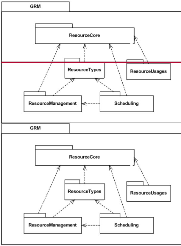
Figure 10.2 - Architecture of the GeneralResourceModel (GRM) package
