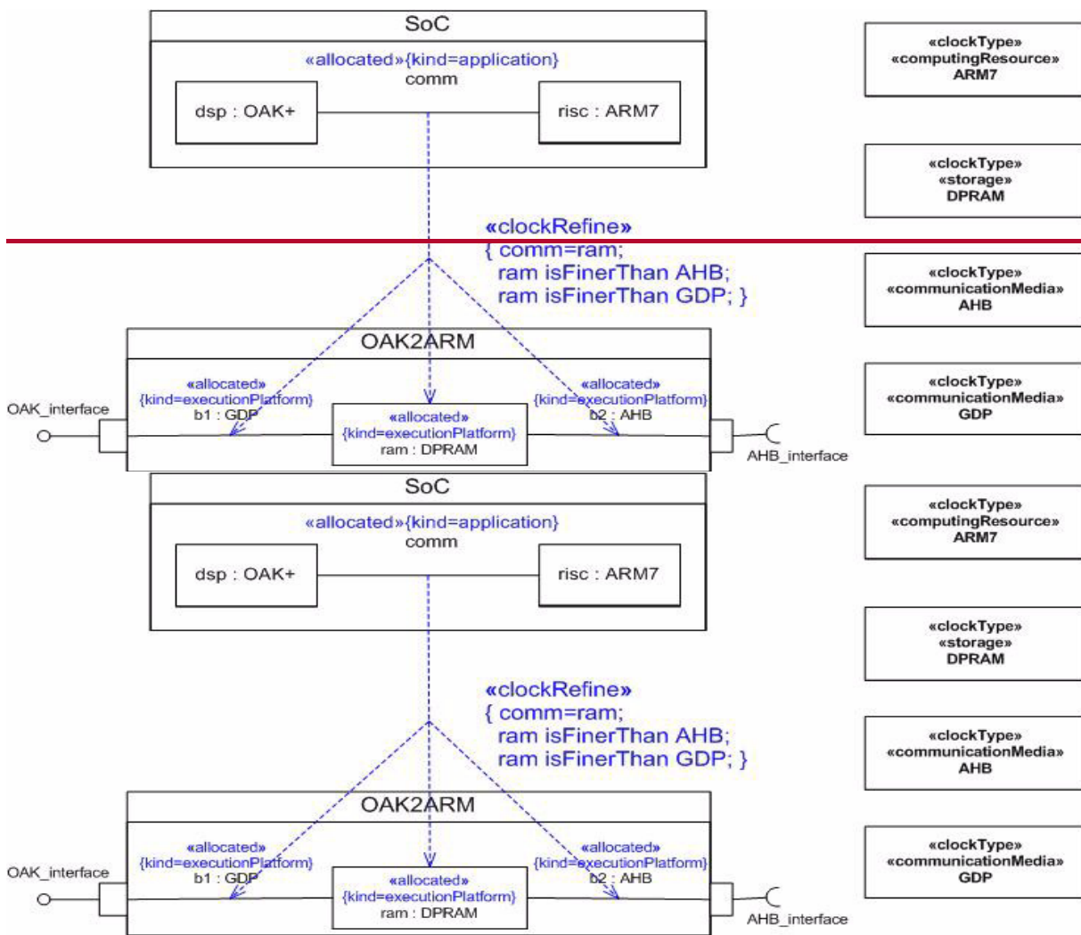
Figure 11.9 - Communication refinement
