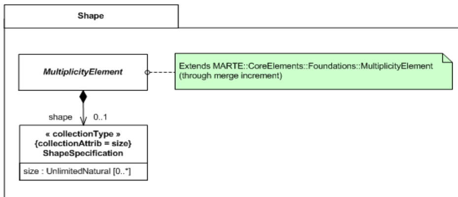
Figure E.2 - Shape modeling concepts
