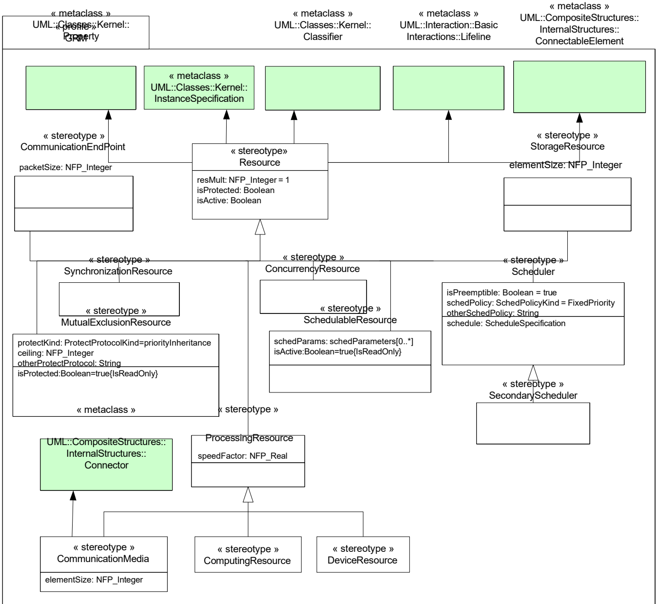
Figure 10.14 - UML extensions for GeneralResourceModeling
