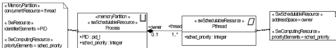
Figure 14.47 - POSIX Process and Pthread example
