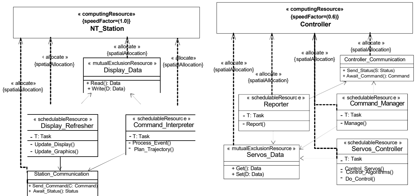
Figure 10.21 - Example of usage of the GRM Profile to annotate initial structural architectural choices
