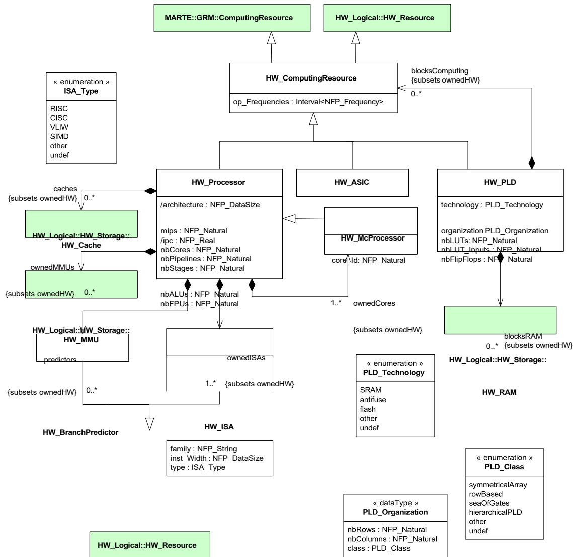
Figure 14.55 - HW_Computing package details
