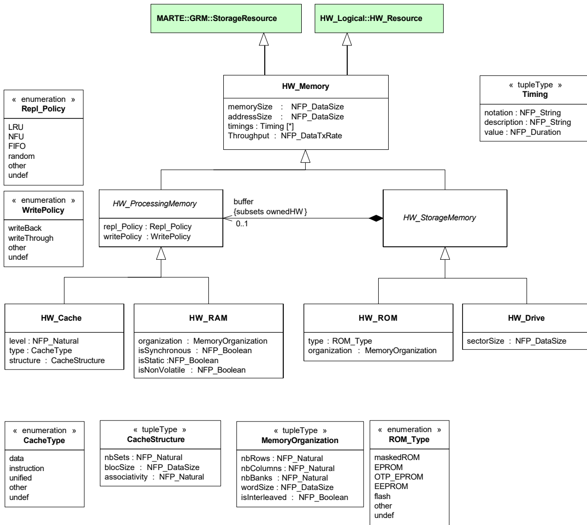
Figure 14.56 - HW_Storage package details (HW_Memory)
