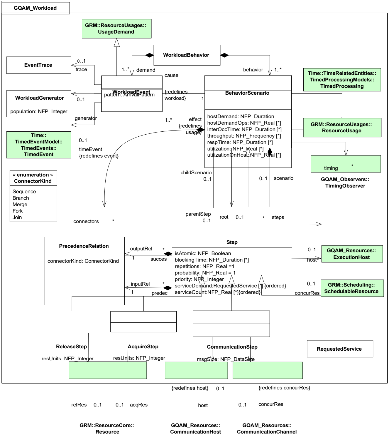
Figure 15.3 - GQAM_Workload package of the GQAM domain model
