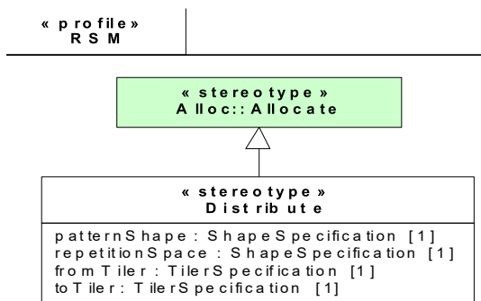
Figure E.7 - Profile diagram for distribution modeling
