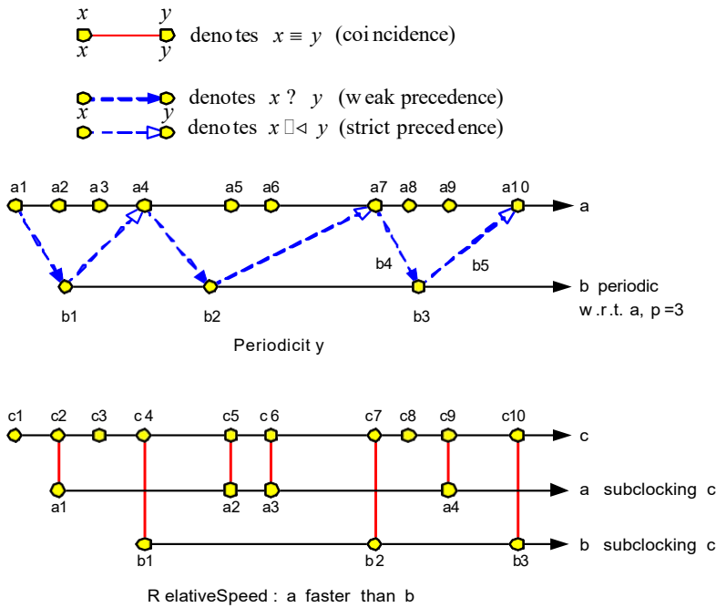
Figure C.4 - Examples of clock relations
