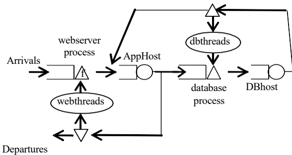
Figure 17.12 - Extended Queueing Network diagram
