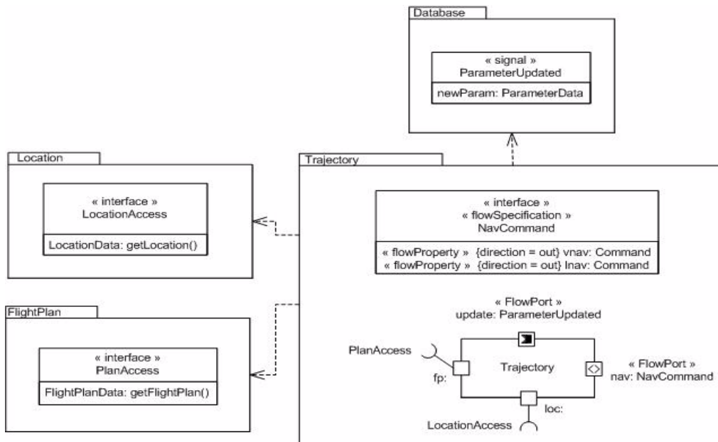
Figure 12.30 - Trajectory component definition
