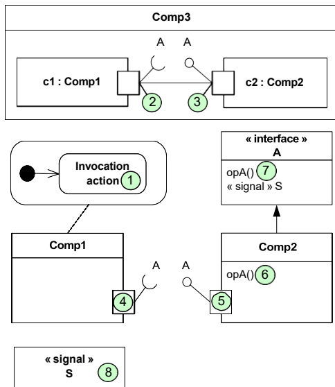
Figure 13.12 - RtFeature annotation possibilities and priority rules for interpretation of these annotations
