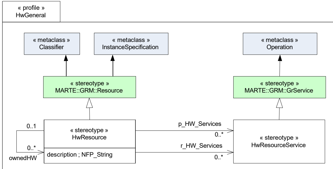
Figure 14.65 - HwGeneral profile details (HwLogical)
