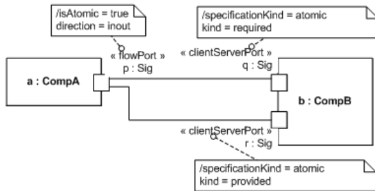
Figure 12.13 - Combined usage of atomic FlowPorts with "atomic" ClientServerPorts
