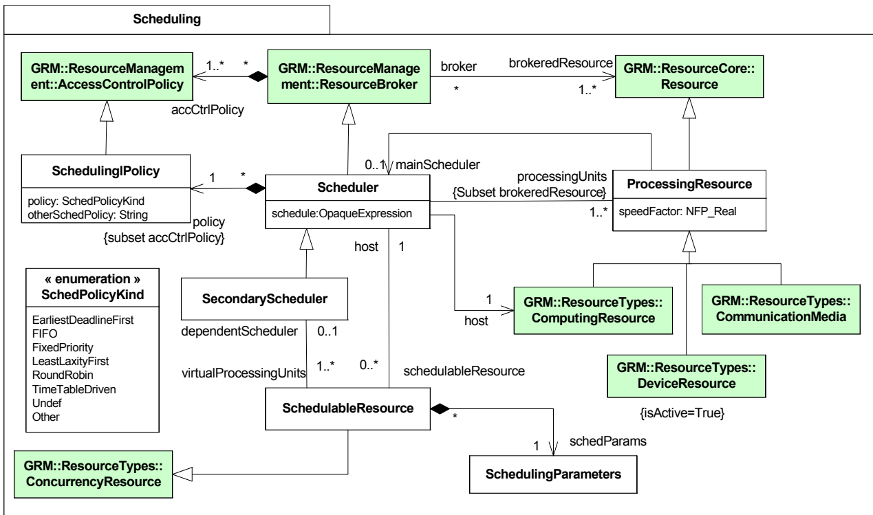
Figure 10.11 - The Scheduling package
