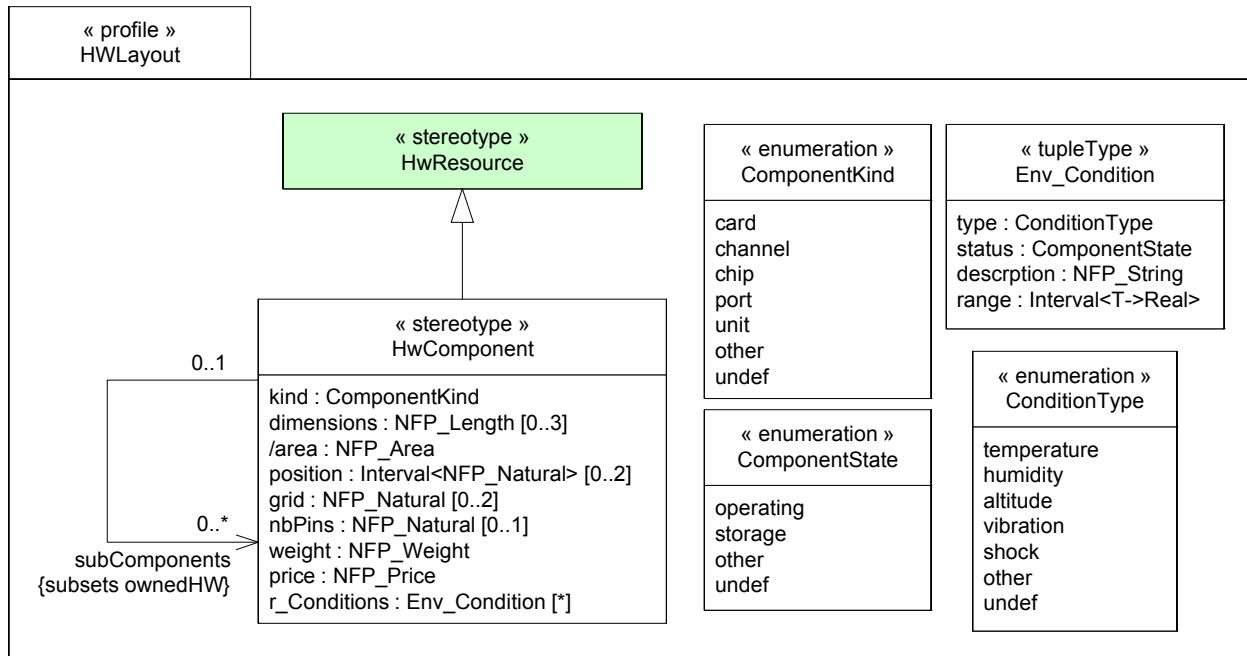
Figure 14.72 - HwLayout profile details-
