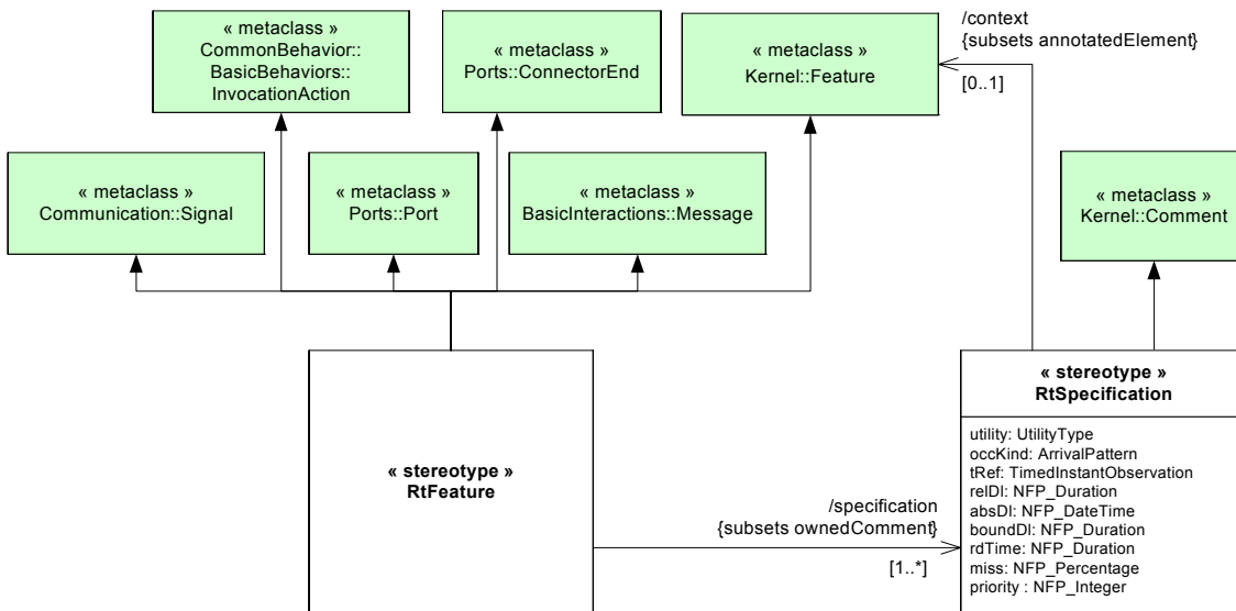
Figure 13.9 - RtFeature stereotype of the MARTE::HLAM sub-profile
