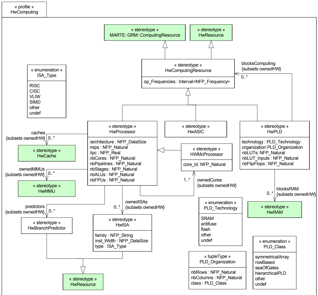
Figure 14.66 - HwComputing package details
