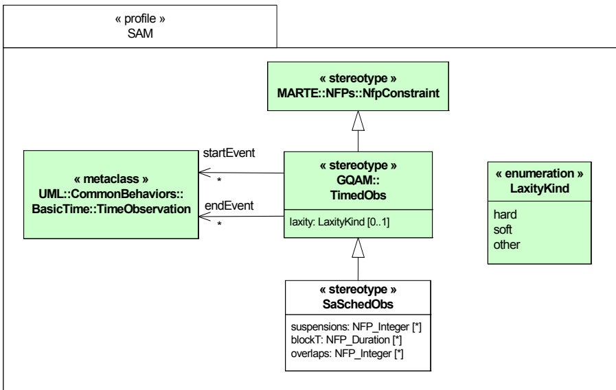
Figure 16.8 - The SAM Profile: Timed Observers
