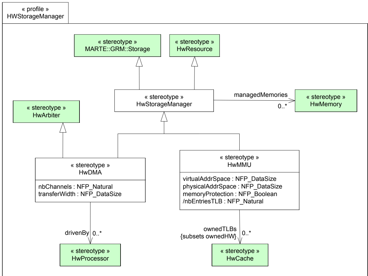
Figure 14.68 - HwStorageManager profile details (HwStorage)
