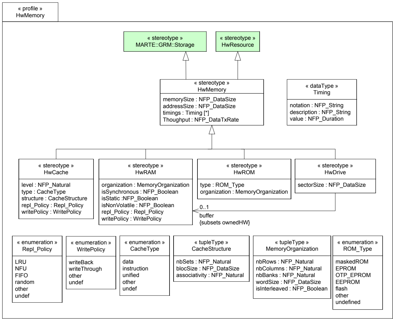
Figure 14.67 - HwMemory profile details (HwStorage)
