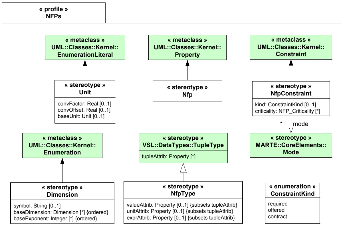
Figure 8.5 - UML profile diagram for NFPs modeling
