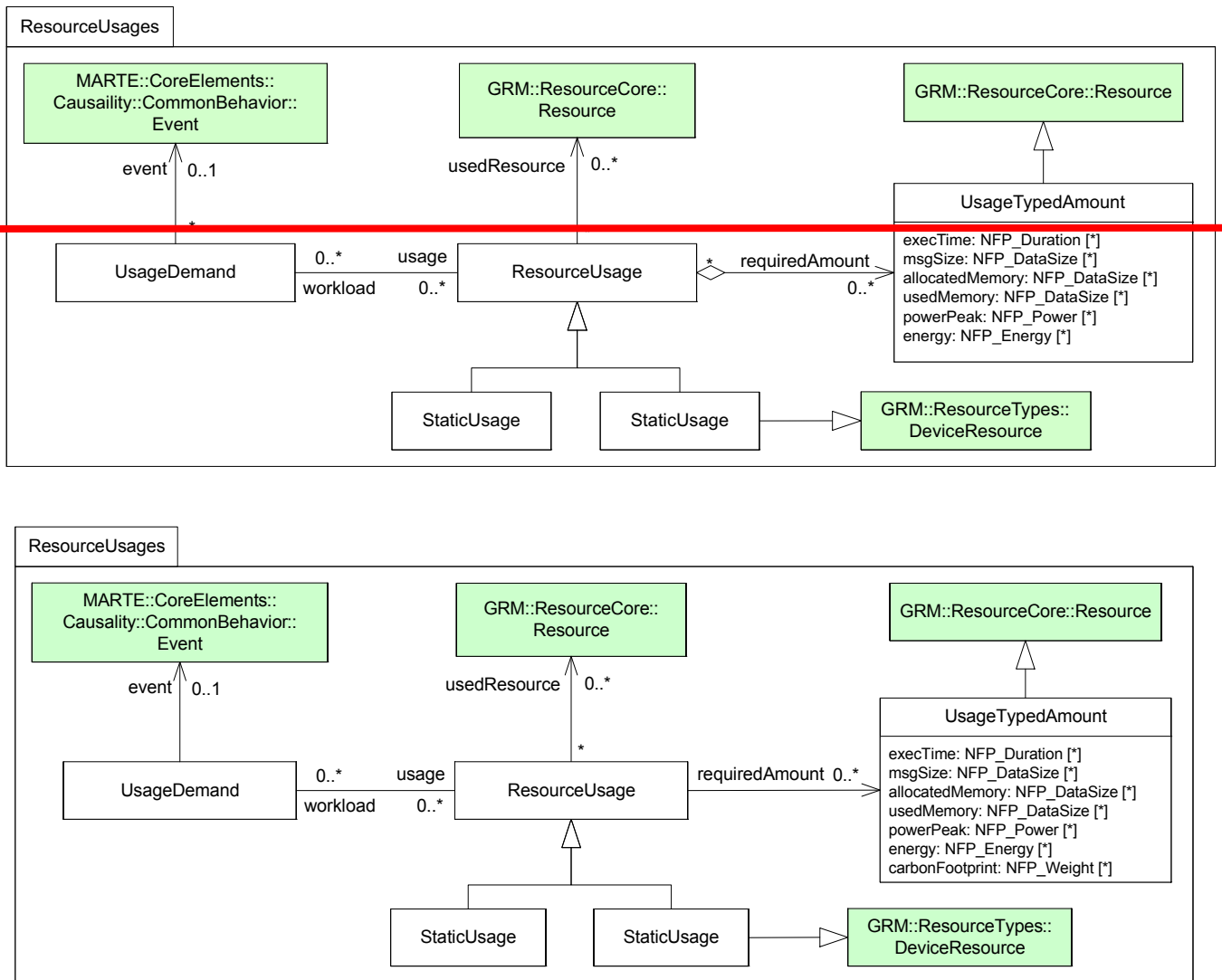
Figure 10.13 - Resource usage
