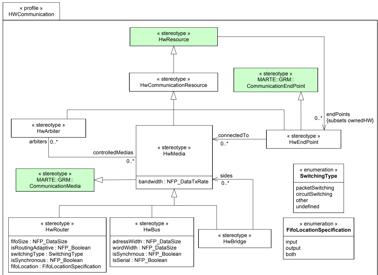
Figure 14.69 - HwCommunication profile details
