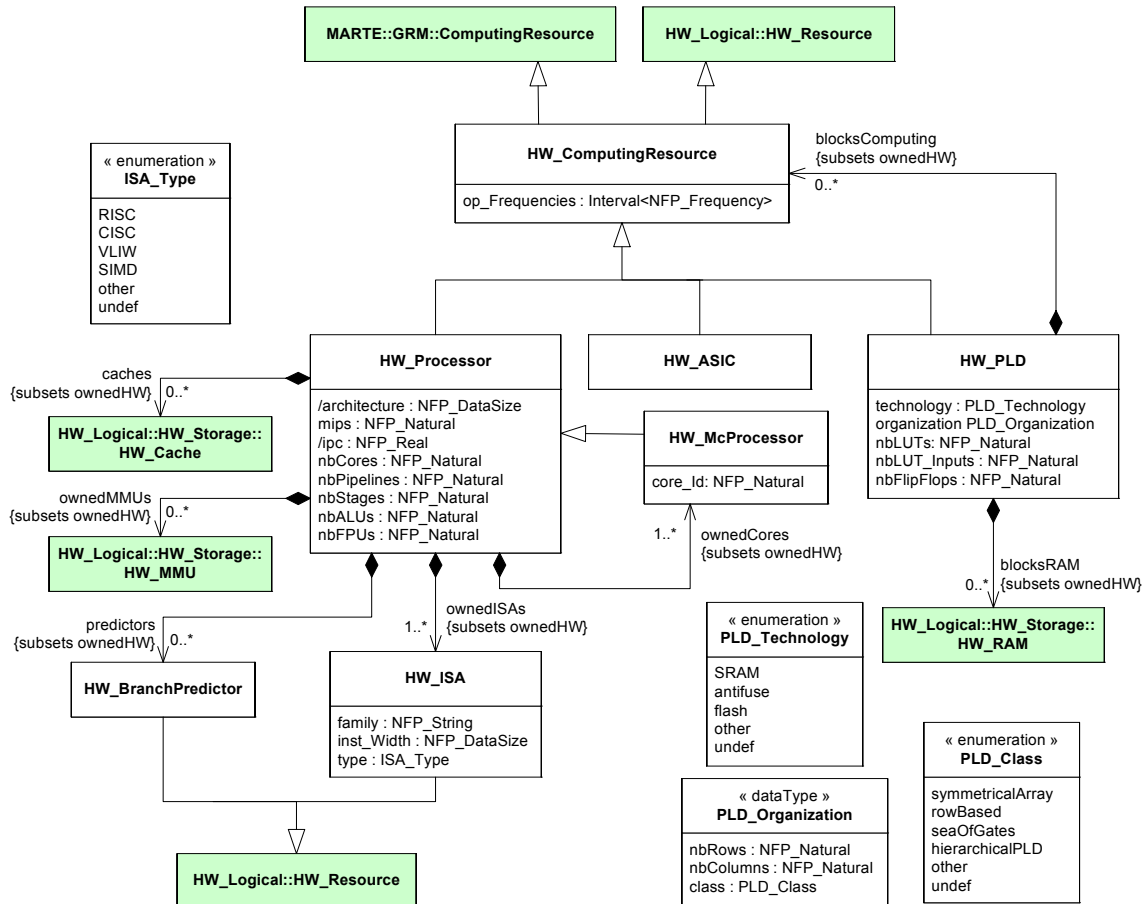
Figure 14.55 - HW_Computing package details
