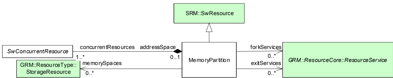
Figure 14.9 - The MemoryPartition resource
