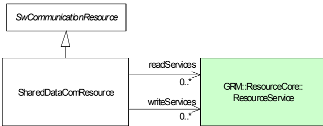
Figure 14.16 - The shared data communication resource
