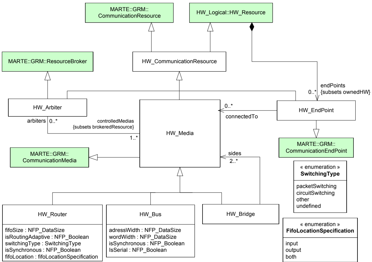
Figure 14.58 - HW_Communication package details
