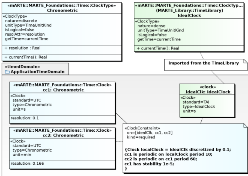
Figure 9.32 - Example of chronometric clocks
