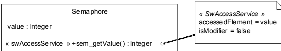
Figure 14.44 - SwAccessService example
