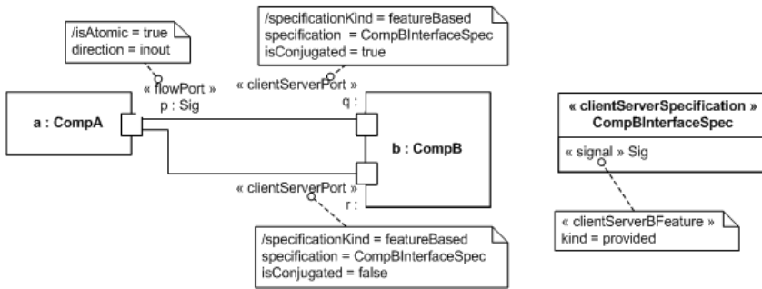
Figure 12.15 - Combined usage of atomic FlowPorts with "featureBased" ClientServerPorts
