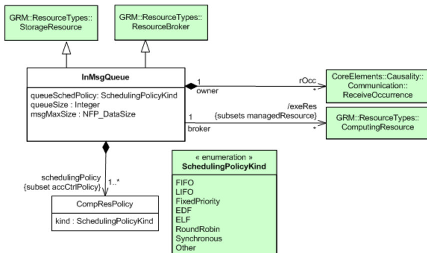
Figure 13.4 - InMsgQueue of the HLAM package
