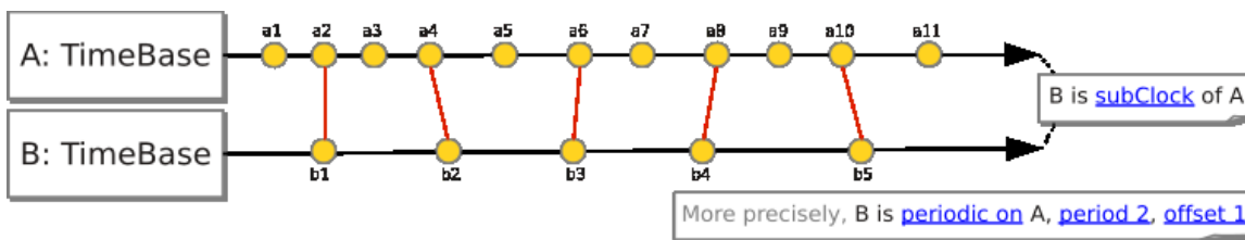
Figure 9.7 - Example of time relations between two time bases
