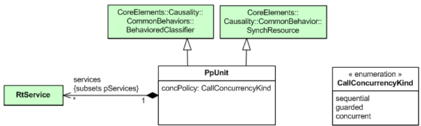
Figure 13.3 - PpUnit of the HLAM package
