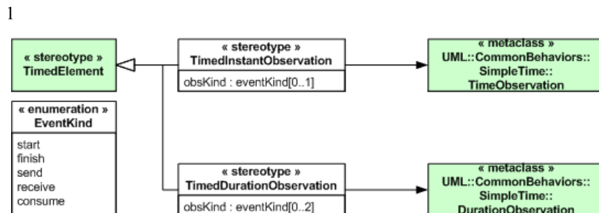
Figure 9.29 - UML extensions for Time modeling (4)
