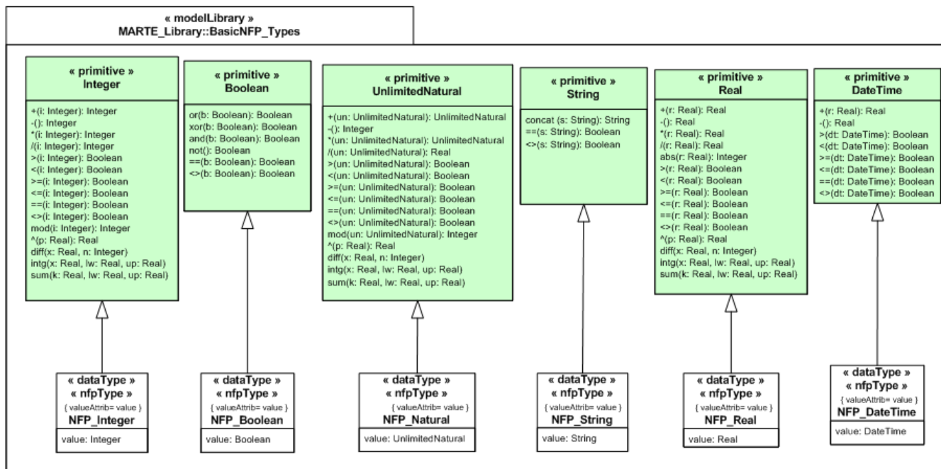
Figure D.7 - Inherited Operations for NfpTypes
