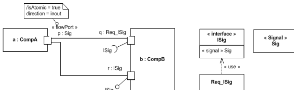
Figure 12.12 - Combined usage of atomic FlowPorts with standard UML ports
