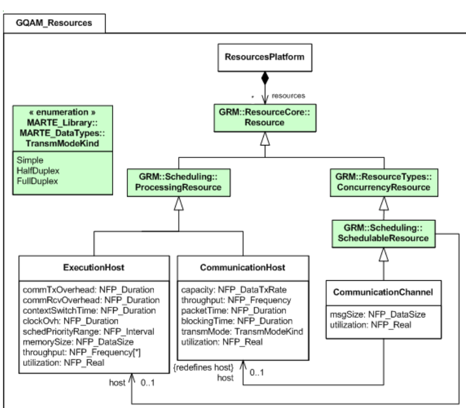
Figure 15.5 - GQAM_resources package of the GQAM domain model
