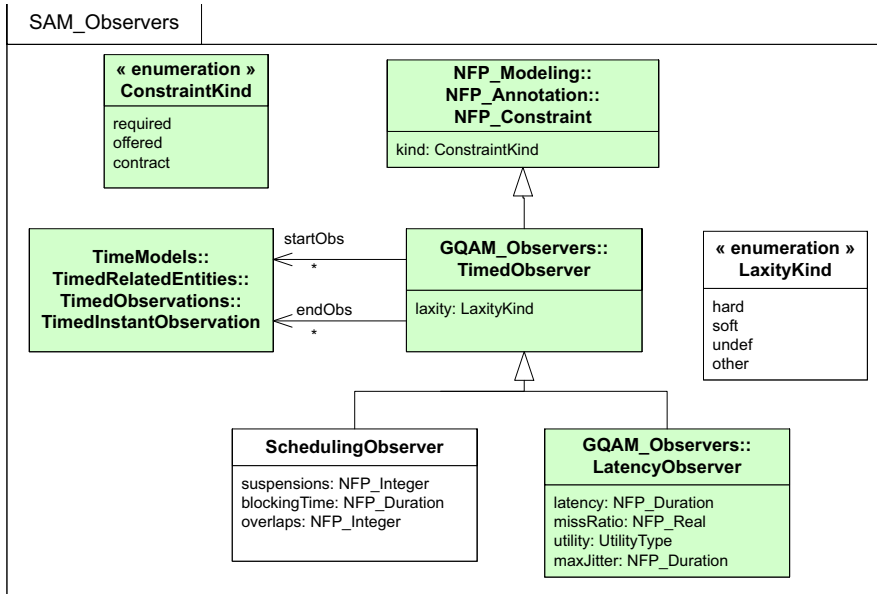
Figure 16.5 - The SAM Observers domain model
