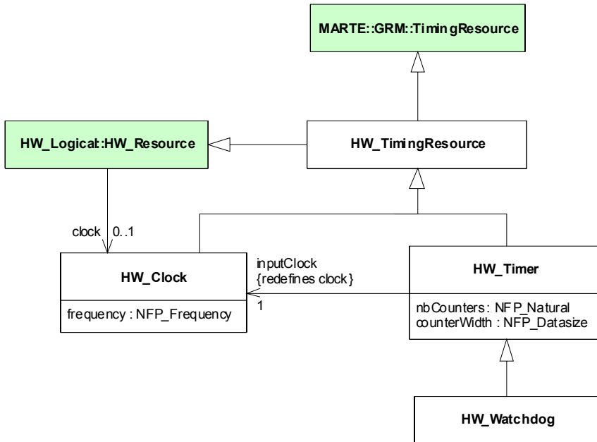
Figure 14.59 - HW_Timing package details
