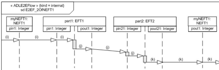
Figure A.26. Example 1 of an internal end-to-end flow for one non-elementary function
