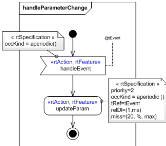
Figure 13.19 - A trajectory behavior that handles events from Database
