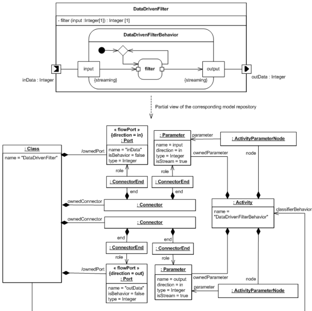
Figure 12.26 - Example 65, on the "push" form of the flow port semantics
