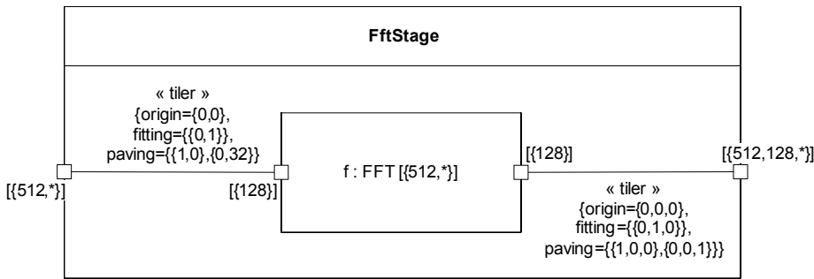
Figure E.8 - 2D repetition of a FFT component
