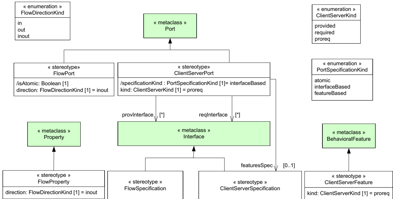
Figure 12.8 - UML profile of the MARTE GeneralComponentModel
