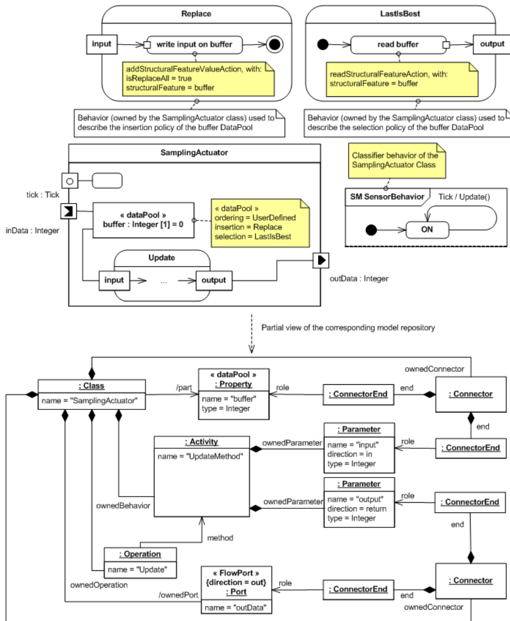
Figure 12.25 - Example 54, on the usage of the stereotype "DataPool" in the context of the "pull" form of the flow port semantics
