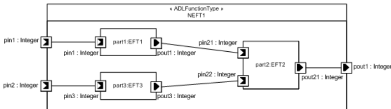
Figure A.25. Example of a non-elementary function type owning two elementary function prototypes
