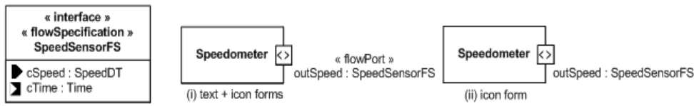
Figure 12.19 - Example of non-atomic flow port
