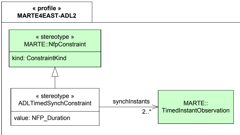
Figure A.31. UML profile diagram for EAST-ADL2 timed synchronization constraint
