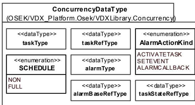
Figure D.14 - OSEK/VDX ConcurrencyDataType package
