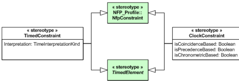
Figure 9.28 - UML extensions for Time modeling (3)
