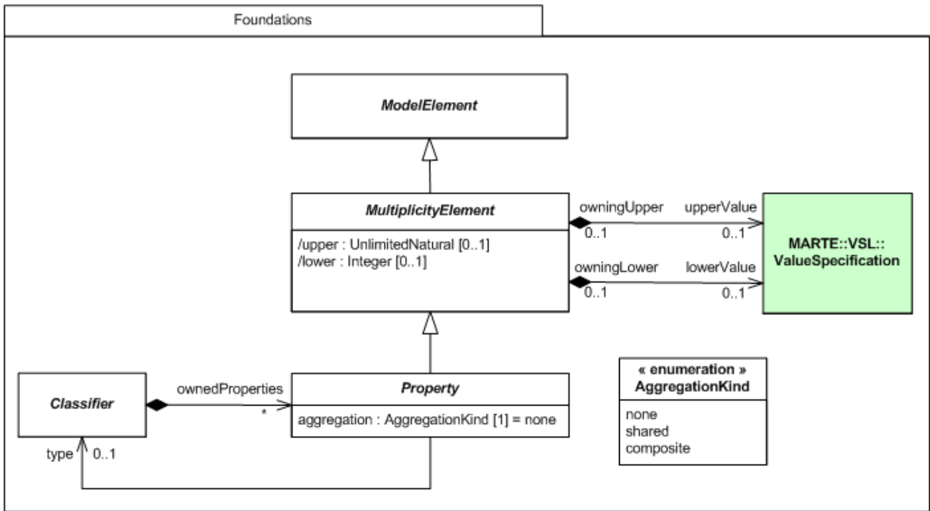
Figure 7.4 - Property diagram of the Foundations package
