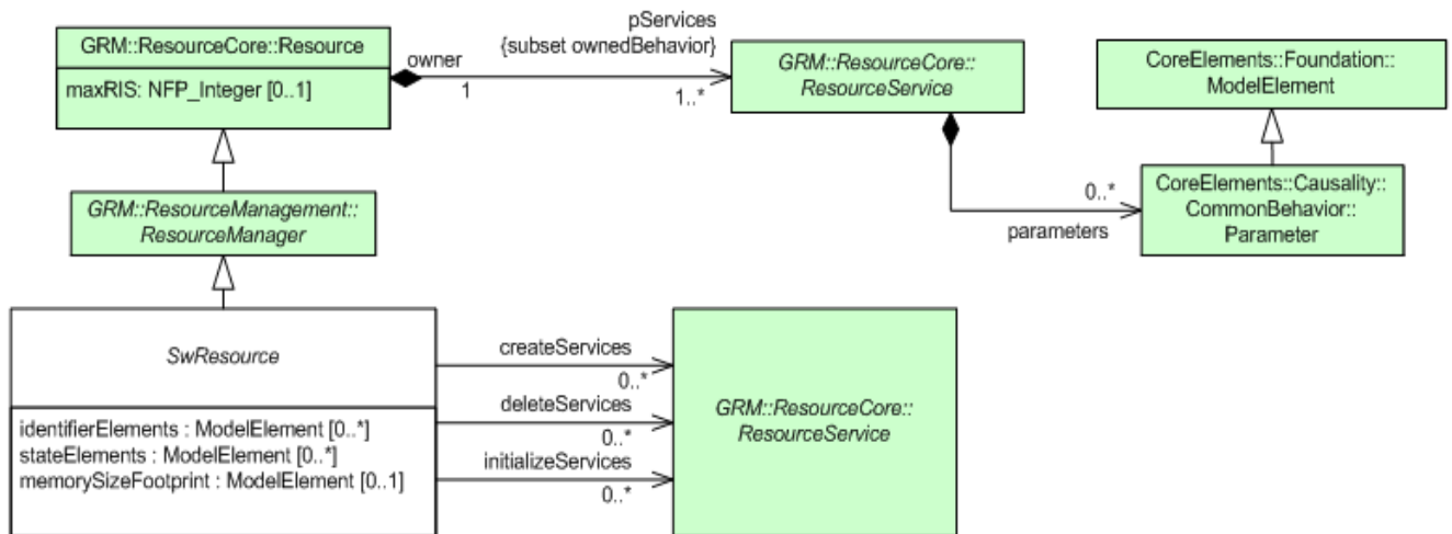
Figure 14.2 - The SW_ResourceCore package overview
