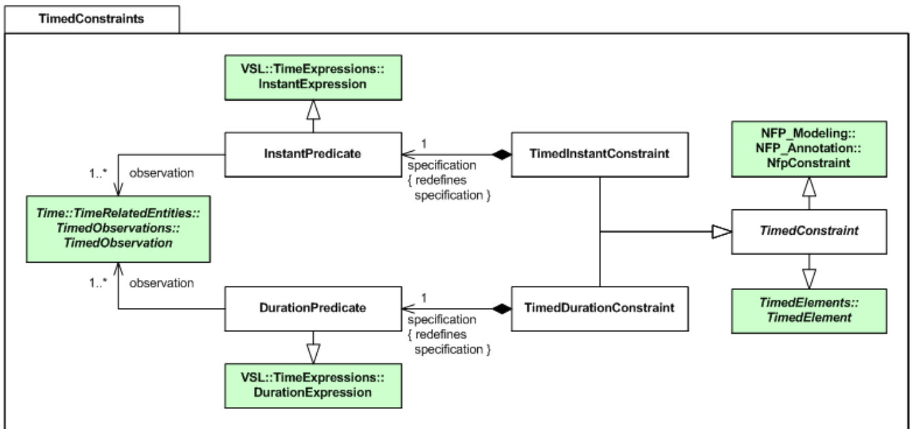
Figure 9.18 - TimedConstraints diagram of the time model
