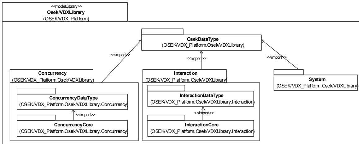
Figure D.12 - OSEK/VDX library overview
