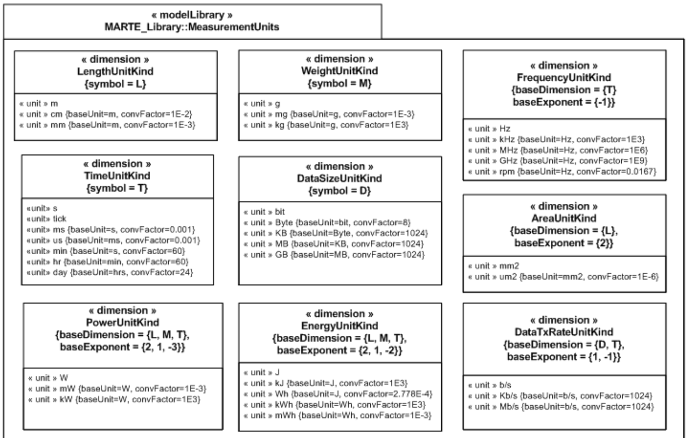
Figure D.3 - MARTE library of measurement units
