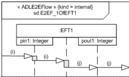
Figure A.22. Example 2 of an EAST- ADL2 internal end-to-end flow for an elementary ADLFunctionType
