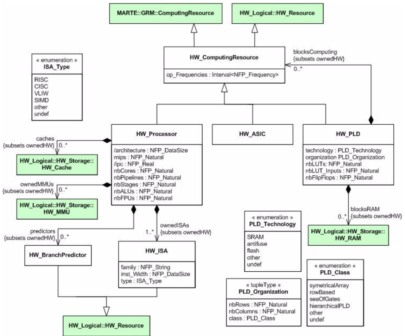
Figure 14.55 - HW_Computing package details
