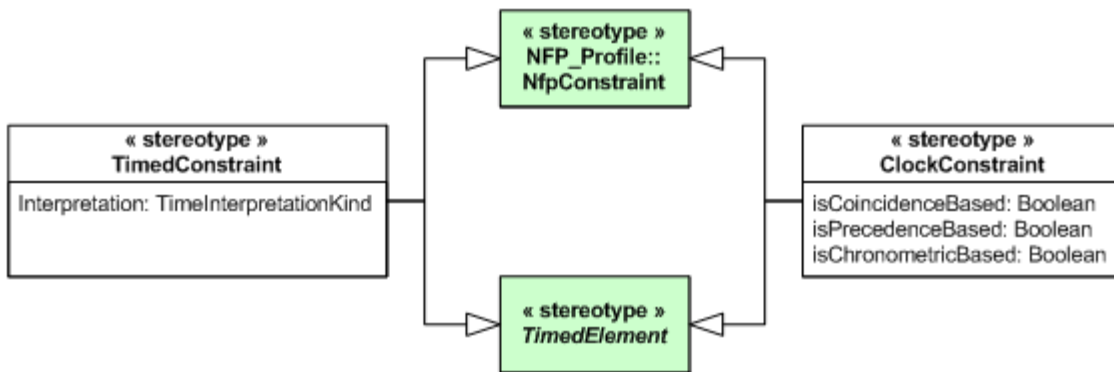
Figure 9.28 - UML extensions for Time modeling (3)
