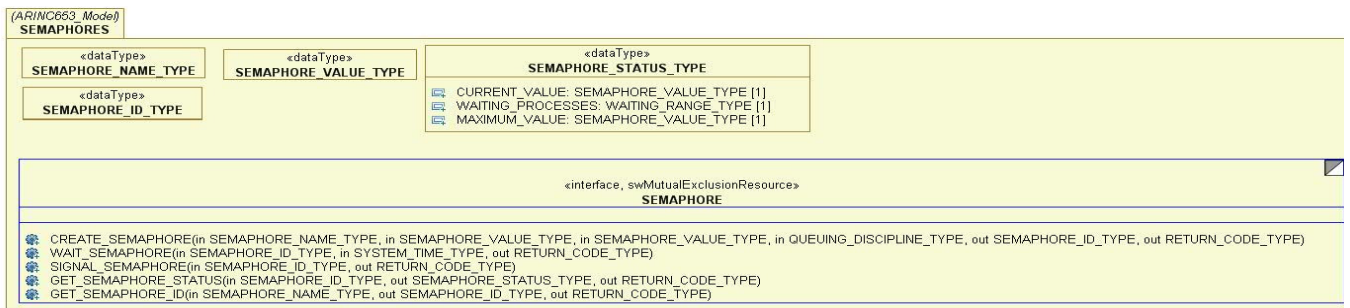
Figure D.30. ARINC-653 Semaphores package
