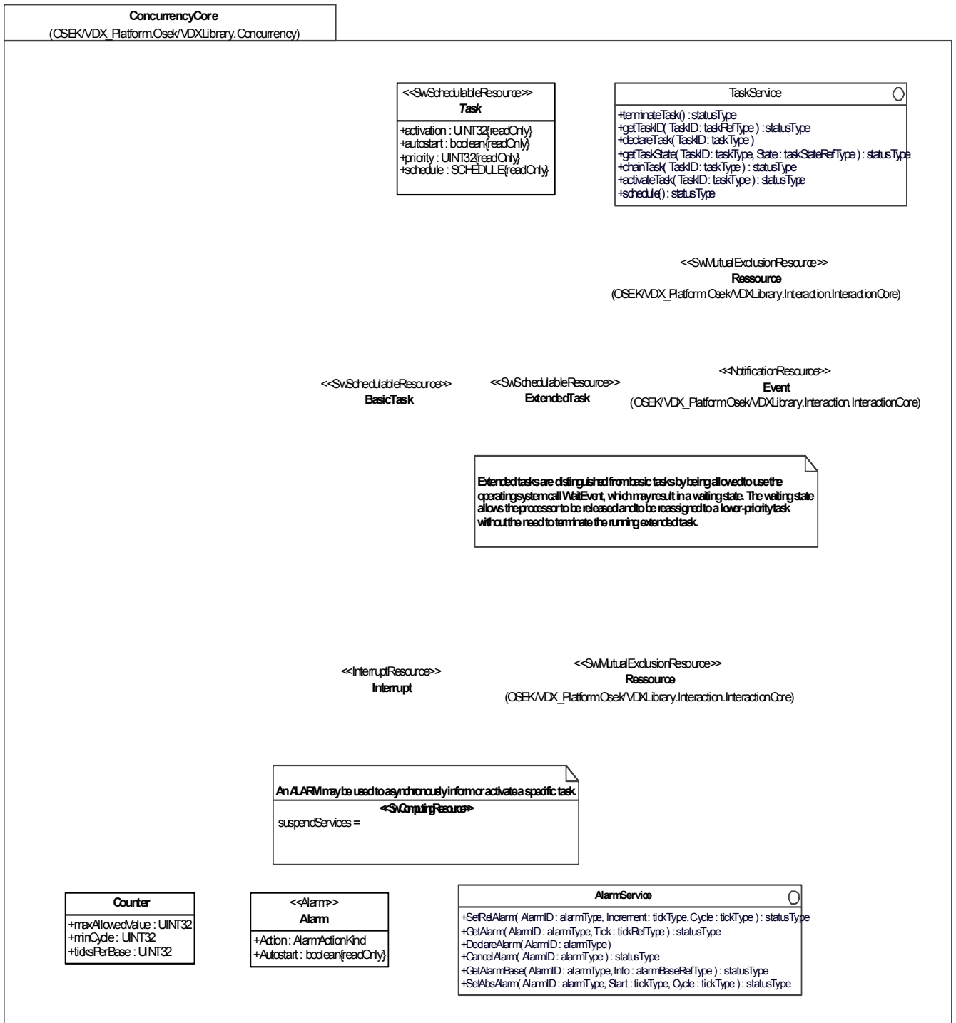
Figure D.15 - OSEK/VDX ConcurrencyCore package
