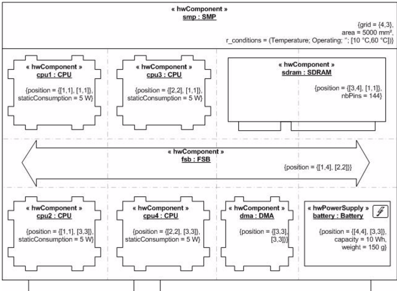
Figure 14.82 - SMP detailed physical model
