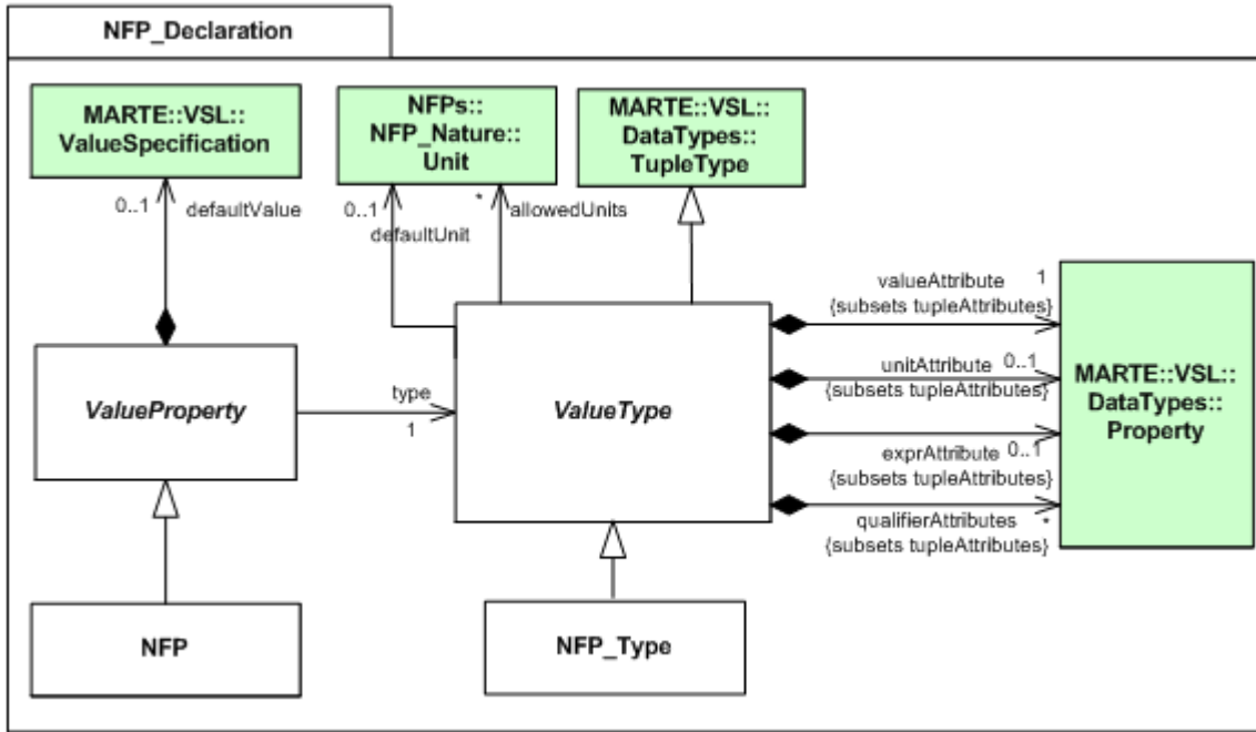
Figure 8.4 - Domain Model of NFP Declaration
