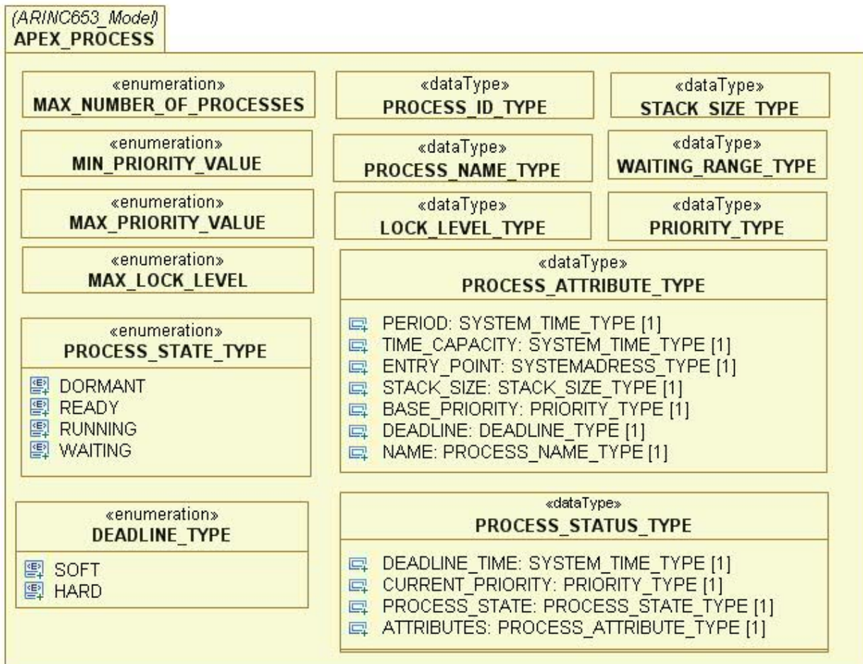
Figure D.22. ARINC-653 APEX PROCESS Types package
