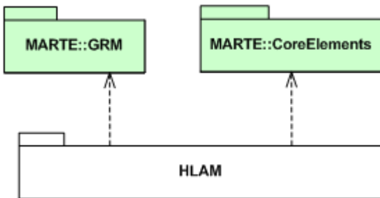
Figure 13.1 - Dependencies of the HLAM package
