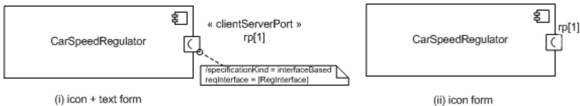
Figure 12.16 - Example of interface-based ClientServerPorts
