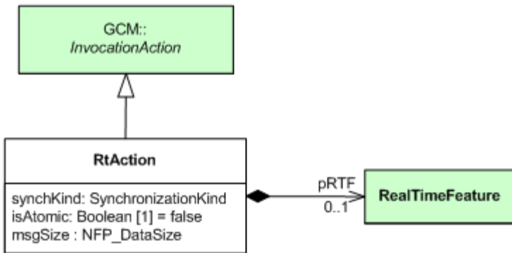
Figure 13.6 - RtAction of the HLAM package
