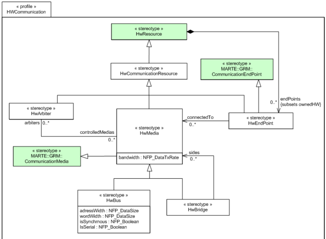
Figure 14.69 - HwCommunication profile details
