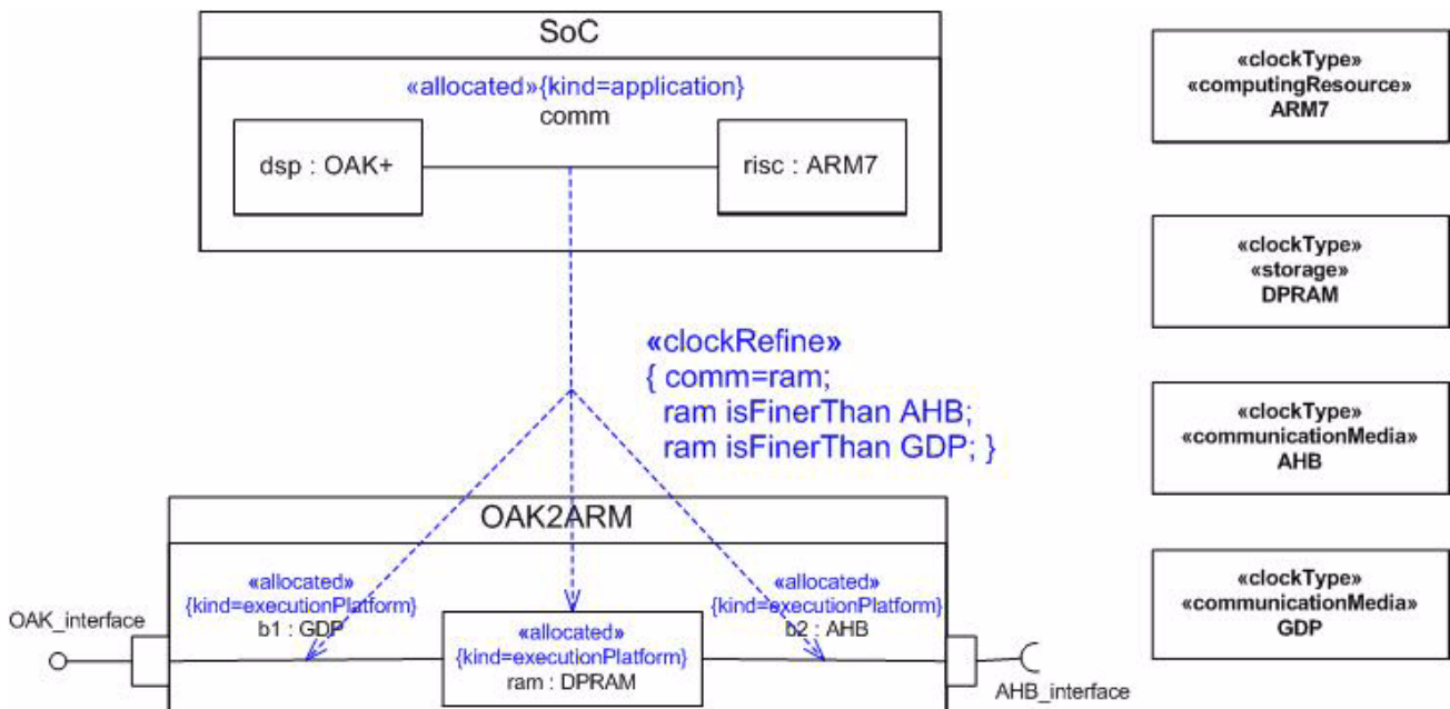
Figure 11.9 - Communication refinement
