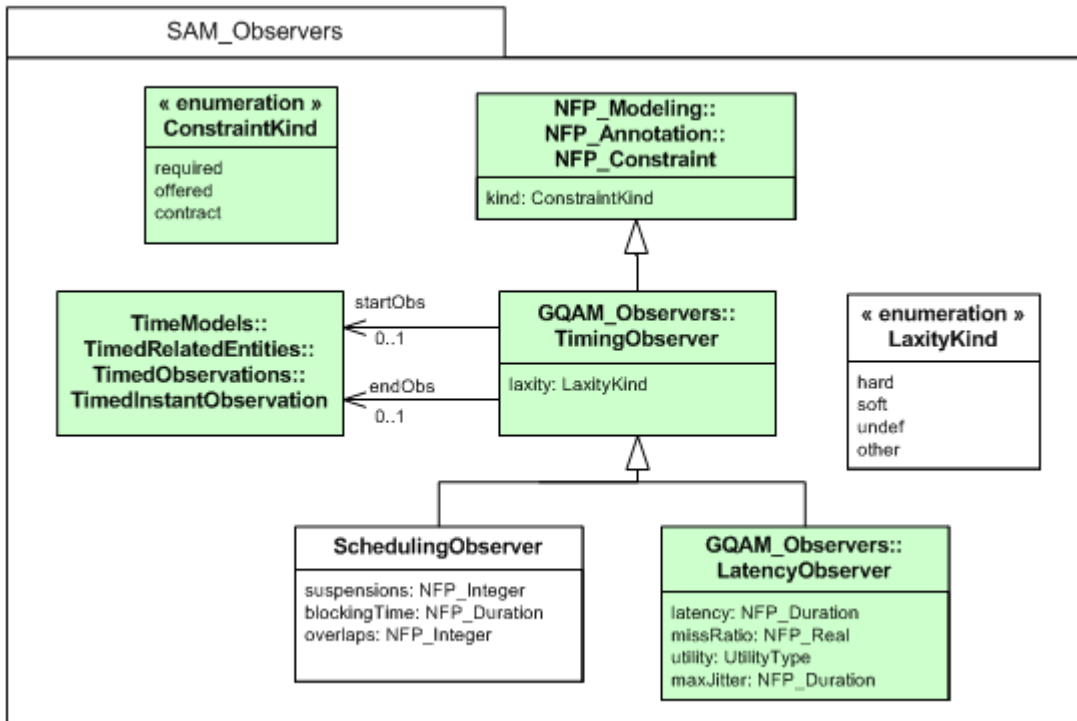
Figure 16.5 - The SAM Observers domain model
