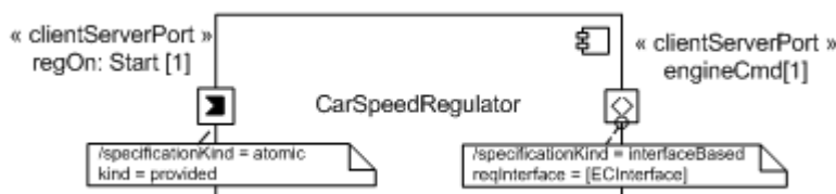
Figure 12.28 - Example of UML component with specialized MARTE ports
