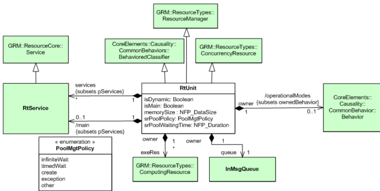
Figure 13.2 - RtUnit of the HLAM package
