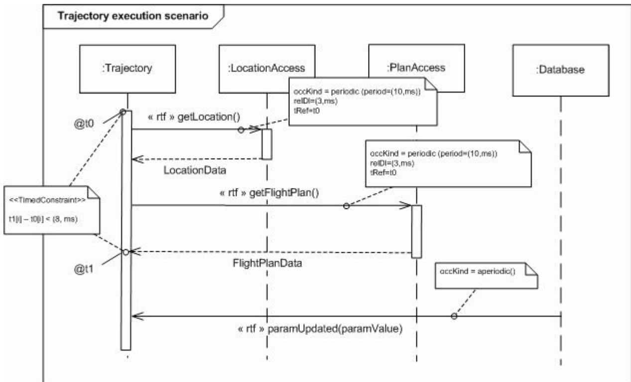
Figure 13.20 - A Trajectory execution scenario within a period
