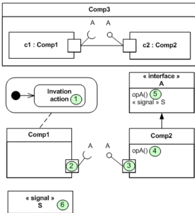
Figure 13.12 - RtFeature annotation possibilities and priority rules for interpretation of these annotations
