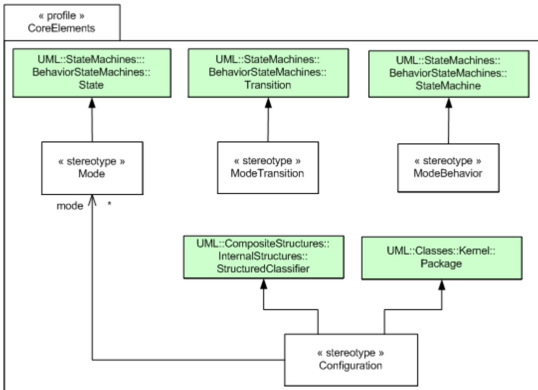
Figure 7.10 - UML profile diagram for CoreElements modeling
