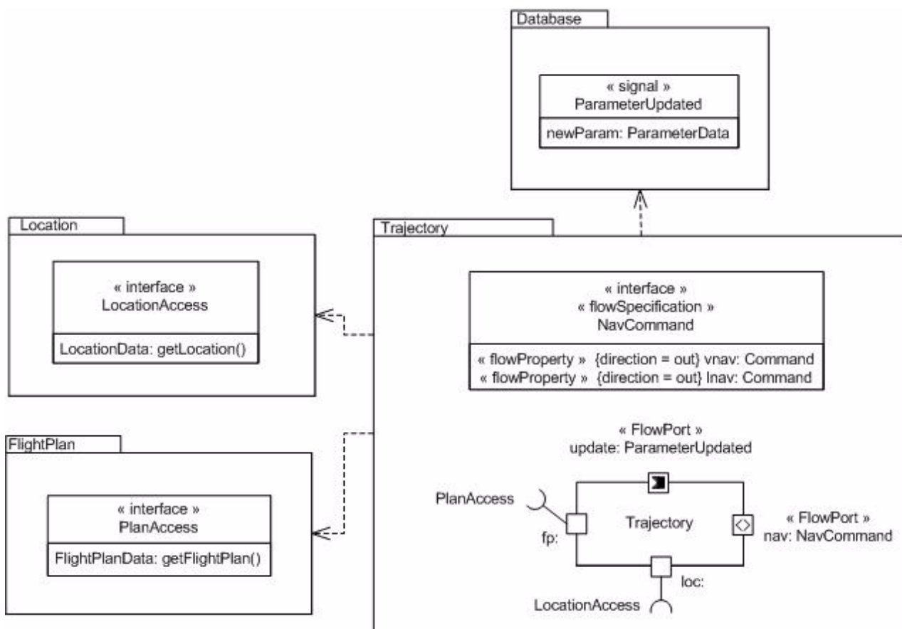
Figure 12.29 - Trajectory component definition
