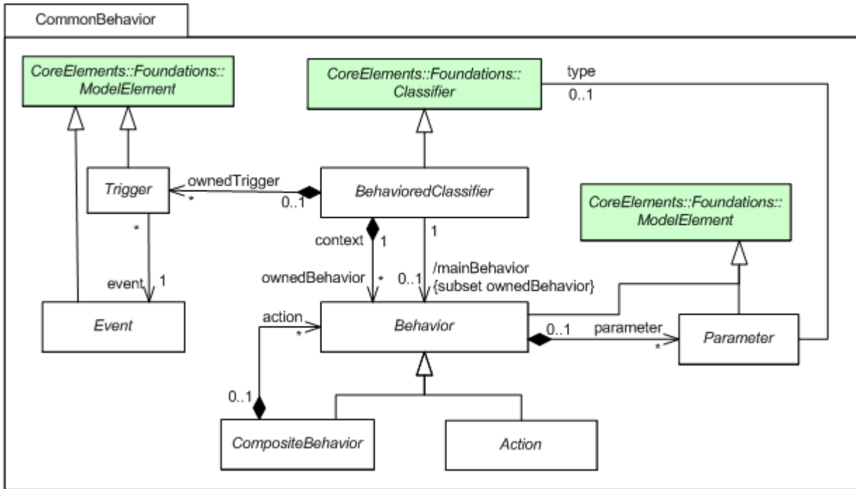
Figure 7.5 - The CommonBehavior package
