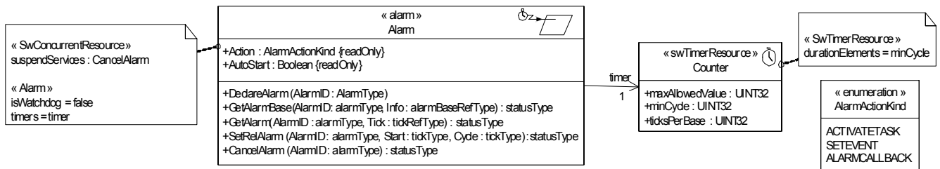
Figure 14.49 - OSEK/VDX Alarm example
