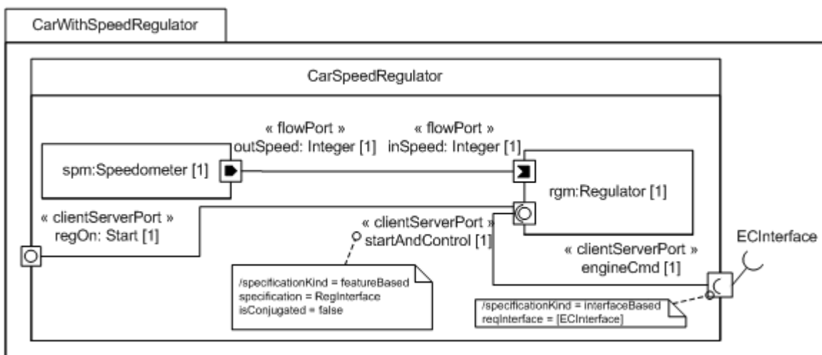
Figure 12.27 - Example of UML composite classes and parts with specialized MARTE ports
