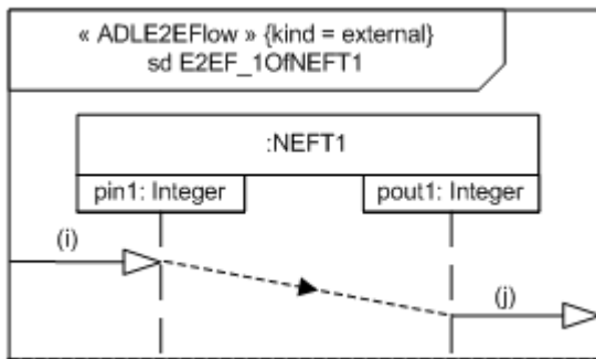
Figure A.25. End-to-end flow 1 for NEFT1
