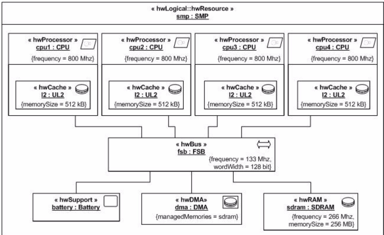
Figure 14.81 - SMP detailed logical model
