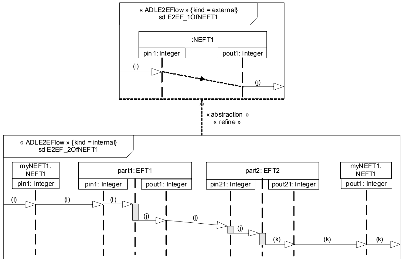
Figure A.32. Example of end-to-end flow refinement
