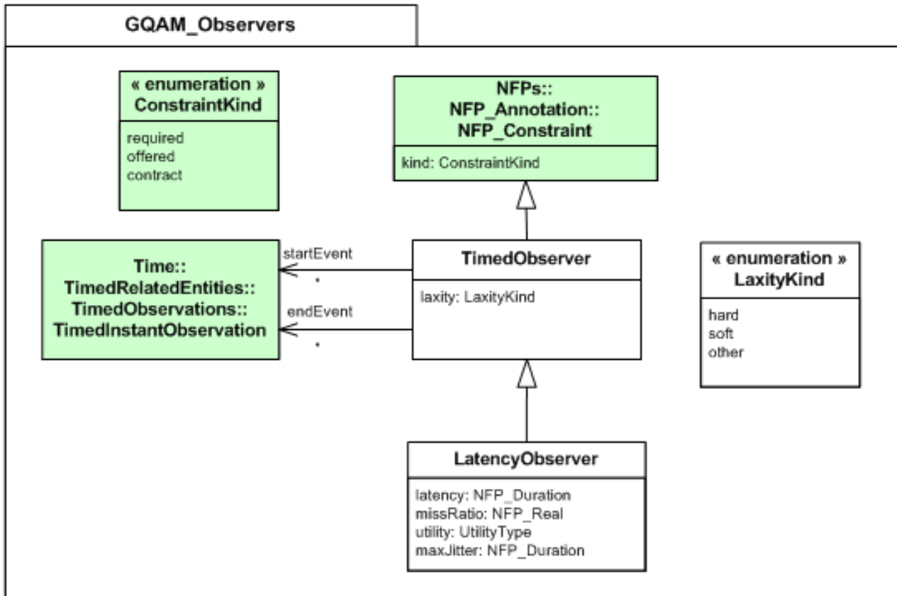
Figure 15.4 - The GQAM Observers package
