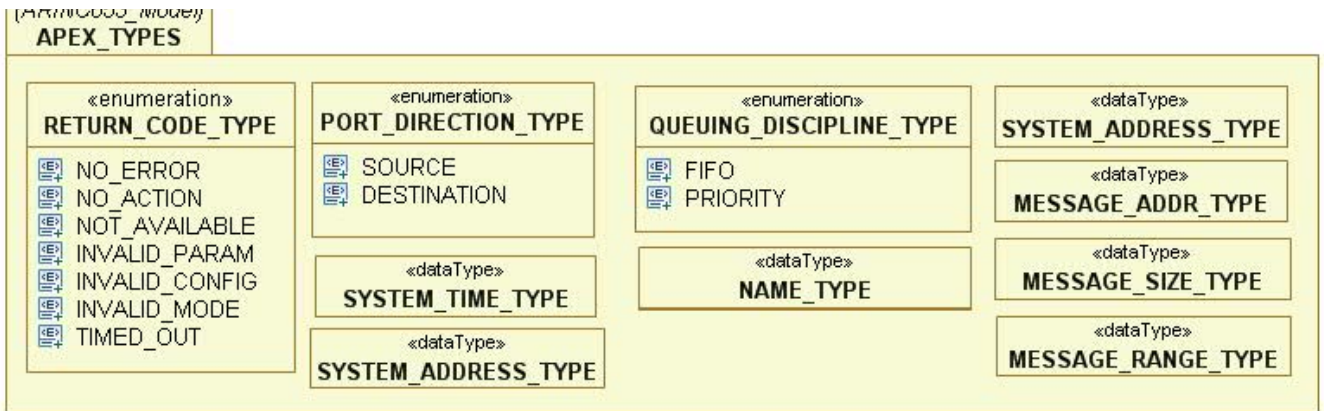
Figure D.21. ARINC-653 Generic APEX Types package
