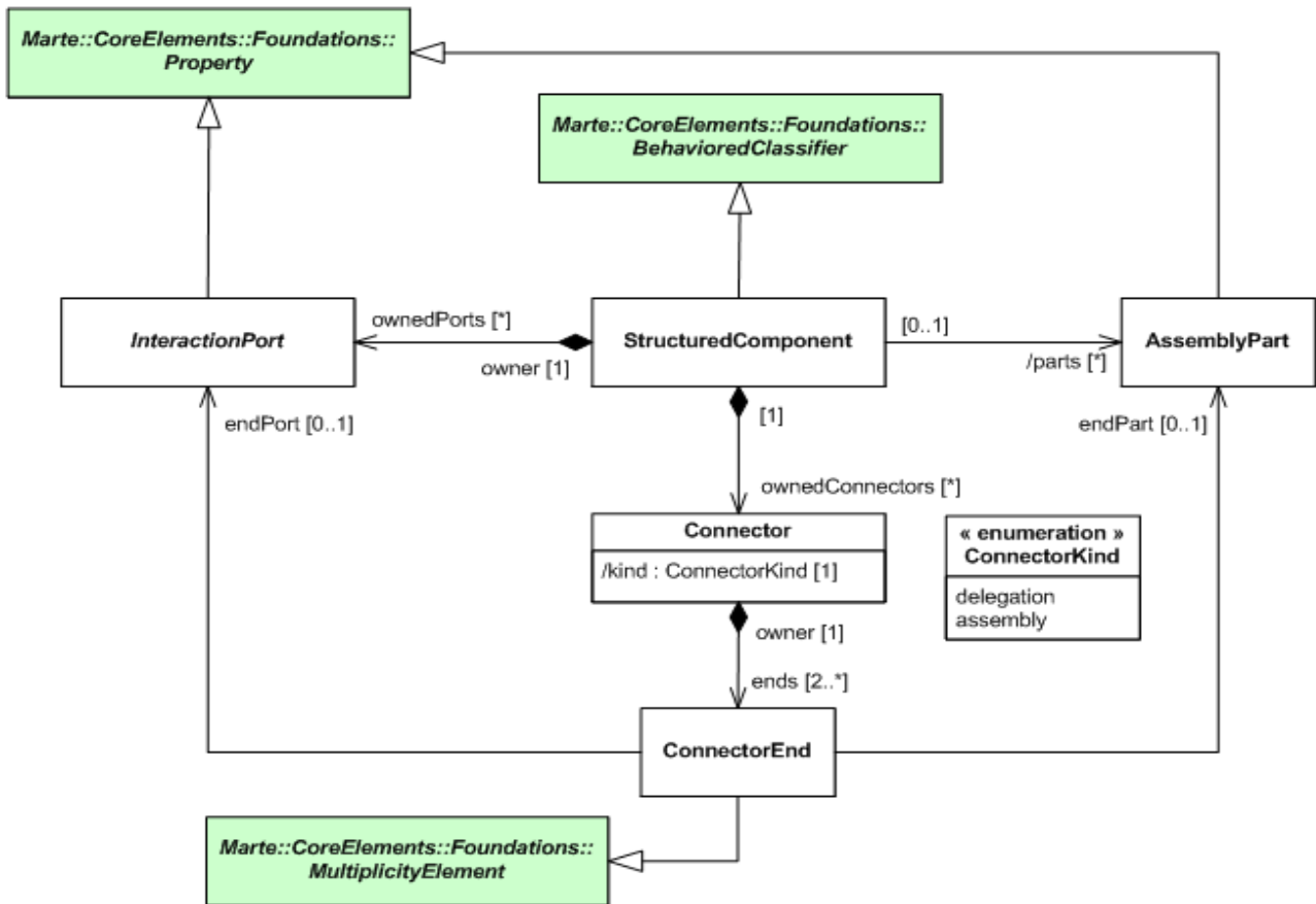
Figure 12.2 - The bulk of the MARTE GenericComponentModel package
