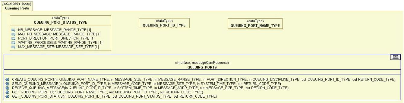
Figure D.27. ARINC-653 Queuing Ports package
