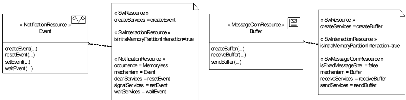
Figure 14.51 - ARINC-653 Event and Buffer example
