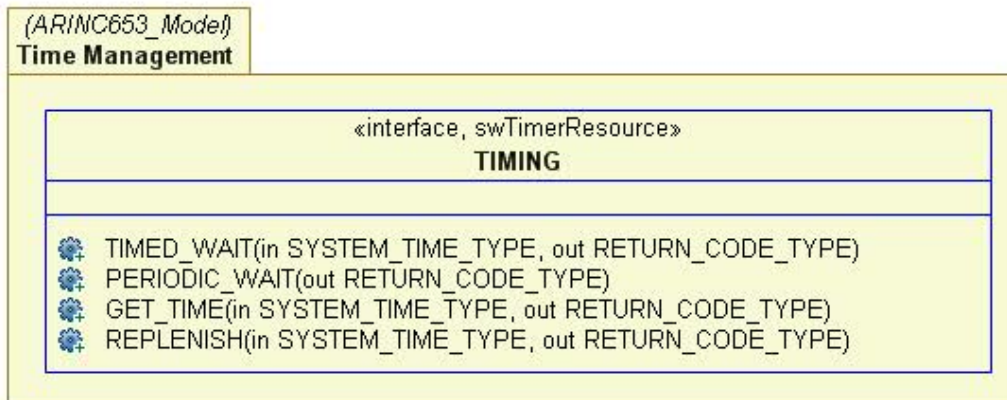
Figure D.23. ARINC-653 Time Management package
