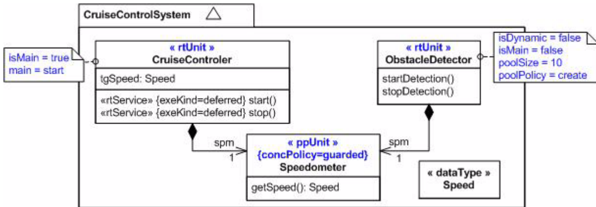
Figure 13.13 - A very simple cruise control model
