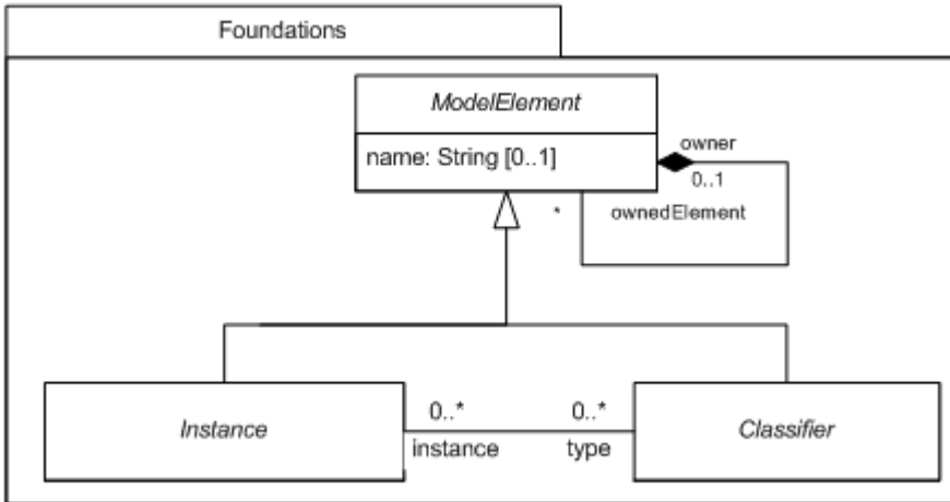
Figure 7.3 - Instance and Classifier root diagram of the Foundations package
