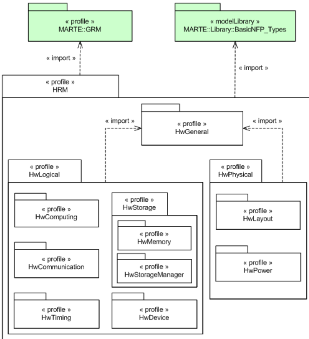
Figure 14.64 - Hardware Resource Model profile structure
