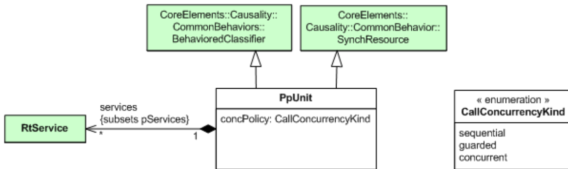
Figure 13.3 - PpUnit of the HLAM package
