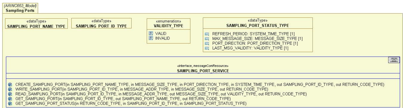
Figure D.26. ARINC-653 Sampling Ports package
