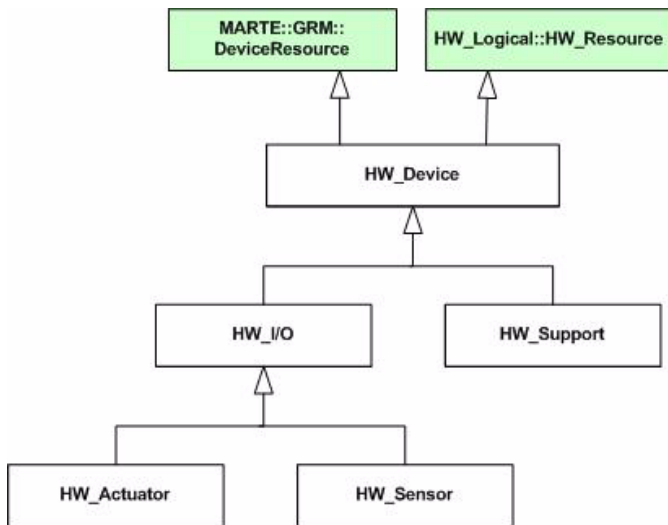
Figure 14.60 - HW_Device package details
