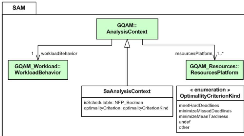
Figure 16.2 - The SAM root domain model: Analysis context
