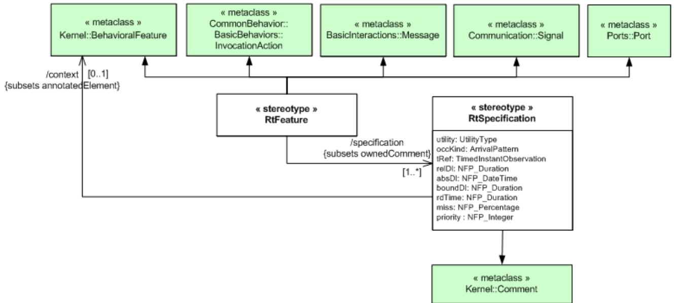
Figure 13.9 - RtFeature stereotype of the MARTE::HLAM sub-profile
