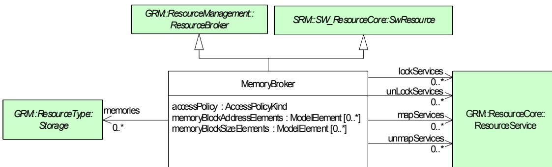
Figure 14.19 - The MemoryBroker overview
