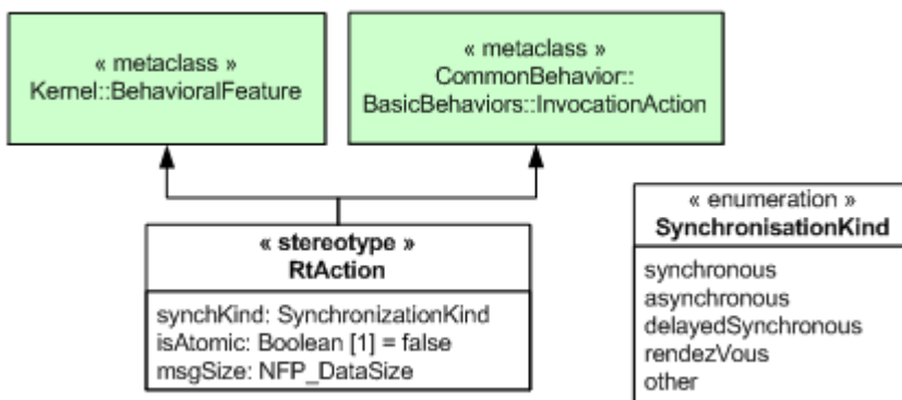
Figure 13.10 - RtAction of the MARTE::HLAM sub-profile
