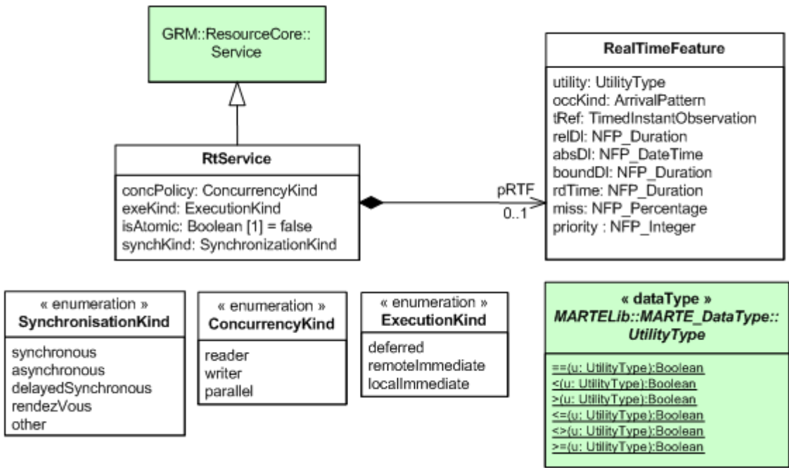
Figure 13.5 - RtService of the HLAM package
