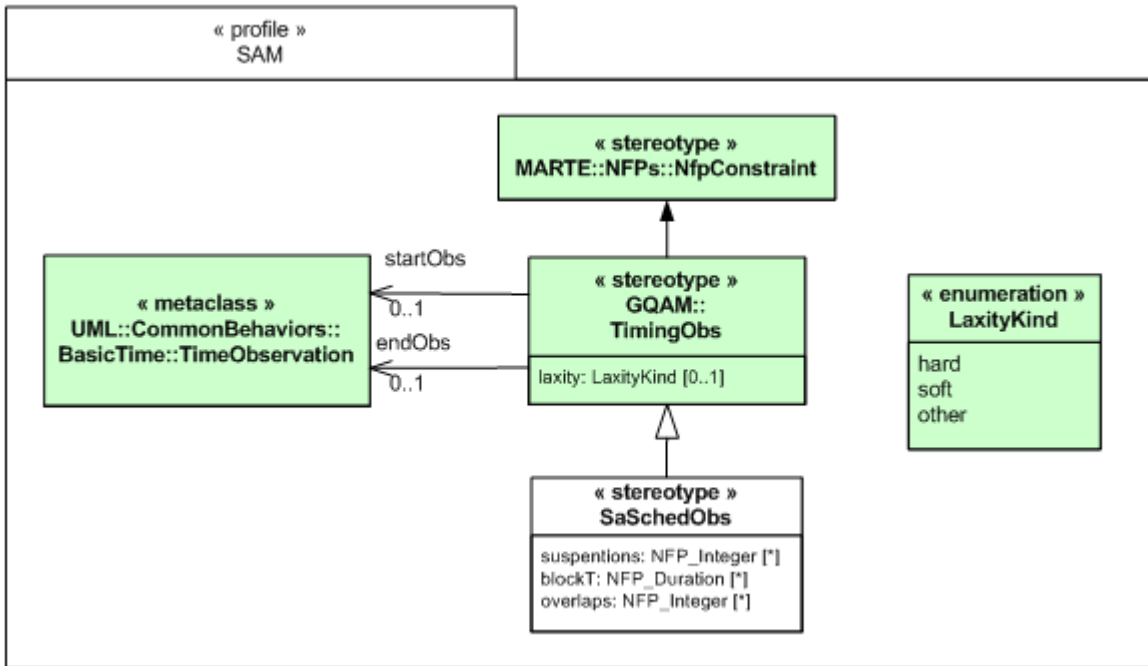
Figure 16.8 - The SAM Profile: Timed Observers
