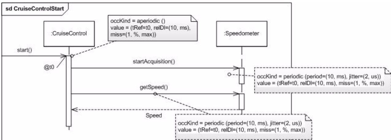
Figure 13.16 - Examples of real-time feature within sequence diagrams
