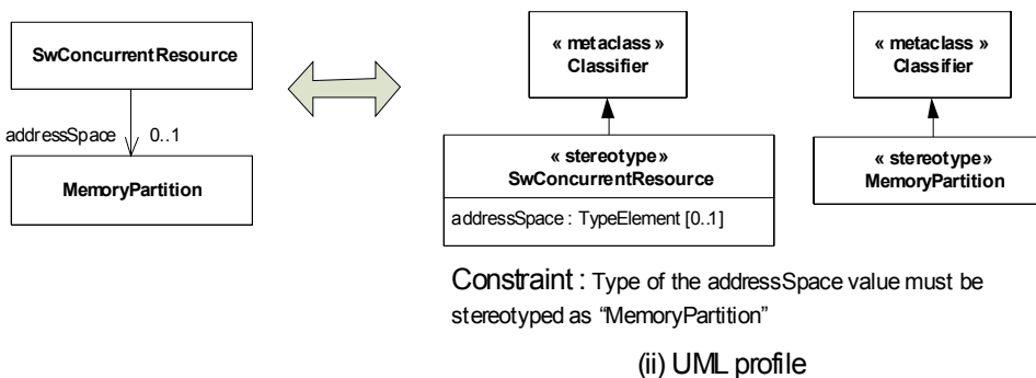
Figure 14.22 - SRM Matched rule on Associations
