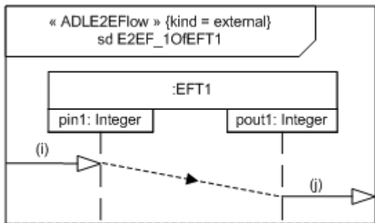
Figure A.20. Example of an EAST-ADL2 external end-to-end flow for an elementary ADLFunctionType
