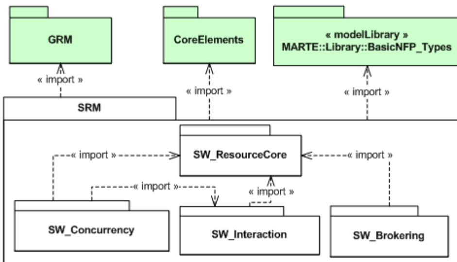
Figure 14.1 - Structure of the SRM modeling framework
