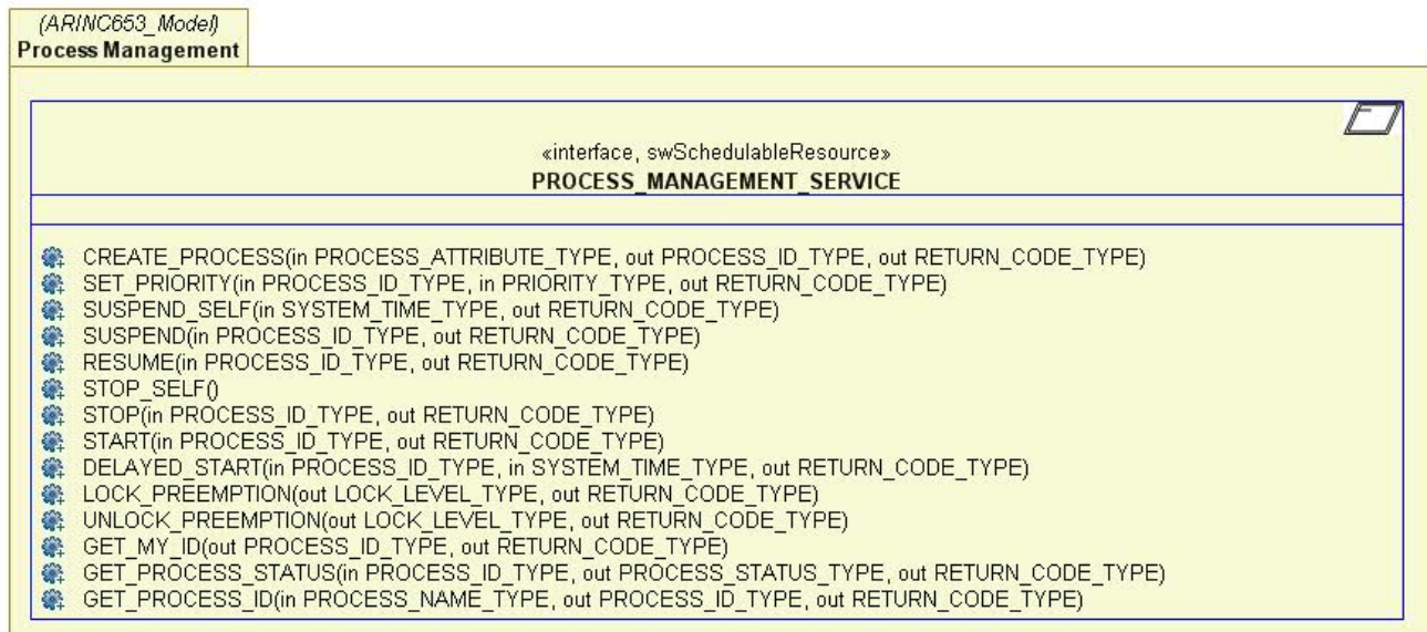
Figure D.24. ARINC-653 PROCESS package
