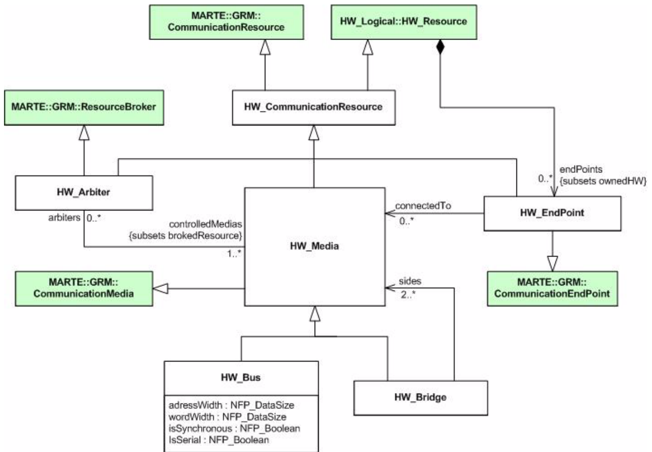
Figure 14.58 - HW_Communication package details
