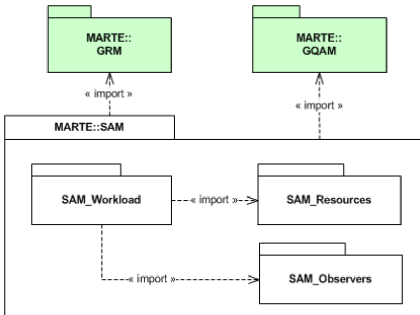
Figure 16.1 - Structure of the SAM domain model
