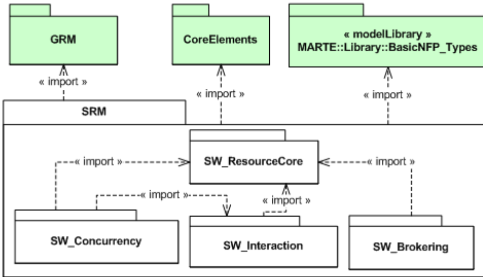
Figure 14.23 - The SRM profile overview
