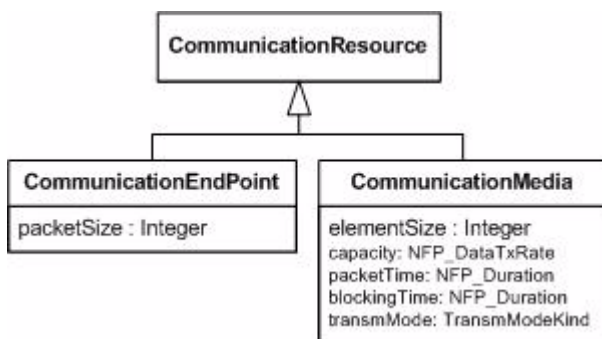
Figure 10.8 - Kinds of Communication resource in the ResourceTypeResourceTypes package
