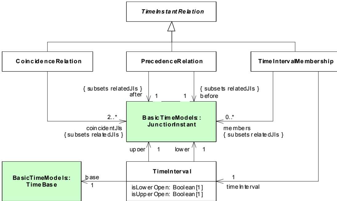
Figure 9.5 - TimeInstantRelation diagram of the time model
