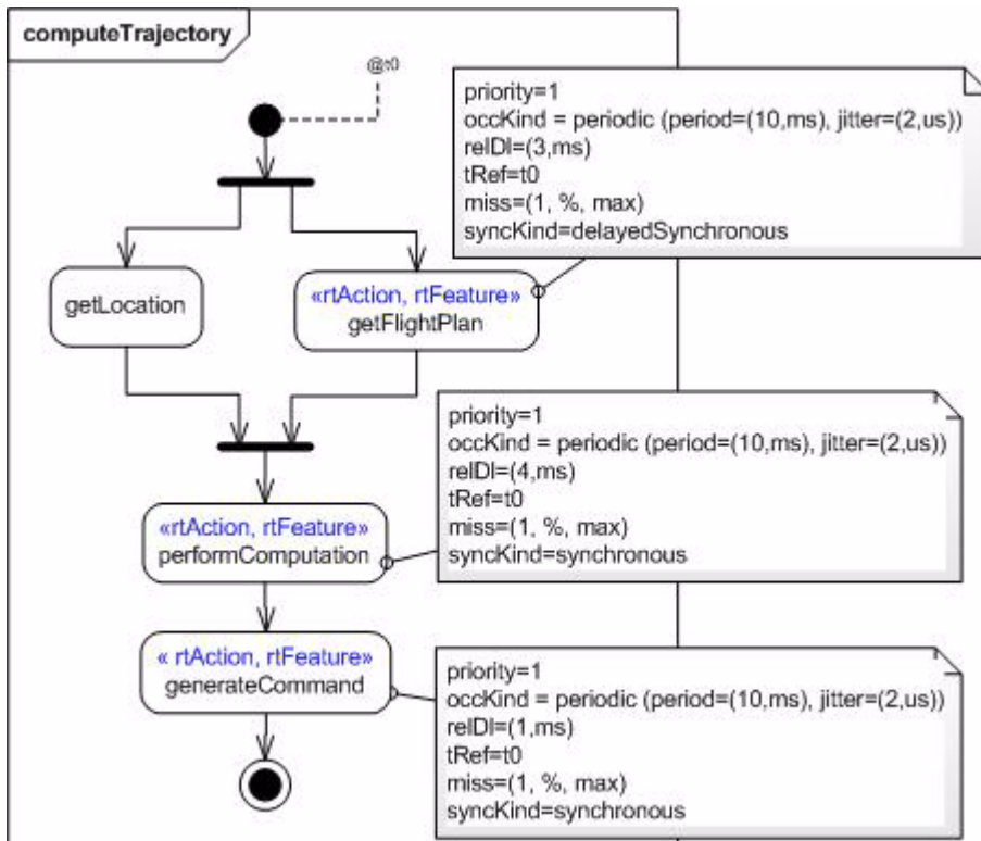
Figure 13.18 - Main behavior of the Trajectory component
