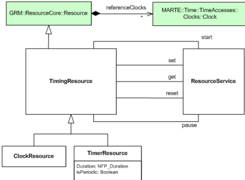
Figure 10.7 - Timing resources
