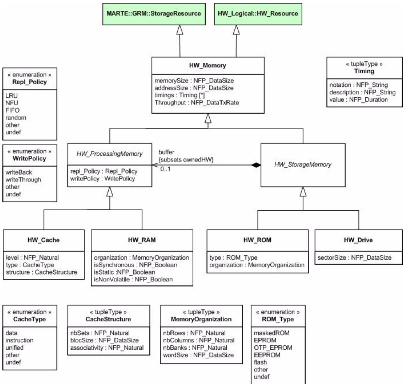
Figure 14.56 - HW_Storage package details (HW_Memory)
