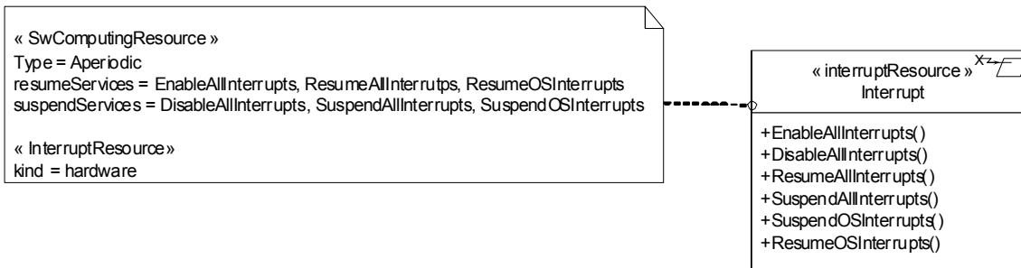
Figure 14.48 - OSEK/VDX Interrupt example
