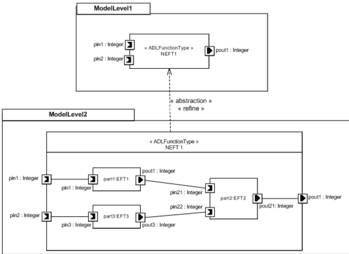
Figure A.31. Example of non-elementary function refinement
