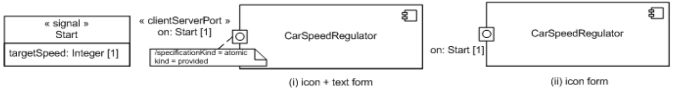
Figure 12.11 - Example of atomic client-server port
