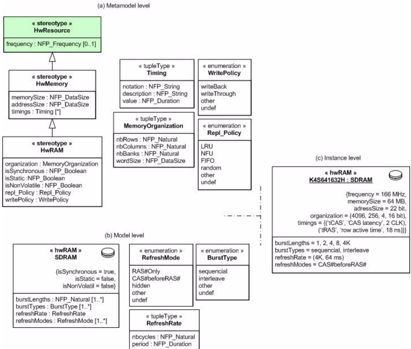
Figure 14.76 - Stereotype application example (SDRAM)
