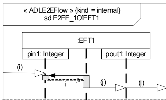
Figure A.23. Example of an EAST- ADL2 internal end-to-end flow for an elementary ADLFunctionType owning a non-triggered input port
