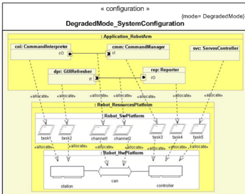
Figure 7.11 - Modelling Modes and Configurations
