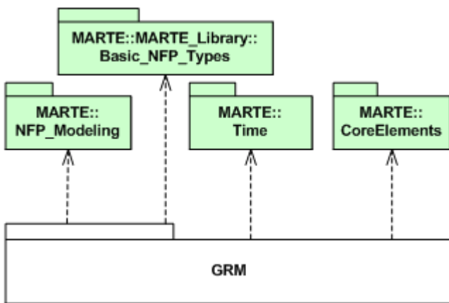
Figure 10.1 - Dependencies of the GeneralResourceModel (GRM) package
