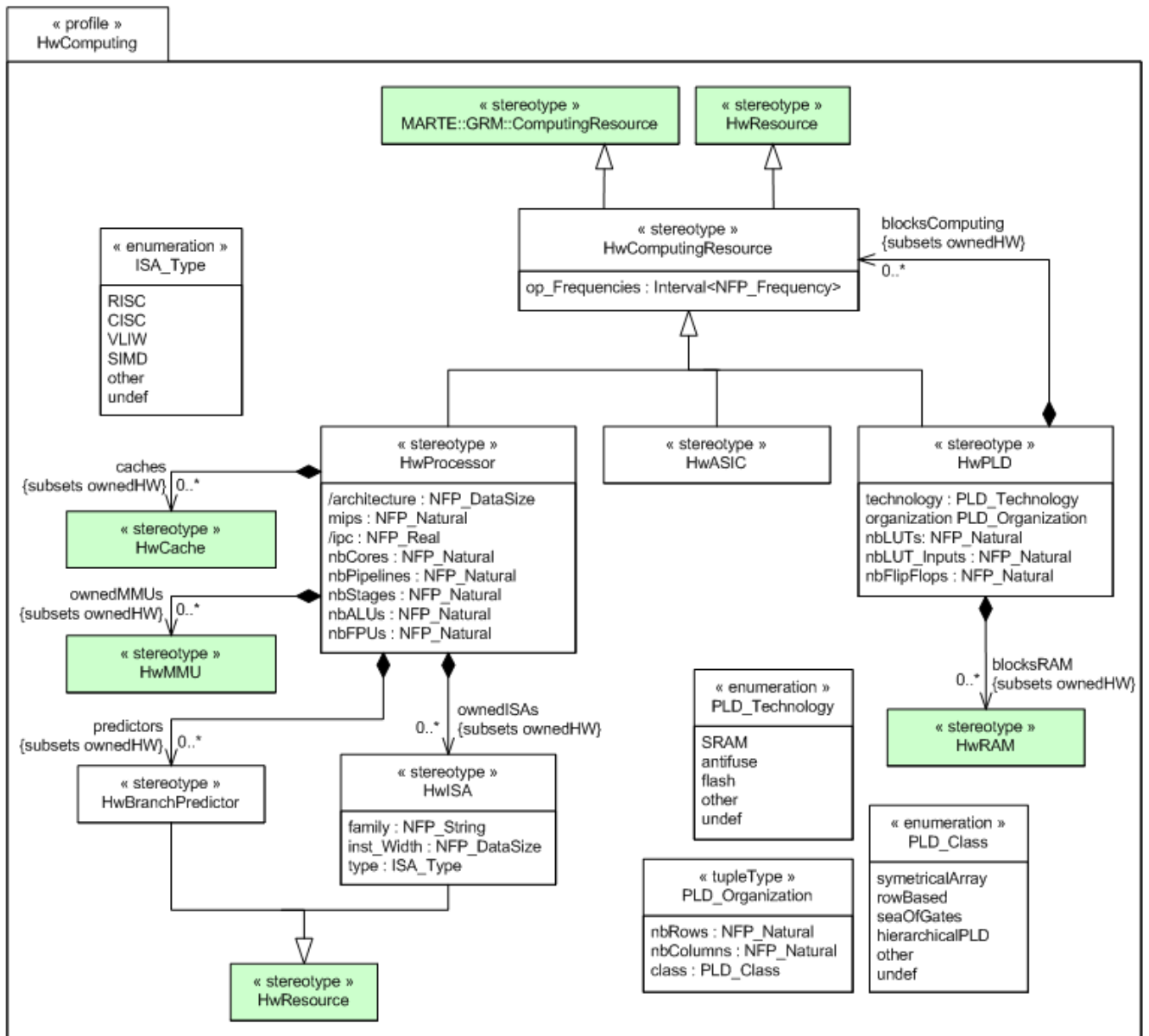
Figure 14.66 - HwComputing package details
