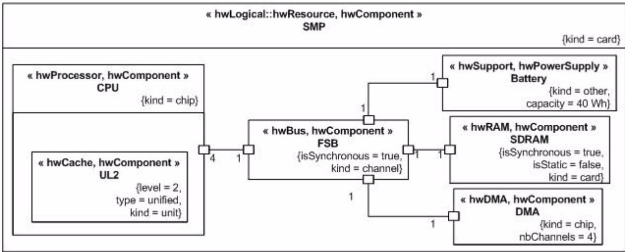
Figure 14.80 - SMP merged (logical/physical) view
