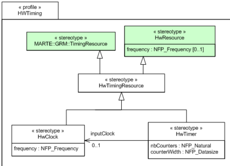
Figure 14.70 - HwTiming profile details
