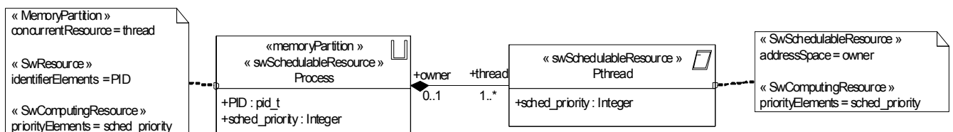
Figure 14.47 - POSIX Process and Pthread example
