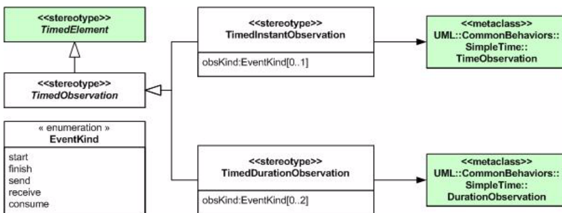
Figure 9.29 - UML extensions for Time modeling (4)
