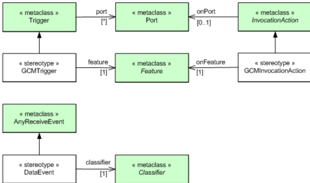
Figure 12.9 - UML2 profile of the MARTE GeneralComponentModel, event and communication
