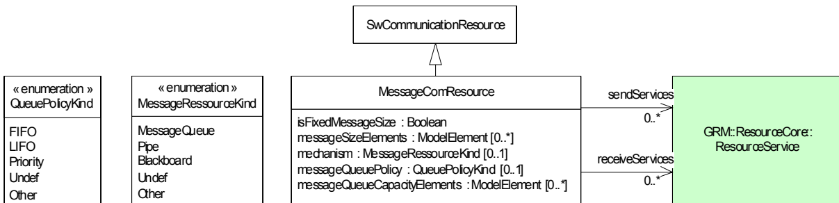
Figure 14.15 - The Messaging Communication resource
