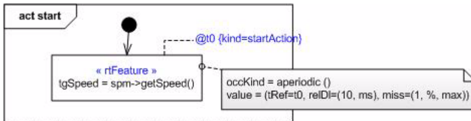
Figure 13.14 - An example of call action with a deadline real-time feature
