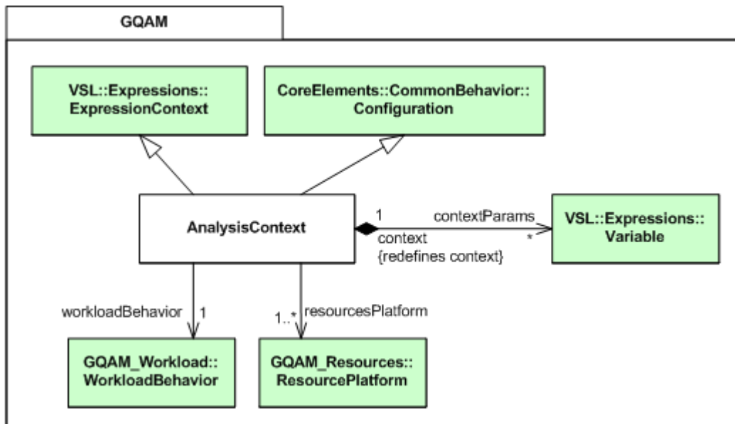
Figure 15.2 - Top package of the GQAM domain model
