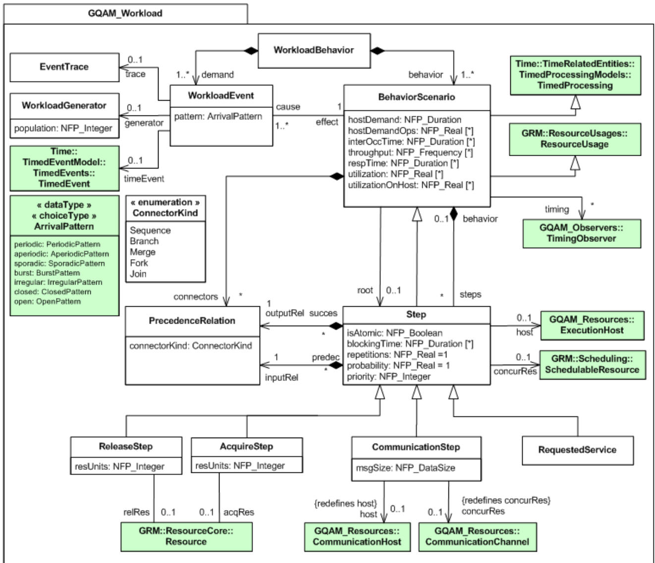
Figure 15.3 - GQAM_Workload package of the GQAM domain model
