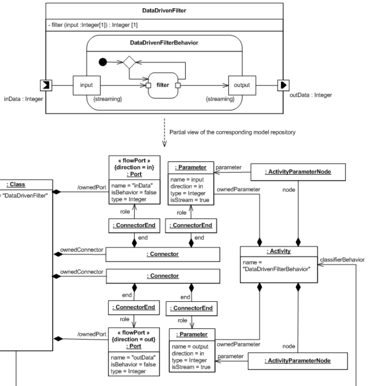
Figure 12.25 - Example 5, on the "push" form of the flow port semantics
