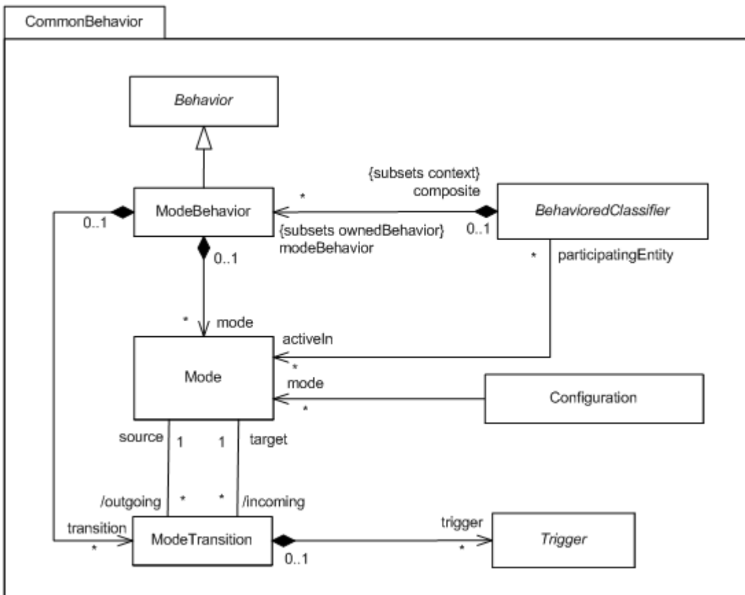
Figure 7.6. Domain model of Modal Behavior
