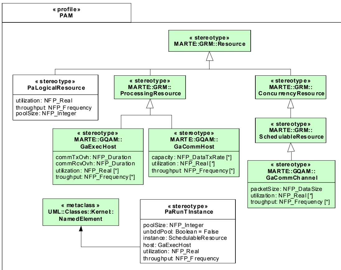
Figure 17.8 - Profile diagram of performance extensions for resources
