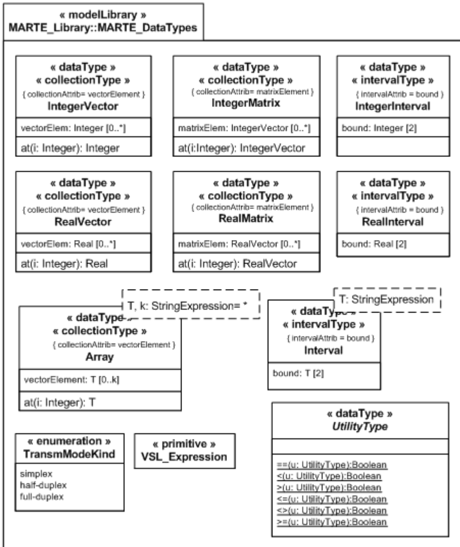
Figure D.4 - MARTE library of general data-types
