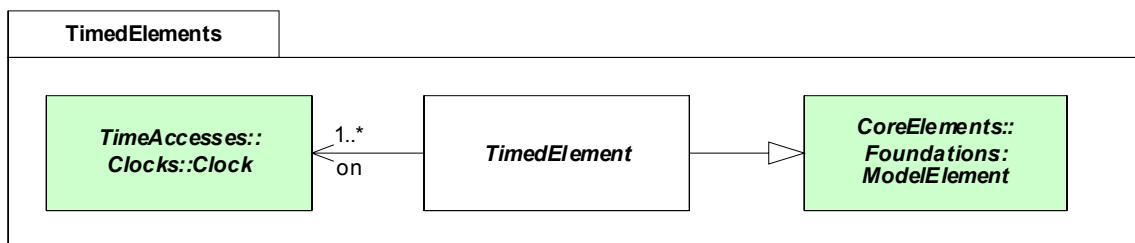
Figure 9.15 - TimedElement diagram of the time model
