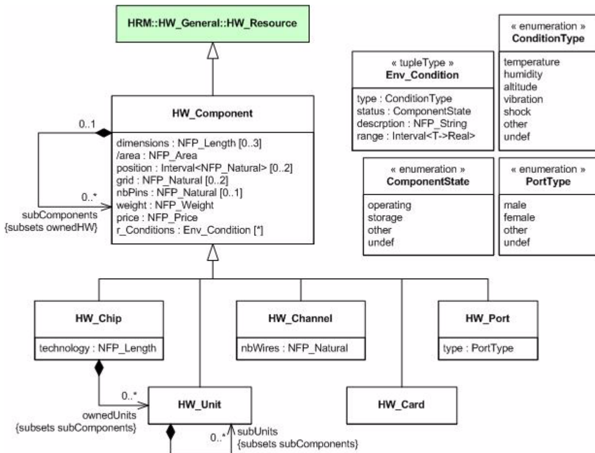
Figure 14.62 - HW_Layout package details
