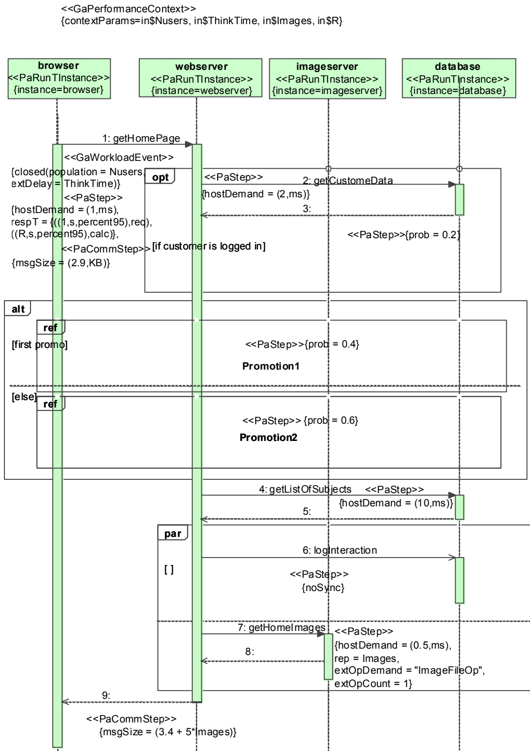
Figure 17.15 - Example 2: the home page scenario of the TPC-W standard benchmark, with some additions to
