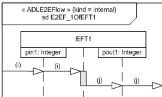
Figure A.21. Example 1 of an EAST-ADL2 internal end-to-end flow for an elementary ADLFunctionType
