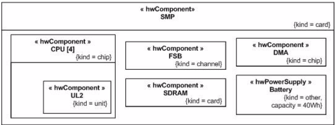
Figure 14.79 - SMP physical view
