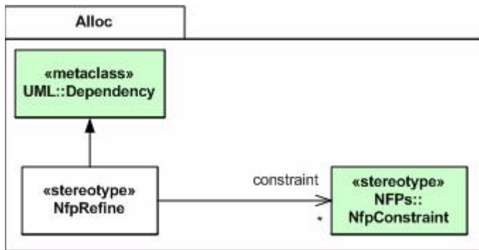
Figure 11.7 - The stereotype NfpRefine
