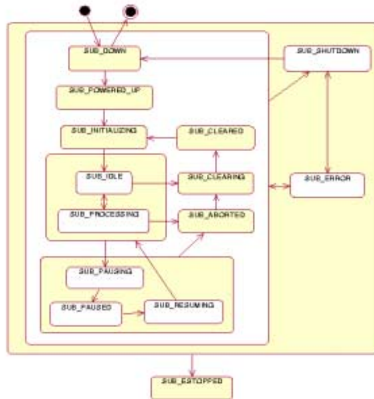
Figure 2-3 Sub-Unit State Model
