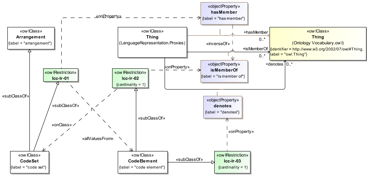
Figure 8.5 - Definition of Code Set and Code Element
