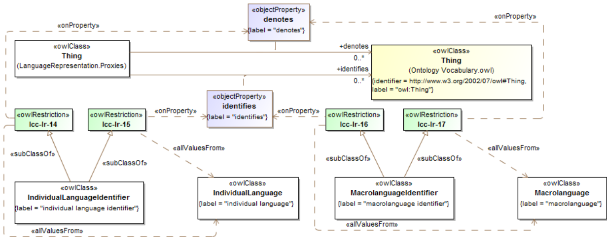
Figure 8.9 Definition of Individual and Macrolanguage Identifiers
