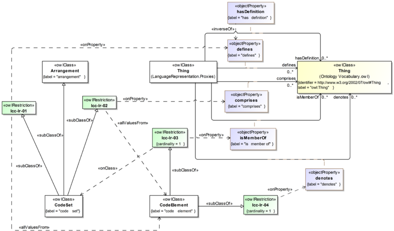
Figure 8.5 Definition of Code Set and Code Element
