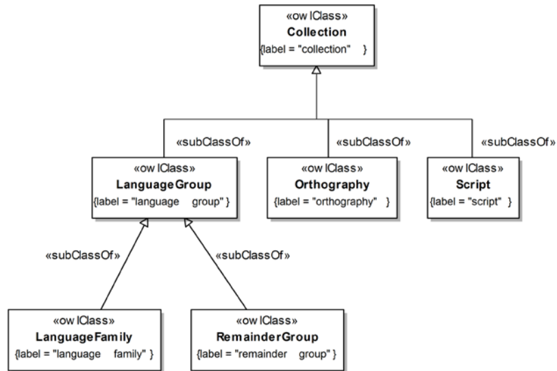
Figure 8.2 Collection Class Hierarchy
