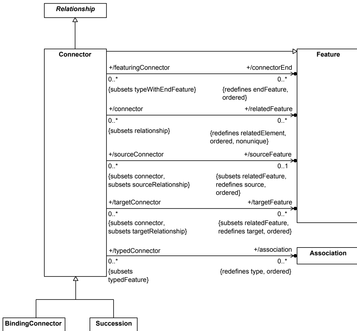
Figure 26. Connectors
