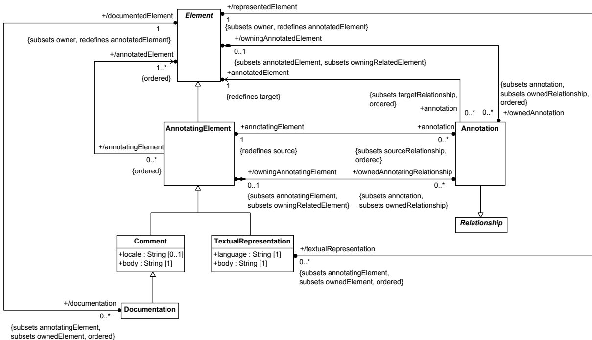
Figure 6. Annotation
