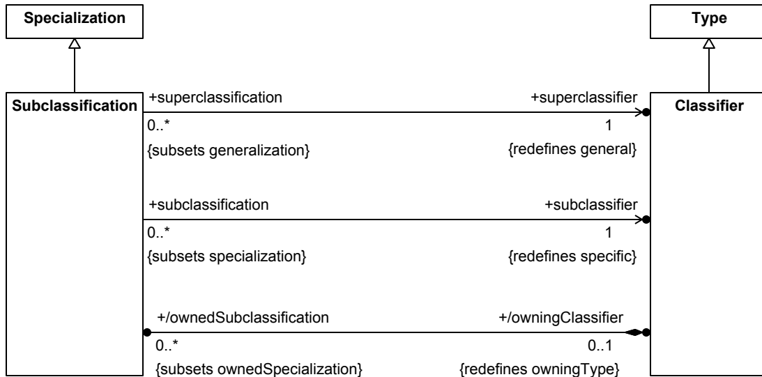
Figure 16. Classifiers
