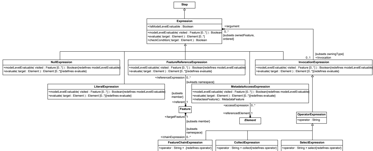
Figure 33. Expressions
