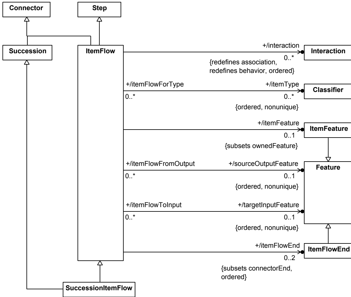
Figure 36. Item Flows
