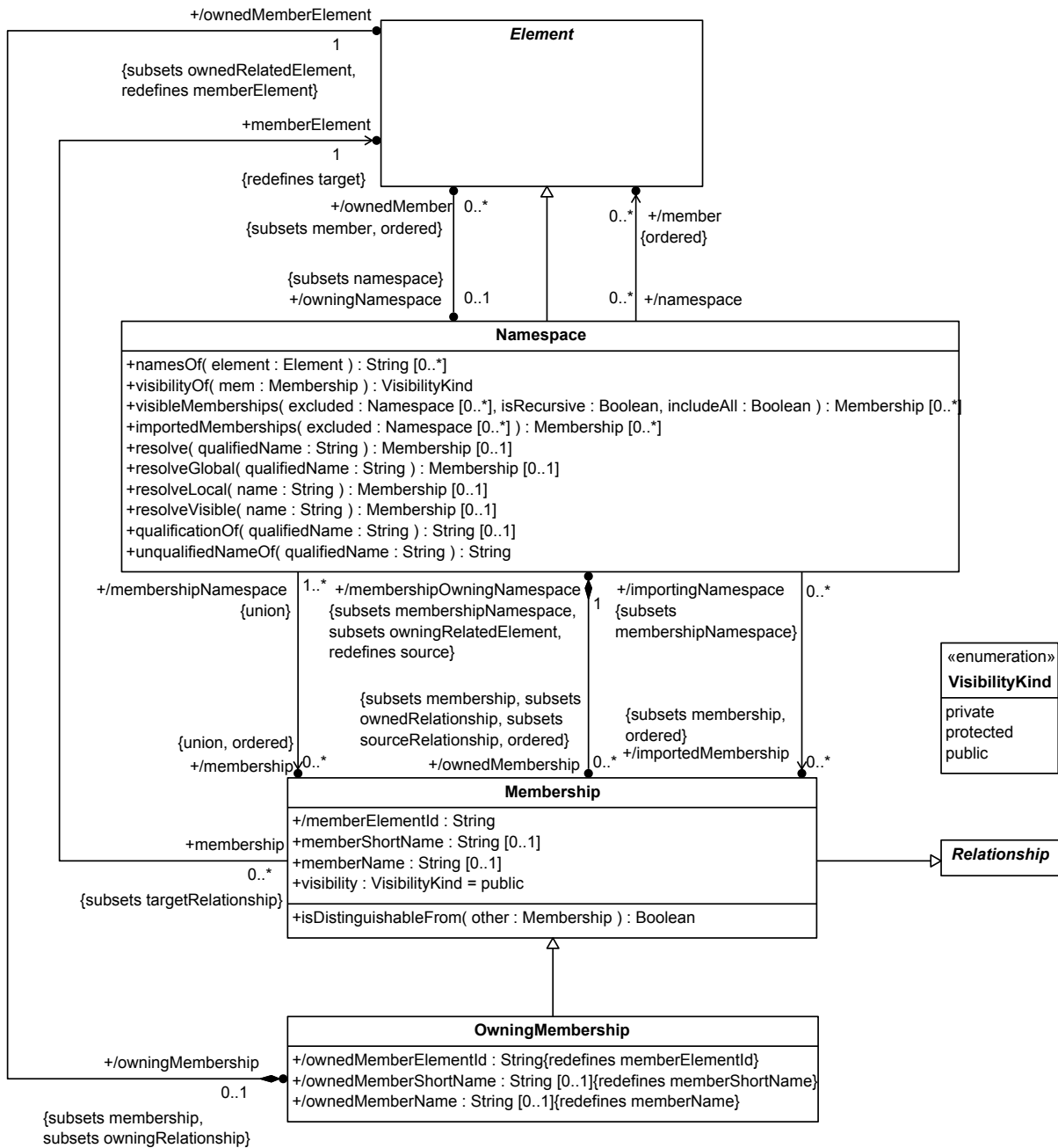
Figure 7. Namespaces
