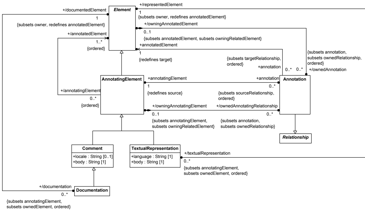
Figure 6. Annotation
