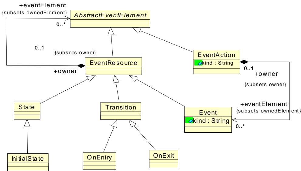
Figure 17.3 - EventResourcesClass Diagram
