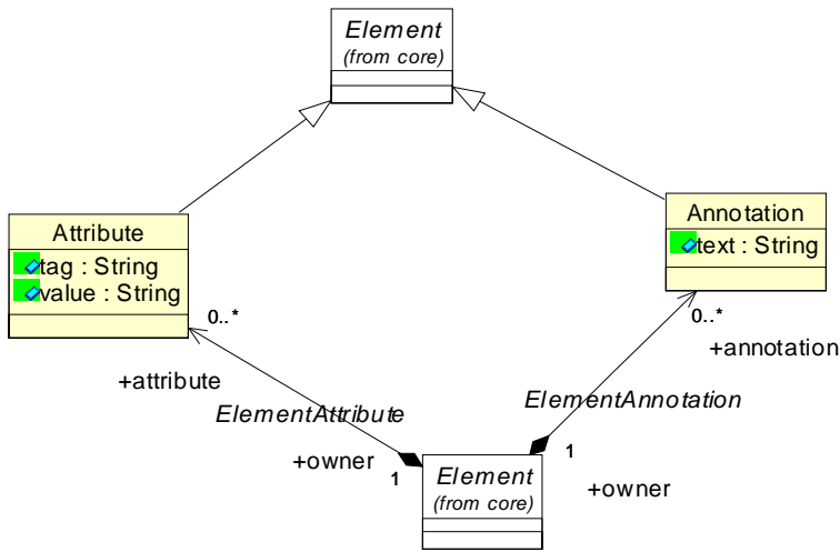
Figure 10.5 - Annotations Class Diagram
