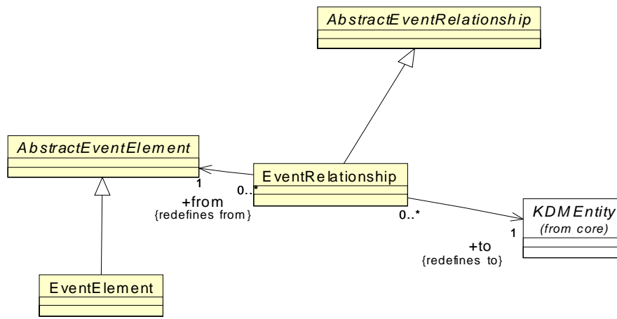
Figure 17.6 - ExtendedEventElements Class Diagram
