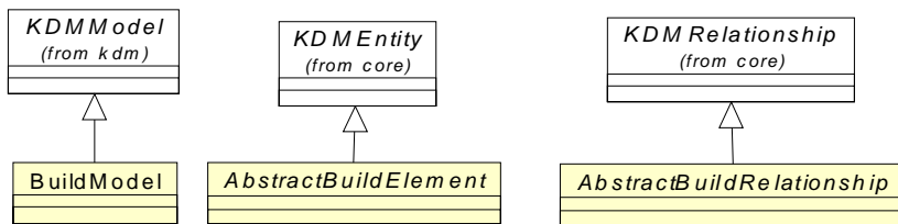
Figure 21.2 - BuildInheritances Class Diagram
