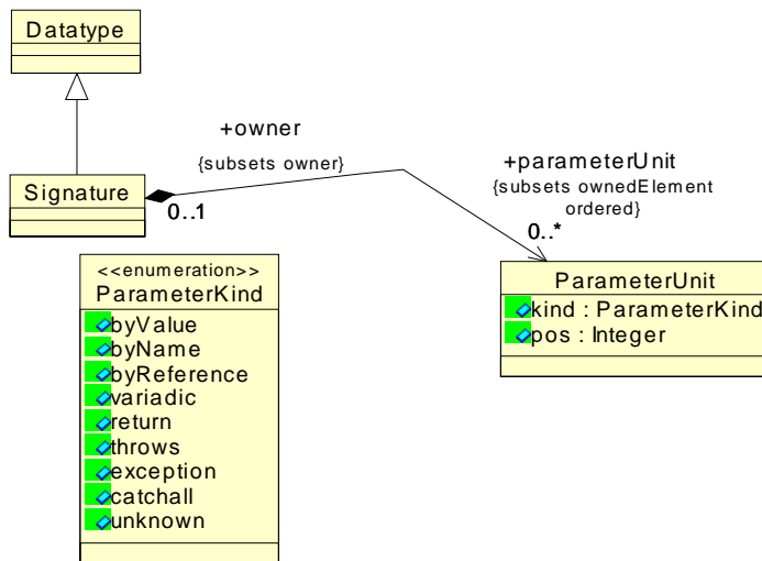
Figure 12.11 - Signature Class Diagram
