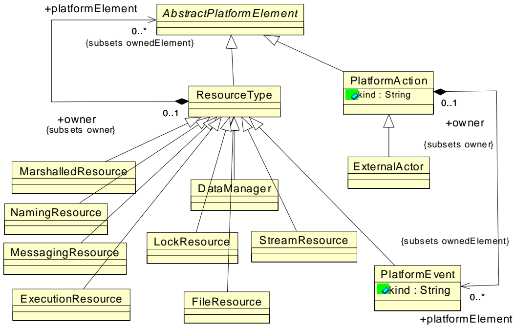
Figure 15.3 - PlatformResources Class Diagram
