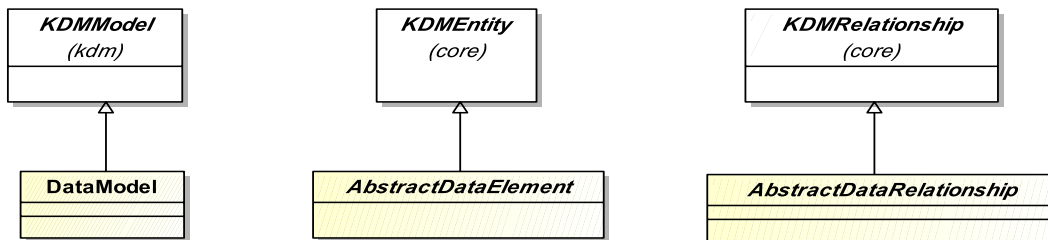
Figure 18.2 - DataInheritances Diagram
