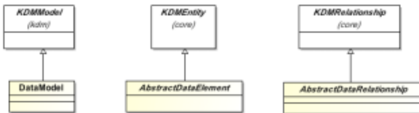
Figure 18.2 - DataInheritances Diagram
