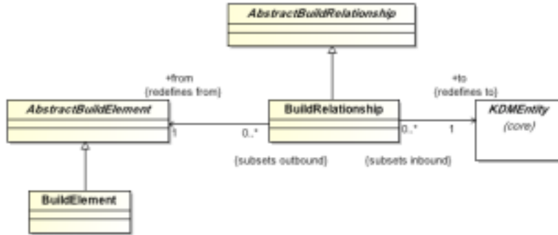
Figure 21.5 - ExtendedBuildElements Class Diagram
