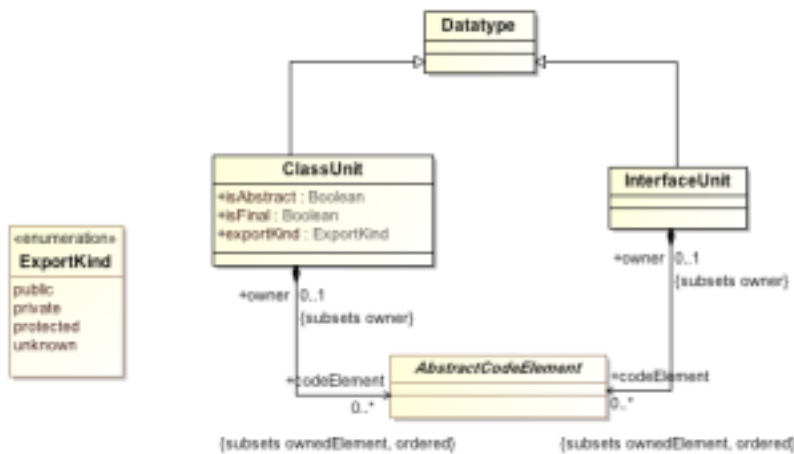
Figure 12.14 - ClassTypes Class Diagram
