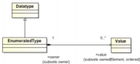
Figure 12.9 - EnumeratedTypes Class Diagram
