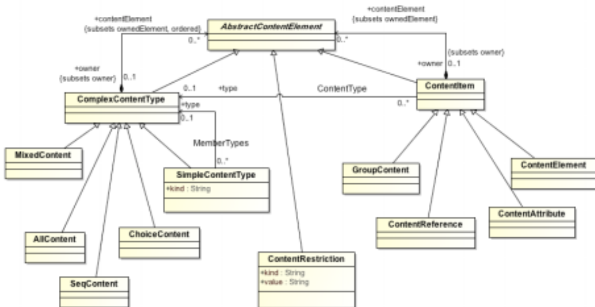
Figure 18.9 - ContentElements Class Diagram
