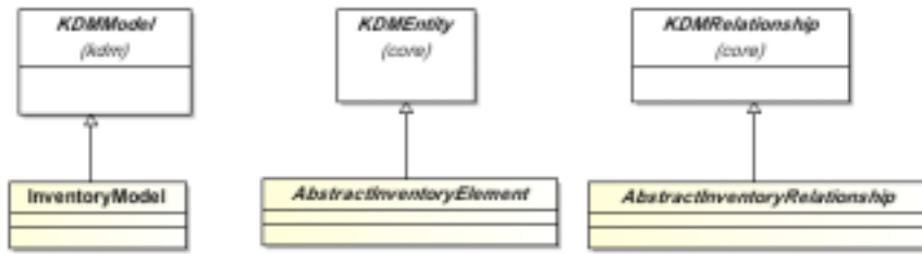
Figure 11.2 - InventoryInheritances Class Diagram
