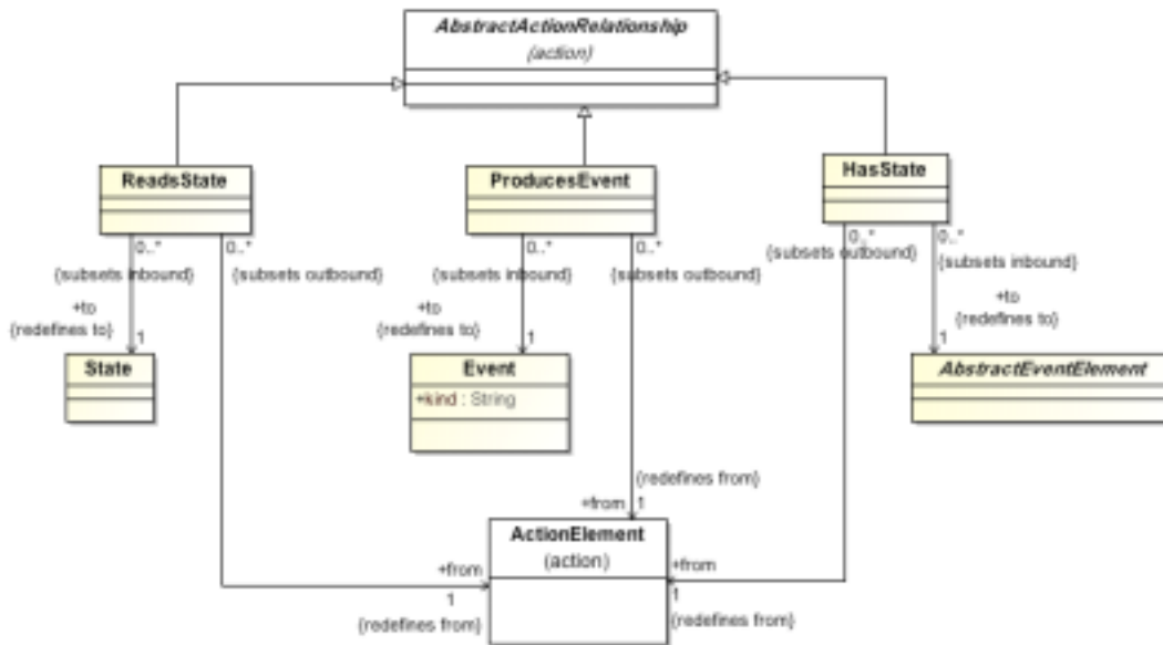
Figure 17.5 - EventActions Class Diagram
