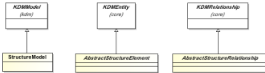
Figure 19.2 - StructureInheritances Class Diagram
