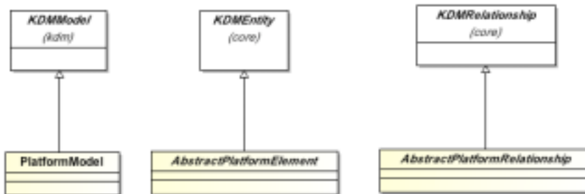
Figure 15.1 - PlatformInheritances Class Diagram
