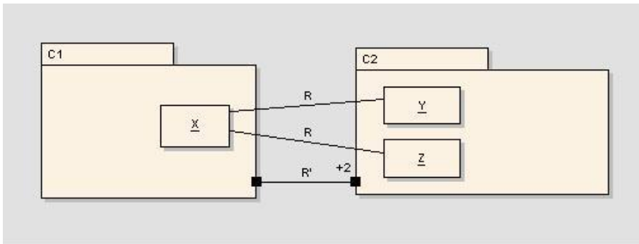
Figure 9.5 - AggregatedRelationships illustrated
