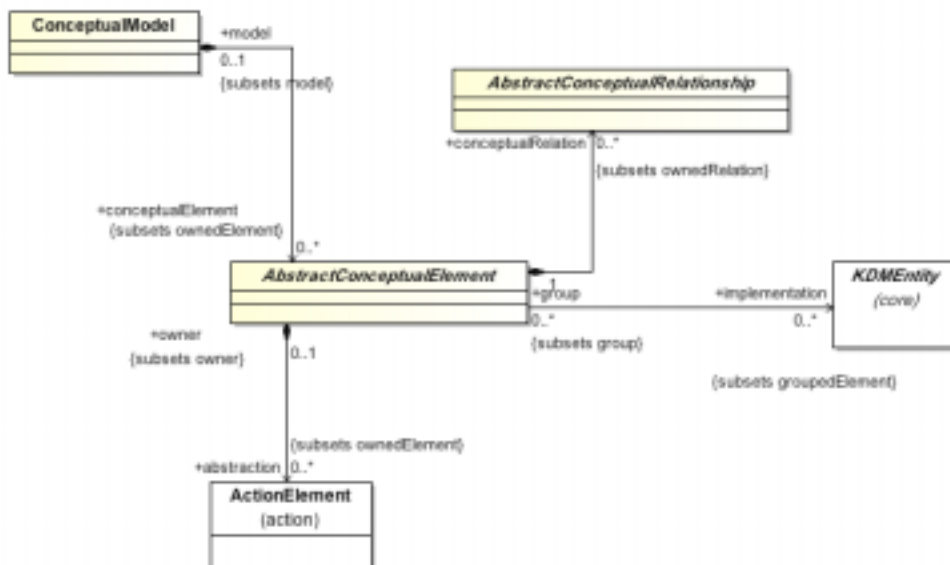
Figure 20.4 - ConceptualModel Class Diagram
