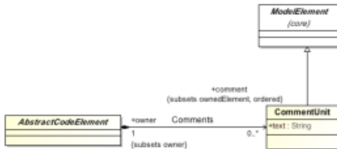
Figure 12.22 - Comments Class Diagram
