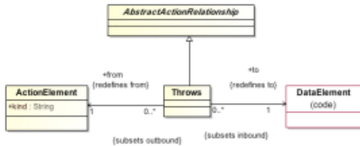
Figure 13.8 - ExceptionRelations Class Diagram
