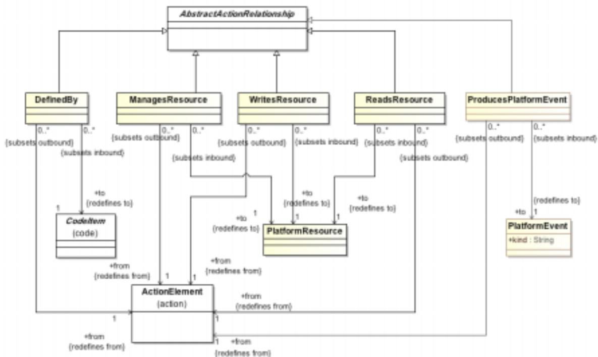
Figure 15.5 - PlatformActions Class Diagram
