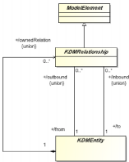
Figure 9.3 - CoreRelations Class Diagram
