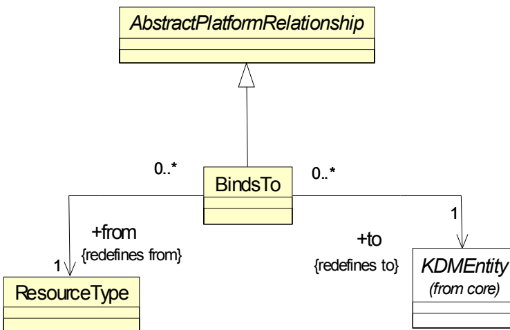
Figure 15.3 - PlatformRelations Class Diagram
