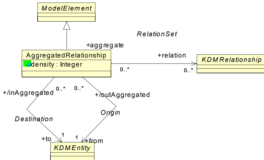
Figure 9.3 - AggregatedRelations Class Diagram
