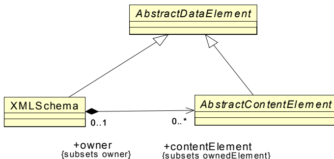
Figure 18.8 - StructuredData Class Diagram
