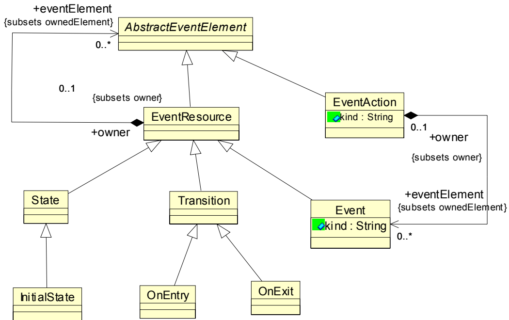
Figure 17.3 - EventResourcesClass Diagram
