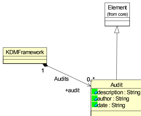
Figure 10.2 - Audit Class Diagram
