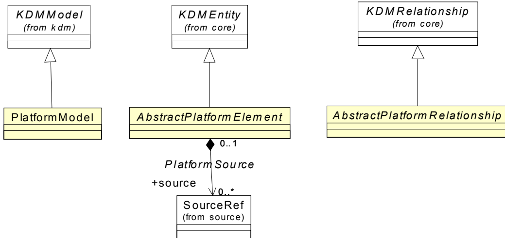
Figure 15.1 - PlatformInheritances Class Diagram
