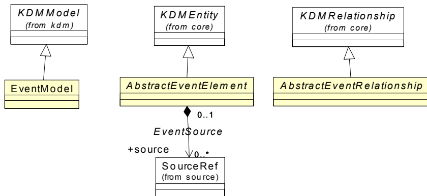
Figure 17.2 - EventInheritances Class Diagram
