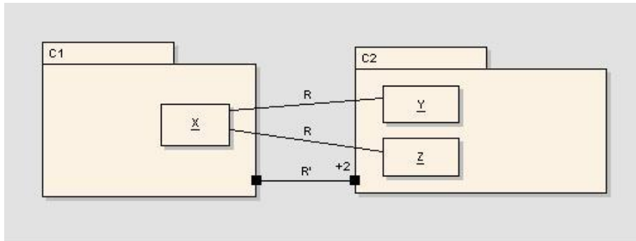
Figure 9.4 - AggregatedRelationships illustrated
