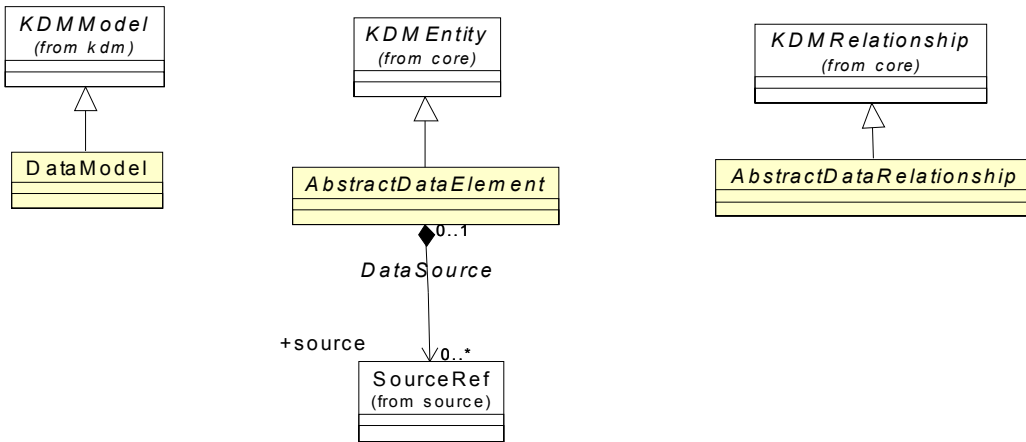
Figure 18.2 - DataInheritance Diagram
