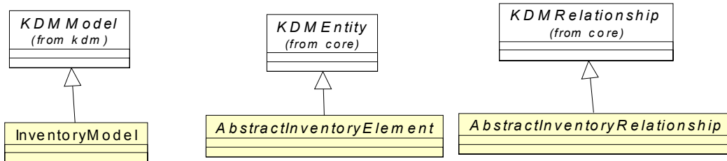
Figure 11.2 - InventoryInheritances Class Diagram
