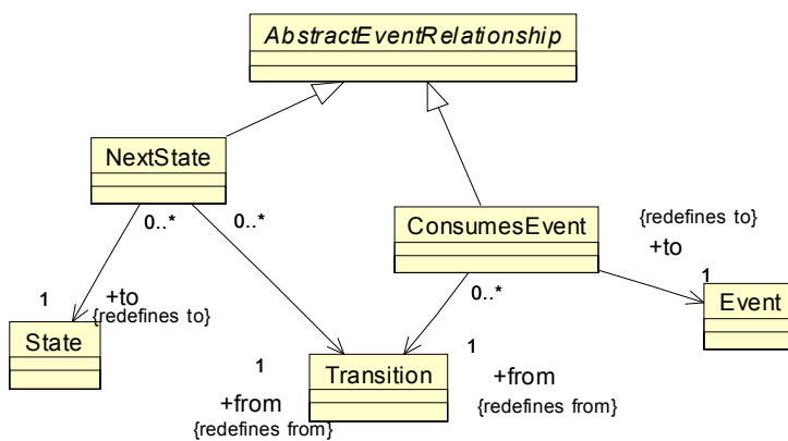
Figure 17.4 - EventRelations Class Diagram
