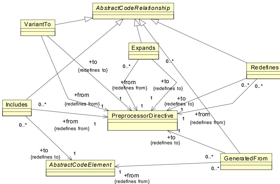
Figure 12.20 - PreprocessorRelations Class Diagram
