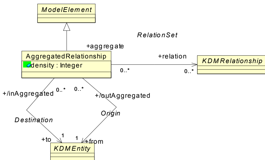
Figure 9.3 - AggregatedRelations Class Diagram
