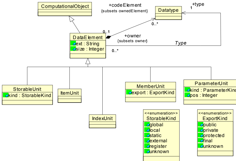
Figure 12.5 - DataElement Class Diagram
