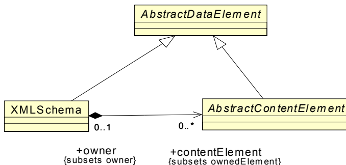
Figure 18.8 - StructuredData Class Diagram
