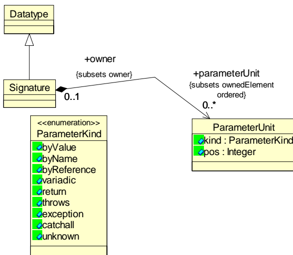
Figure 12.11 - Signature Class Diagram
