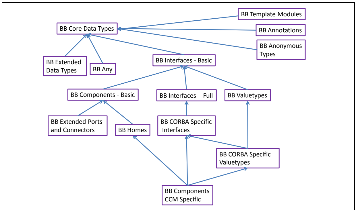
Figure 7-2: Relationships between Building-Blocks
