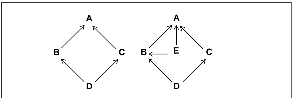
Figure 7-1: Examples of Legal Multiple Inheritance
