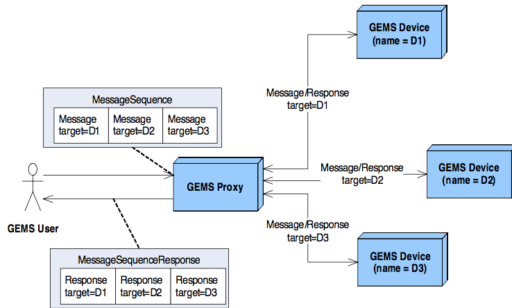
Figure 6.6 Message routing
