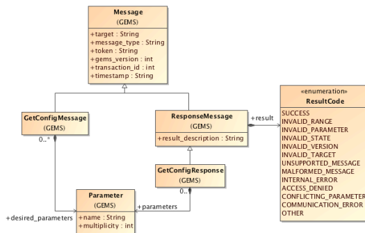
Figure 6.15 GetConfigMessage classes
