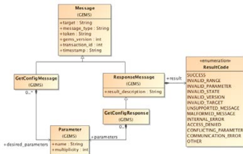
Figure 6.16 Save Config Message Classes
