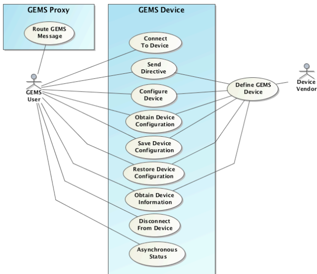
Figure 6.1 GEMS Use Cases
