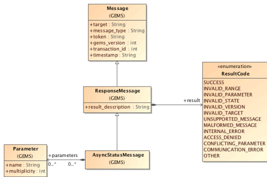
Figure 6.22 AsyncStatusMessage Class
