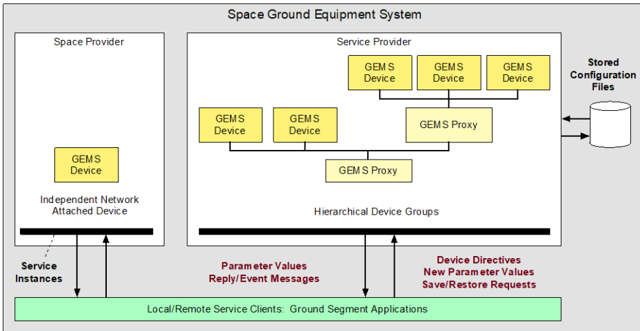
Figure 1.1 GEMS Overview
