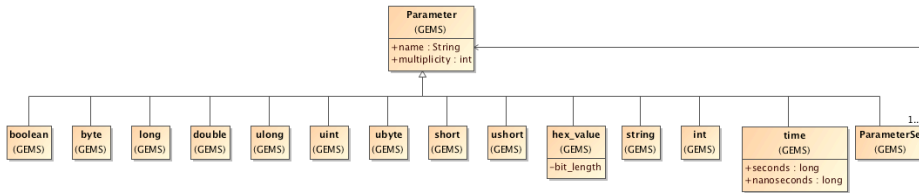
Figure 6.9 GEMS Standard Types
