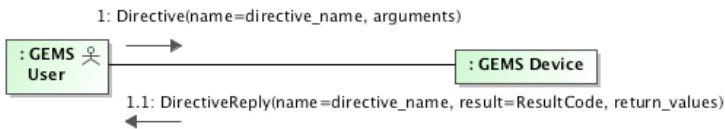
Figure 6.3 Sending a directive
