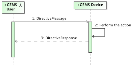
Figure 6.19 Directive Message Sequence
