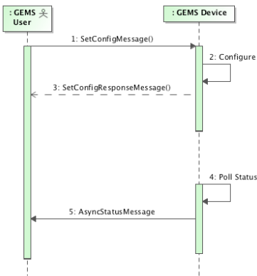
Figure 6.21 Asynchronous Status Message
