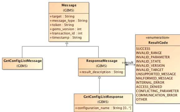
Figure 6.18 Get Config List Message Classes
