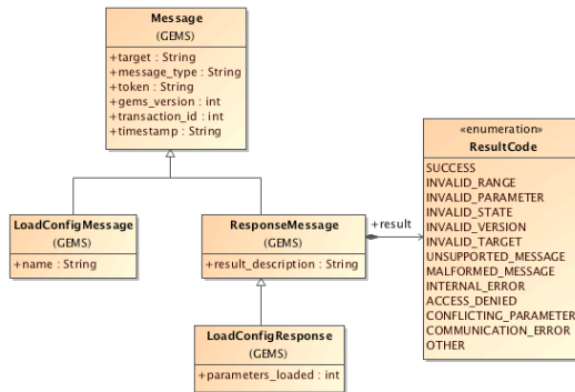
Figure 6.17 Load Config Message Classes
