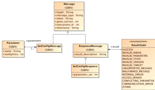
Figure 6.14 Set Configuration Message Classes
