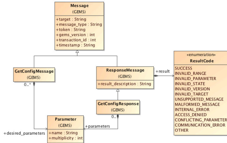
Figure 6.15 GetConfigMessage classes
