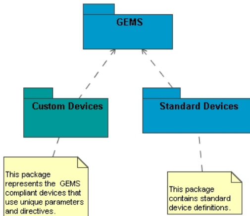
Figure 6.2 - GEMS Packages
