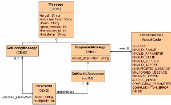
Figure 6.9 - GetConfigMessage UML
