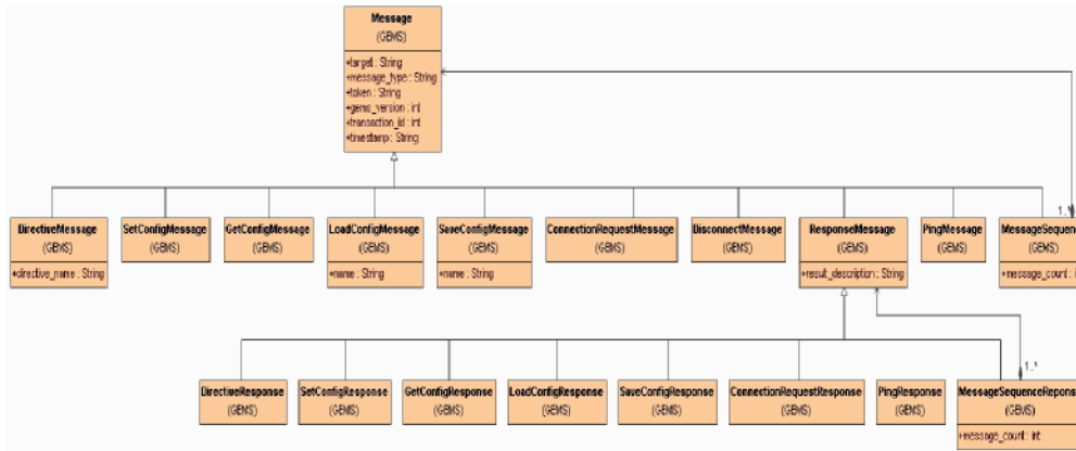
Figure 6.5 - GEMS Message Classes
