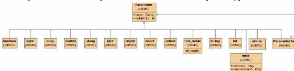
Figure 6.4 - GEMS Standard Types
