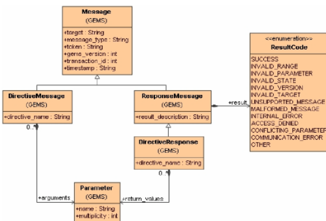
Figure 6.14 - Directive UML
