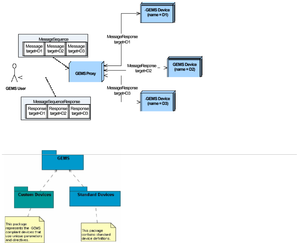
Figure 6.2 - GEMS Packages
