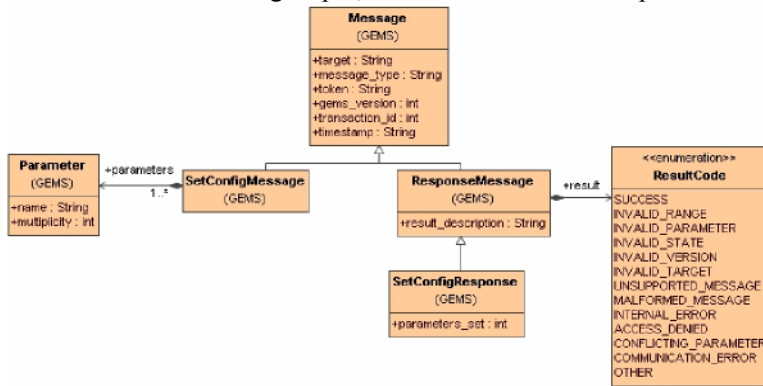
Figure 6.8 - Set Configuration Message Classes
