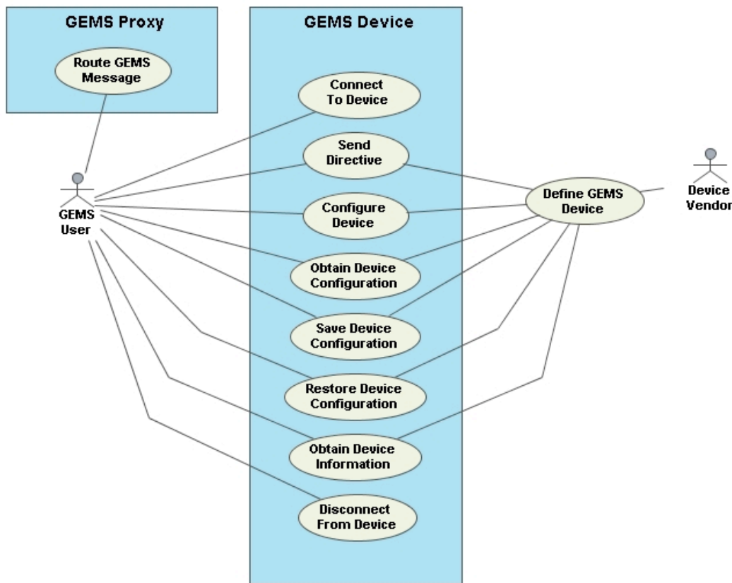
Figure 6.1 - GEMS Use Cases
