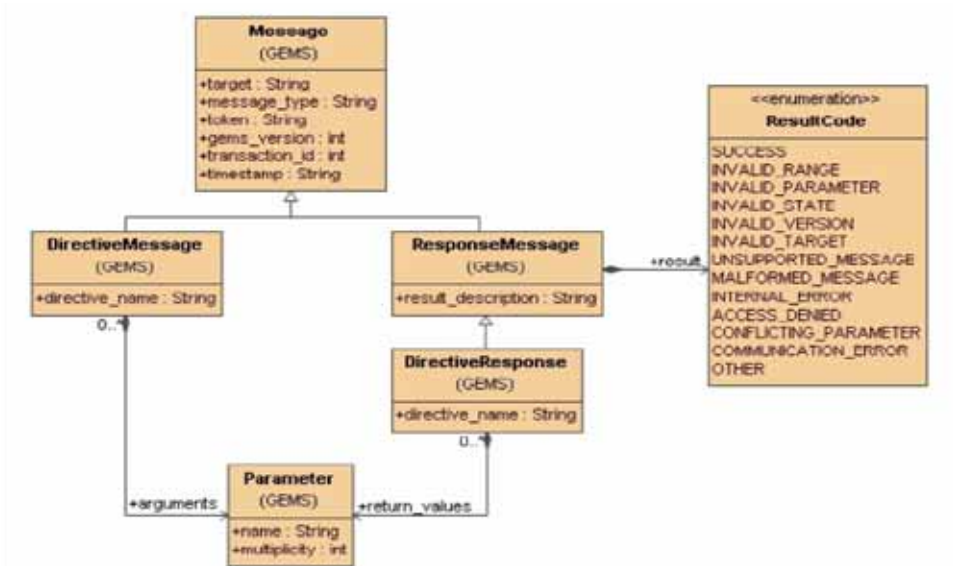
Figure 6.14 - Directive UML
