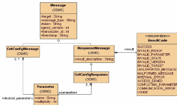
Figure 6.9 - GetConfigMessage UML
