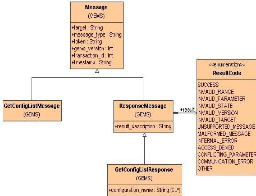
Figure 6.12 - Get Configuration List UML
