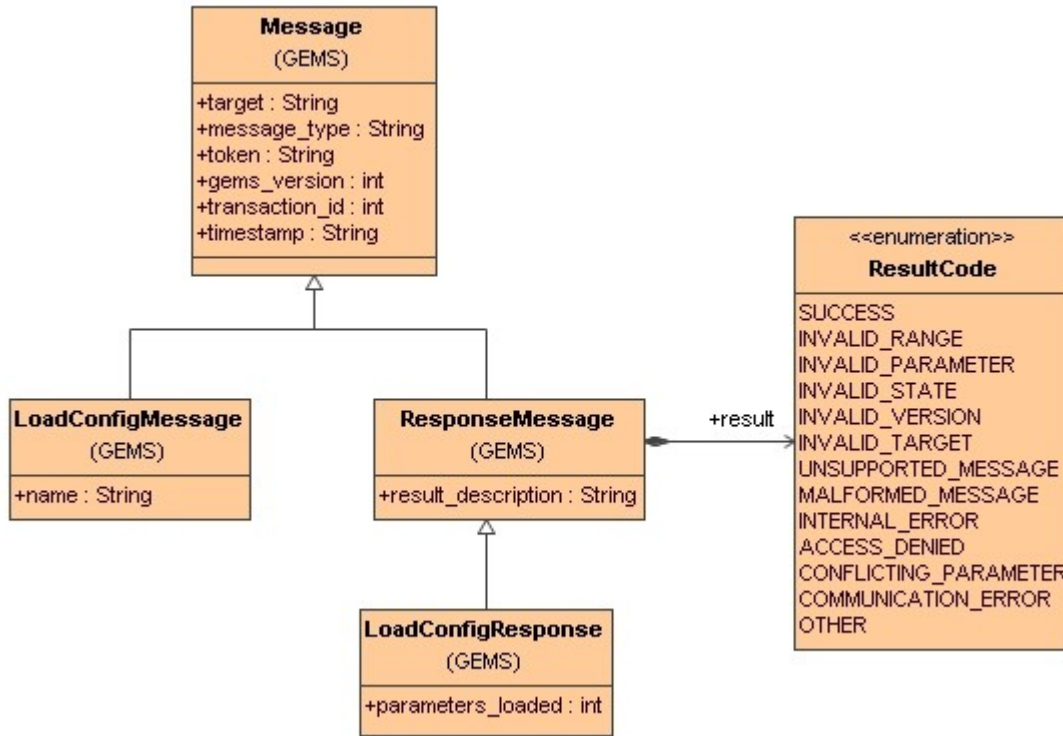
Figure 6.11 - Load Configuration UML
