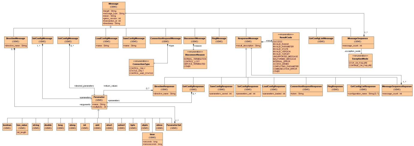
Figure 6.3 - GEMS UML
