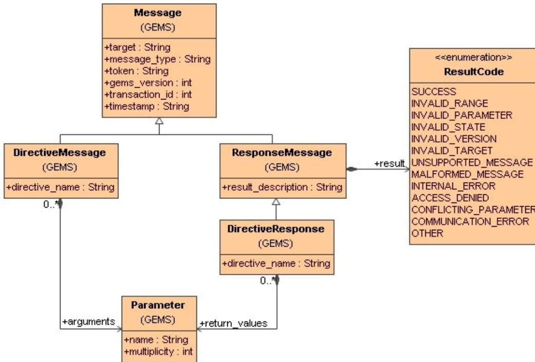
Figure 6.13 - Directive UML
