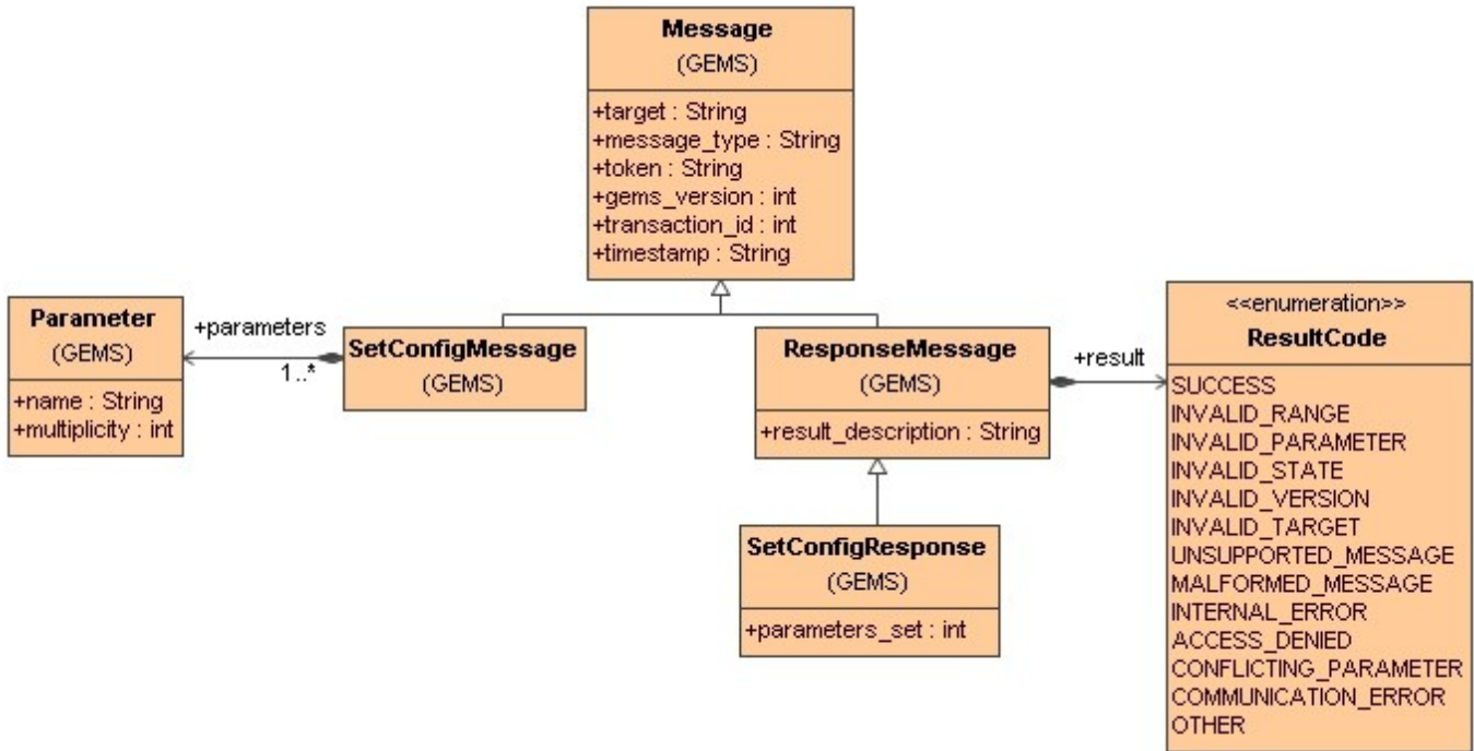
Figure 6.8 - Set Configuration Message Classes
