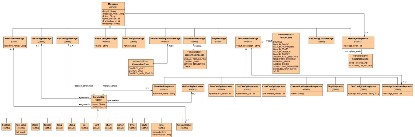
Figure 6.3 - GEMS UML
