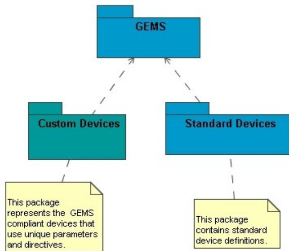
Figure 6.2 - GEMS Packages
