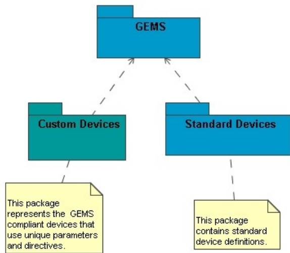
Figure 6.2 - GEMS Packages
