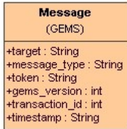
Figure 6.6 - GEMS Message Base Class
