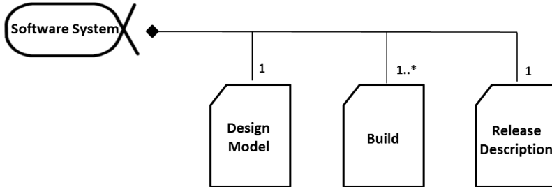
Figure 9.46 – Software System Alpha and three Work Products: Design Model, Build, and Release Description with visualized bounds
