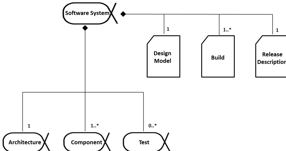
Figure 9.54 – Alpha Containment and Work Product Manifest relationships of the Software System Alpha
