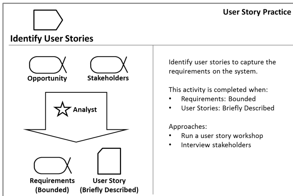
Figure 9.73 – Identify User Stories activity definition card
