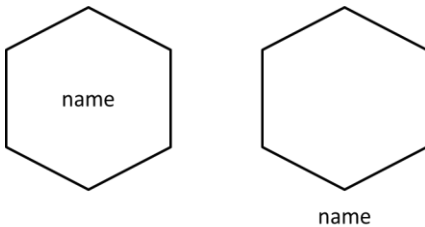
Figure 9.52 – Practice symbol
