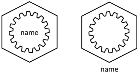
Figure 9.30 – Kernel symbol
