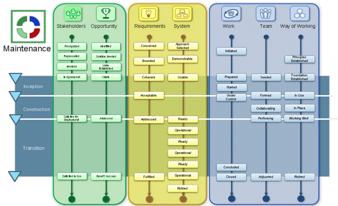
Figure E.32 – The Maintenance lifecycle
