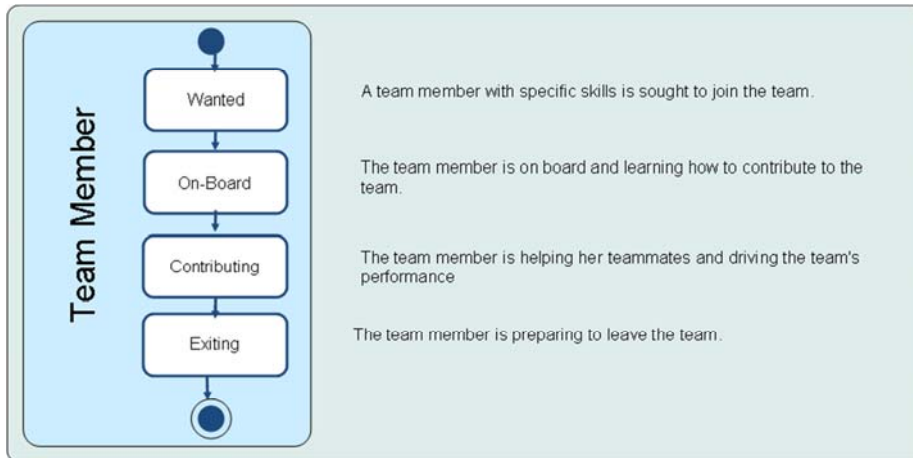
Figure 103 – The states of Team Member
