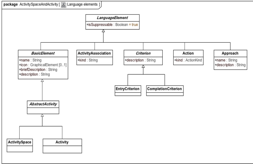
Figure 22 – ActivitySpaceAndActivity::Language elements
