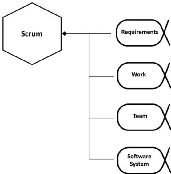
Figure 134 – Scrum practice
