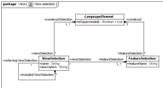
Figure 28 – View::View selection
