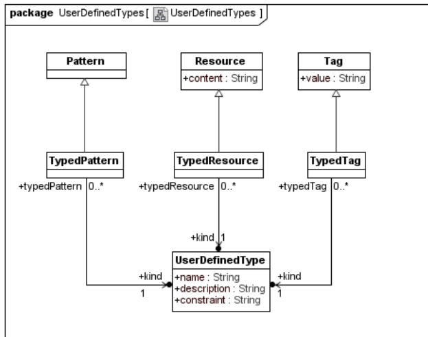
Figure 26 – UserDefinedTypes::UserDefinedTypes
