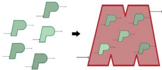
Figure 109 – Practices composition
