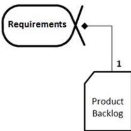
Figure 139 – Product Backlog
