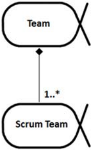
Figure 137 – Scrum Team
