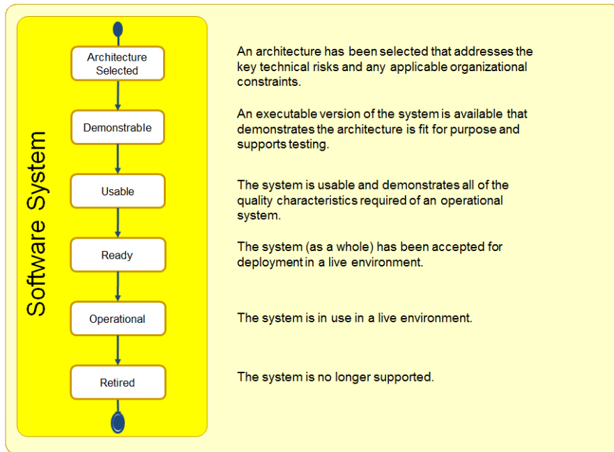
Figure 9 – The states of the Software System
