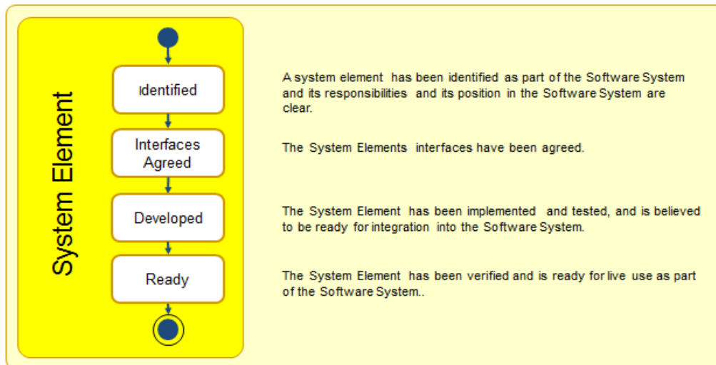
Figure 101 – The states of Software System Element
