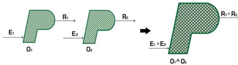
Figure 126 – Practice combination
