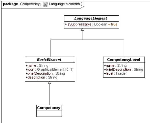
Figure 24 – Competency::Language elements
