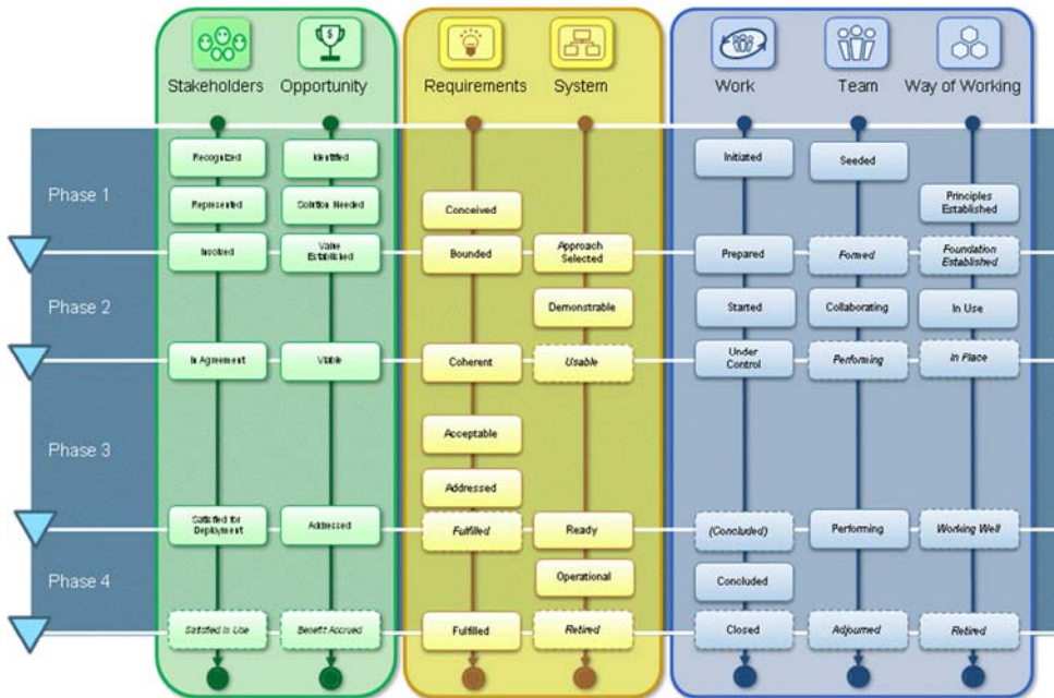
Figure 158 – Lifecycle template
