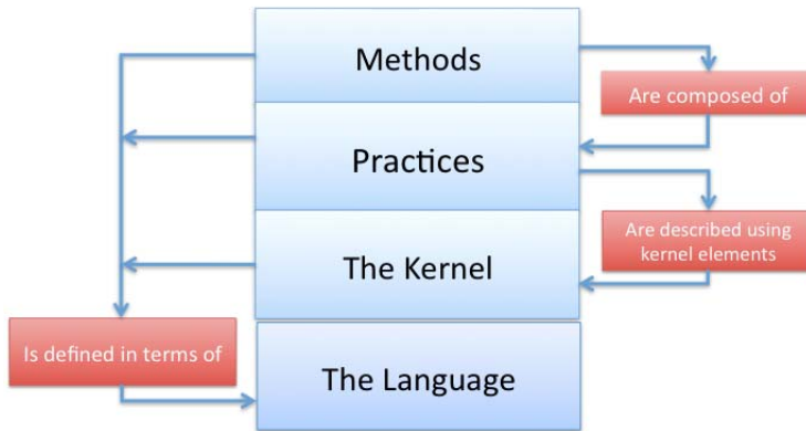
Figure 1 – Method architecture
