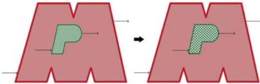
Figure 123 – Practice substitution
