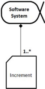
Figure 141 – Increment
