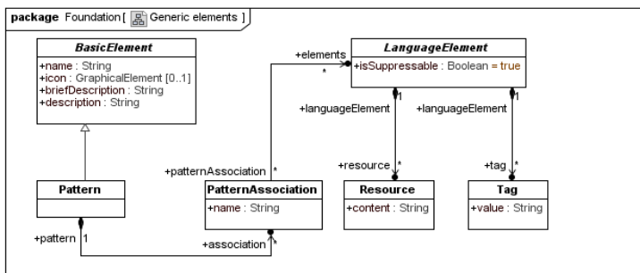
Figure 19 – Foundation::Generic elements
