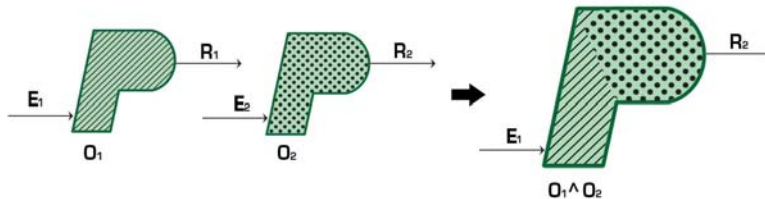
Figure 124 – Practice concatenation
