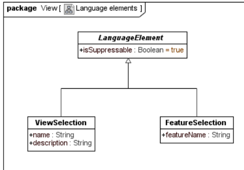
Figure 27 – View::Language elements
