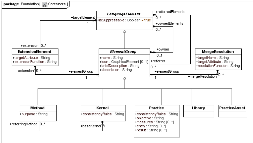
Figure 18 – Foundation::Containers
