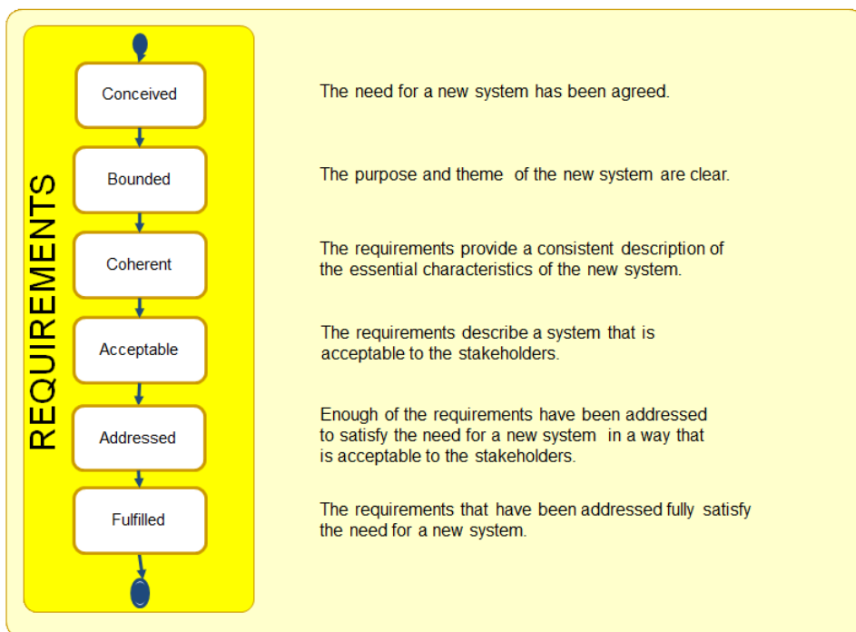
Figure 8 – The states of the Requirements
