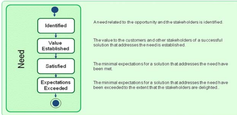
Figure 95 – The states of the Need
