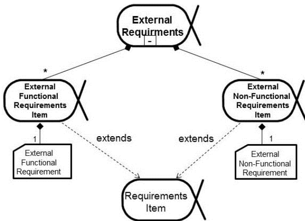
Figure 156 – External Requirements Sub-Alphas and Requirement Work Products
