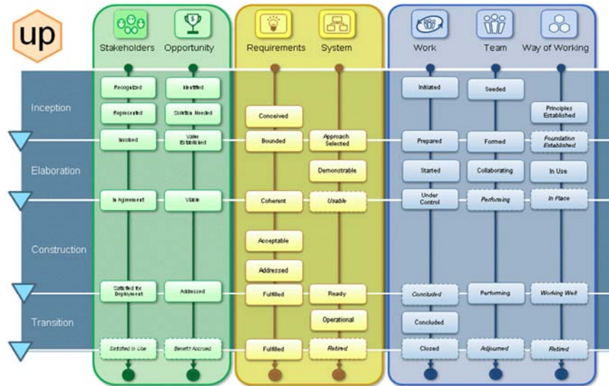
Figure 159 – The Unified Process lifecycle
