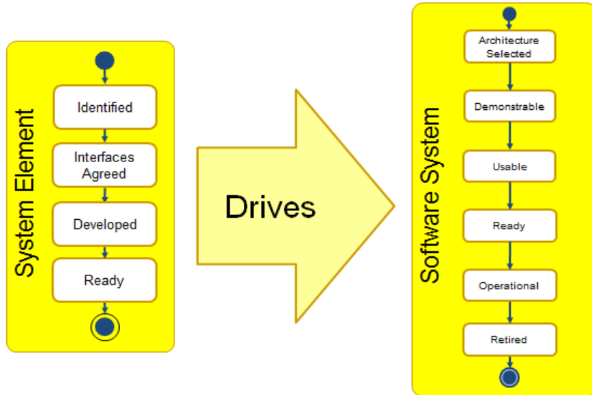
Figure 102 – The Software System Elements drive the progress of the Software System
