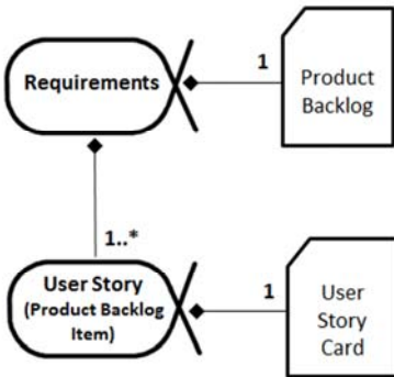
Figure 168 – Scrum with User Story
