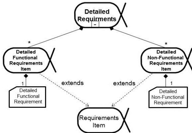
Figure 157 – Detailed Requirements Sub-Alphas and Requirement Work Products
