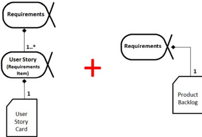
Figure 167 – Merging User Story with Scrum
