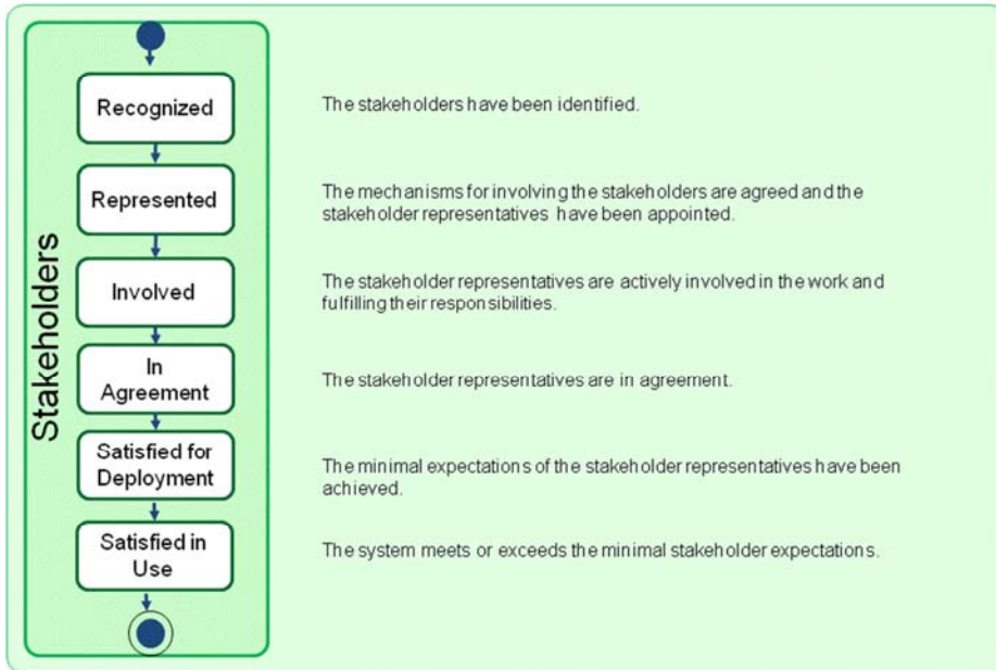
Figure 6 – The states of the Stakeholders
