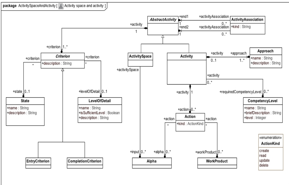
Figure 23 – ActivitySpaceAndActivity::Activity space and activity
