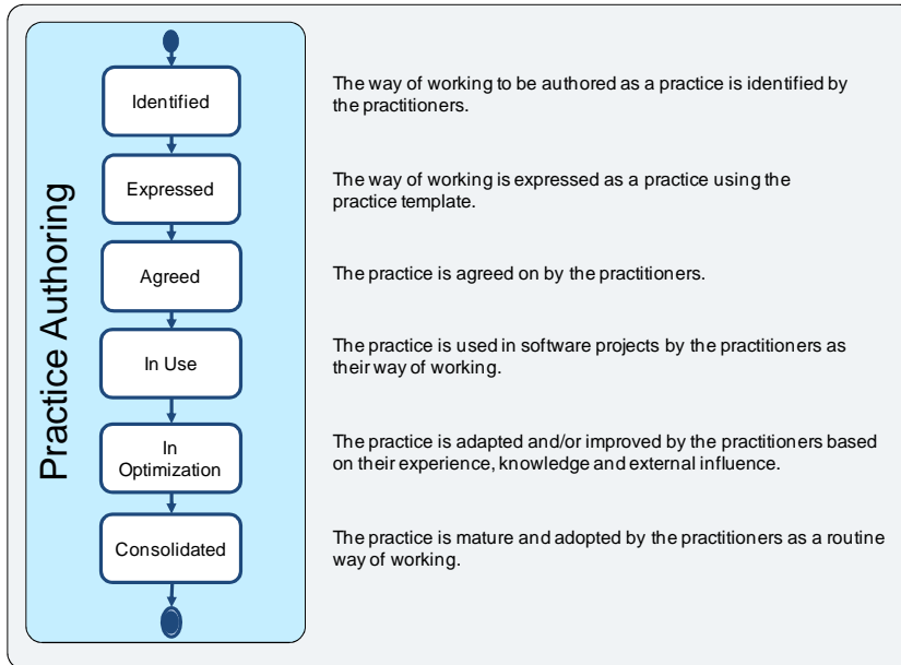
Figure 111 – The states of Practice Authoring
