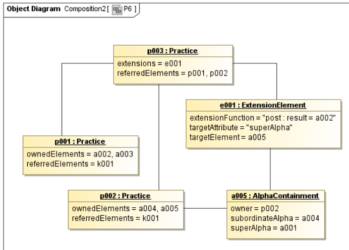
Figure 33 – Partial object diagrams for P6
