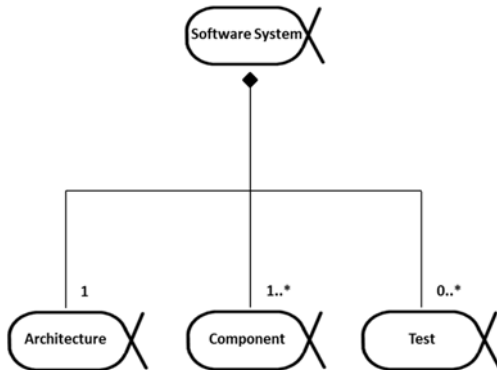
Figure 56 – Software System super-Alpha and three sub-Alphas: Architecture, Component, and Test with visualized bounds
