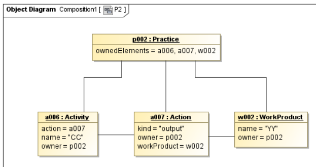
Figure 30 – Object diagrams for P1 and P2
