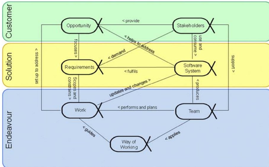
Figure 3 – The Kernel Alphas
