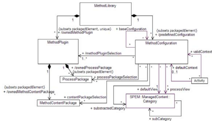
Figure 131 – SPEM Method Library and Configurations
