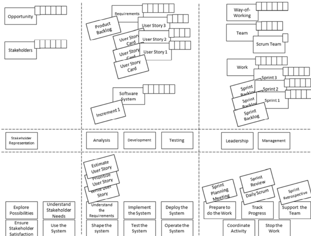
Figure 169 – Illustration of the complete initial set of cards for the example. Top section shows Alpha cards, attached Work Product cards (rotated) and attached Alpha State cards (small). Middle section shows Competency cards. Bottom section shows Activity Space cards with attached Activity cards (rotated).
