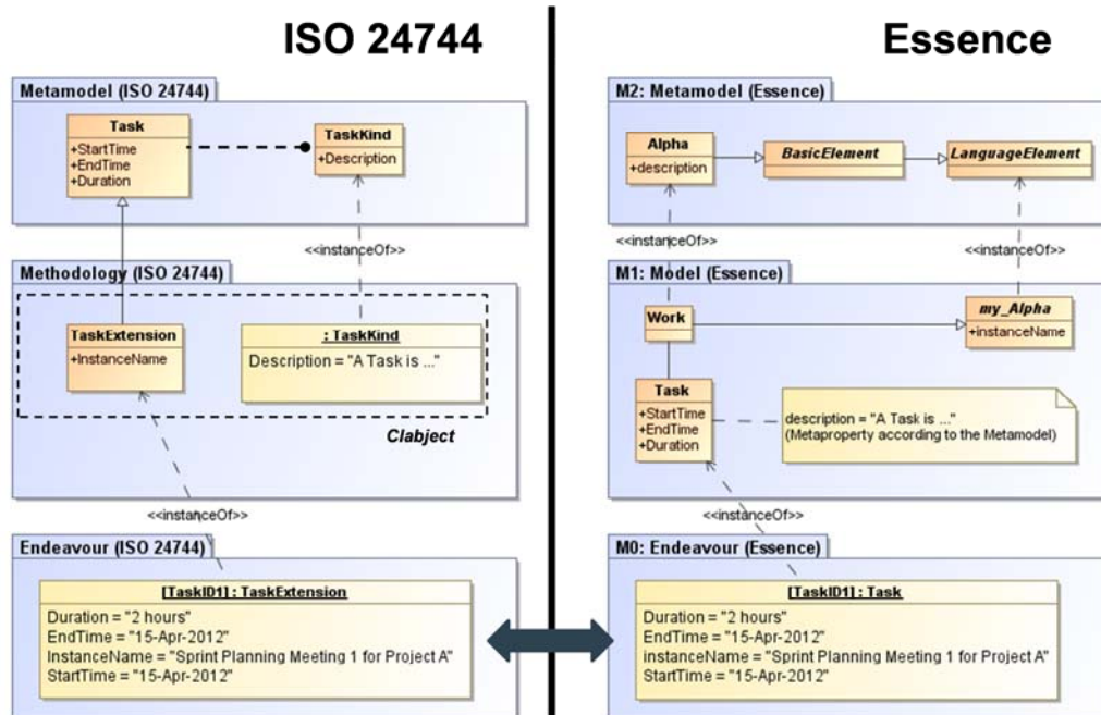
Figure 133 – Task example alignment between ISO 24744 and Essence
