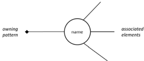
Figure 89 – Pattern Association symbol
