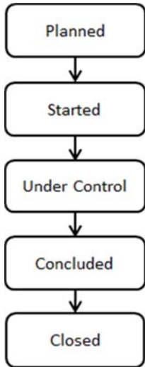
Figure 136 – The states of the Sprint sub-alpha
