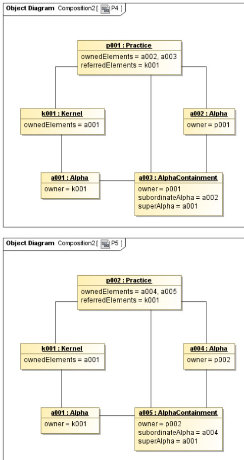
Figure 32 – Object diagrams for P4 and P5
