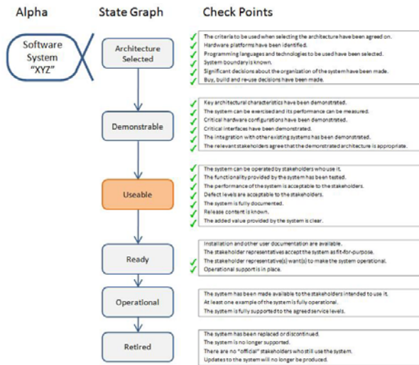
Figure 35 – Determination of State using Check Points
