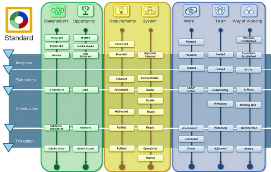
Figure 164 – The Standard lifecycle
