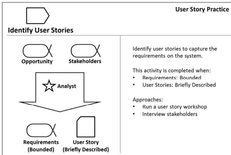
Figure 84 – Identify User Stories activity definition card
