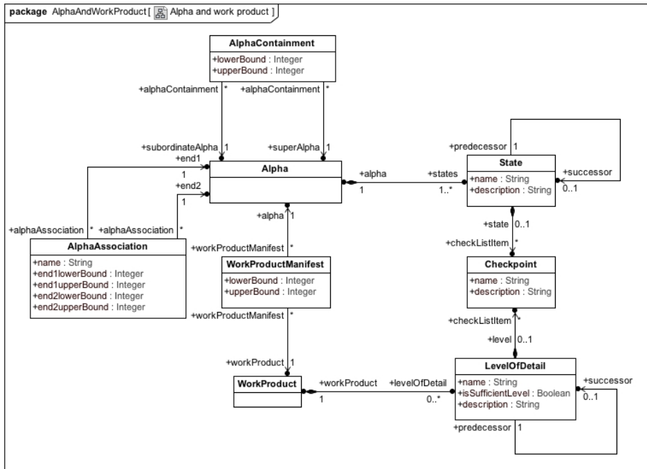
Figure 21 – AlphaAndWorkProduct::Alpha and work product
