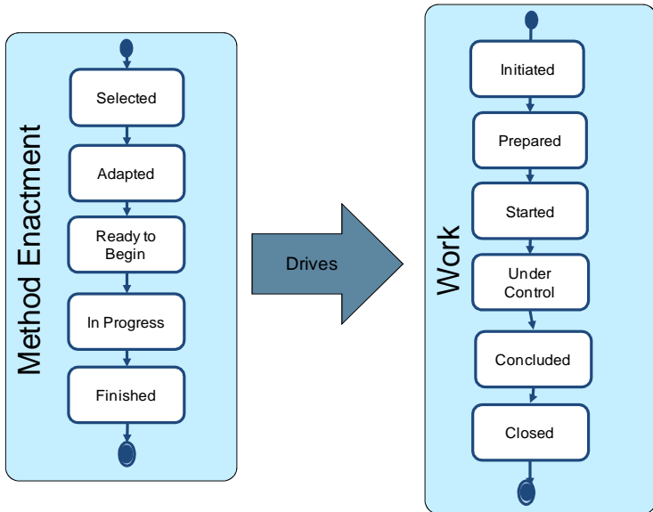
Figure 127 – Method Enactment Drives the progress of the Work
