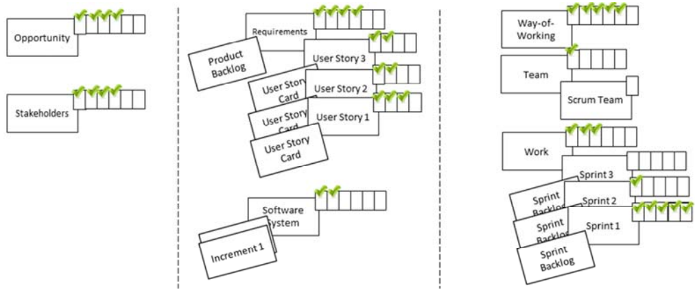
Figure 171 – Illustration of the updated overall state in the example. Some Alphas have advanced in their states, thus having more of their Alpha States ticked off. Others were set back to an earlier state. An additional Work Product card has been added to the Alpha “Software System”.
