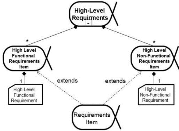
Figure 155 – High-Level Requirements Sub-Alphas and Requirement Work Products
