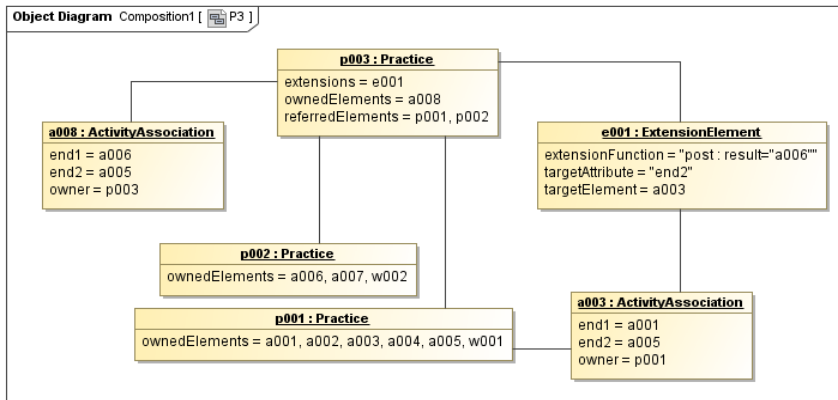
Figure 31 – Partial object diagram for P3
