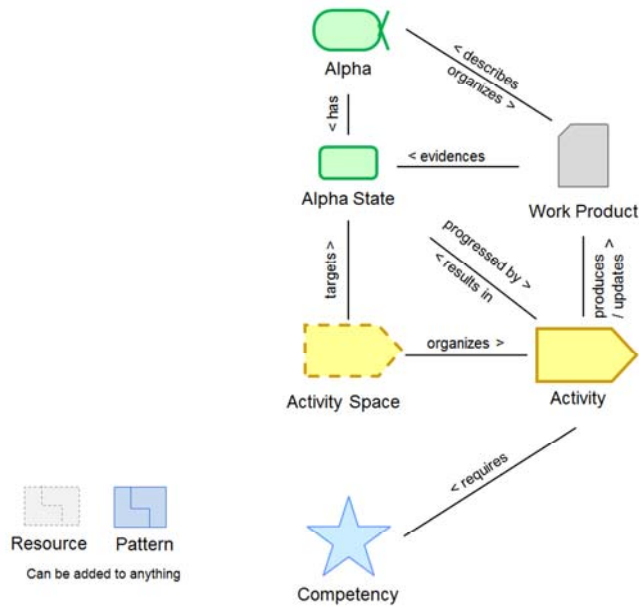
Figure 13 –Conceptual Overview of the Language
