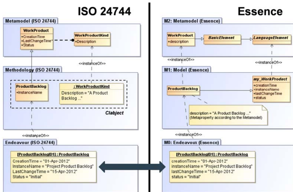
Figure 132 – WorkProduct example alignment between ISO 24744 and Essence
