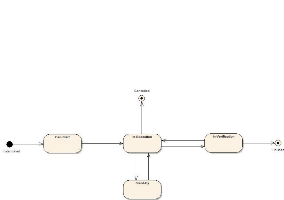
Figure 119 – Practice Instance Lifecycle
