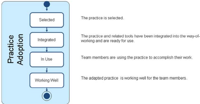
Figure 107 – The states of Practice Adoption
