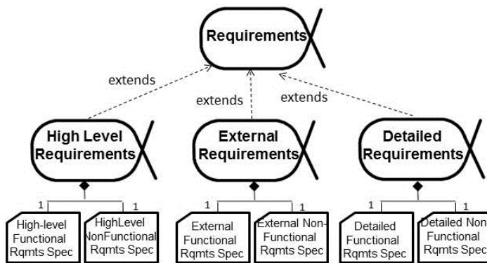
Figure 153 – Multi-phase Waterfall Requirements Alpha Extensions and Requirements Spec Work Products
