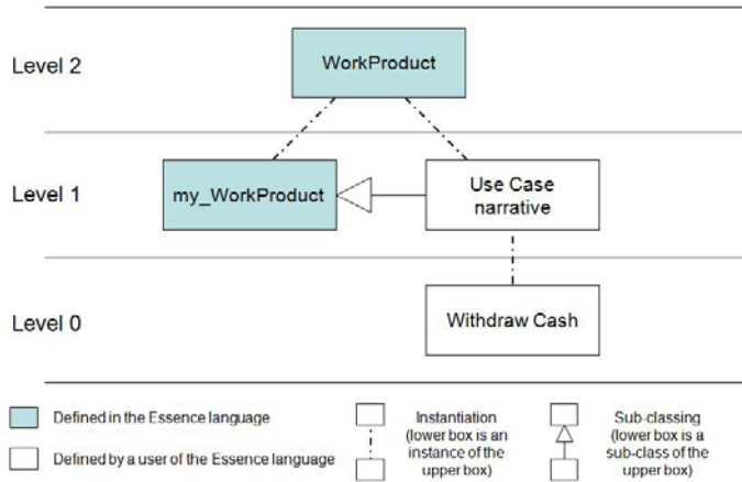
Figure 34 – The Essence language framework
