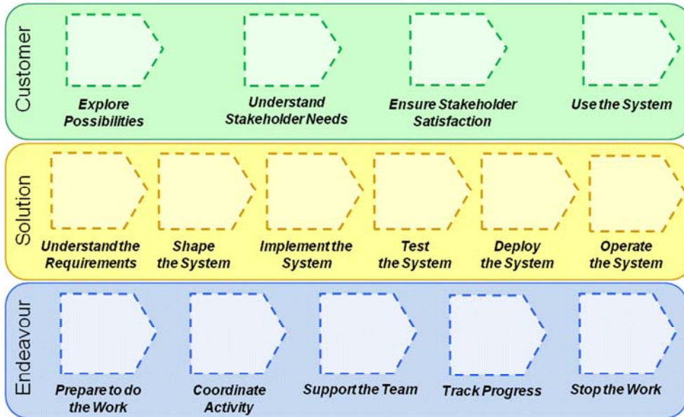
Figure 4 – The Kernel Activity Spaces
