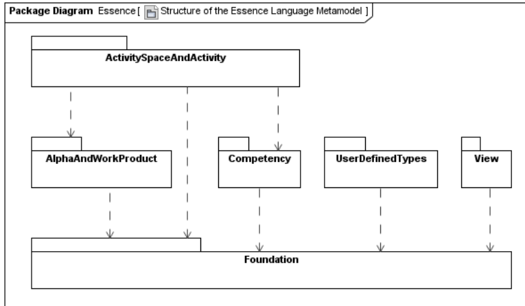
Figure 15 – Structure of the Essence Language metamodel
