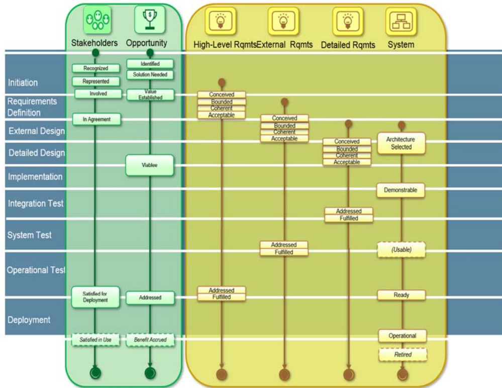
Figure 154 – Lifecycle Diagram for Multi-Phase Waterfall Requirements Alpha Extensions
