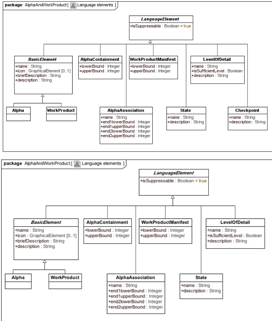
Figure 20 – AlphaAndWorkProduct::Language elements
