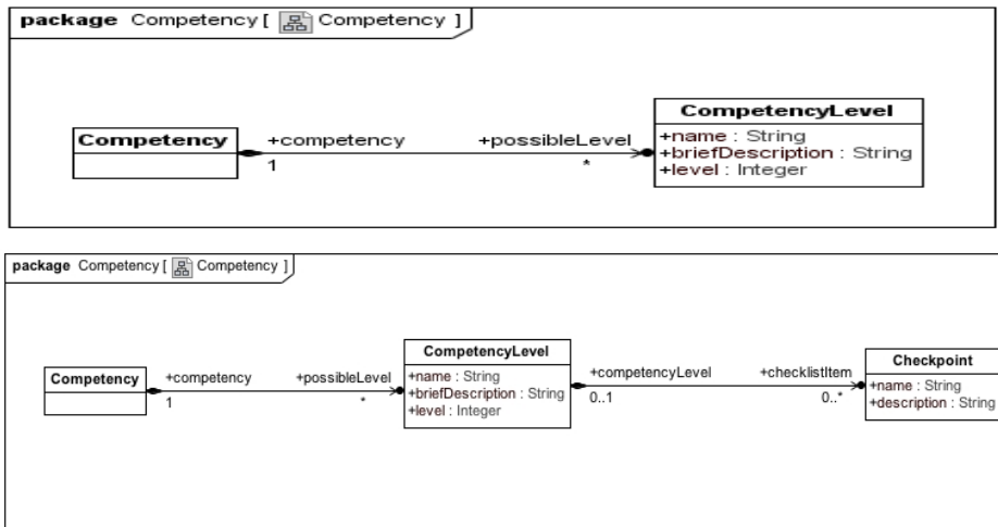
Figure 25 – Competency::Competency
