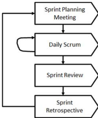
Figure 142 – Scrum activities
