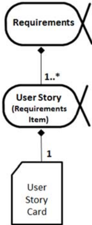
Figure 148 – User Story
