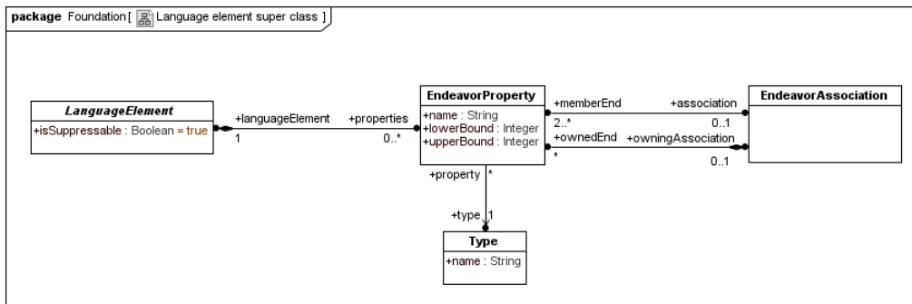
Figure 16 – Foundation::Language element super class
