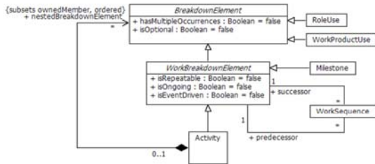
Figure 130 – A SPEM breakdown structure is defined by Activities nesting Breakdown Elements
