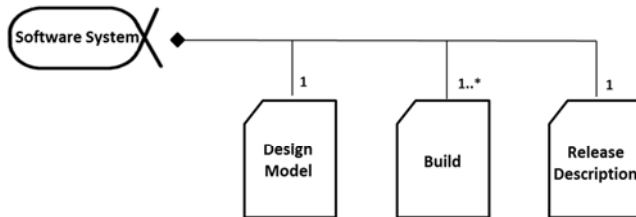
Figure 58 – Software System Alpha and three Work Products: Design Model, Build, and Release Description with visualized bounds
