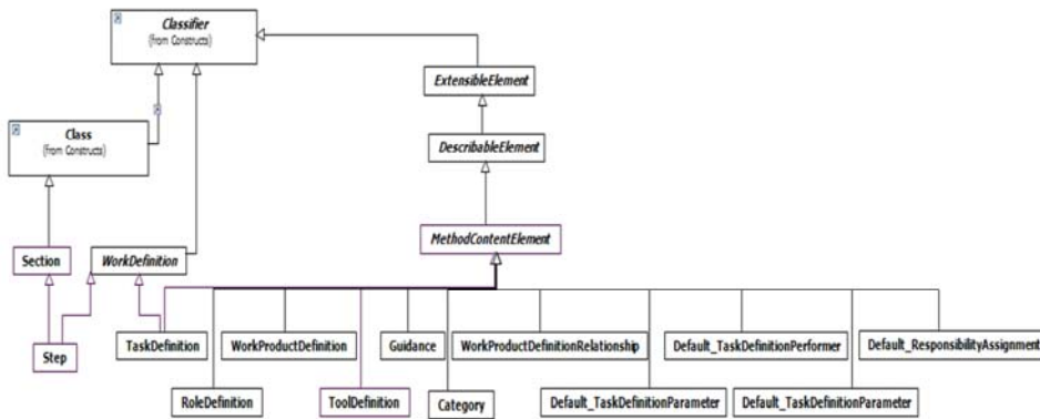
Figure 129 – SPEM Taxonomy of Core Describable Elements
