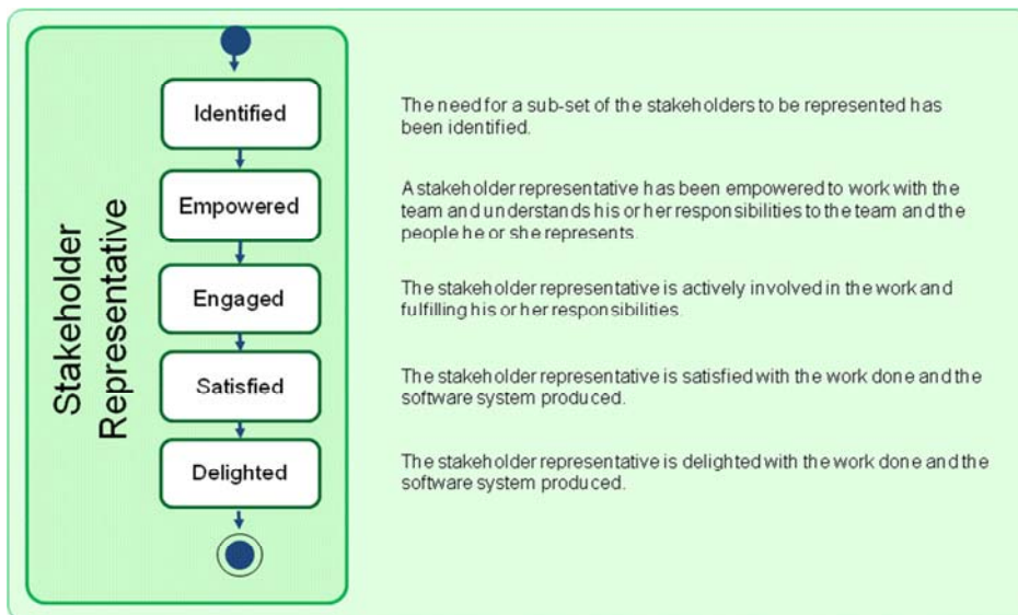
Figure 93 – The states of the Stakeholder Representative
