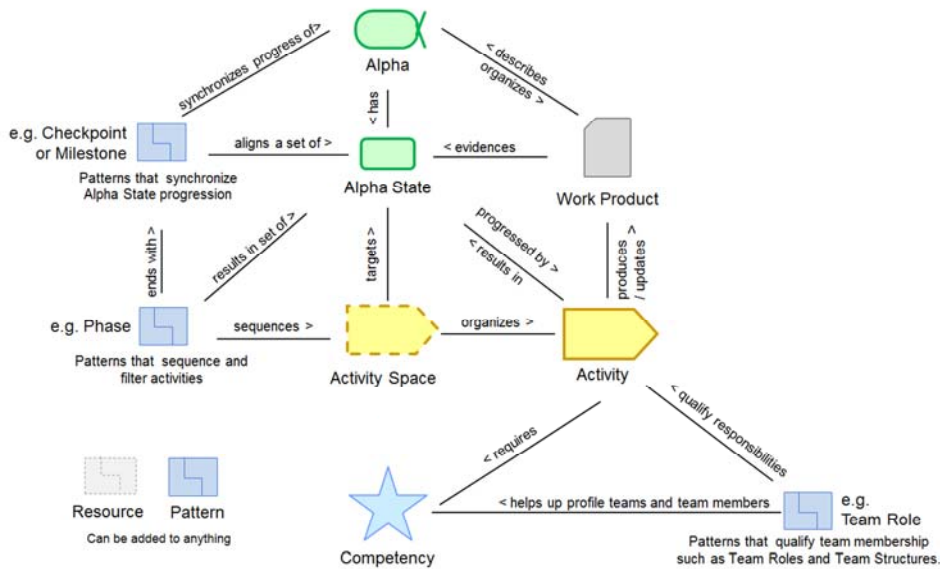
Figure 14 – Examples of Patterns
