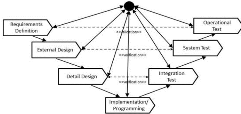
Figure 152 – Multi-phase Waterfall Practice Activities Flow
