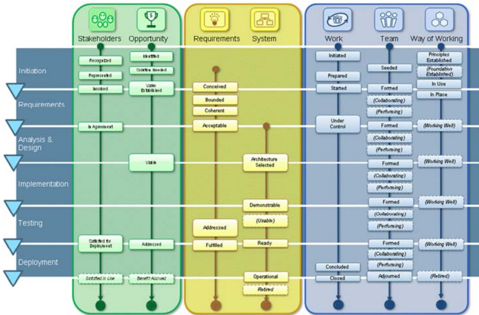
Figure 160 – A Waterfall lifecycle
