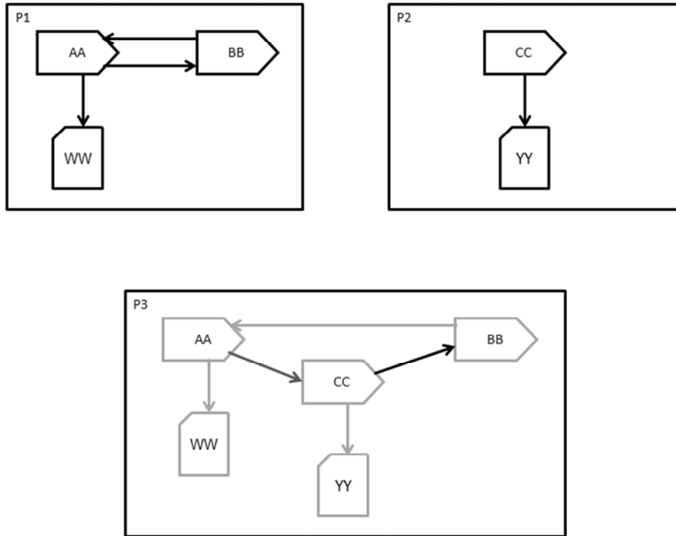
Figure 29 – Two practices P1 and P2 and their merge result P3. Elements that are referred to by P3 are shown in light grey. Elements that are modified by P3 are shown in dark grey. Elements that are owned by P3 are shown in black.
