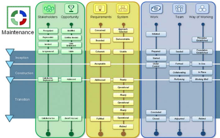
Figure 165 – The Maintenance lifecycle
