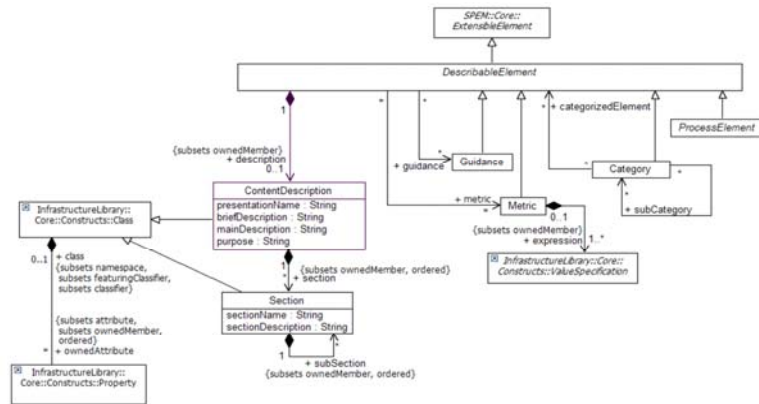
Figure 128 – SPEM Describable Element parts and subclasses
