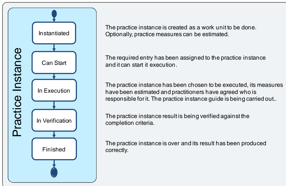
Figure 118 – The Practice Instance states
