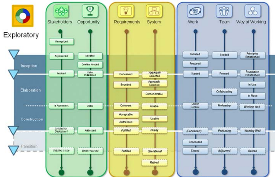
Figure 163 – The Exploratory lifecycle
