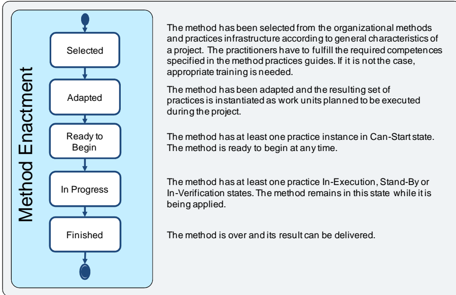
Figure 121 – The states of Method Enactment
