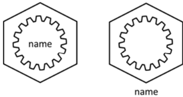
Figure 42 – Kernel symbol
