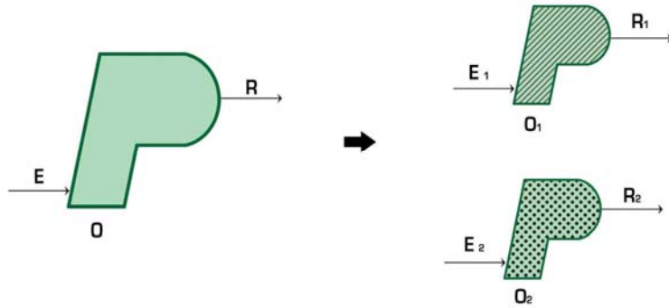
Figure 125 – Practice splitting
