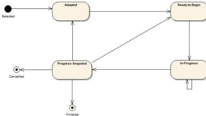
Figure 122 – Method Enactment
