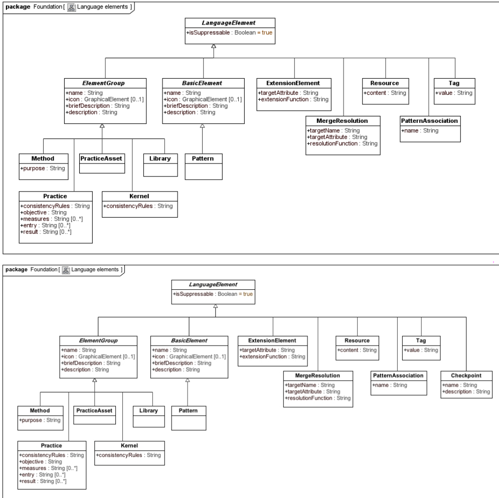
Figure 17 – Foundation::Language elements
