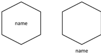
Figure 64 – Practice symbol
