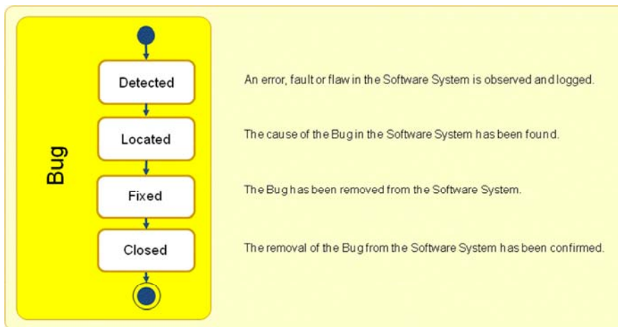
Figure 99 – The states of a Bug
