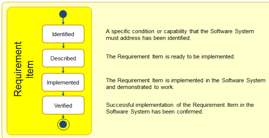
Figure 97 – The states of Requirement Item
