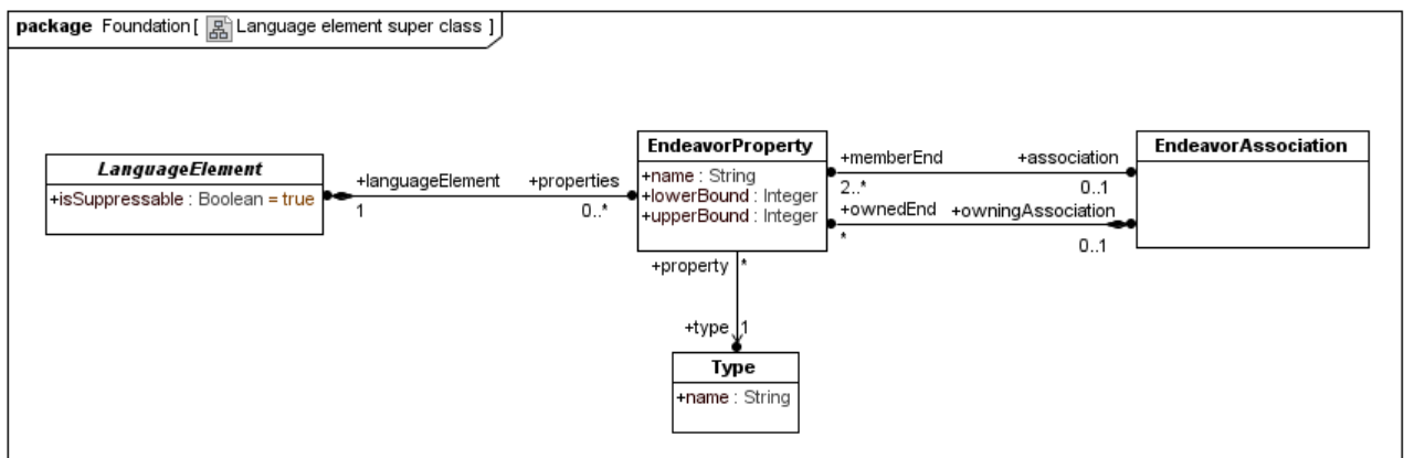
Figure 16 – Foundation::Language element super class
