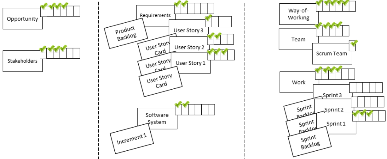
Figure 170 – Illustration of the individual Alpha State cards marking the overall state. States with all checkpoints fulfilled in the example are ticked off with a green check mark at the related Alpha State cards.
