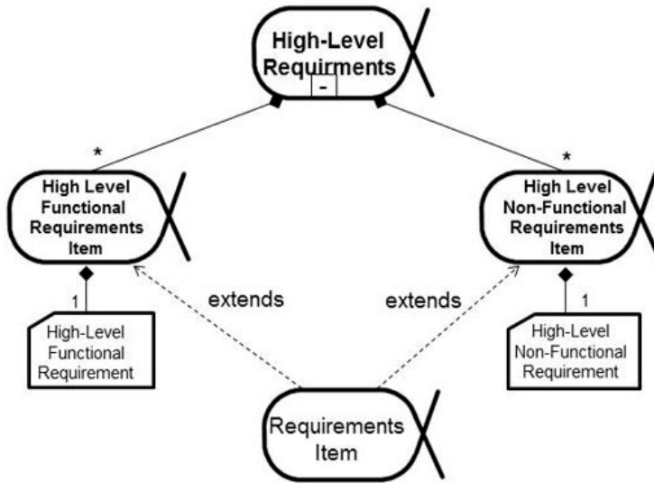
Figure 155 – High-Level Requirements Sub-Alphas and Requirement Work Products
