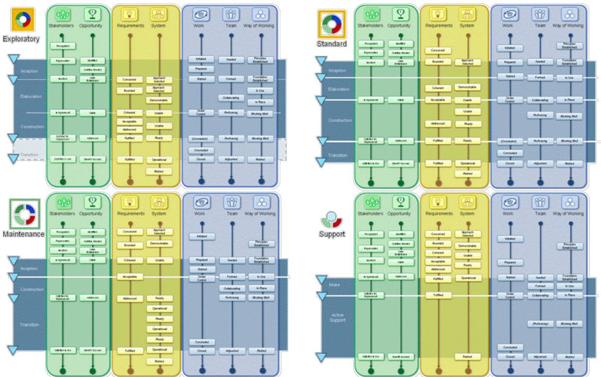
Figure 162 – Four complementary lifecycles to support application development
