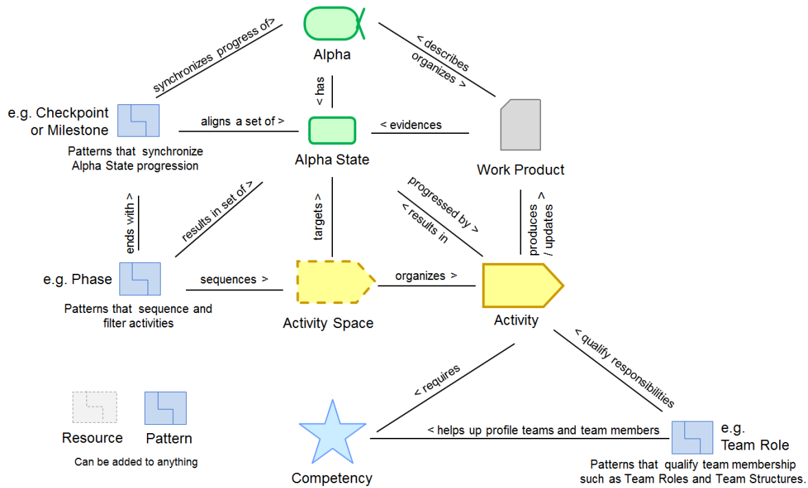
Figure 14 – Examples of Patterns
