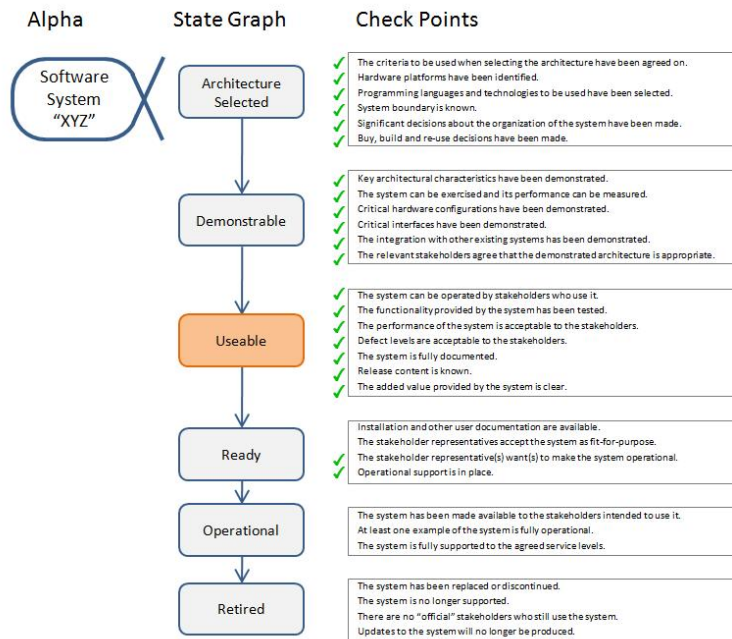
Figure 35 – Determination of State using Check Points
