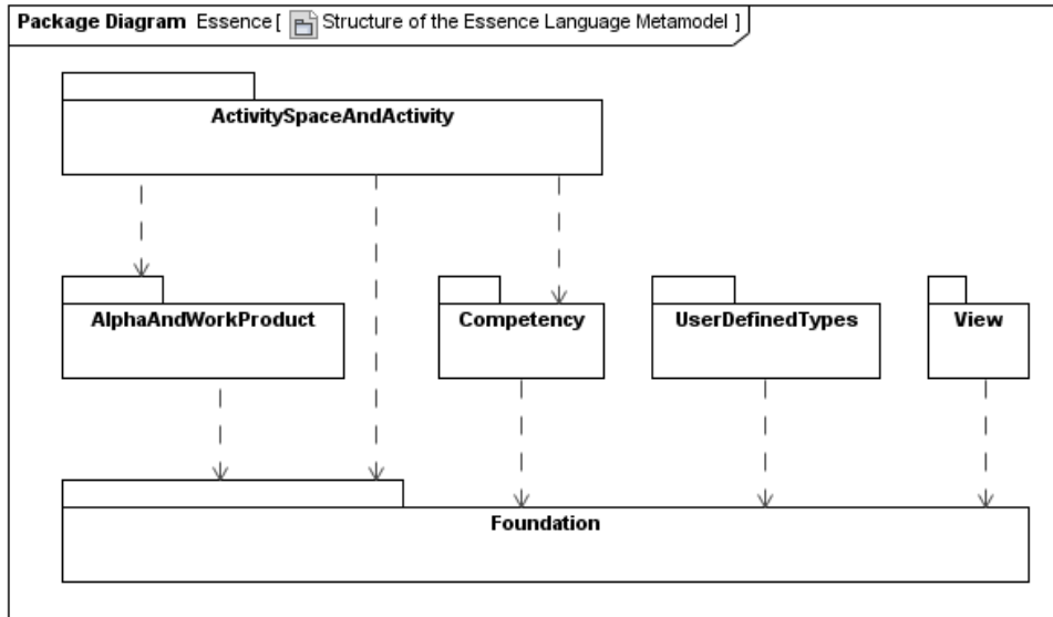
Figure 15 – Structure of the Essence Language metamodel
