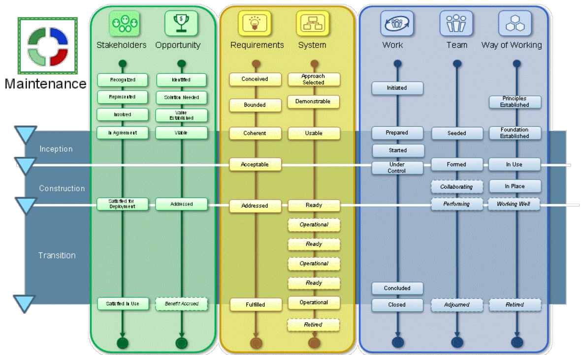
Figure 165 – The Maintenance lifecycle
