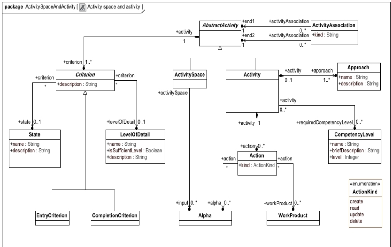
Figure 23 – ActivitySpaceAndActivity::Activity space and activity
