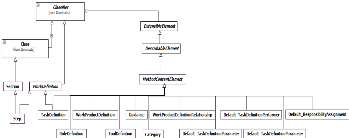
Figure 129 – SPEM Taxonomy of Core Describable Elements
