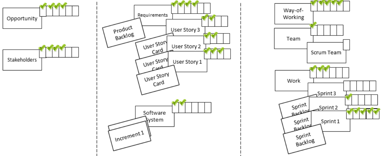
Figure 171 – Illustration of the updated overall state in the example. Some Alphas have advanced in their states, thus having more of their Alpha States ticked off. Others were set back to an earlier state. An additional Work Product card has been added to the Alpha “Software System”.
