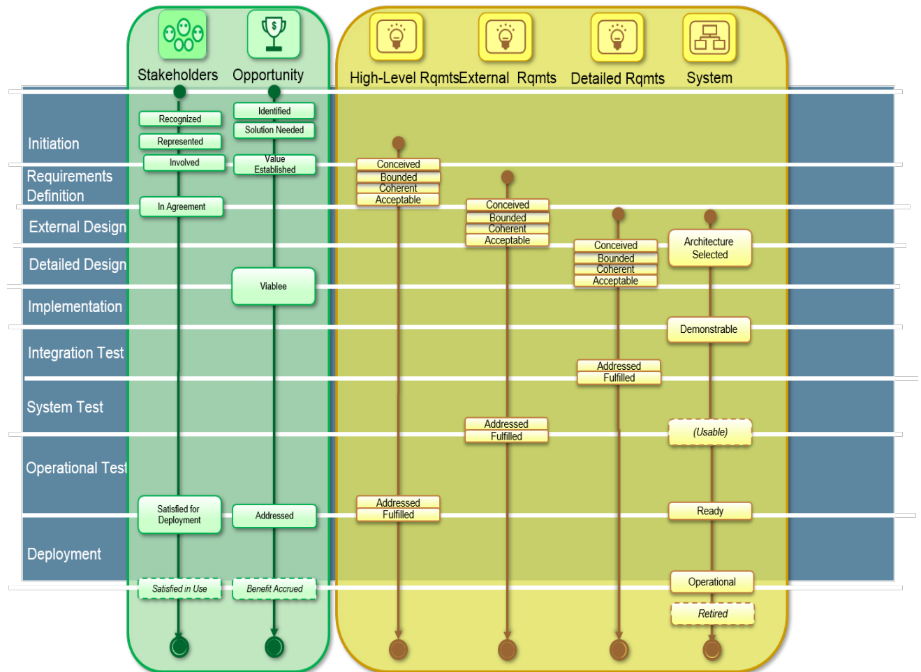
Figure 154 – Lifecycle Diagram for Multi-Phase Waterfall Requirements Alpha Extensions
