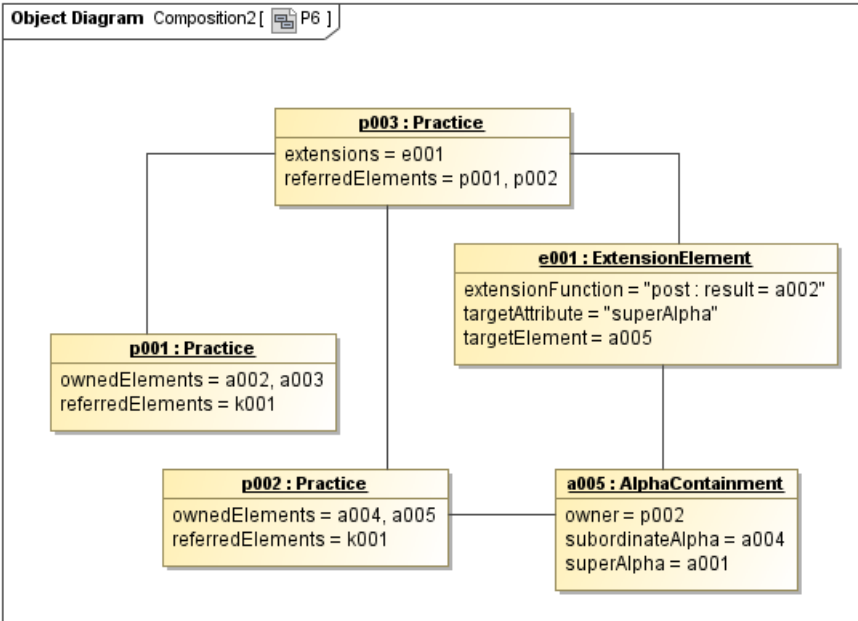
Figure 33 – Partial object diagrams for P6
