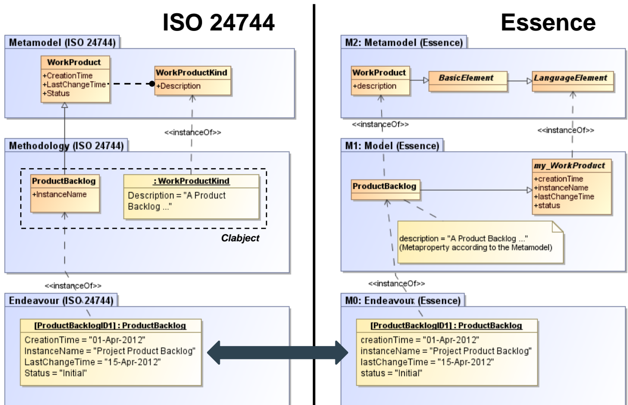
Figure 132 – WorkProduct example alignment between ISO 24744 and Essence
