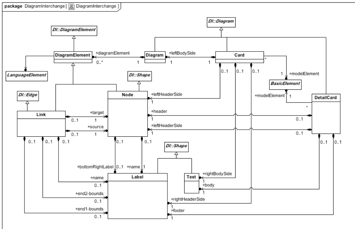
Figure 36 - Metamodel of the graphical syntax for diagram interchange
