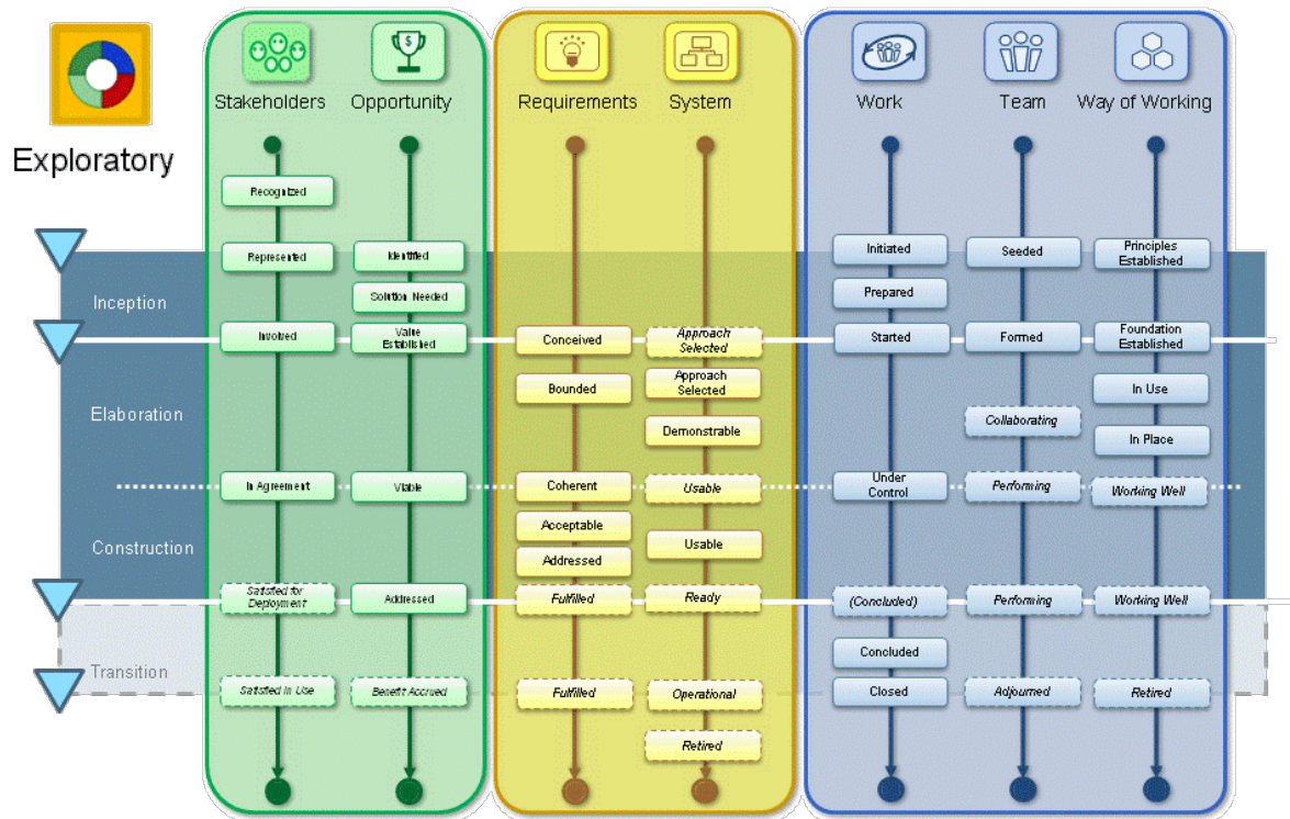
Figure 163 – The Exploratory lifecycle
