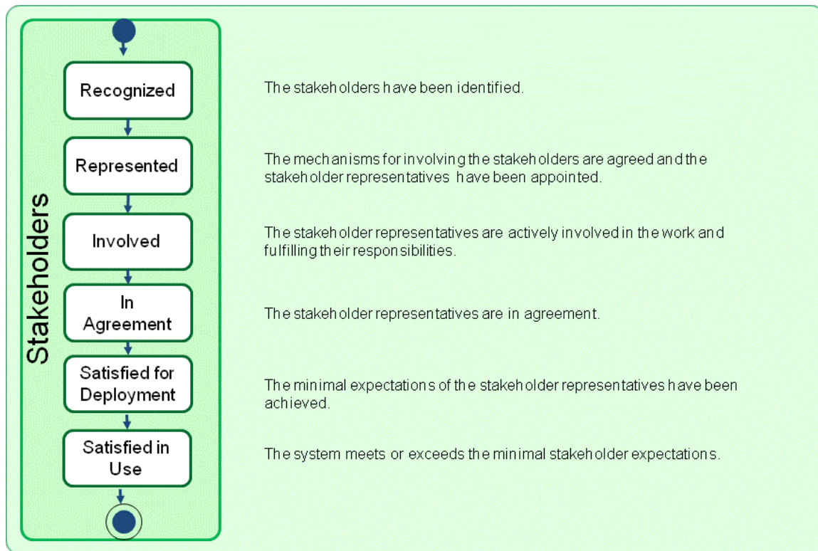
Figure 6 – The states of the Stakeholders
