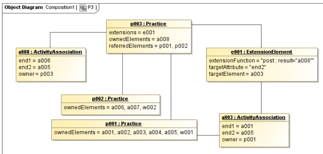
Figure 31 – Partial object diagram for P3
