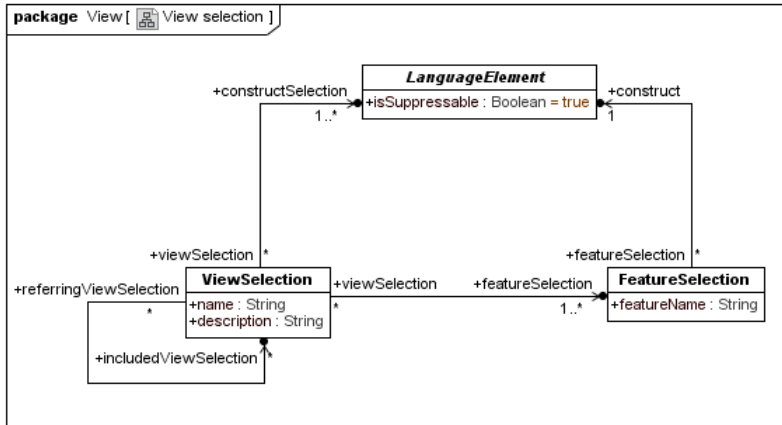
Figure 28 – View::View selection
