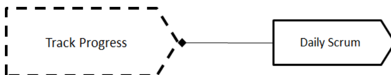
Figure 144 – Daily Scrum
