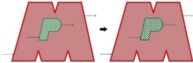
Figure 123 – Practice substitution
