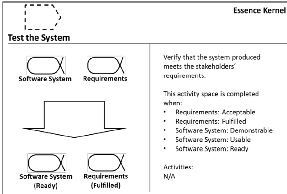
Figure 85 – Test the System Activity Space definition card
