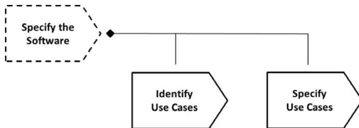
Figure 74 – Specify the Software Activity Space and two Activities: Identify Use Cases and Specify Use Cases
