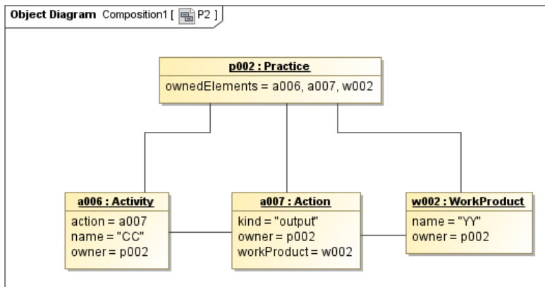
Figure 30 – Object diagrams for P1 and P2
