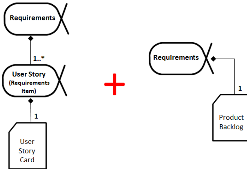
Figure 167 – Merging User Story with Scrum
