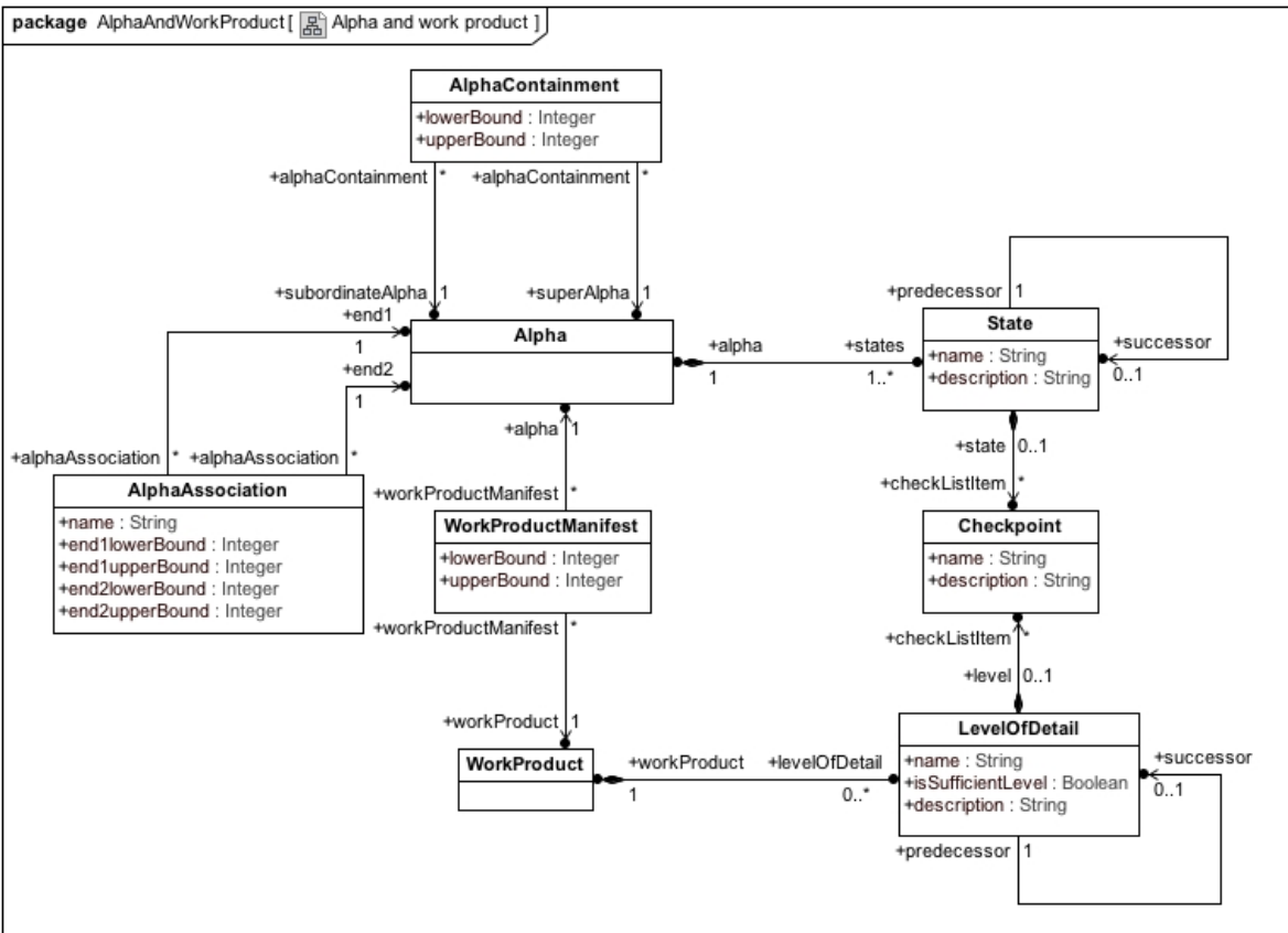
Figure 21 – AlphaAndWorkProduct::Alpha and work product
