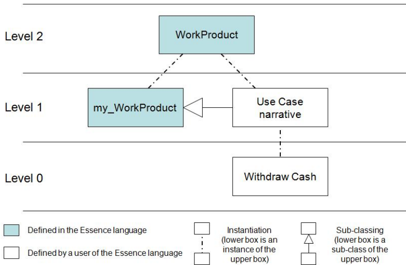
Figure 34 – The Essence language framework
