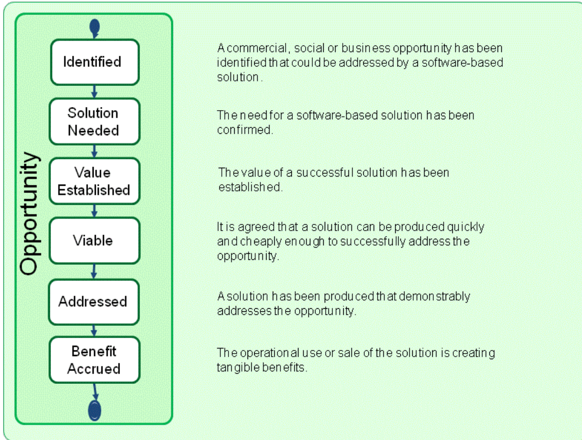
Figure 7 – The states of the Opportunity
