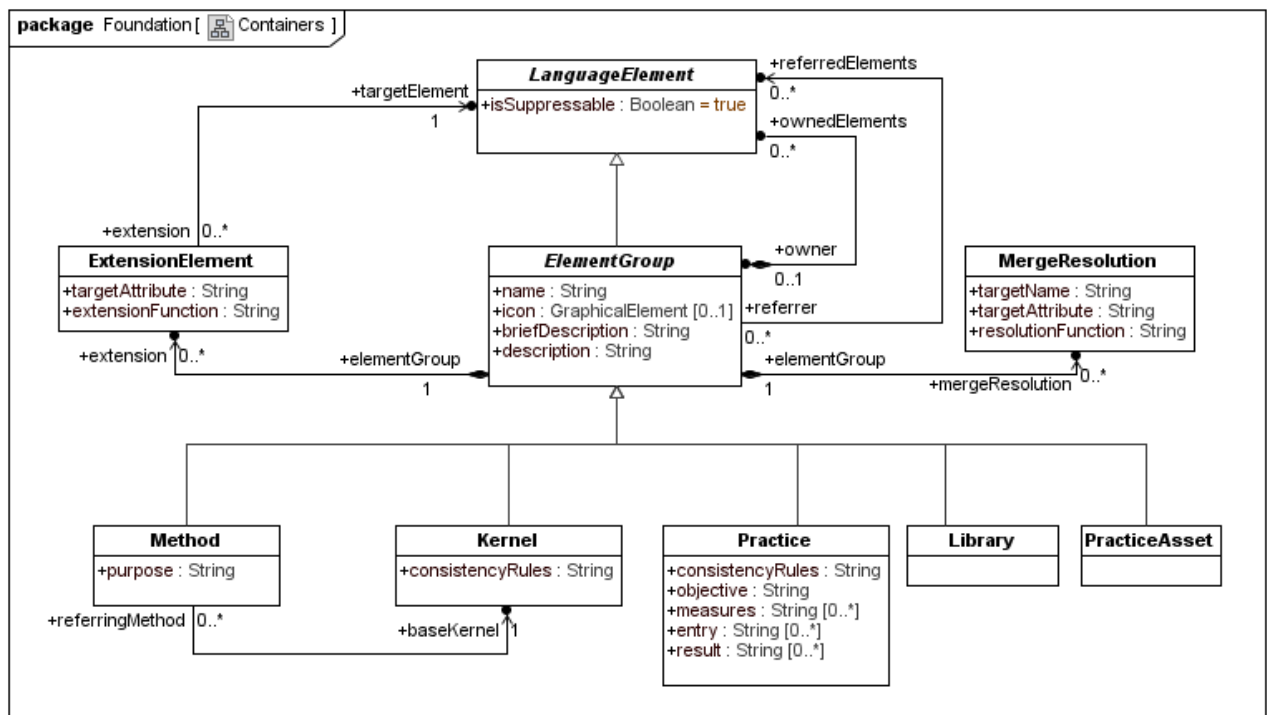
Figure 18 – Foundation::Containers
