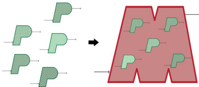
Figure 109 – Practices composition
