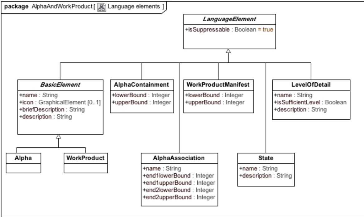
Figure 20 – AlphaAndWorkProduct::Language elements
