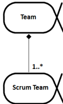
Figure 137 – Scrum Team
