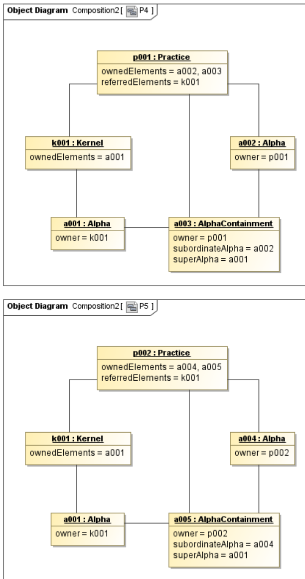
Figure 32 – Object diagrams for P4 and P5
