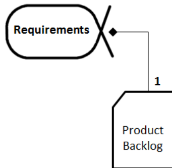
Figure 139 – Product Backlog
