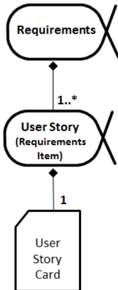
Figure 148 – User Story
