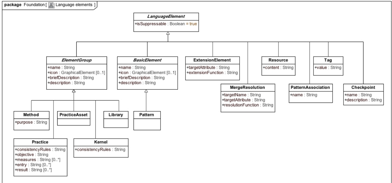
Figure 17 – Foundation::Language elements
