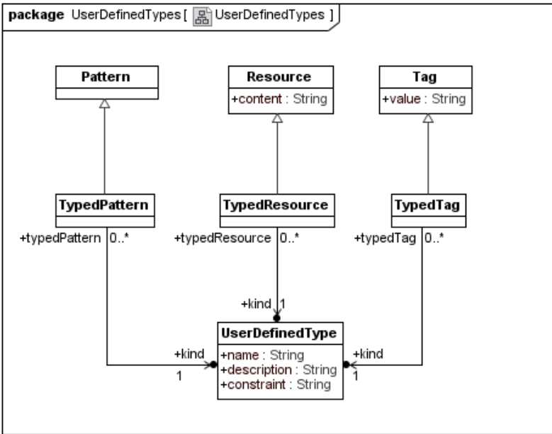
Figure 26 – UserDefinedTypes::UserDefinedTypes
