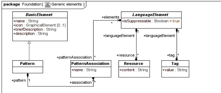
Figure 19 – Foundation::Generic elements
