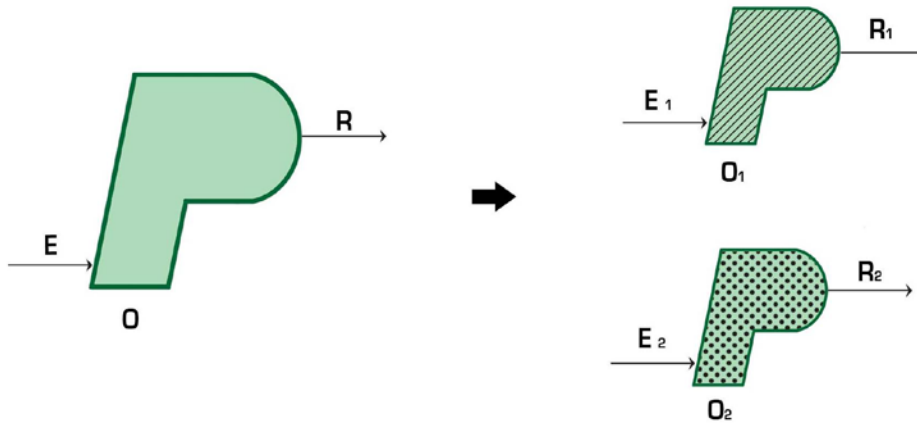
Figure 125 – Practice splitting
