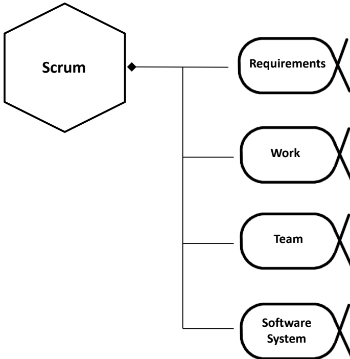
Figure 134 – Scrum practice
