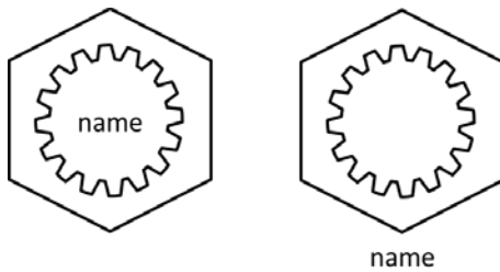
Figure 42 – Kernel symbol
