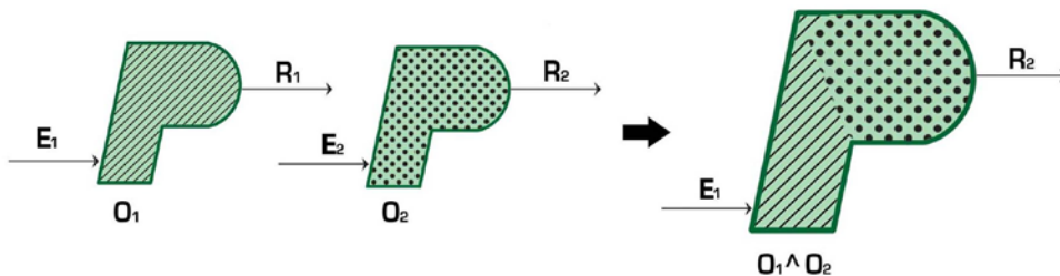
Figure 124 – Practice concatenation
