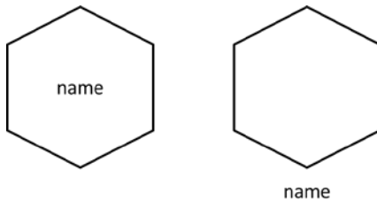
Figure 64 – Practice symbol
