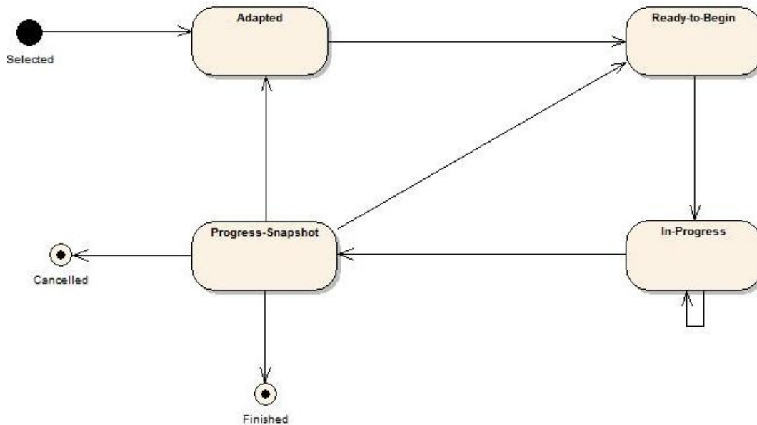
Figure 122 – Method Enactment
