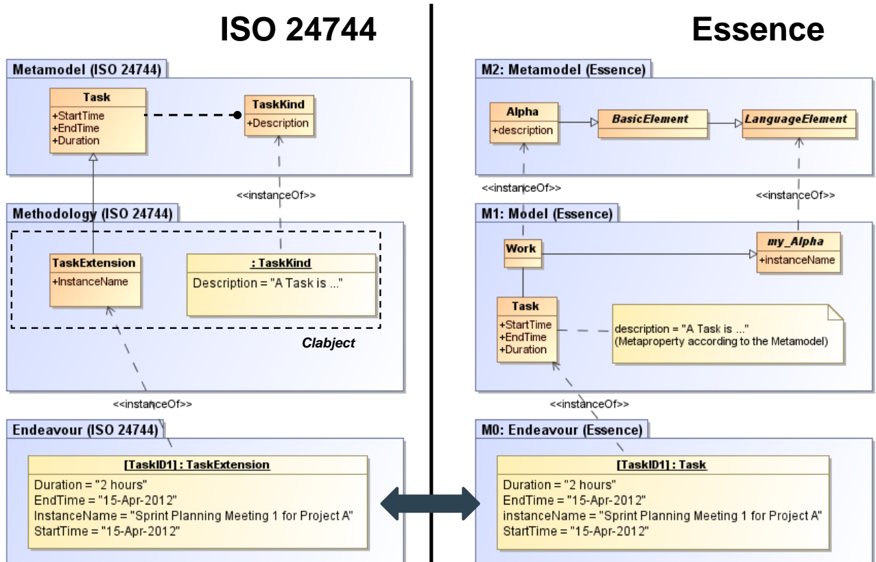
Figure 133 – Task example alignment between ISO 24744 and Essence
