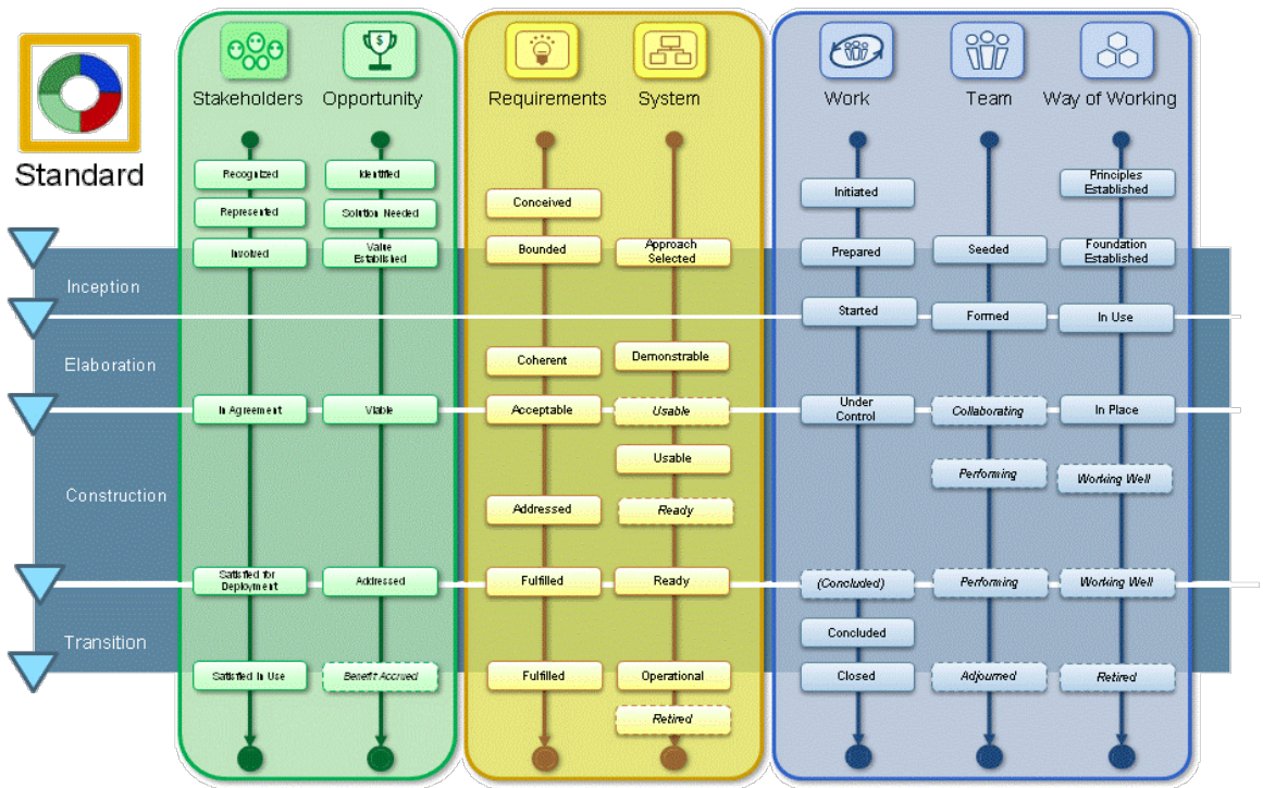
Figure 164 – The Standard lifecycle
