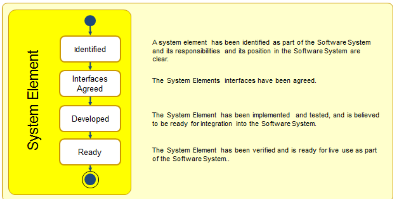
Figure 101 – The states of Software System Element
