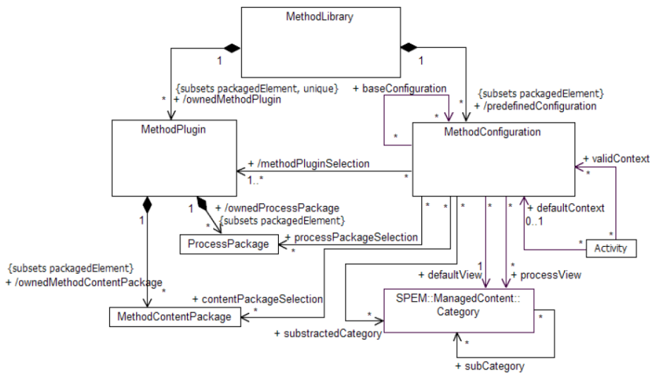
Figure 131 – SPEM Method Library and Configurations
