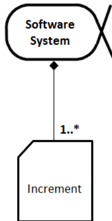
Figure 141 – Increment
