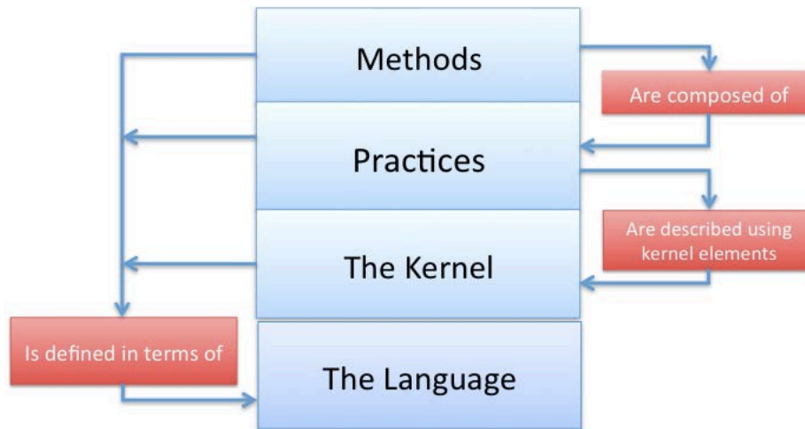
Figure 1 – Method architecture
