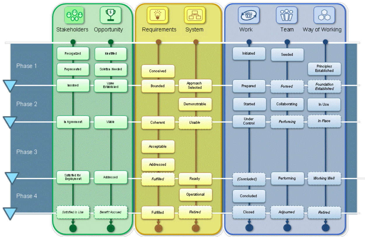
Figure 158 – Lifecycle template
