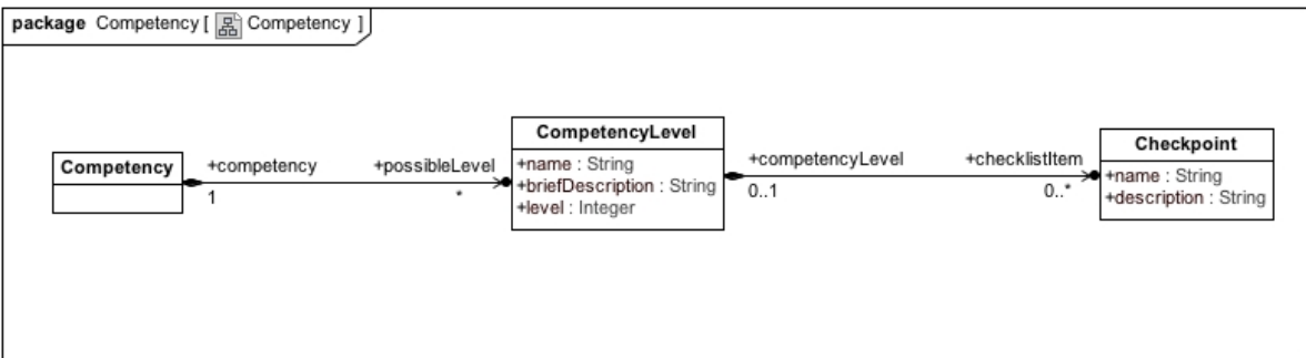
Figure 25 – Competency::Competency
