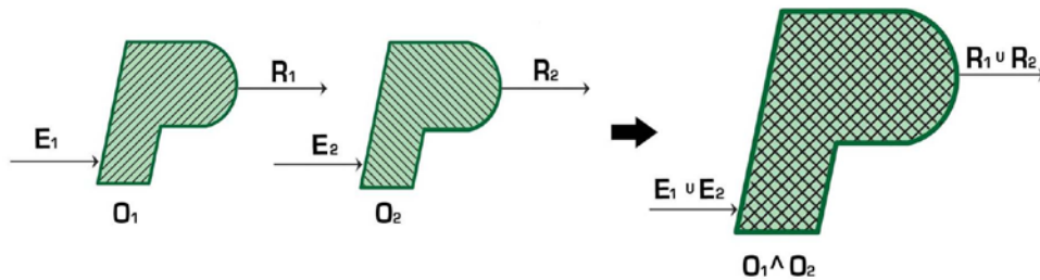
Figure 126 – Practice combination
