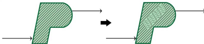
Figure 110 – Practice modification
