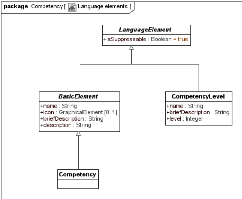
Figure 24 – Competency::Language elements
