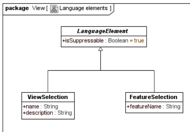
Figure 27 – View::Language elements
