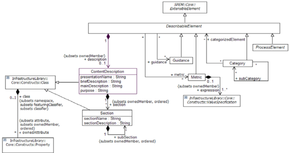
Figure 128 – SPEM Describable Element parts and subclasses
