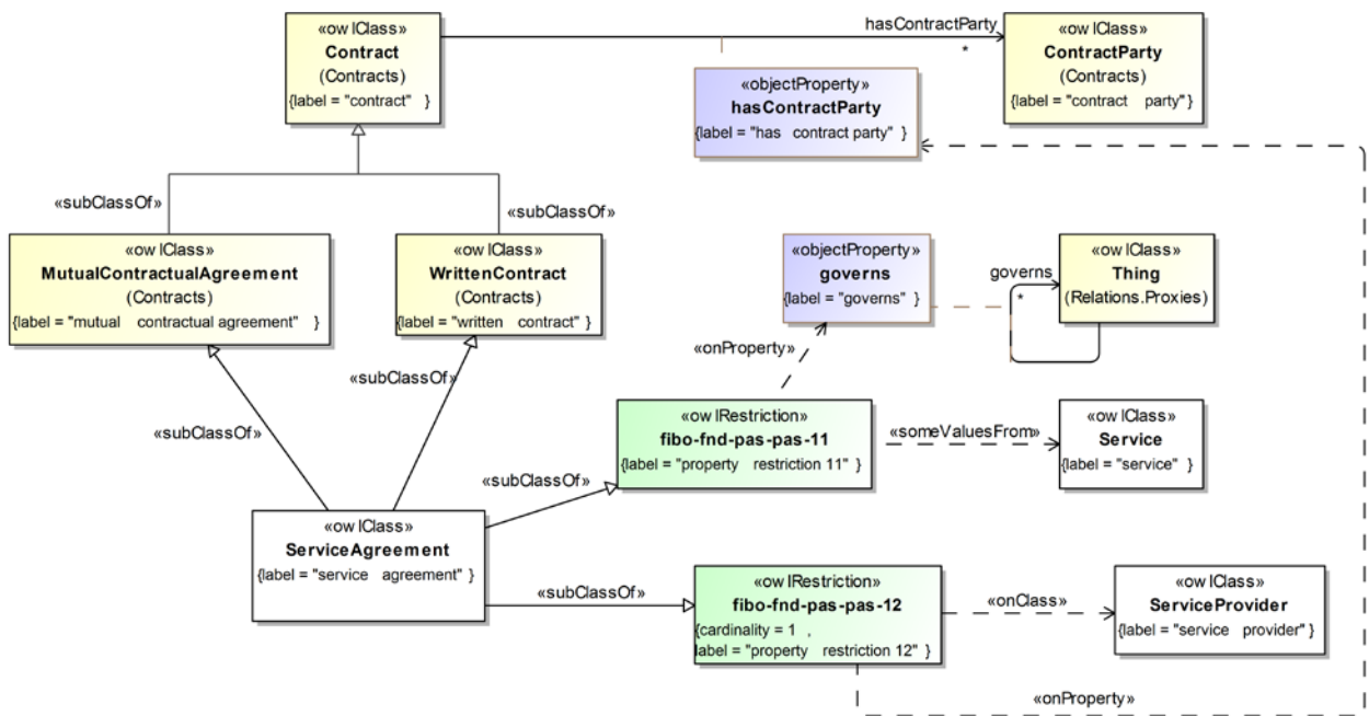
Figure 10.99 Definition of Service Agreement
