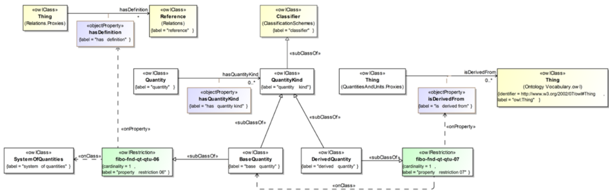
Figure 10.92 Definitions for Quantity Kinds
