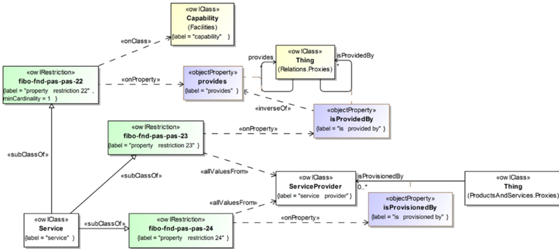
Figure 10.103 Definition of Service
