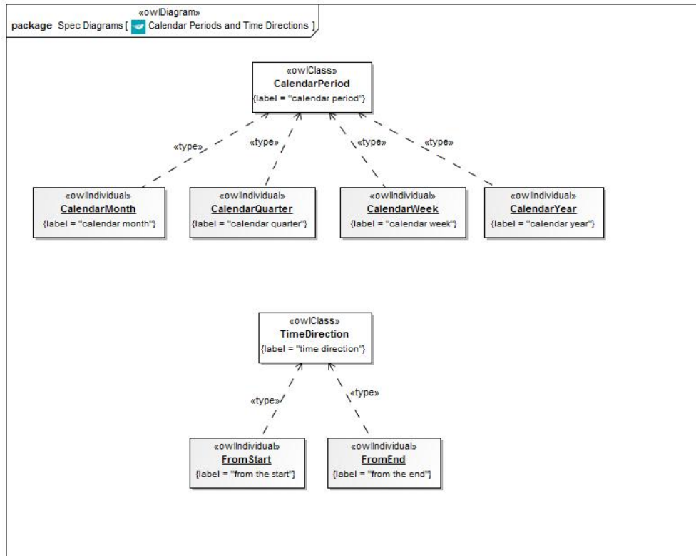
Figure 110.76 Calendar Periods and Time Directions
