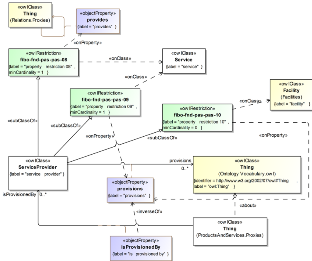
Figure 10.98 Definition of Service Provider
