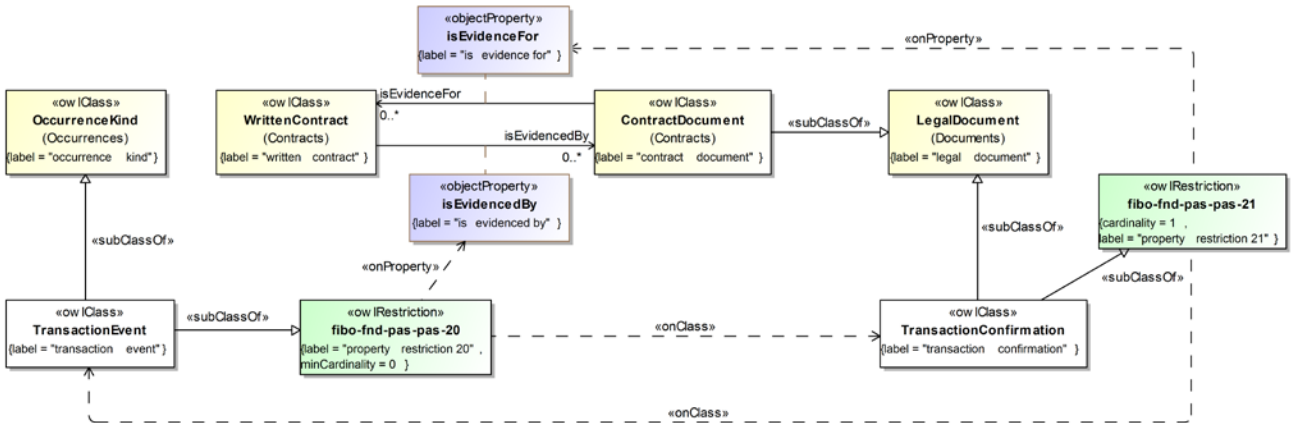
Figure 10.102 Transaction Events and Confirmations
