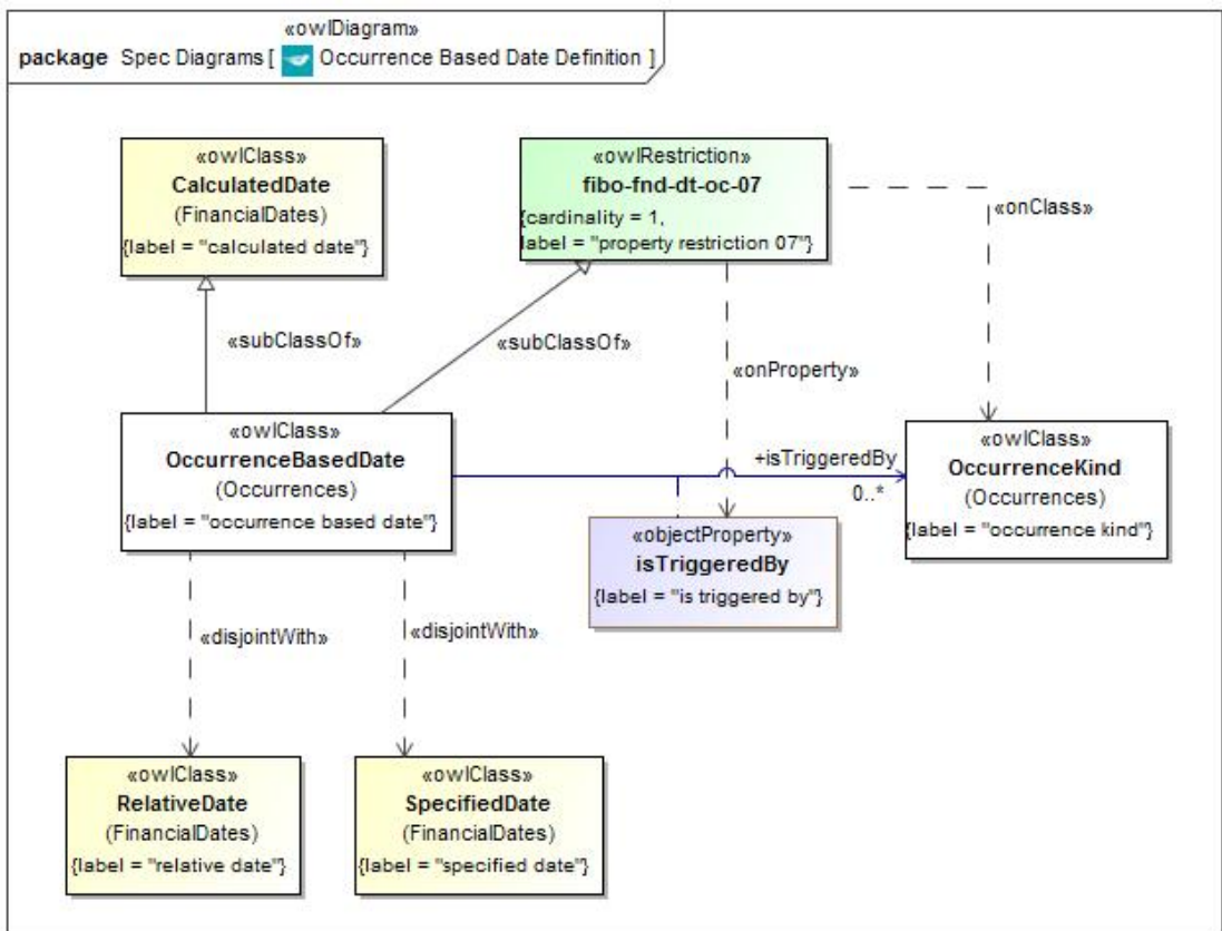
Figure 210.86 Occurrence Based Date Definition
