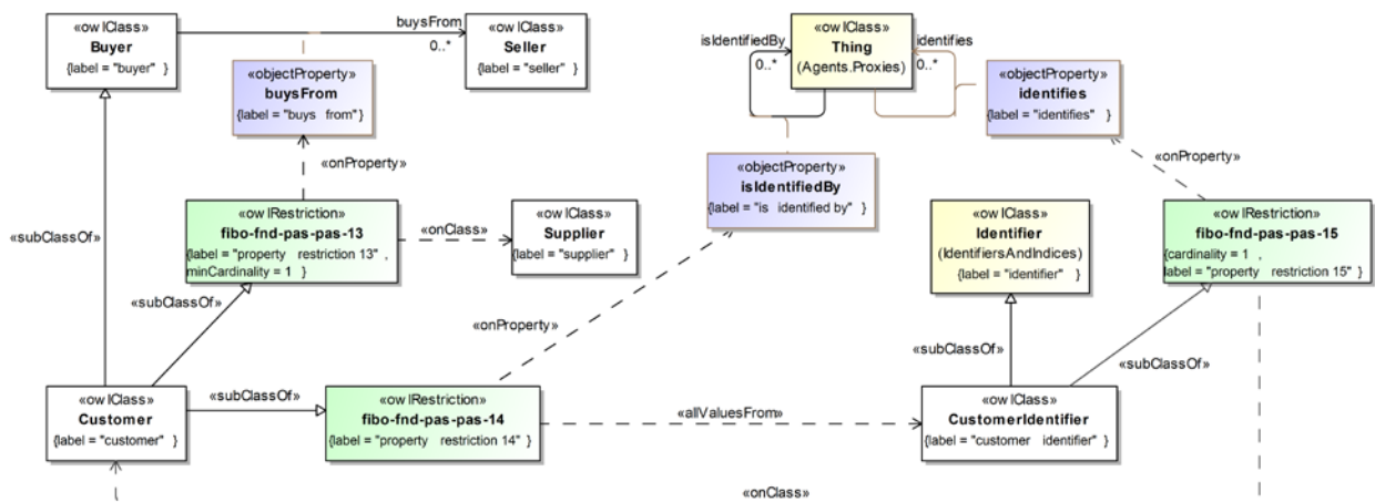
Figure 10.100 Definition of Customer
