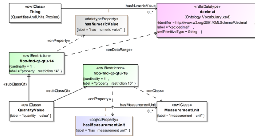
Figure 10.94 Definitions for Quantity Values
