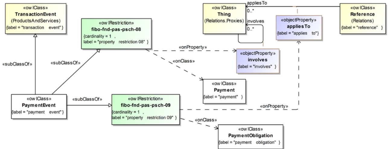
Figure 10.108 Definition of Payment Event
