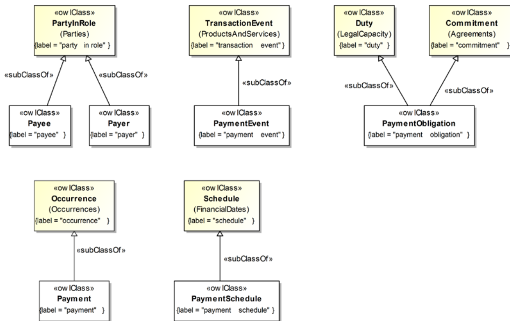
Figure 10.104 Payments and Schedules Class Hierarchy
