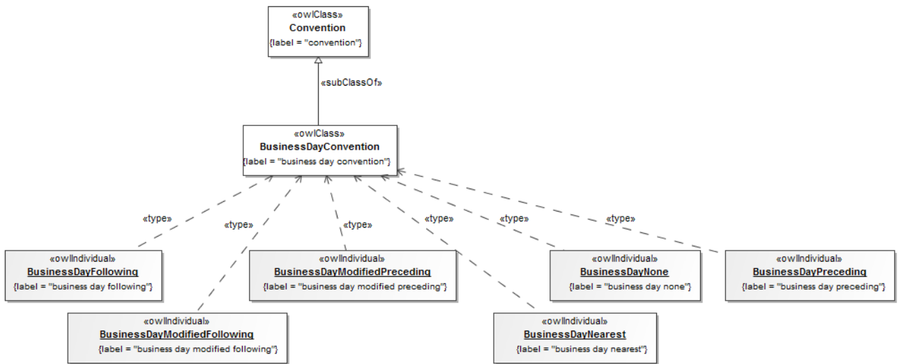
Figure 240.89 Business Day Conventions
