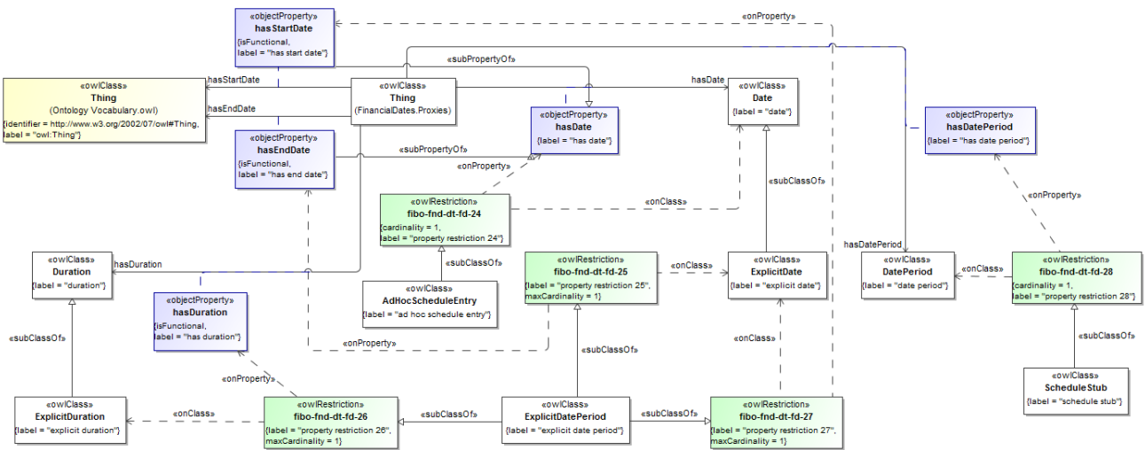
Figure 170.82 Explicit Dates, Periods, and Durations
