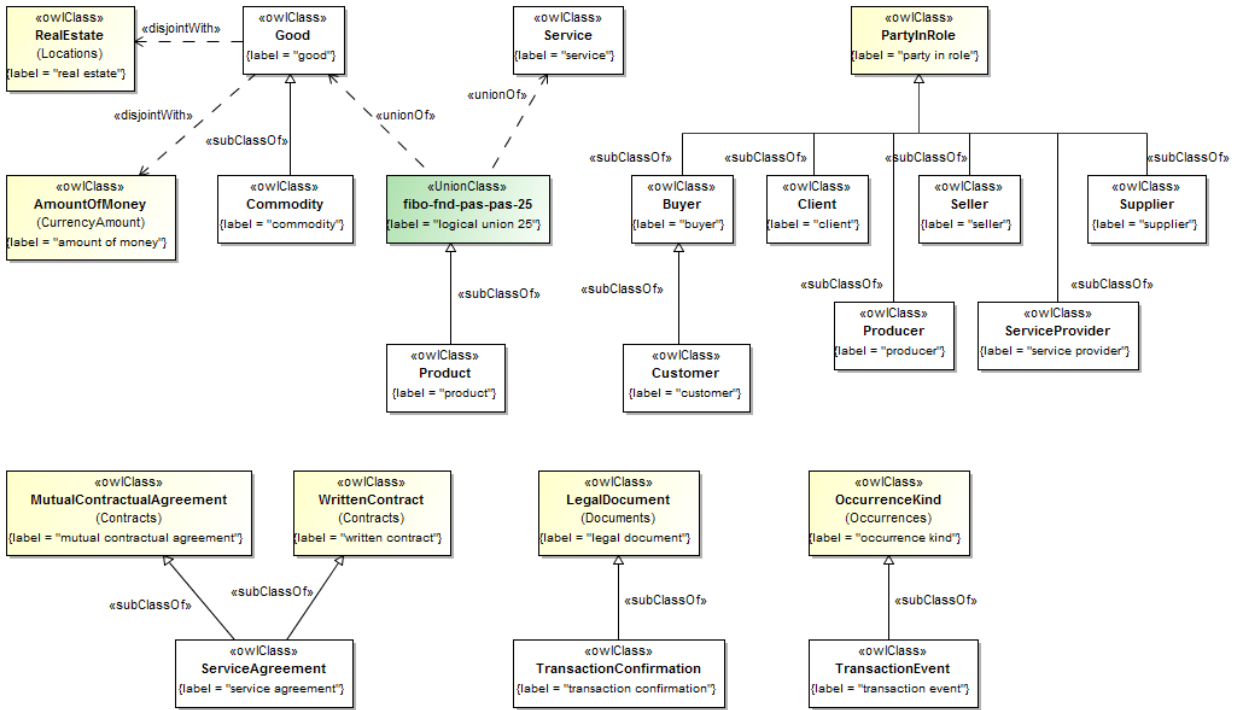
Figure 10.95 Products and Services Class Hierarchy
