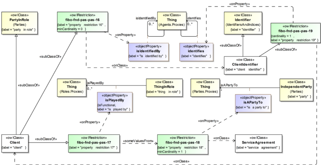
Figure 10.101 Definition of Client
