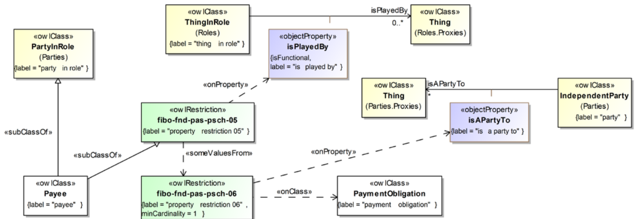
Figure 10.106 Definition of Payee
