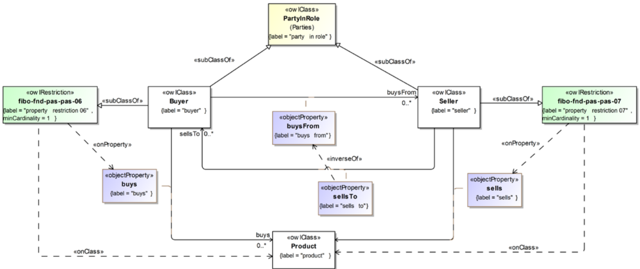
Figure 10.97 Definitions of Buyer and Seller
