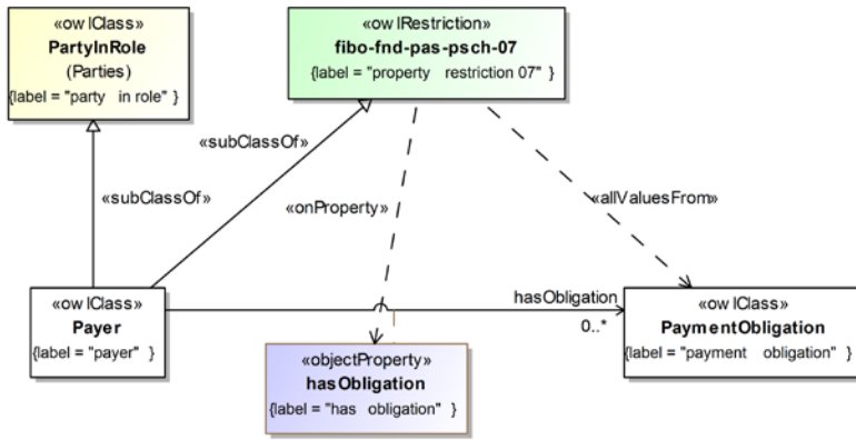
Figure 10.107 Definition of Payer
