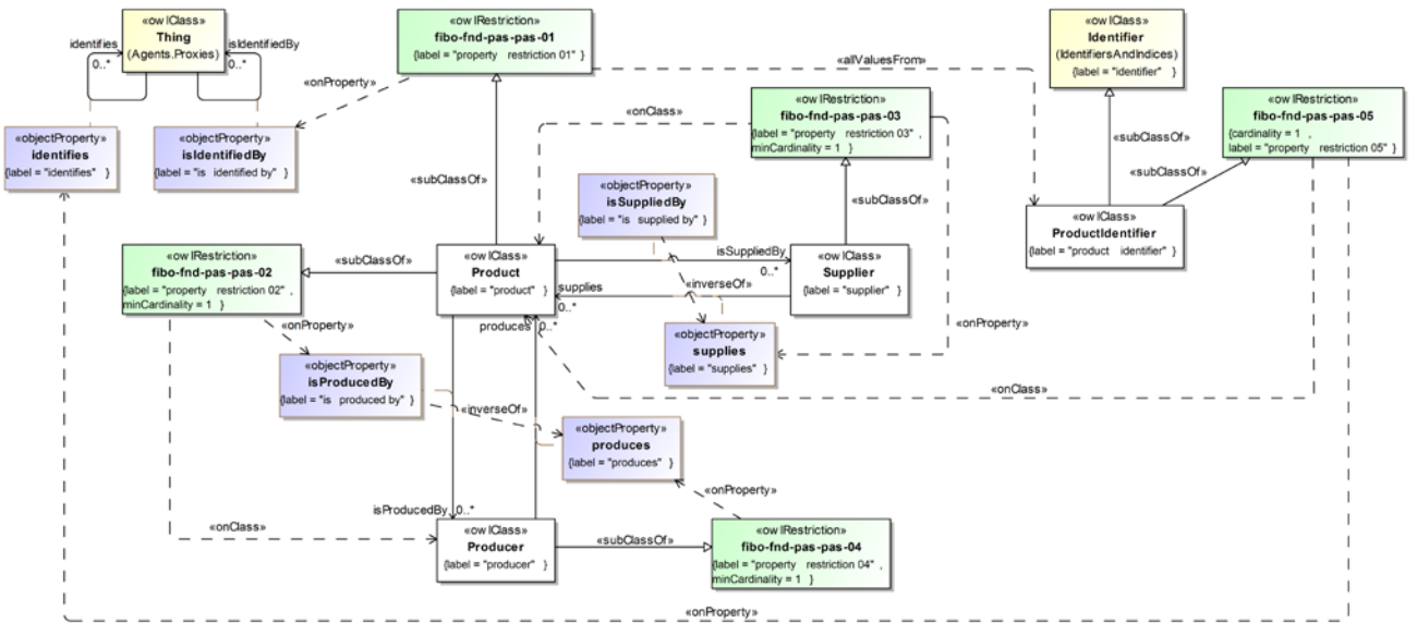
Figure 10.96 Definition of Product – Producers and Suppliers
