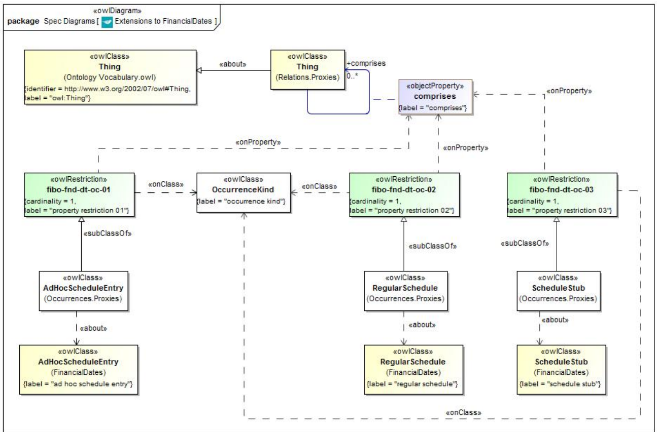
Figure 200.85 Extensions to FinancialDates
