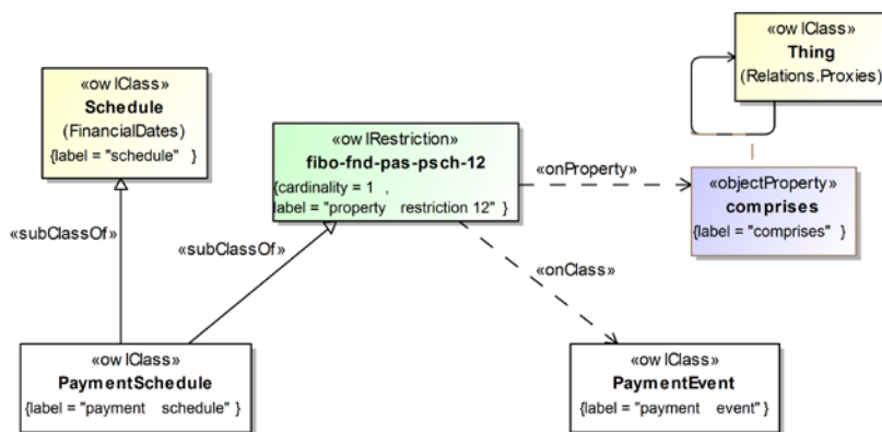
Figure 10.110 Definition of Payment Schedule
