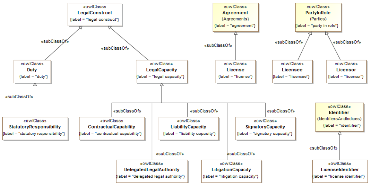
Figure 10.57 - Legal Capacity Class Hierarchy
