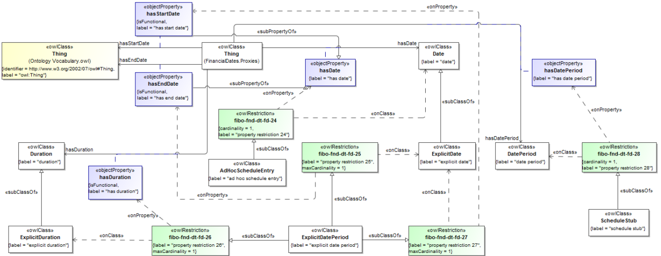
Figure 170.82 - Explicit Dates, Periods, and Durations
