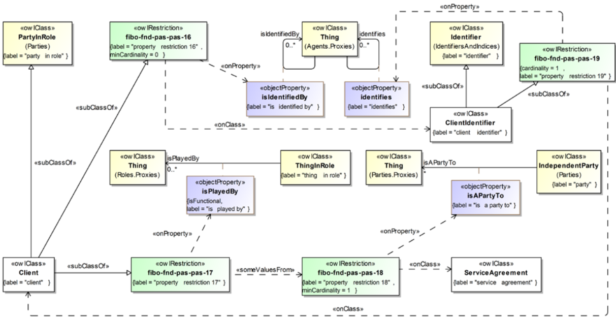
Figure 10.102 - Definition of Client
