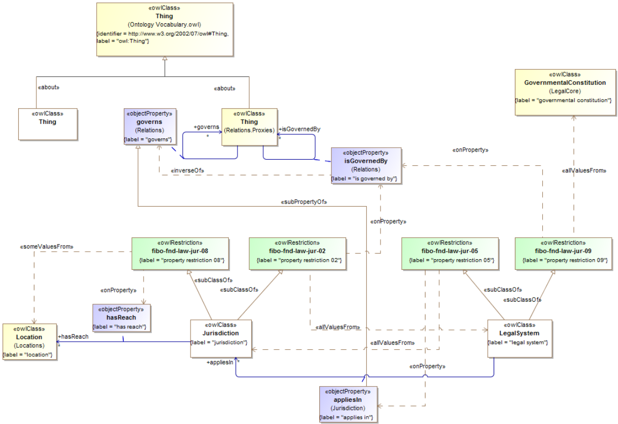
Figure 10.53 - Jurisdiction Basic Concepts
