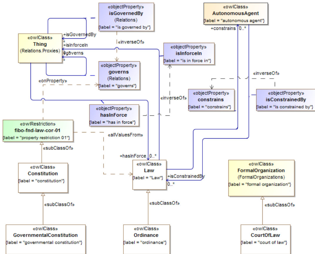
Figure 10.52 - Legal Core Concepts
