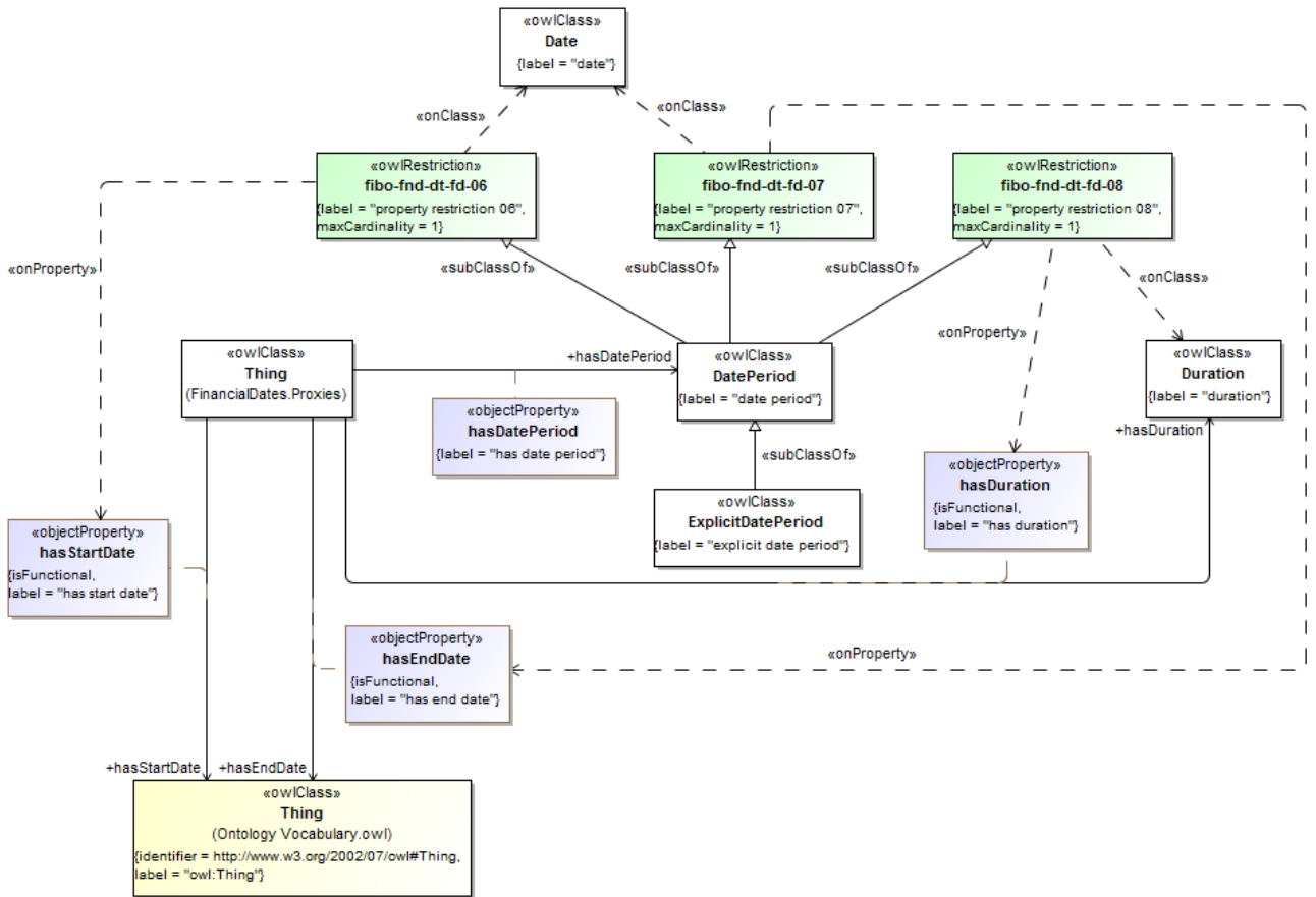
Figure 160.81 - Date Period Definitions
