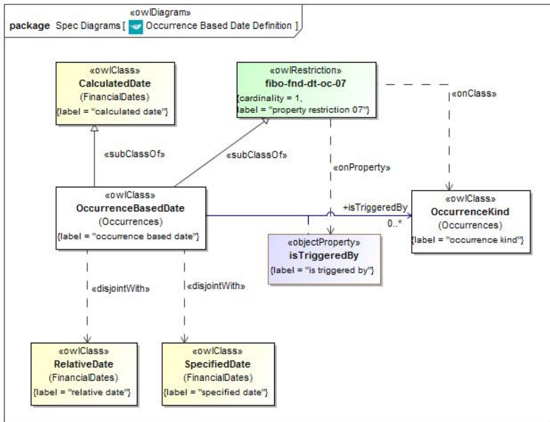
Figure 210.86 - Occurrence Based Date Definition
