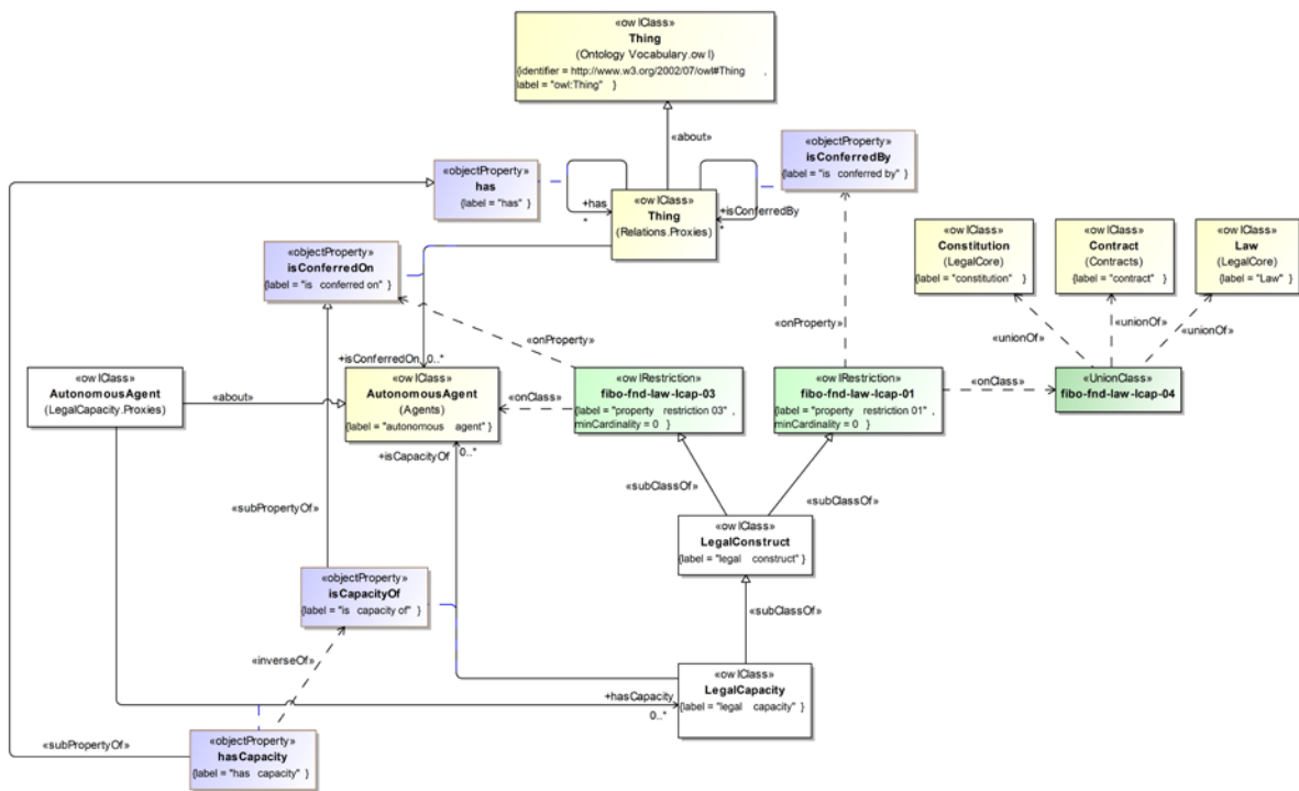
Figure 10.58 - Definition of Legal Capacity
