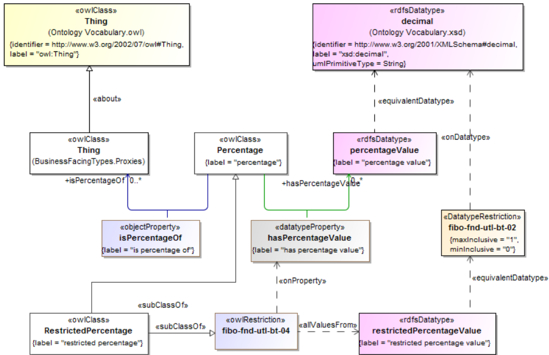
Figure 10.6 - Percentage Definitions
