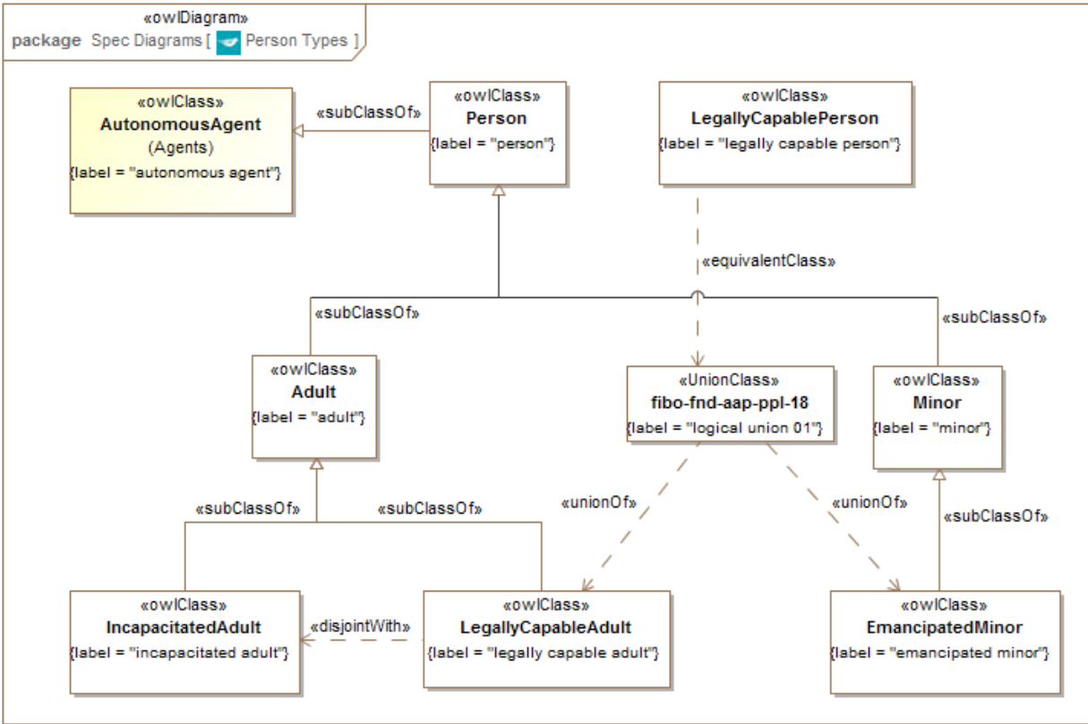
Figure 10.32 - Person Types
