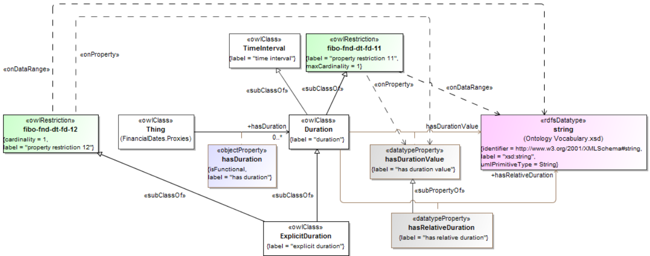
Figure 180.83 - Duration Definitions
