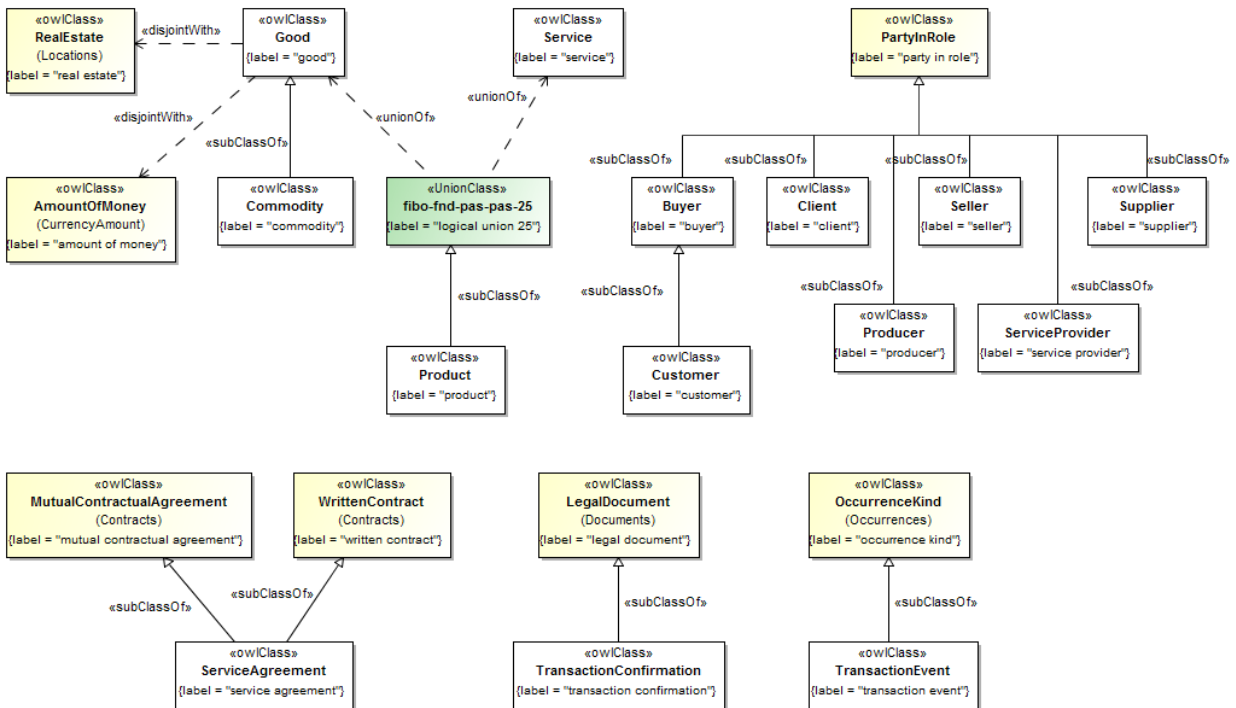
Figure 10.96 - Products and Services Class Hierarchy
