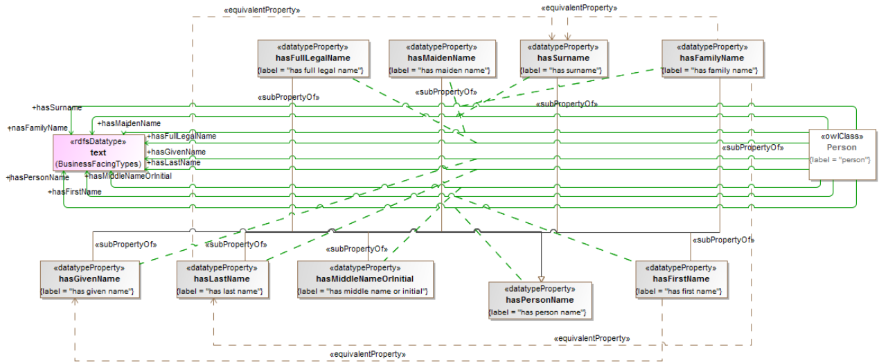
Figure 10.33 - People Names
