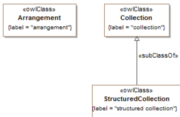
Figure 10.24 - Arrangements Concepts
