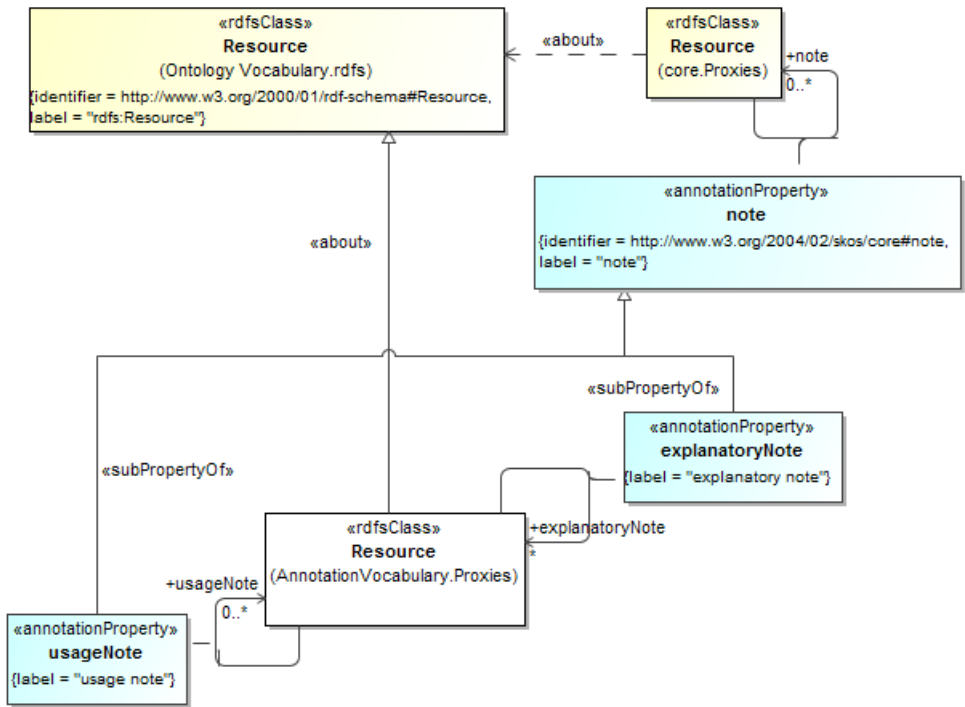
Figure 10.2 - Explanatory Annotations
