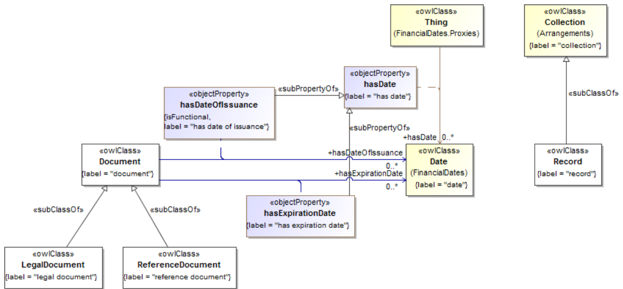
Figure 40.29 - Documents Concepts
