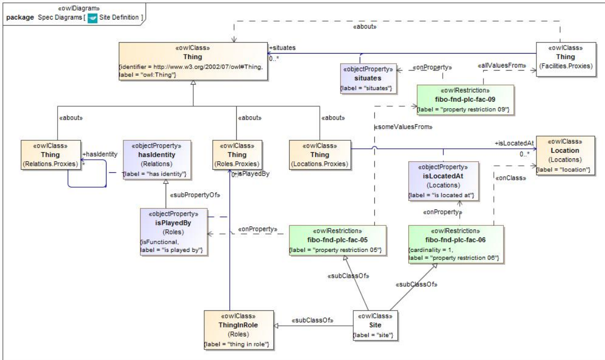
Figure 60.40 - Site Definition
