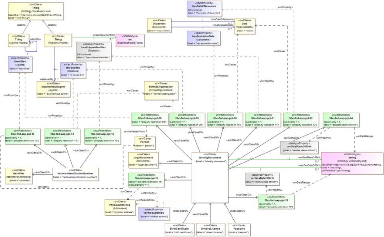
Figure 10.35 - Identification Documents
