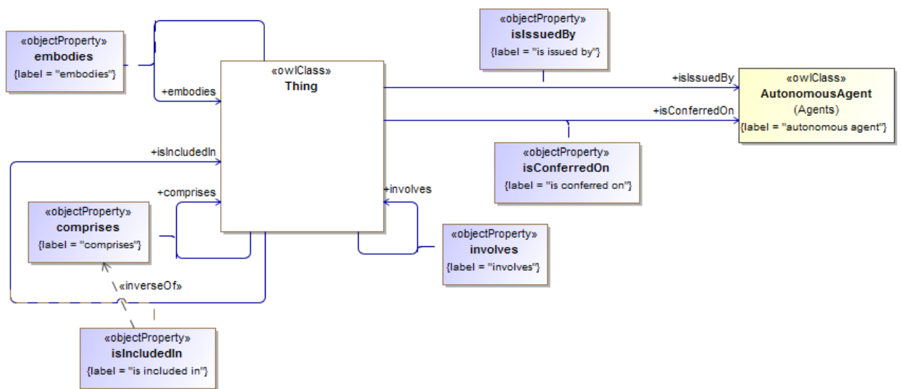
Figure 10.12 - Singular Relations
