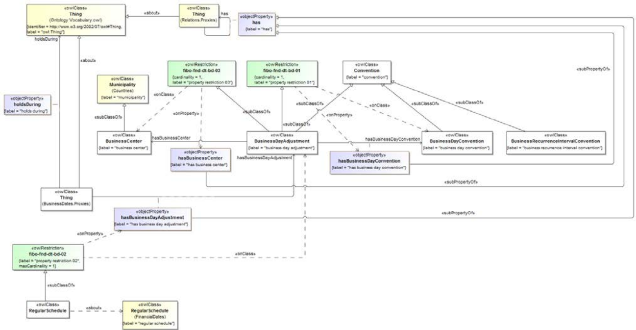
Figure 220.87 - Business Conventions
