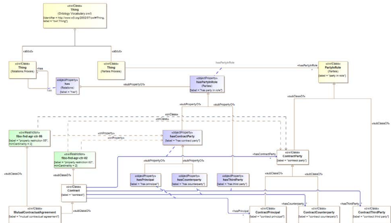
Figure 10.48 - Contract Parties
