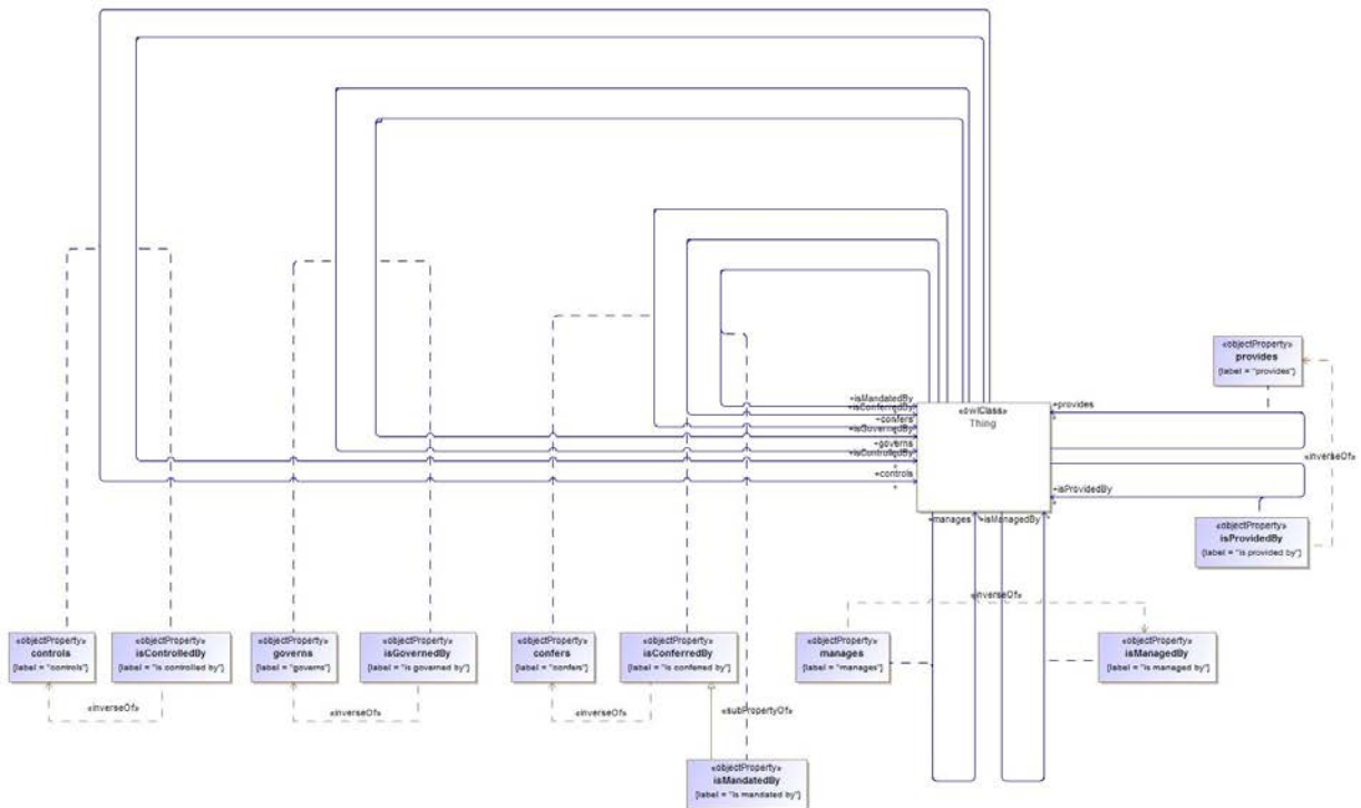
Figure 10.14 - Construct Relations
