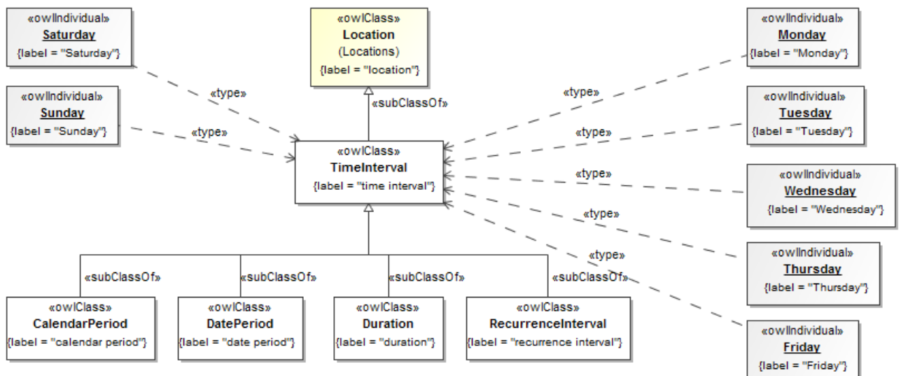
Figure 100.75 - Time Intervals
