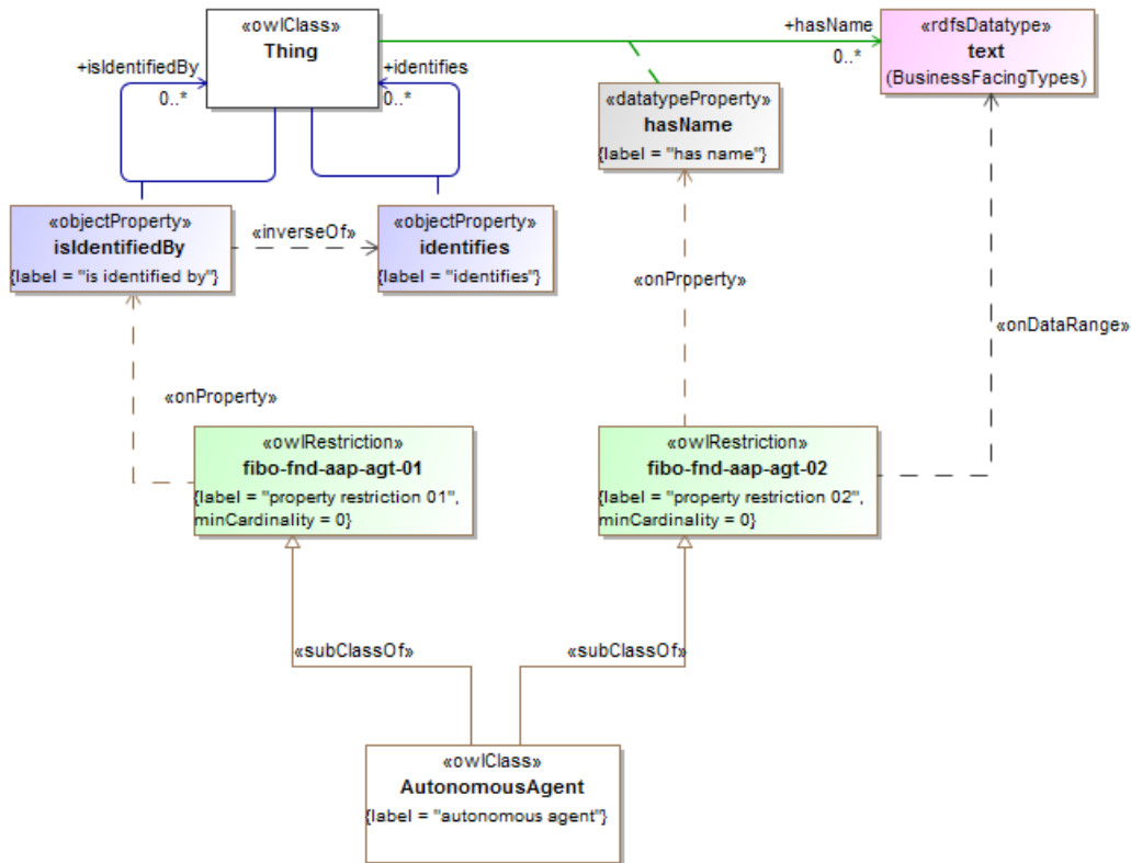
Figure 10.30 - Agents Concepts
