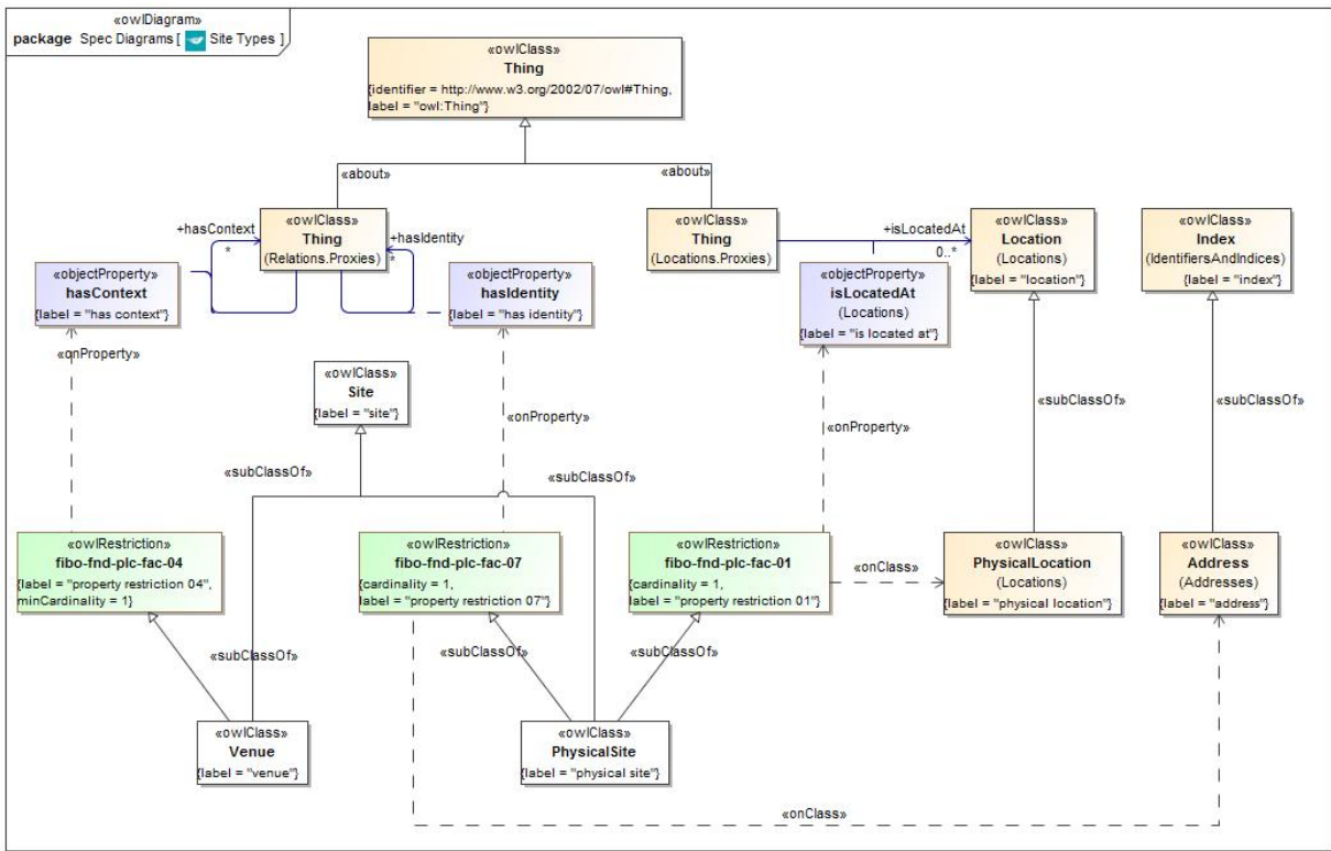
Figure 50.39 - Site Types
