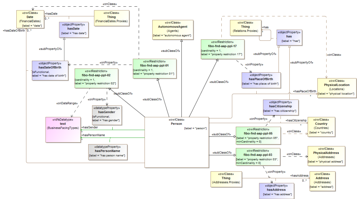
Figure 10.31 - Person Fundamentals
