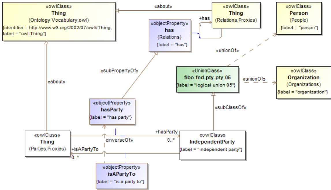
Figure 10.20 - Independent Parties
