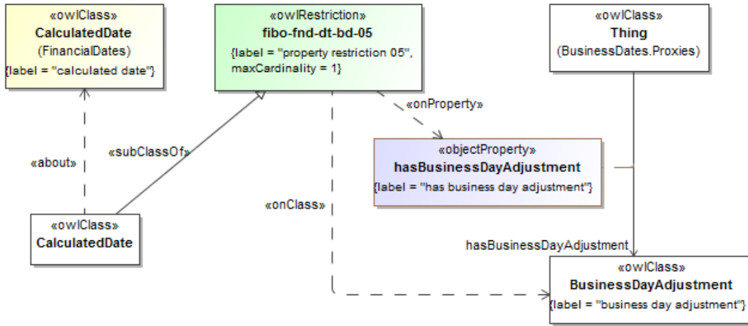
Figure 250.90 - Calculated Dates
