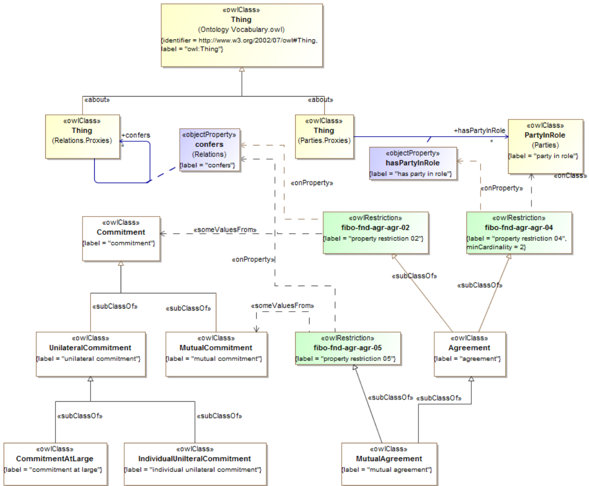
Figure 10.46 - Agreements Concepts
