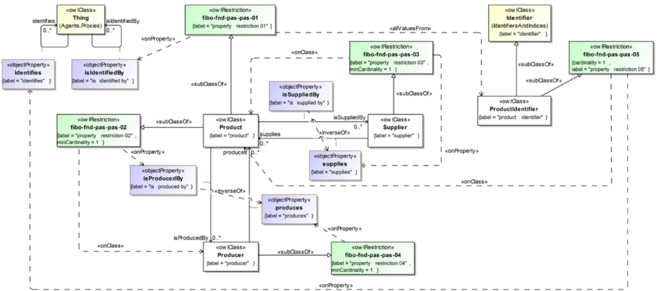
Figure 10.97 - Definition of Product – Producers and Suppliers
