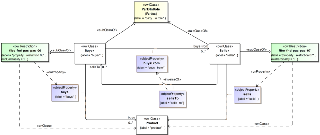
Figure 10.98 - Definitions of Buyer and Seller
