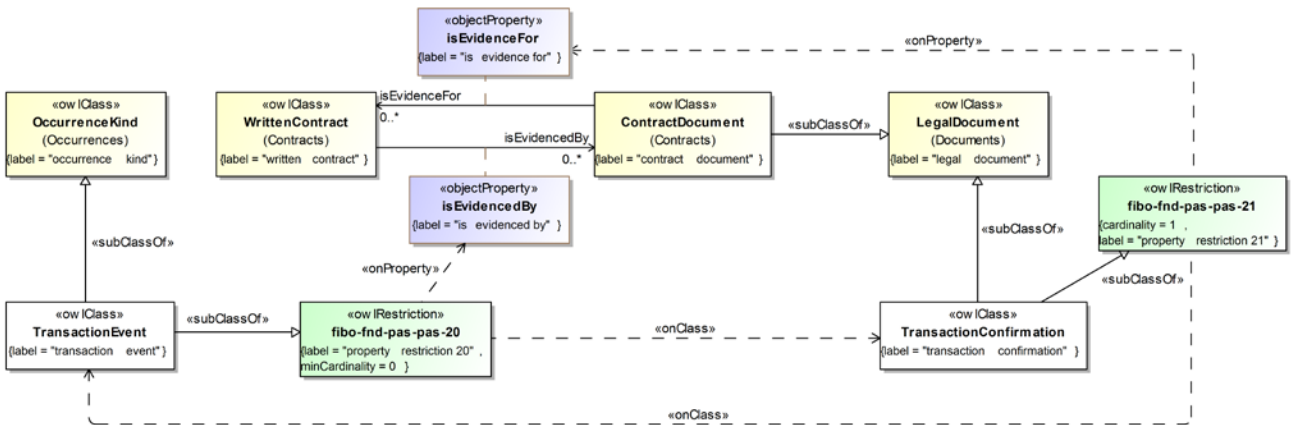
Figure 10.103 - Transaction Events and Confirmations
