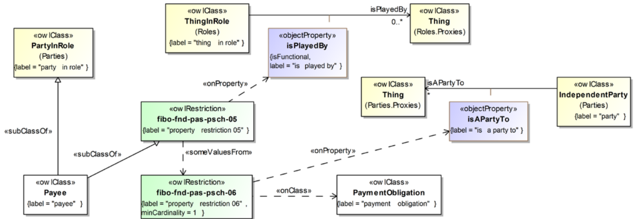
Figure 10.107 - Definition of Payee
