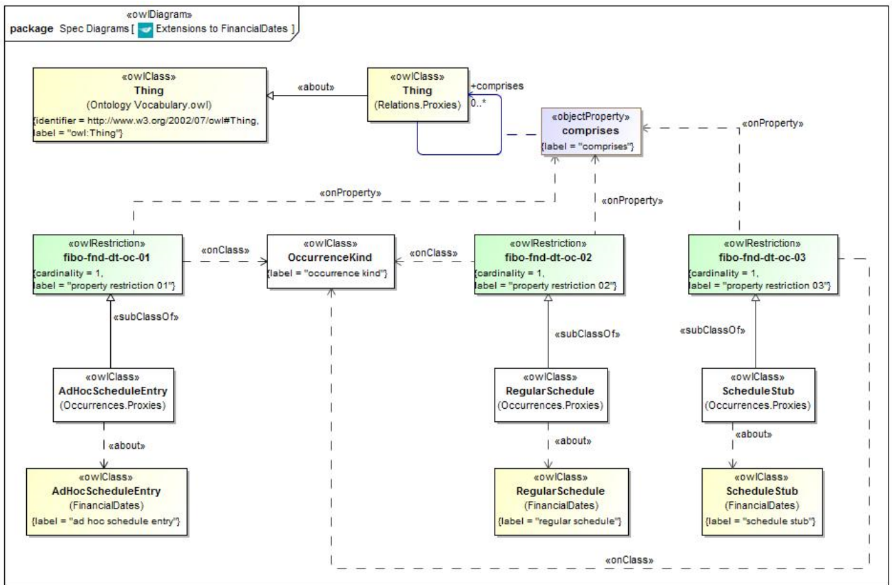
Figure 200.85 - Extensions to FinancialDates
