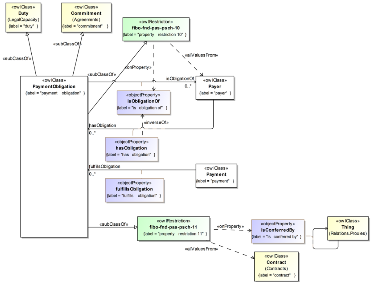
Figure 10.110 Definition of Payment Obligation
