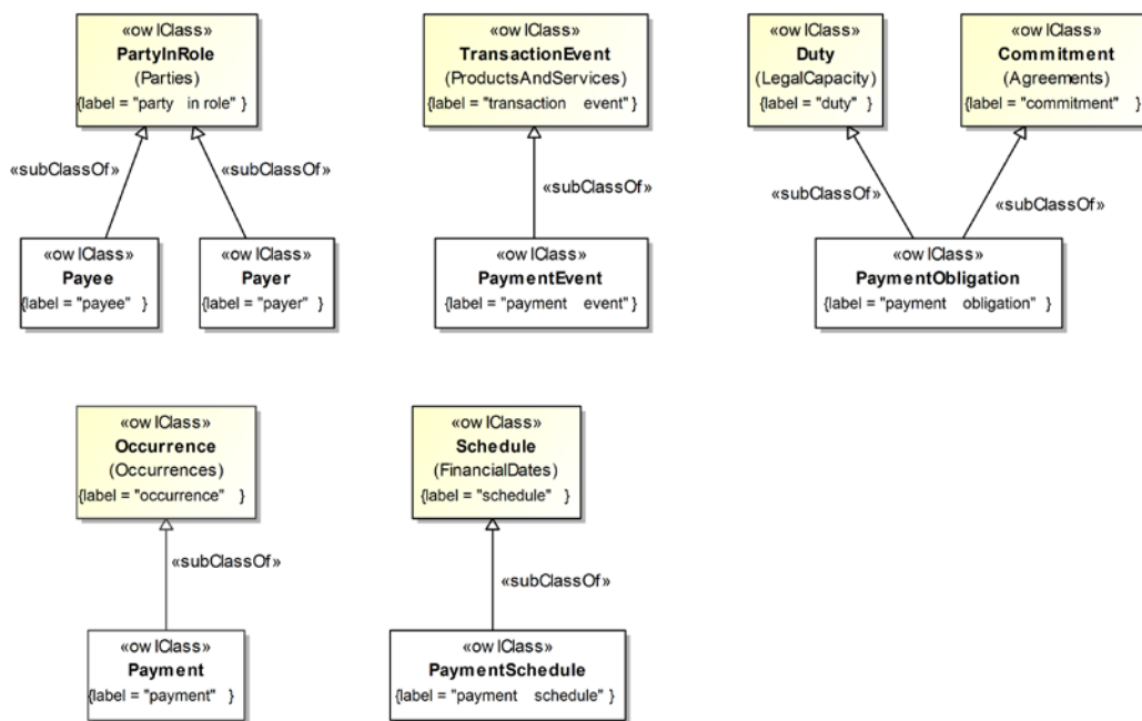
Figure 10.105 - Payments and Schedules Class Hierarchy
