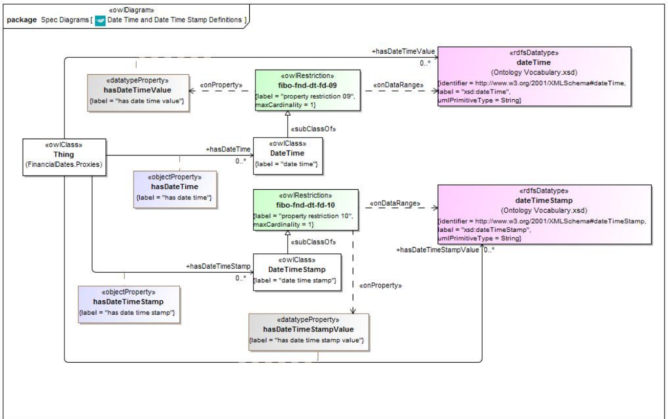
Figure 140.79 - Date Time and Date Time Stamp Definitions
