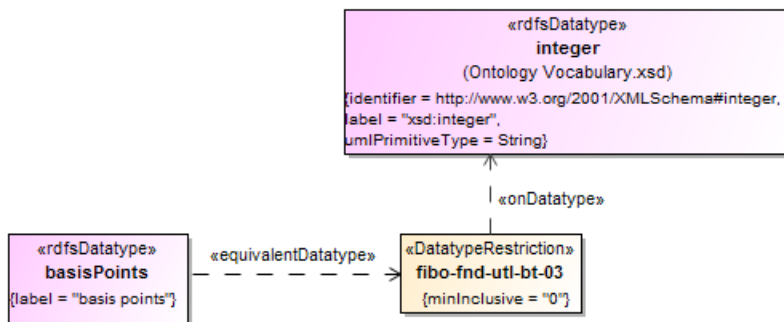
Figure 10.7 - Basis Points Definition
