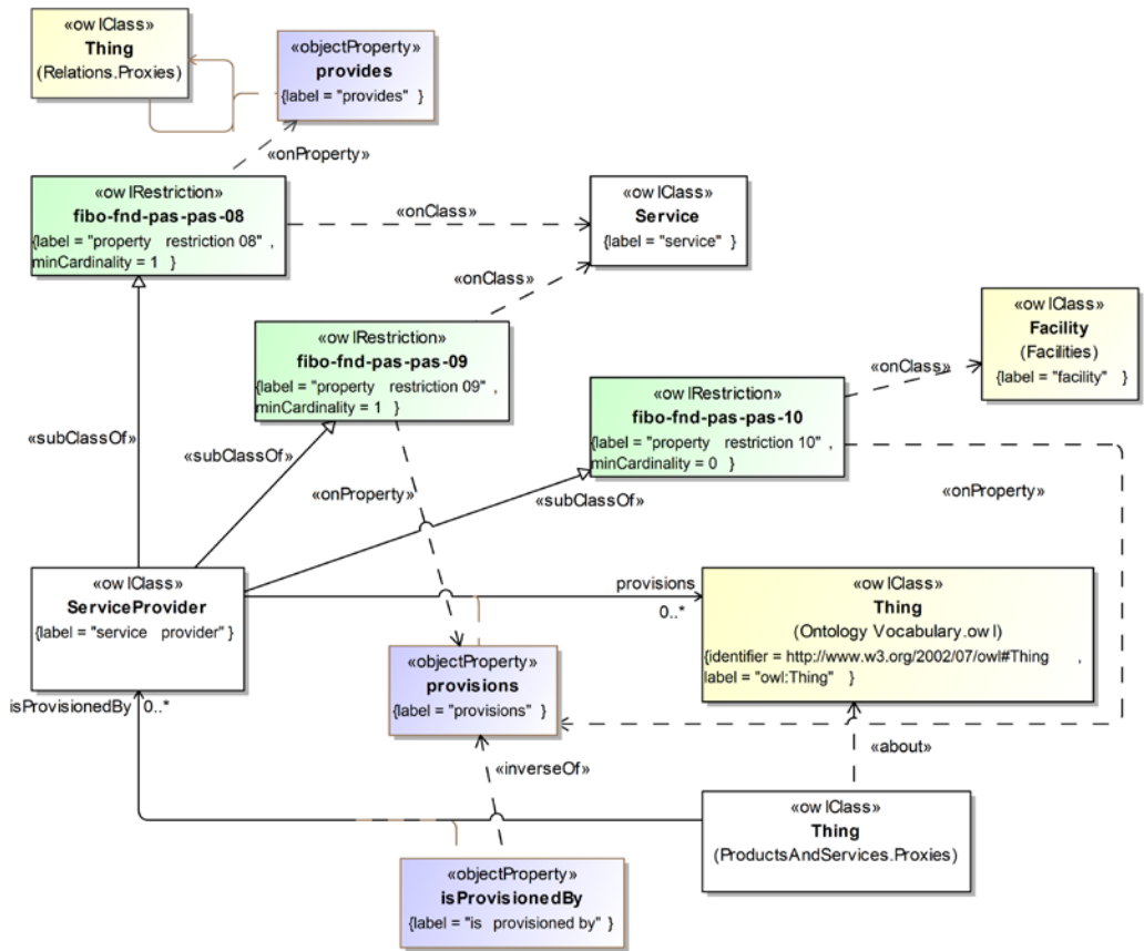
Figure 10.99 - Definition of Service Provider
