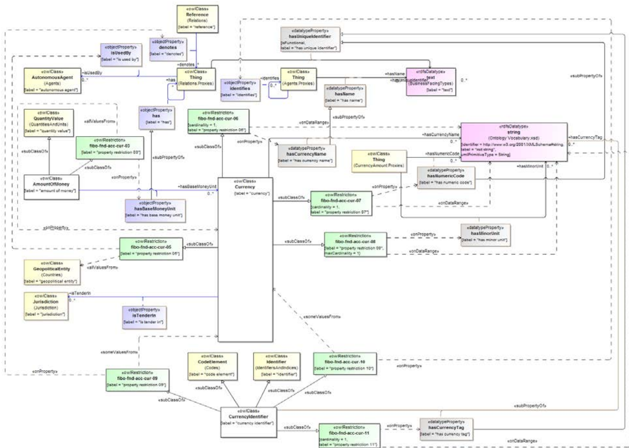
Figure 10.70 - Definitions for Currency and Currency Identifiers
