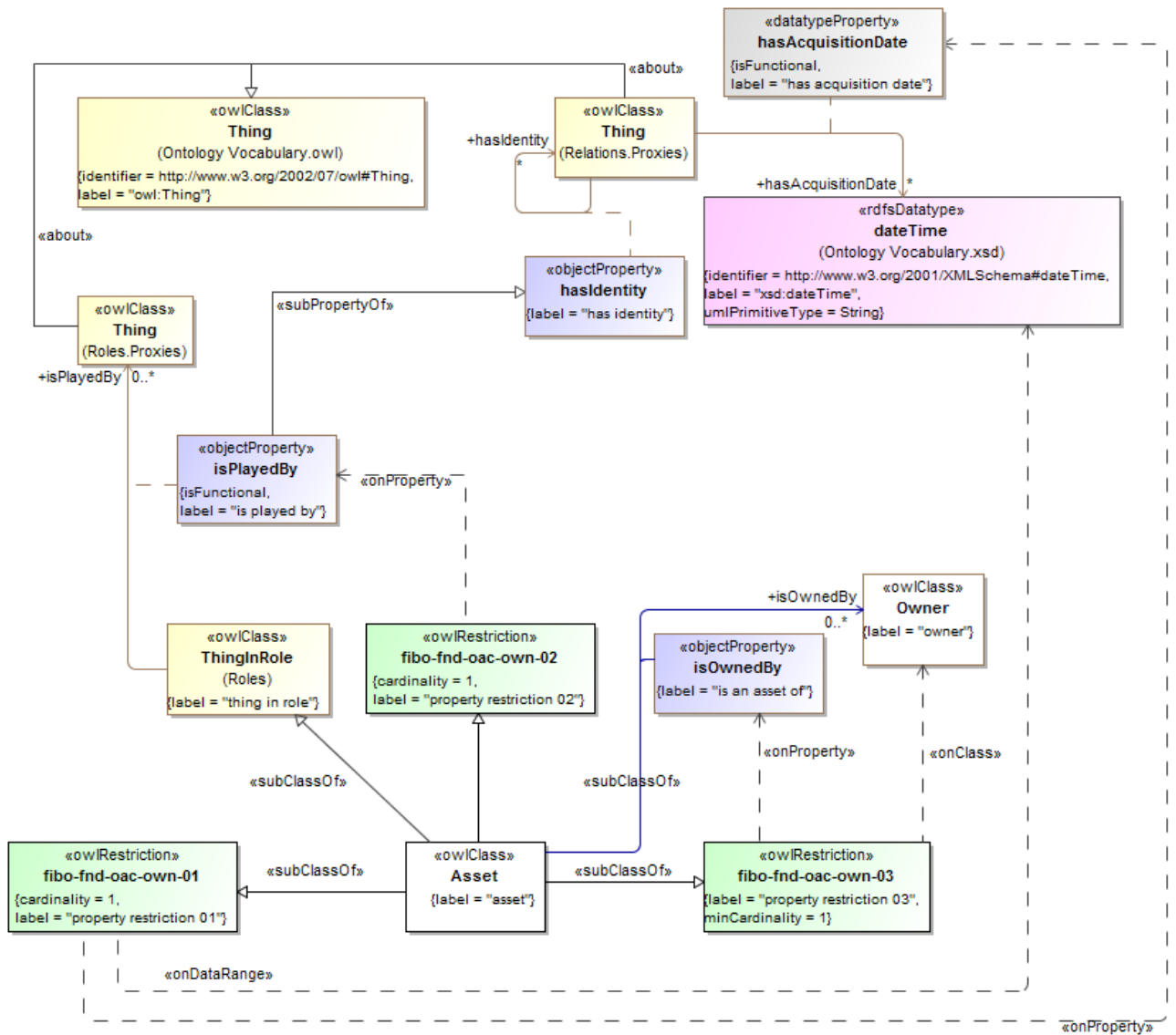
Figure 10.65 - Asset Definition
