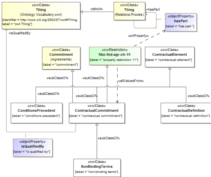
Figure 10.50 - Contractual Commitments
