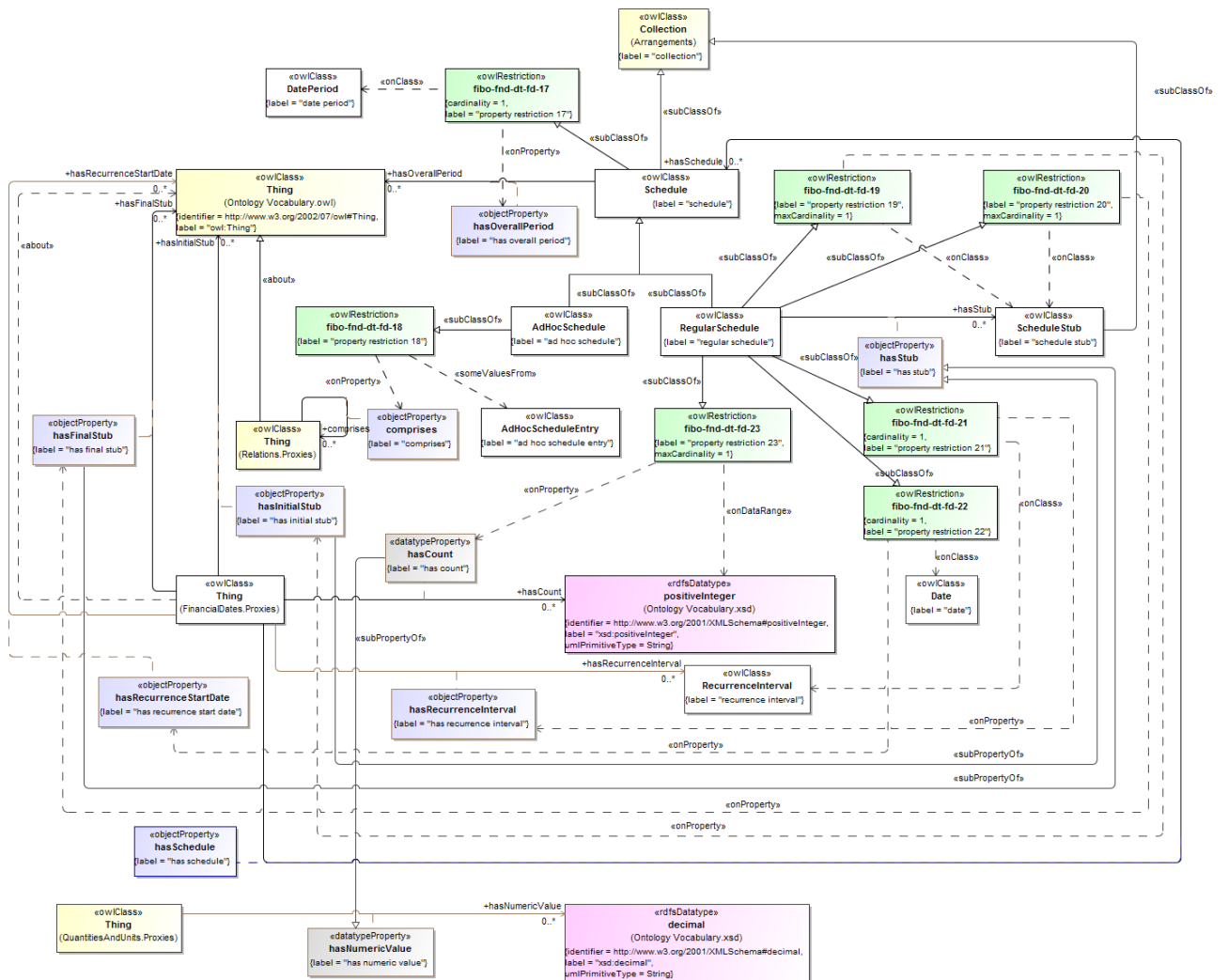
Figure 150.80 - Schedule Definitions
