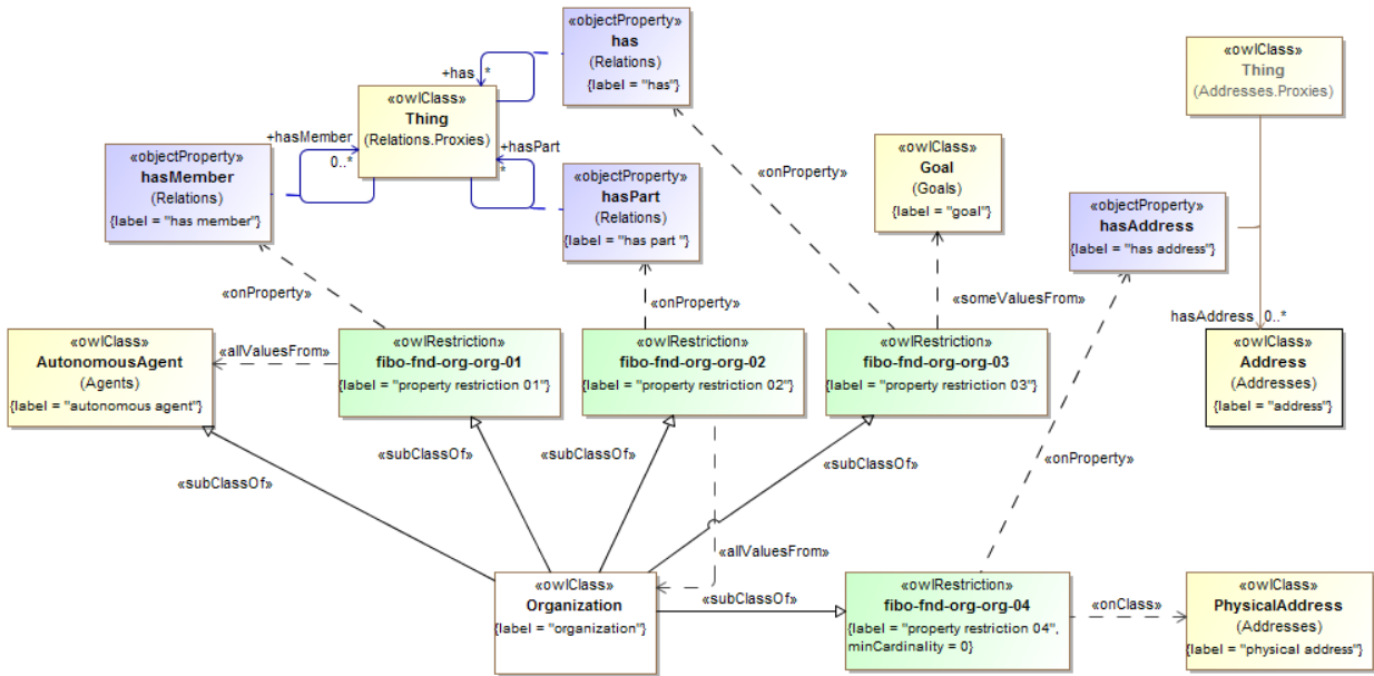
Figure 10.43 - Organizations Concepts
