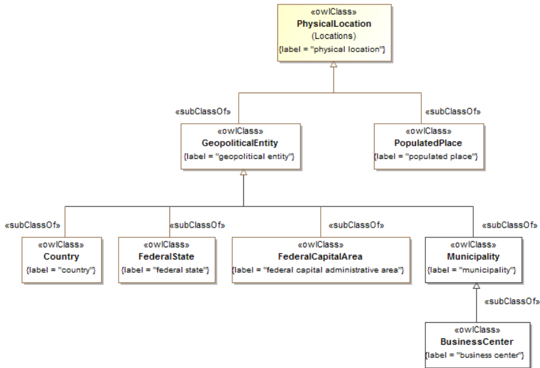
Figure 10.37 - Countries Concepts
