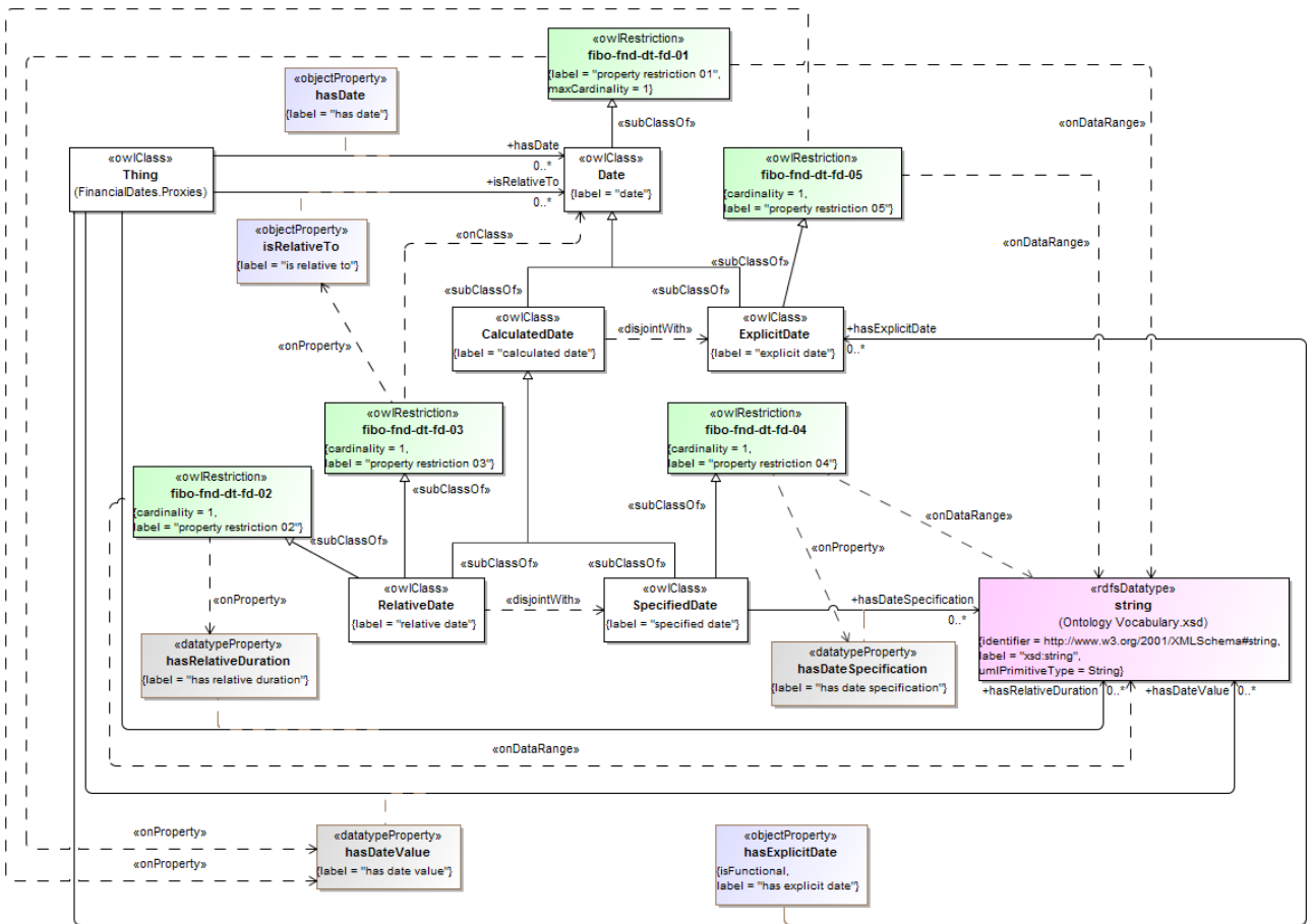
Figure 120.77 - Date Definitions
