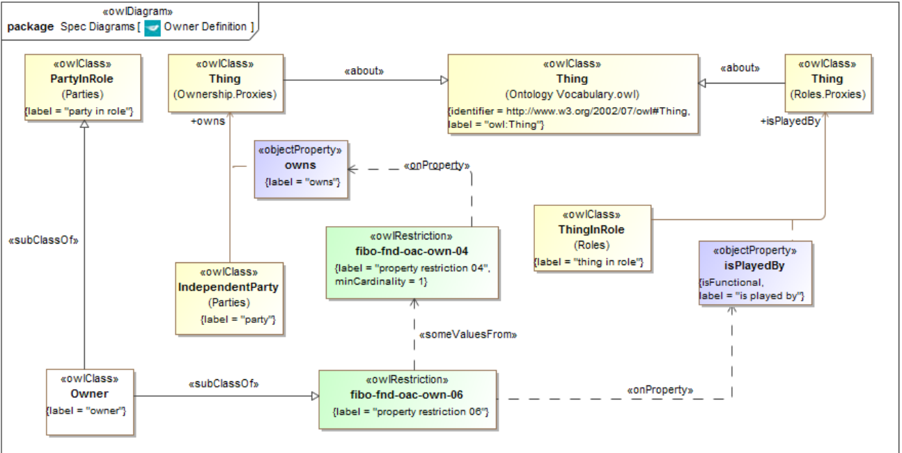
Figure 10.64 - Owner Definition
