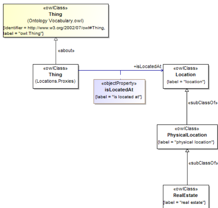
Figure 10.36 - Locations Concepts
