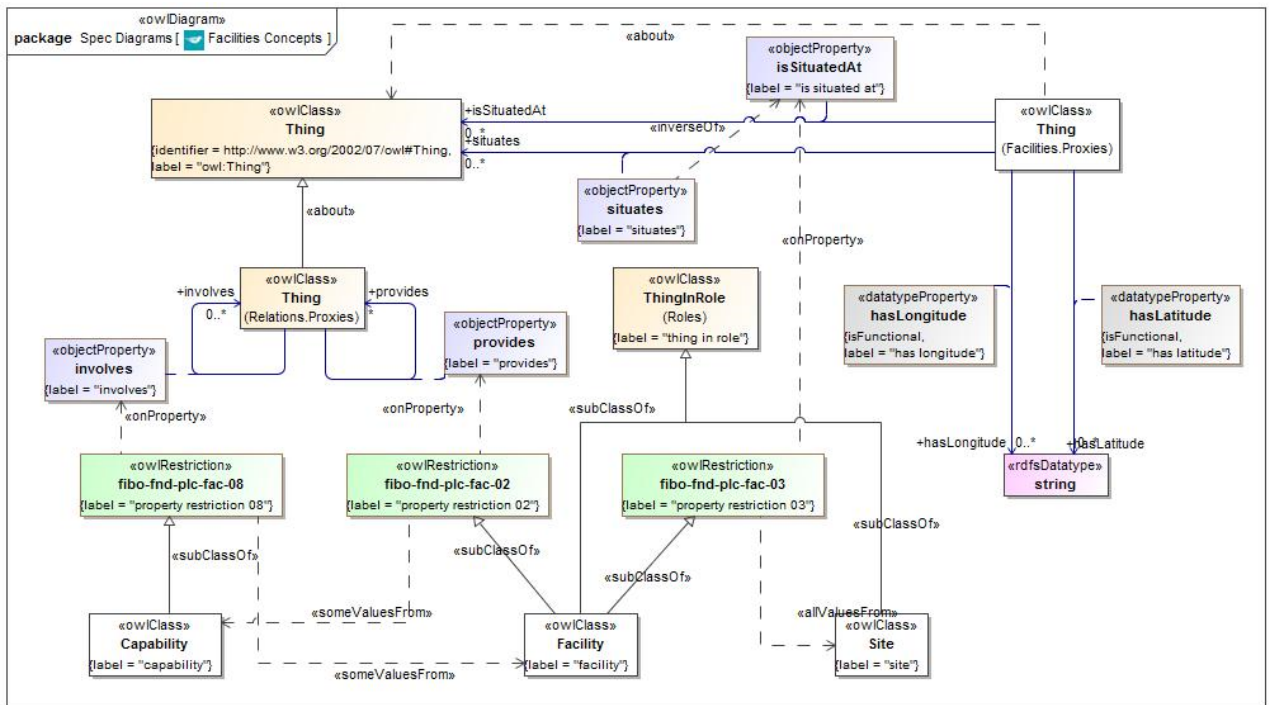
Figure 70.41 - Facilities Concepts
