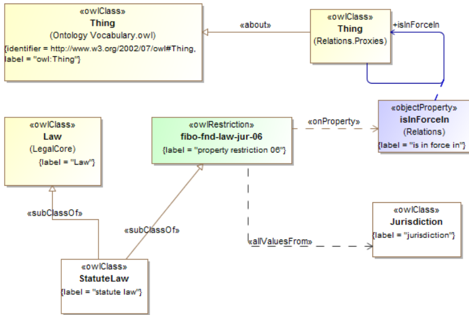
Figure 10.56 - Statute Law
