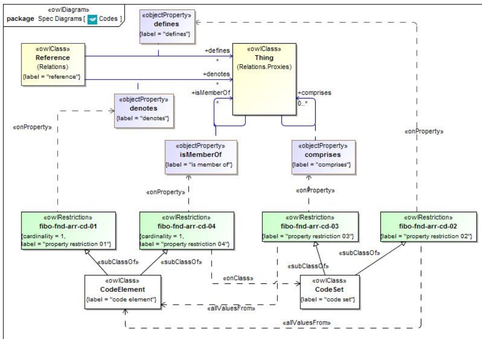
Figure 30.26 - Codes
