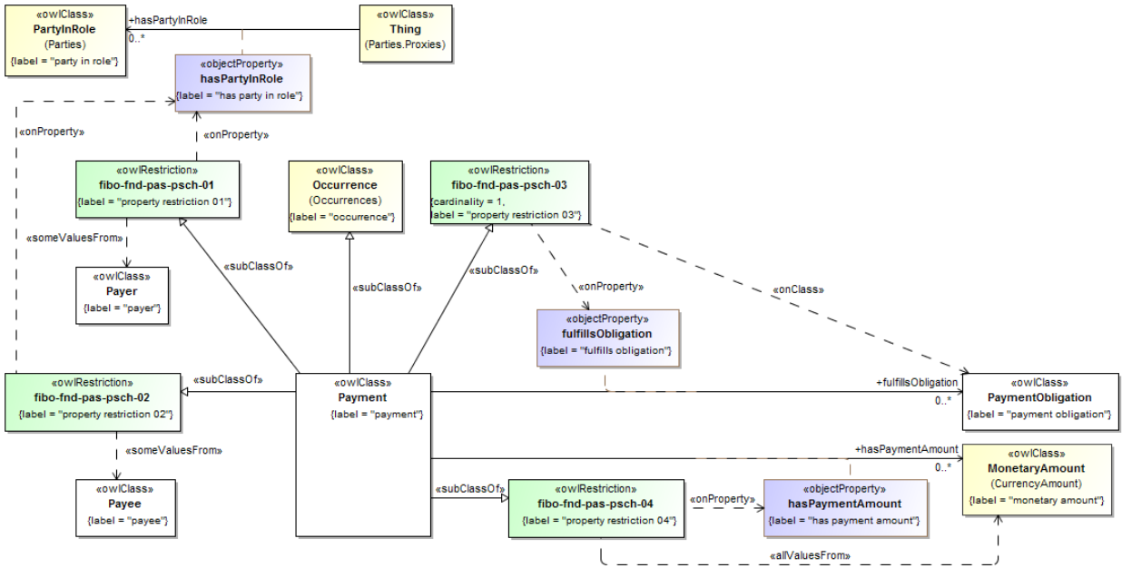
Figure 10.106 - Definition of Payment
