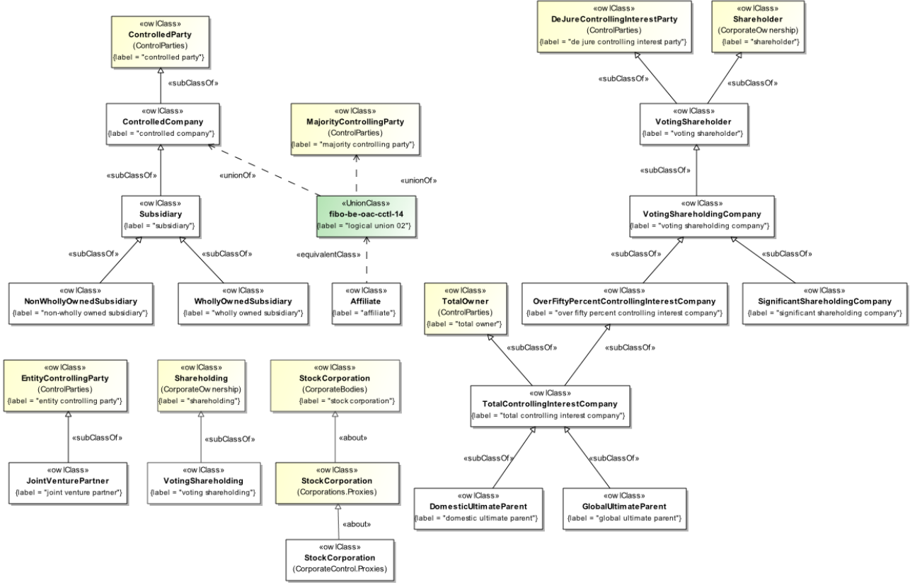
Figure 9.57 - Corporate Control Class Hierarchy
