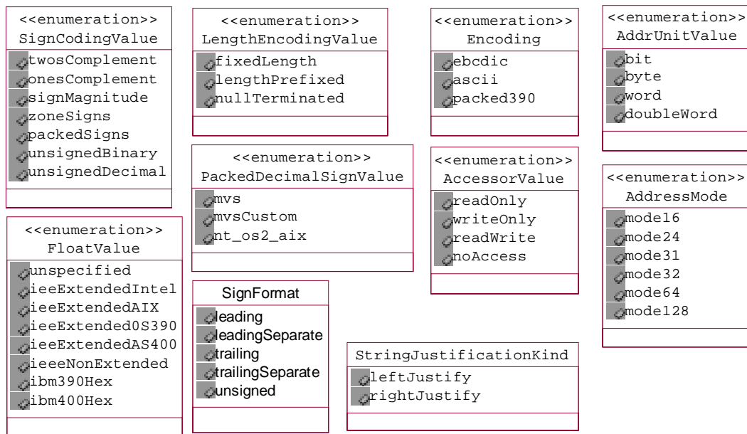
Figure 7-5 Type Descriptor Stereotypes
