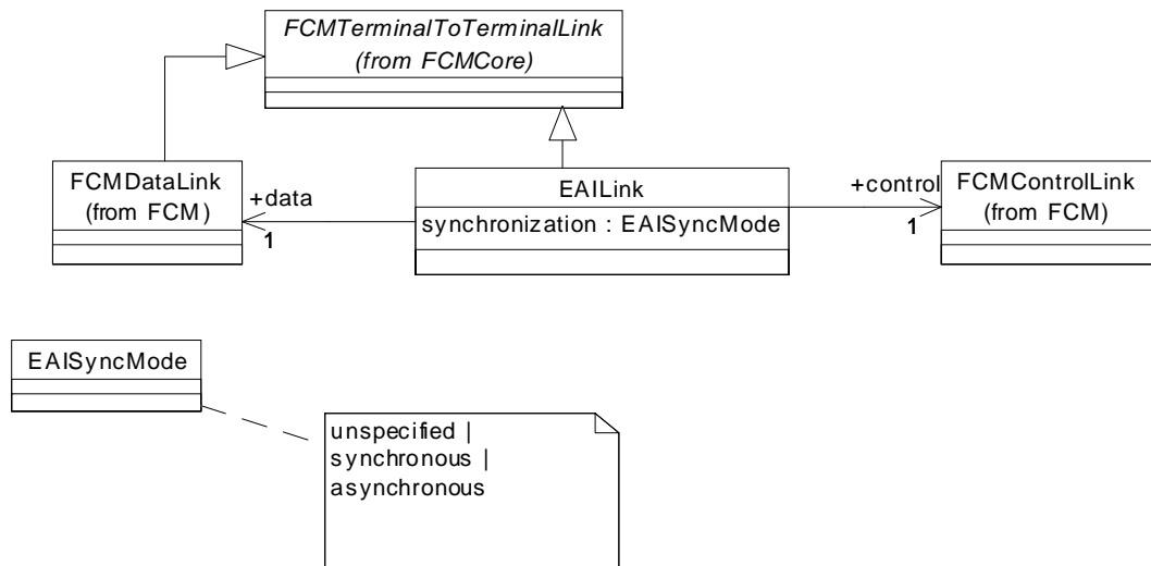
Figure 6-7 Definition of EAILink
