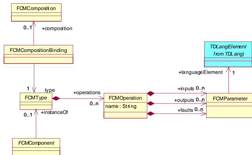
Figure 6-1 FCMComponent metamodel diagram (from ad/2001-06-09)
