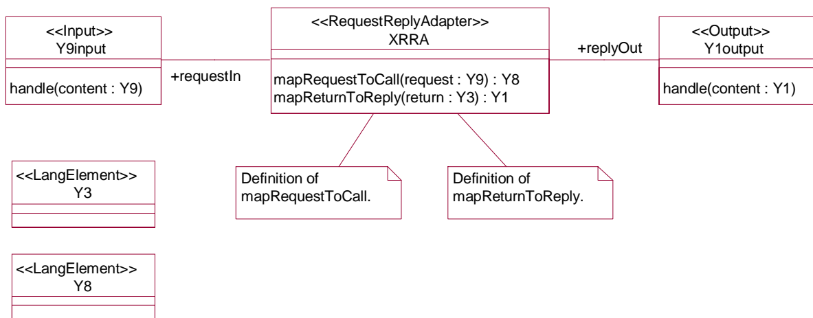
Figure 8-10 Class diagram from prototypical request/reply adapter
