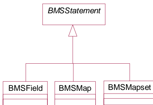
Figure A-11 CICS BMS Inheritance View
