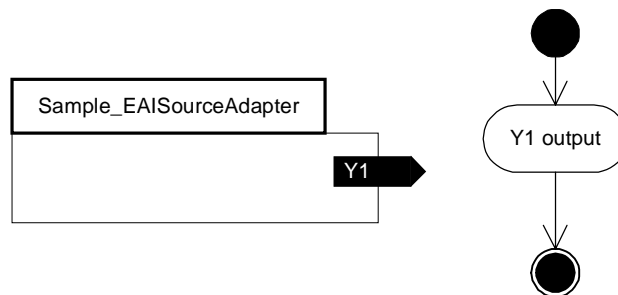
Figure 6-56 CCA notation for a sample EAISourceAdapter
