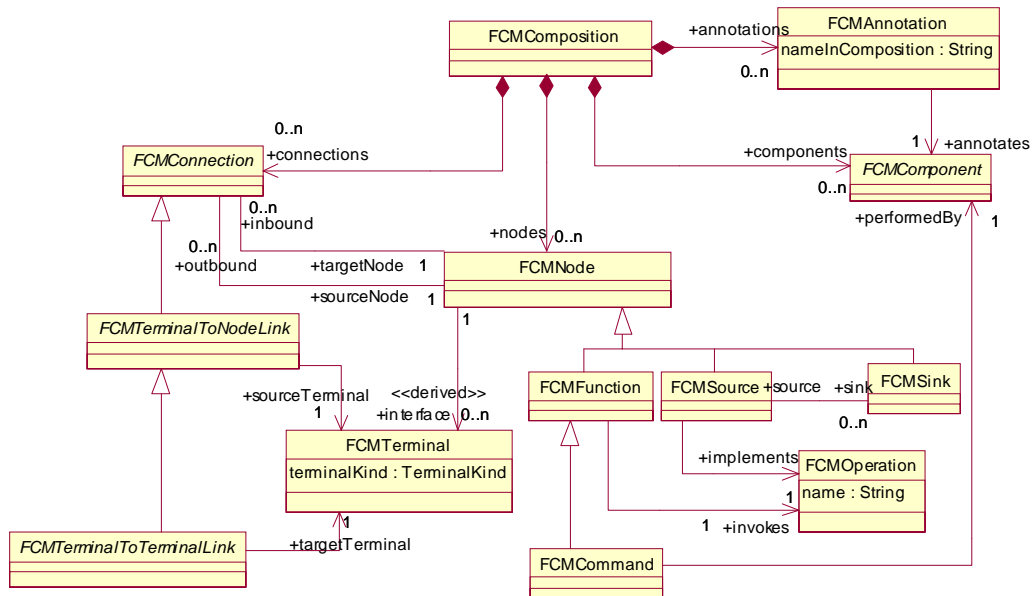
Figure 6-2 Flow Composition Model main diagram (from ad/2001-06-09)
