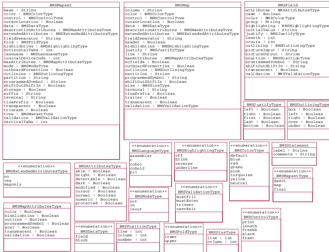
Figure A-12 CICS BMS Attributes
