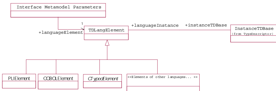
Figure 7-7 Convergent Metamodel
