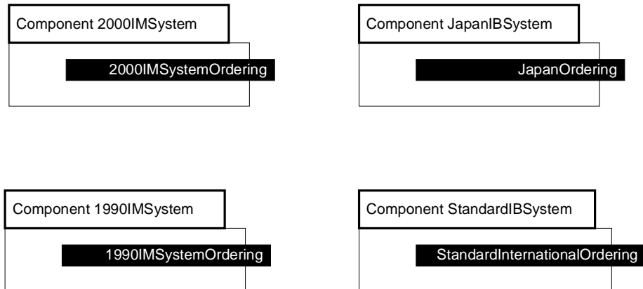
Figure 11-2 Ordering Components
