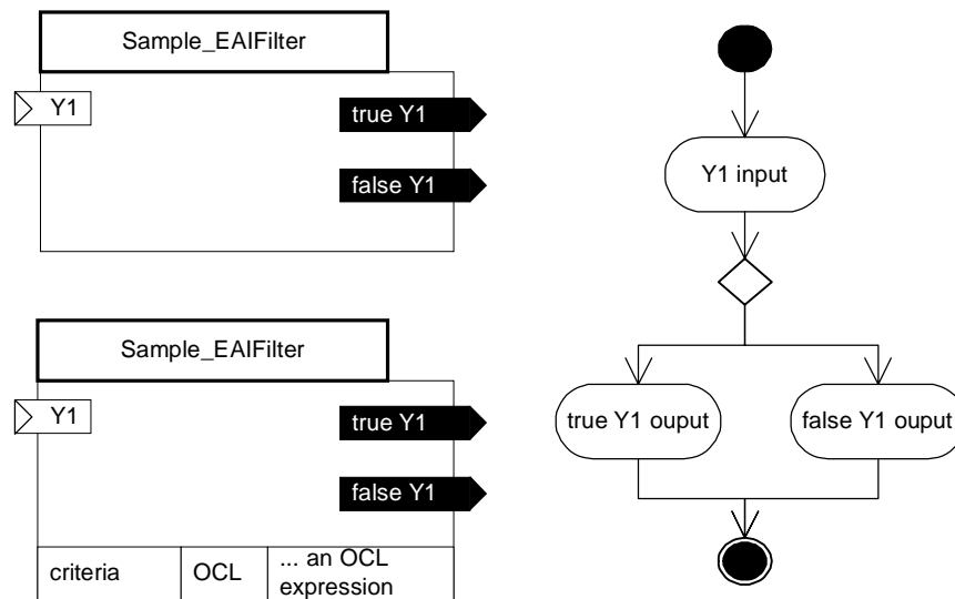
Figure 6-53 CCA notation for a sample EAIFilter
