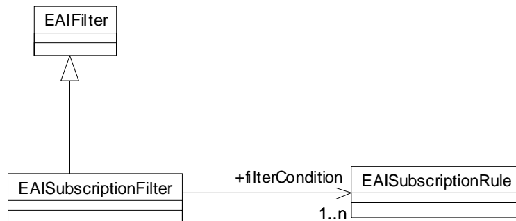
Figure 6-38 SubscriptionFilter
