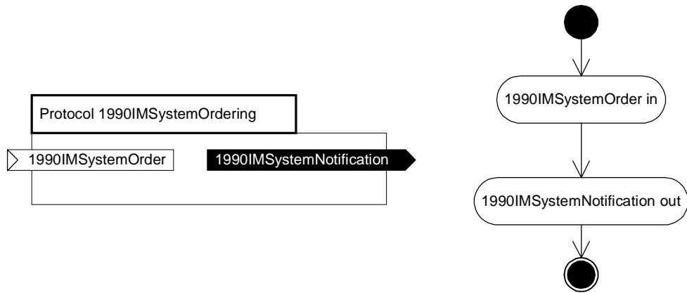
Figure 11-5 1999IMSystemOrdering Protocol
