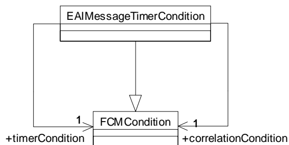
Figure 6-43 EAIMessageTimerCondition
