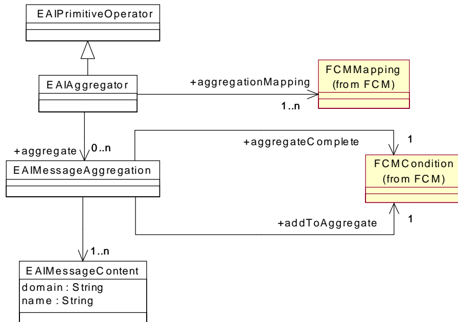
Figure 6-31 EAIAggregator
