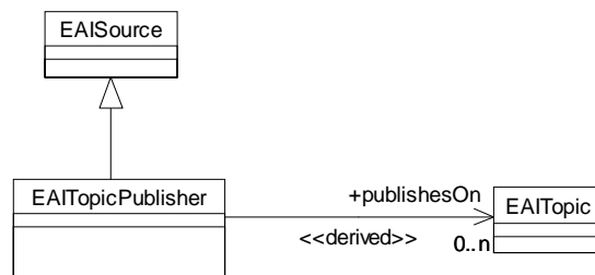
Figure 6-47
