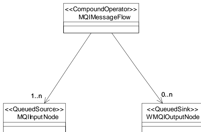
Figure 12-3 WMQIMessageFlow
