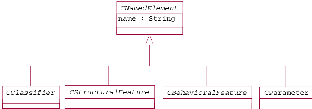
Figure 14-10 C Names
