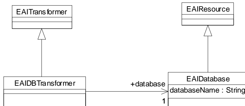
Figure 6-30 EAIDBTransformer
