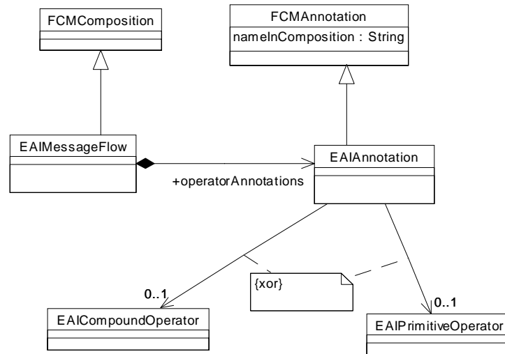
Figure 6-19 EAIMessageFlow
