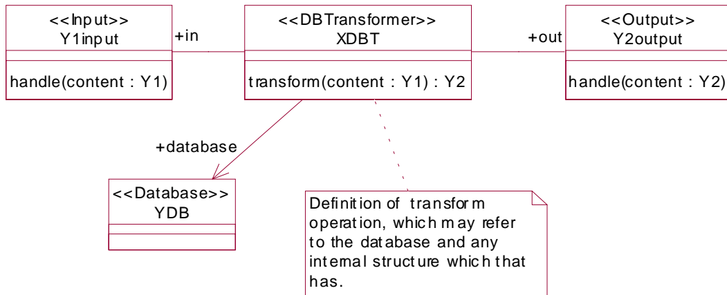
Figure 8-3 Class diagram for prototypical database transformers
