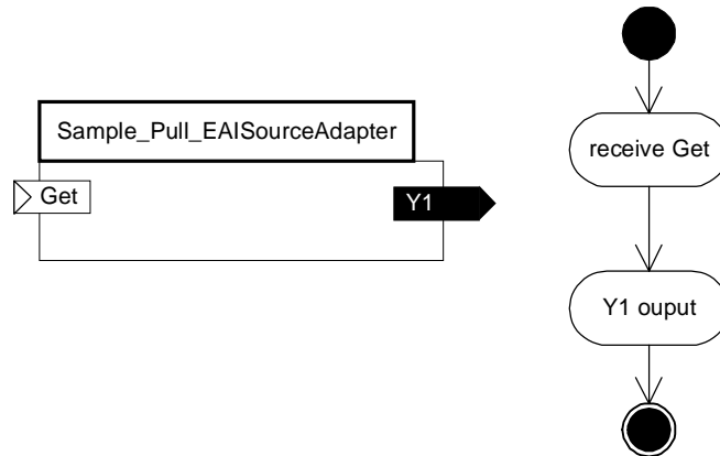
Figure 6-57 CCA notation for a sample Pull mode EAISourceAdapter
