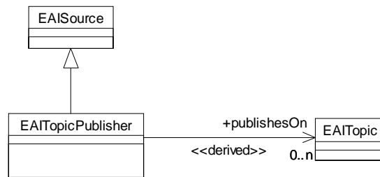
Figure 6-48 Topics allowed by an EAITopicRule
