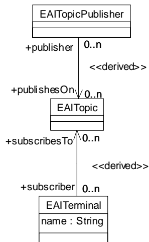
Figure 6-50 Relationship between publishers, subscribers and topics
