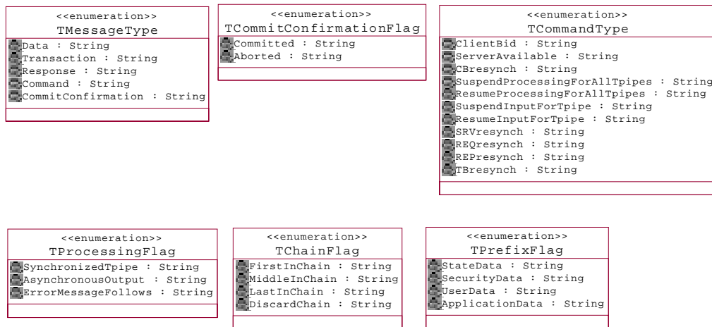
Figure A-3 OTMA Prefix - Defined Types
