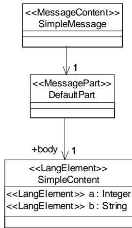
Figure 8-29 A simple message content class
