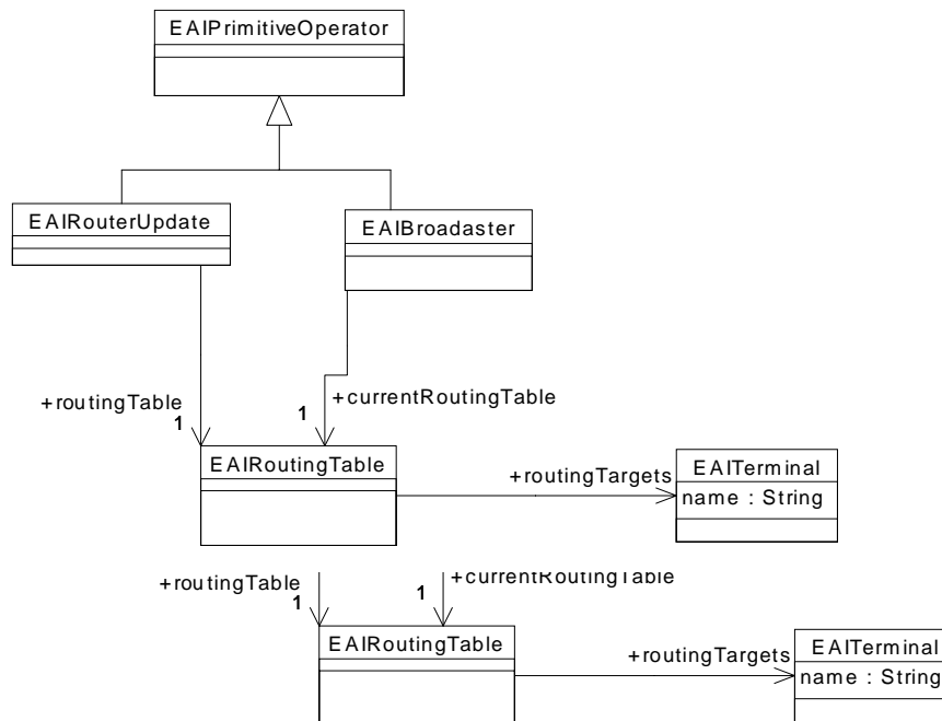
Figure 6-33 EAIRouter and EAIRouterUpdate
