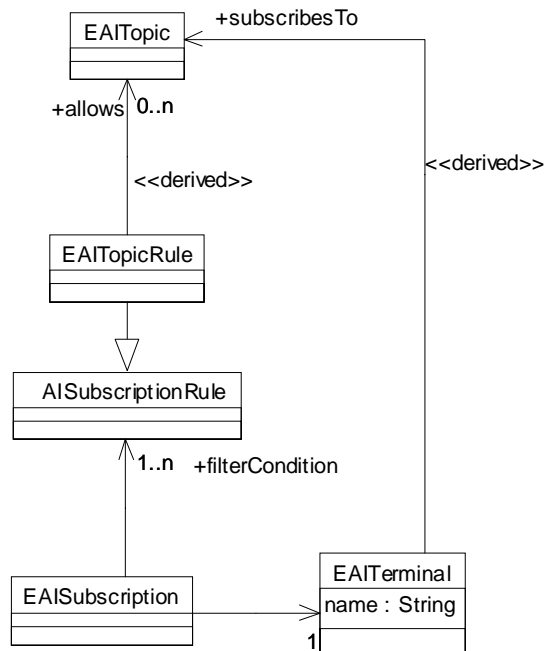
Figure 6-49 Relationship between a terminal and the topics for which it has a subscription
