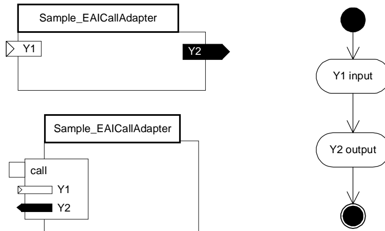
Figure 6-59 CCA notation for sample EAICallAdapter
