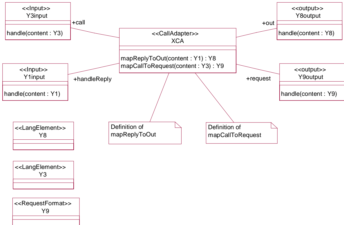
Figure 8-9 Class diagram for prototypical call adapter
