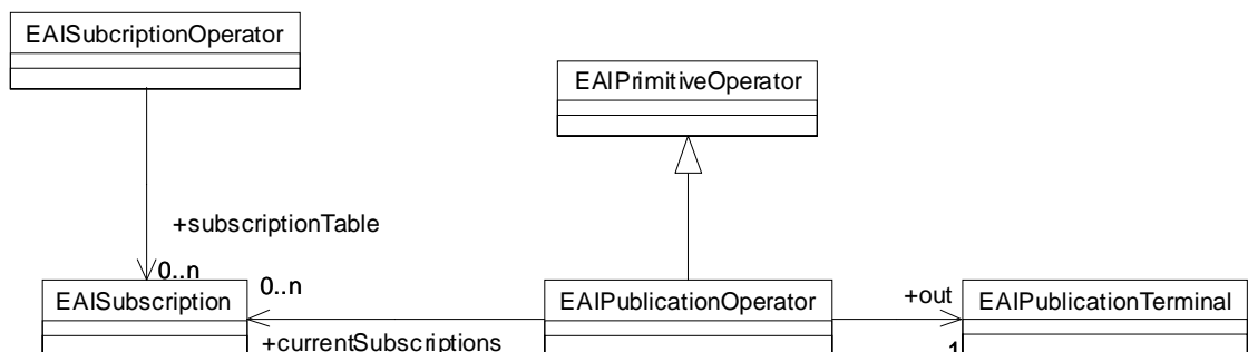
Figure 6-40 EAIPublicationOperator and EAISubscriptionOperator
