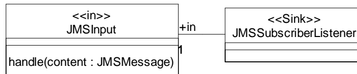
Figure 13-4 A JMSSubscriberListener expects incoming messages
