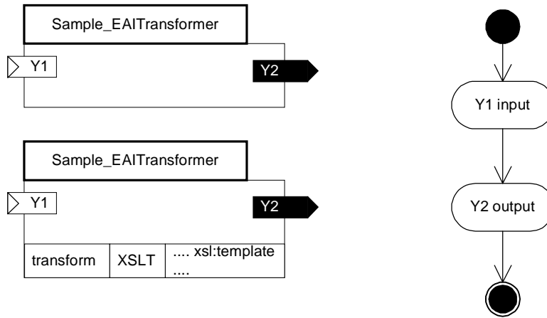
Figure 6-52 CCA notation for sample EAITransformer
