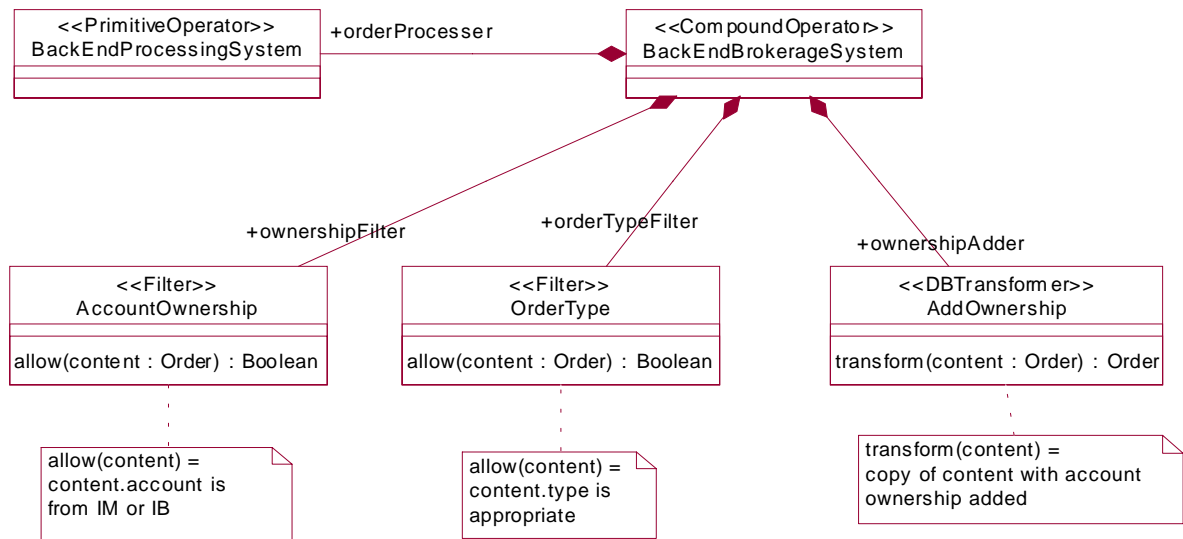
Figure 10-16 Back-end brokerage system - components
