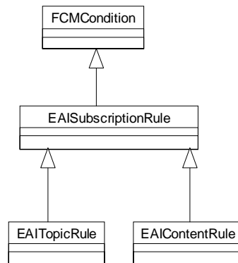
Figure 6-39 EAISubscriptionRule, EAITopicRule and EAIContentRule
