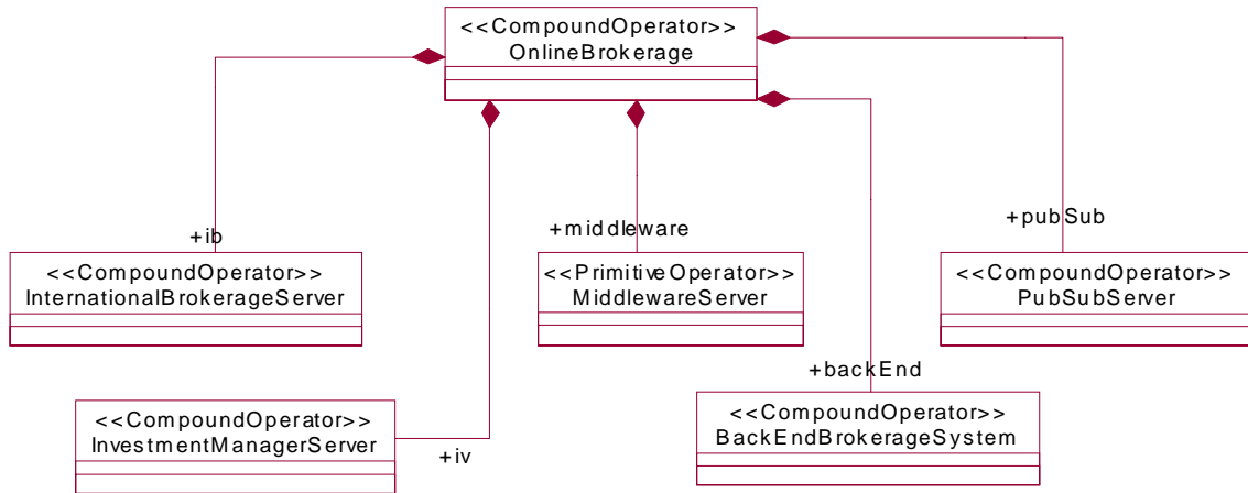
Figure 10-7 On-line brokerage system - components
