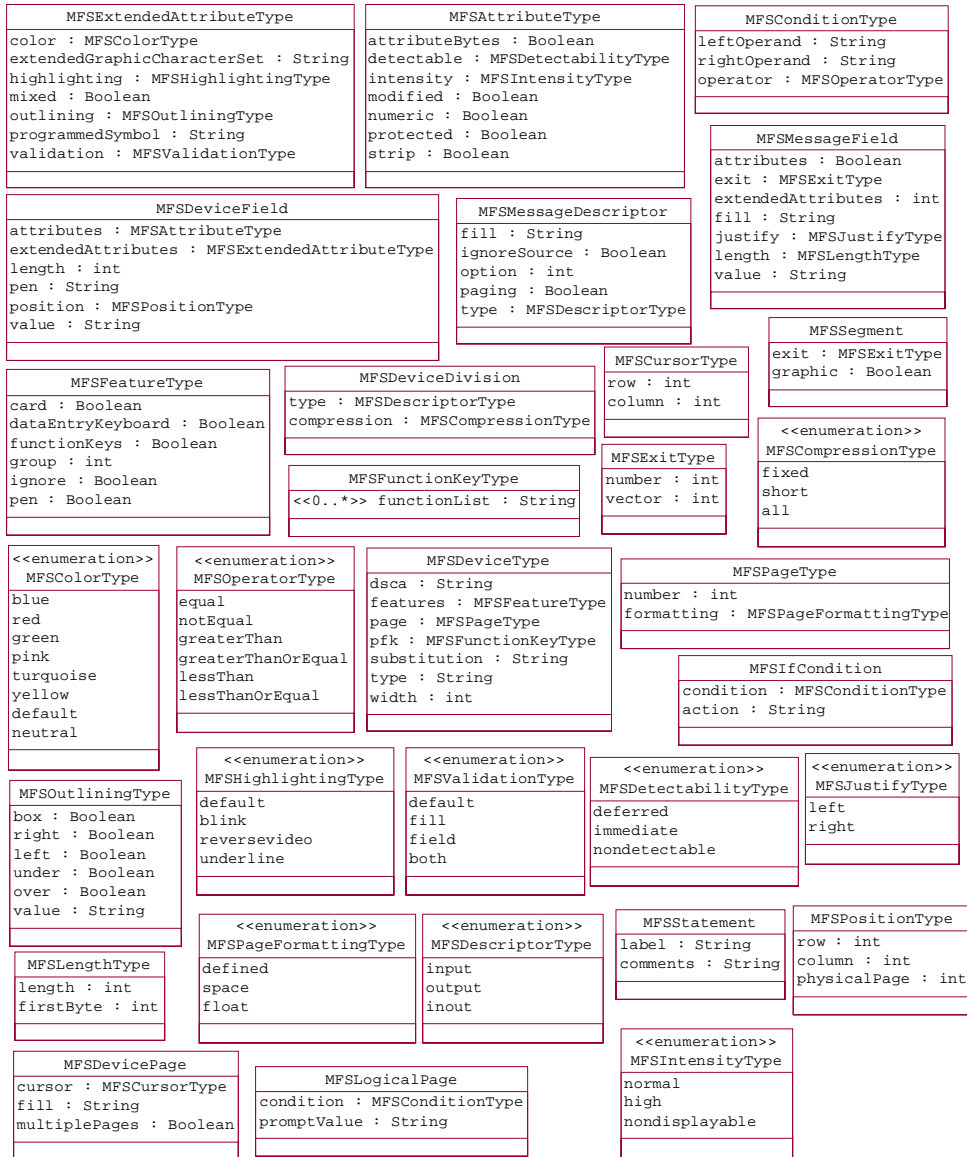
Figure A-9 MFS Attribute View
