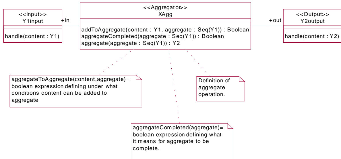
Figure 8-14 Class diagram for prototypical aggregator
