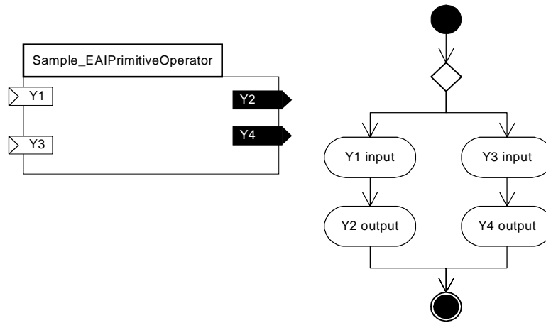
Figure 6-51 CCA notation for a sample generic EAIPrimitiveOperator
