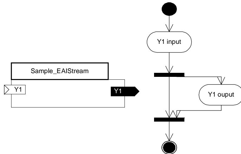
Figure 6-54 CCA notation for a sample EAISStream
