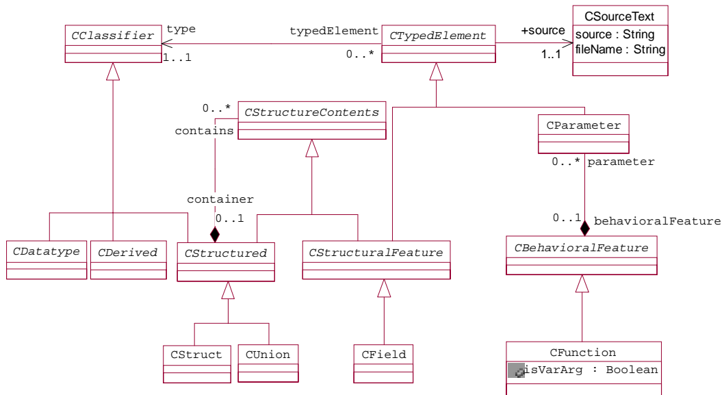
Figure 14-7 C Metamodel
