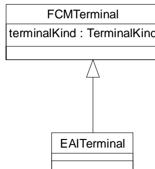
Figure 6-8 EAITerminal
