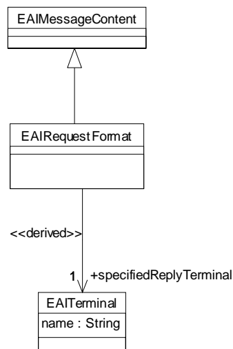
Figure 6-24 EAIRquestFormat
