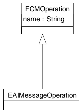
Figure 6-13 MessageOperation
