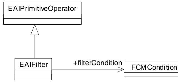
Figure 6-26 Filter
