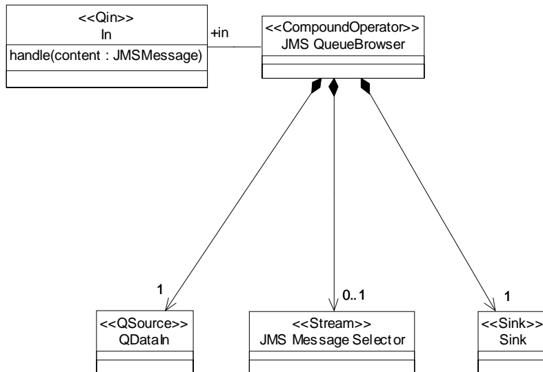
Figure 13-3 JMS QueueBrowser
