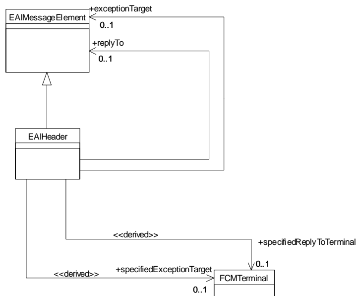
Figure 6-10 EAIHeader
