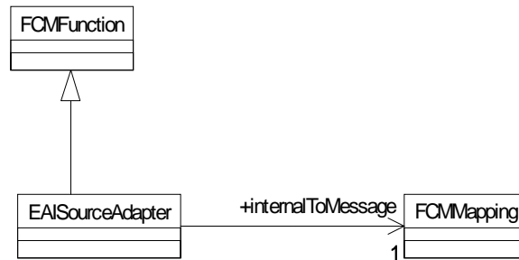
Figure 6-21 SourceAdapter
