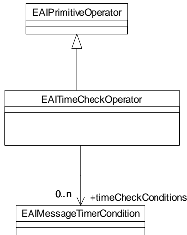
Figure 6-45 EAITimeCheckOperator
