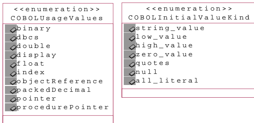
Figure 14-3 COBOL Stereotypes
