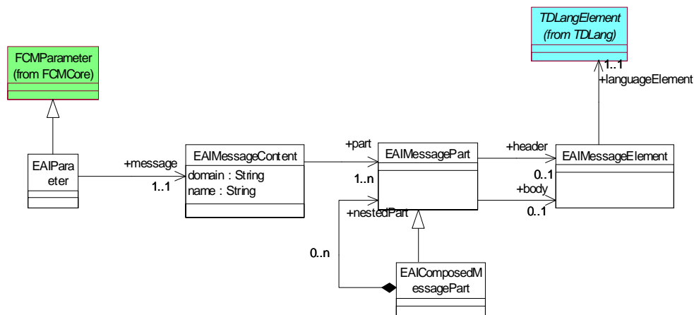
Figure 6-9 EAI MessageContent
