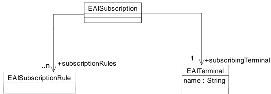
Figure 6-37 EAISubscription
