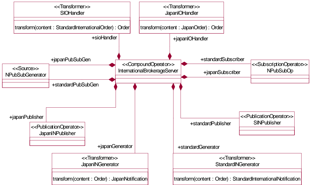
Figure 10-14 IBS - components
