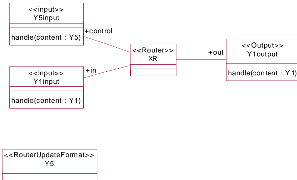
Figure 8-16 Class diagram for prototypical router
