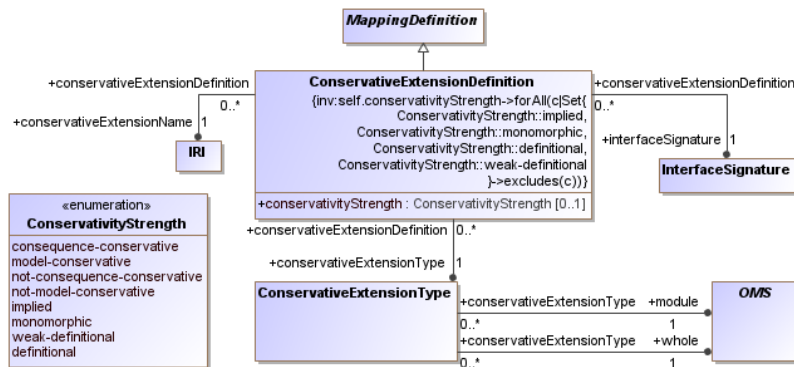
Figure 16 – DOL metamodel: conservative extension definitions
