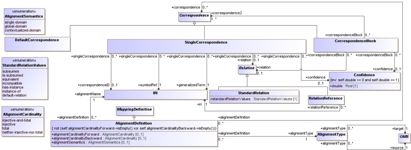
Figure 15 – DOL metamodel: Alignments
