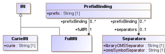
Figure 17 – DOL metamodel: Prefixes
