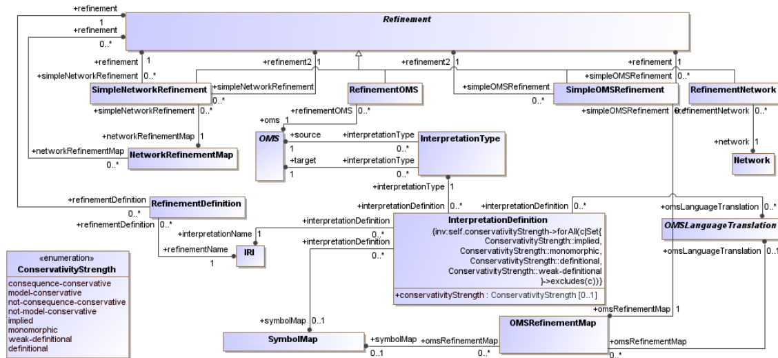
Figure 13 – DOL metamodel: Interpretations and refinements
