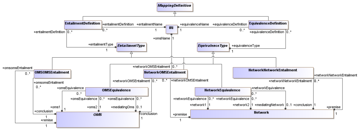
Figure 14 – DOL metamodel: Entailments and equivalences
