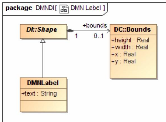
Figure 13-6: DMNLabel1
