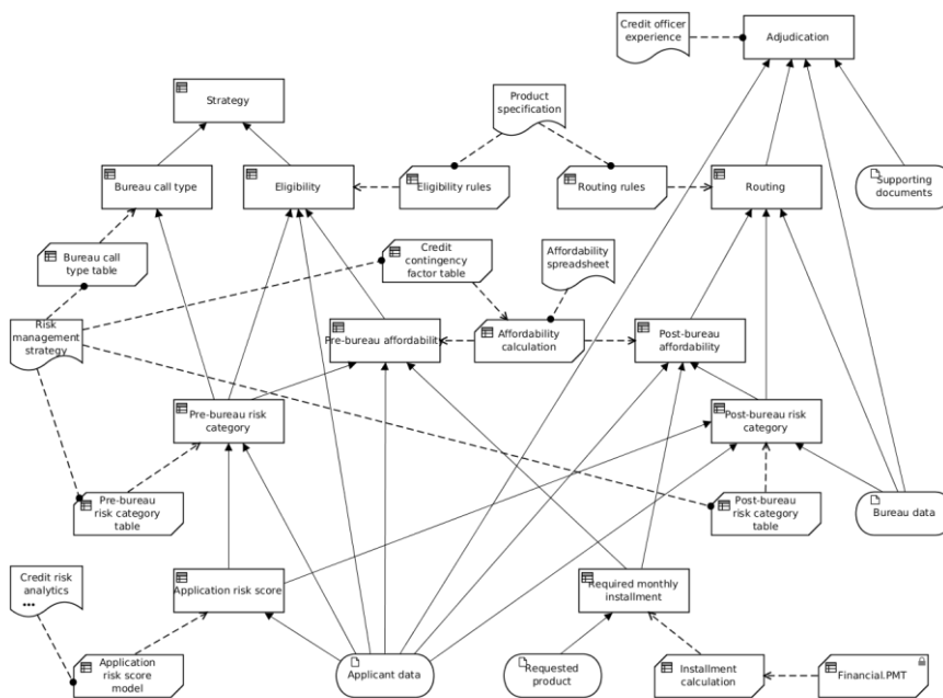
Figure 11-2: DRD of all automated decision-making
