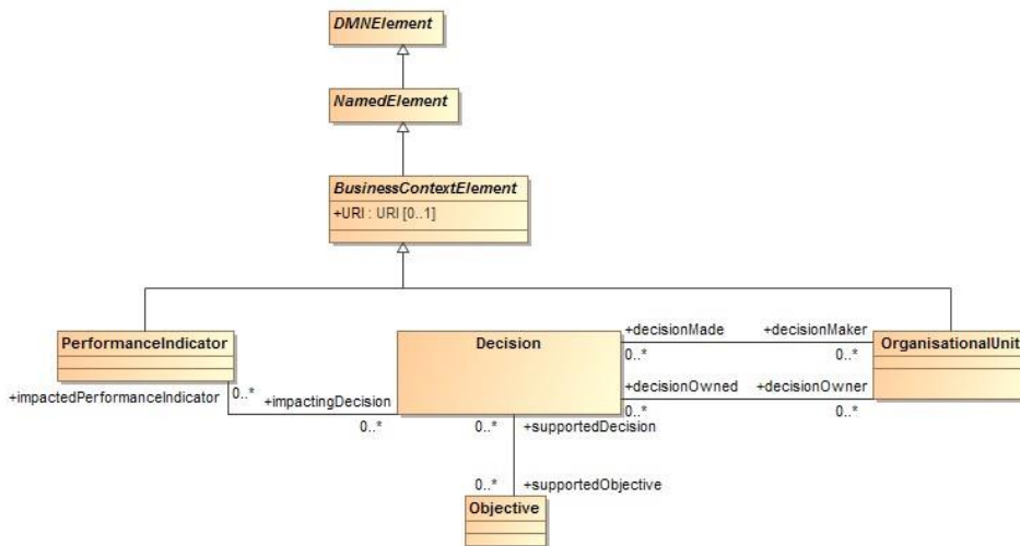
Figure 6-14: BusinessContextElement class diagram
