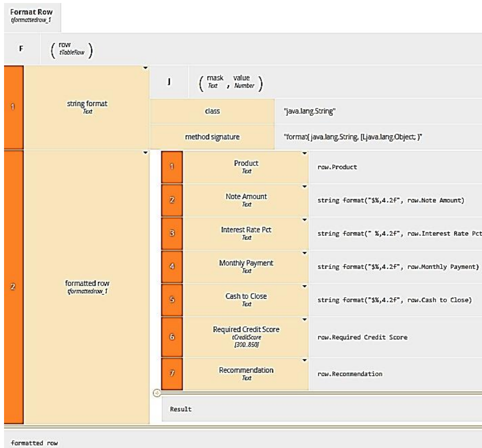
Figure 11-54: Format Row
