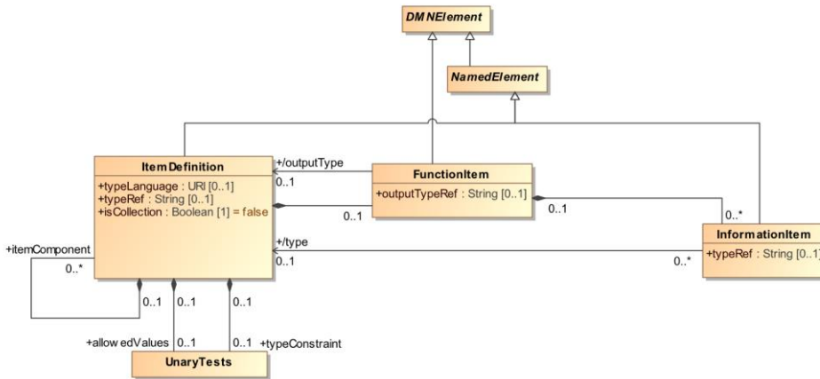
Figure 7-7: ItemDefinition class diagram
