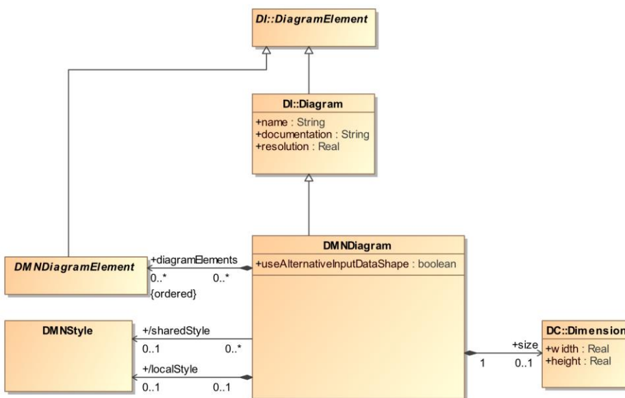
Figure 13-2: DMNDiagram
