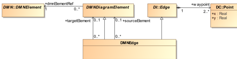
Figure 13-5: DMNEdge
