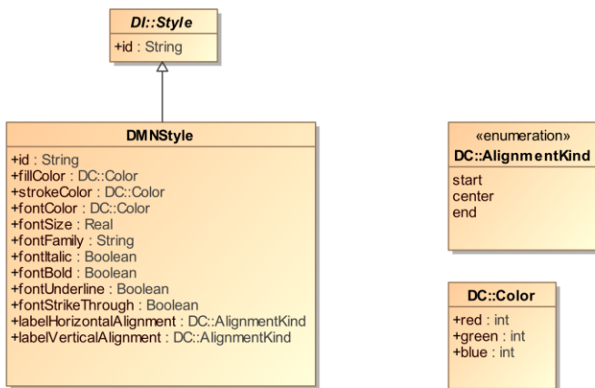
Figure 13-7: DMNStyle
