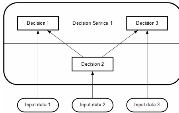
Figure 6-6: Decision Service notation
