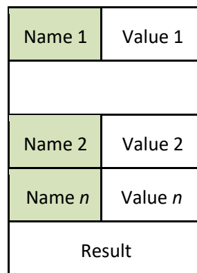
Figure 10-6: Vertical context
