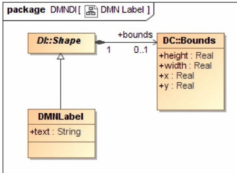
Figure 13-6: DMNLabel
