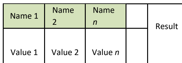
Figure 10-7: Horizontal context
