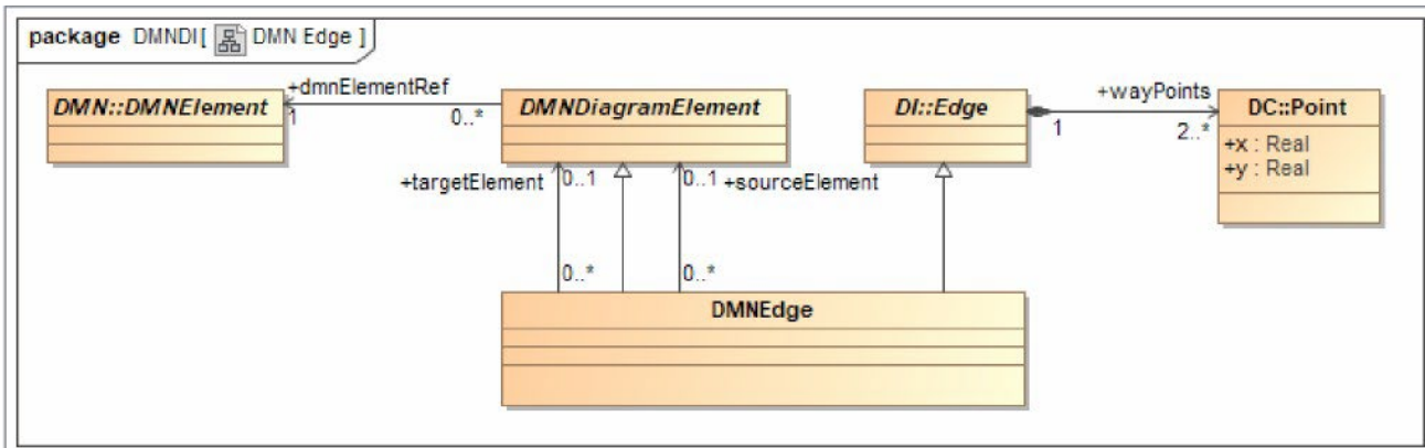
Figure 13-5: DMNEdge
