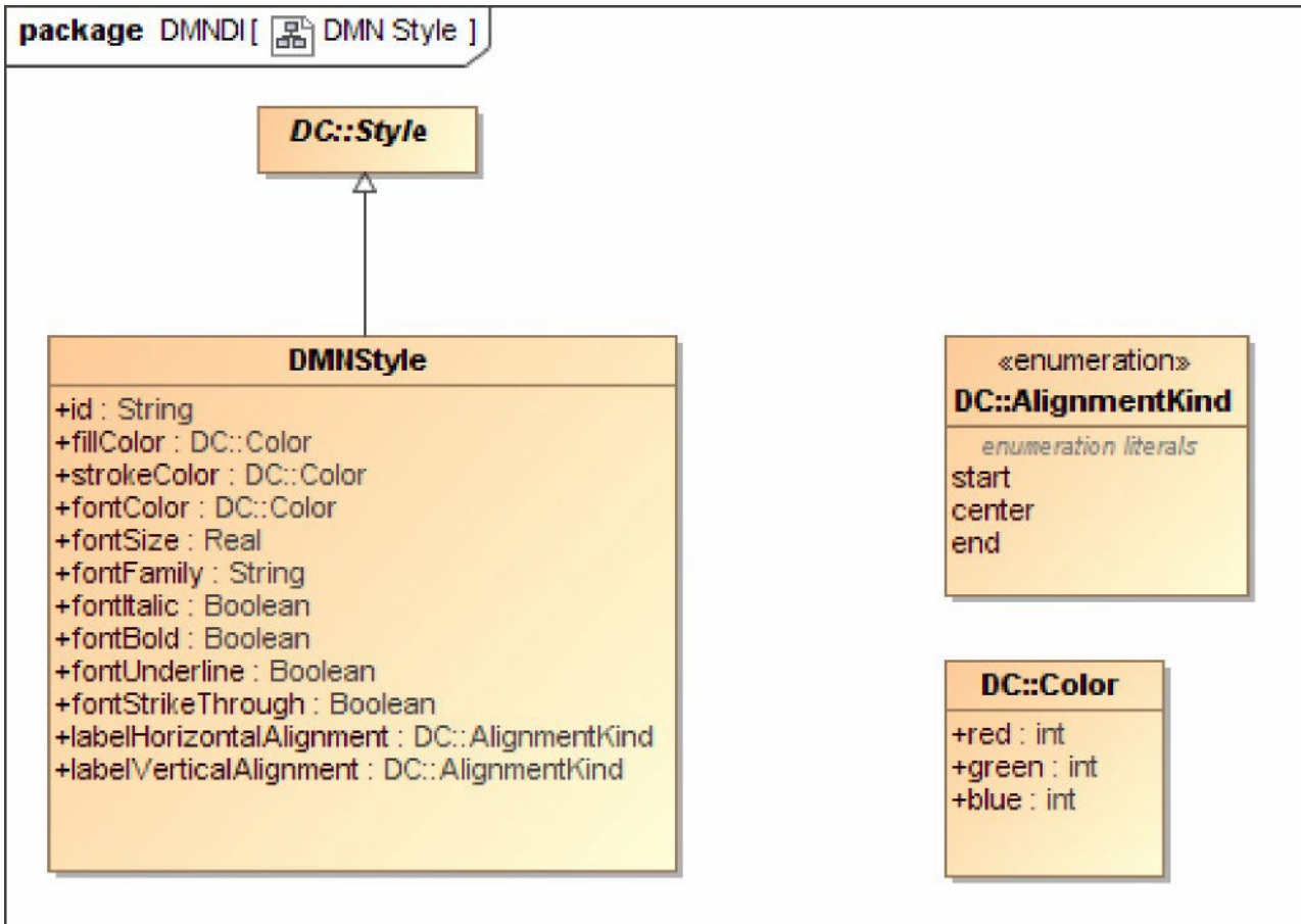
Figure 13-7: DMNStyle
