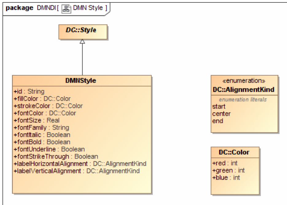
Figure 13-743-7: DMNStyle
