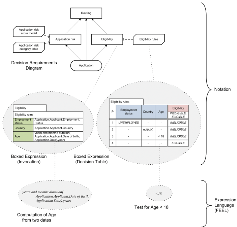
Figure 5-25-25-2: DMN Constructs
