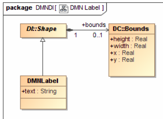
Figure 13-613-613-6: DMNLabel
