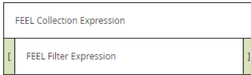
Figure 10-1840-18: Filter expression
