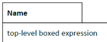
Figure 7-17-17-4: Boxed Expression
