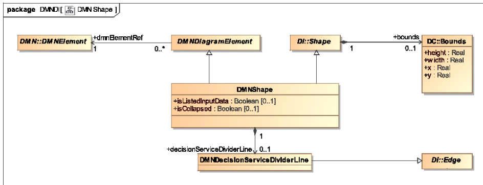
Figure 13-413-413-4: DMNShape
