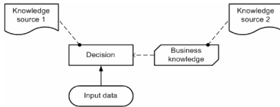
Figure 5-45-45-4: Knowledge sources
