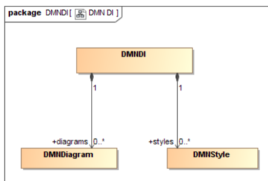
Figure 13-13-413-4: DMNDI
