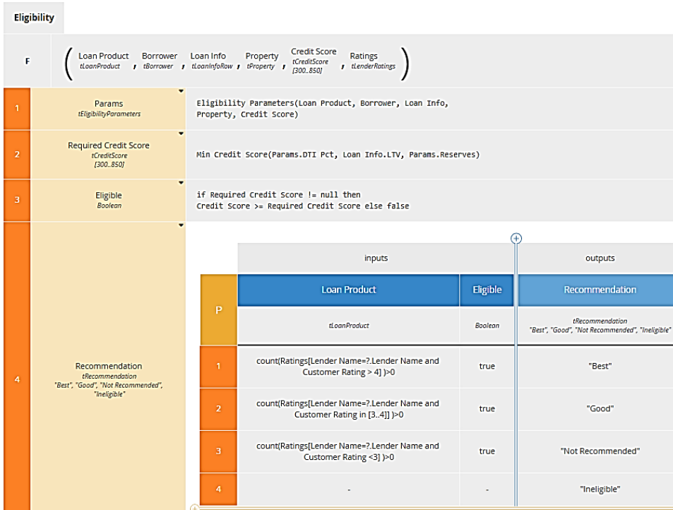
Figure 11-5044-5044-50: Eligibility (top)
