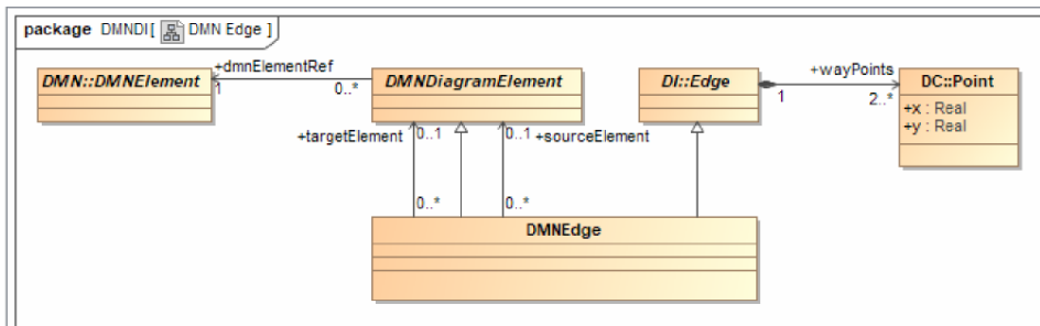
Figure 13-513-513-5: DMNEdge
