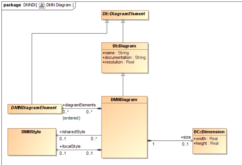
Figure 13-213-213-2: DMNDiagram
