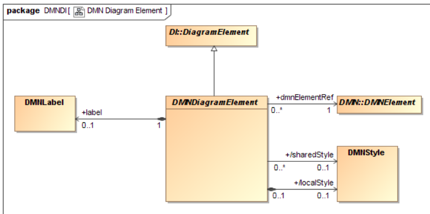
Figure 13-313-3: DMNDiagramElement
