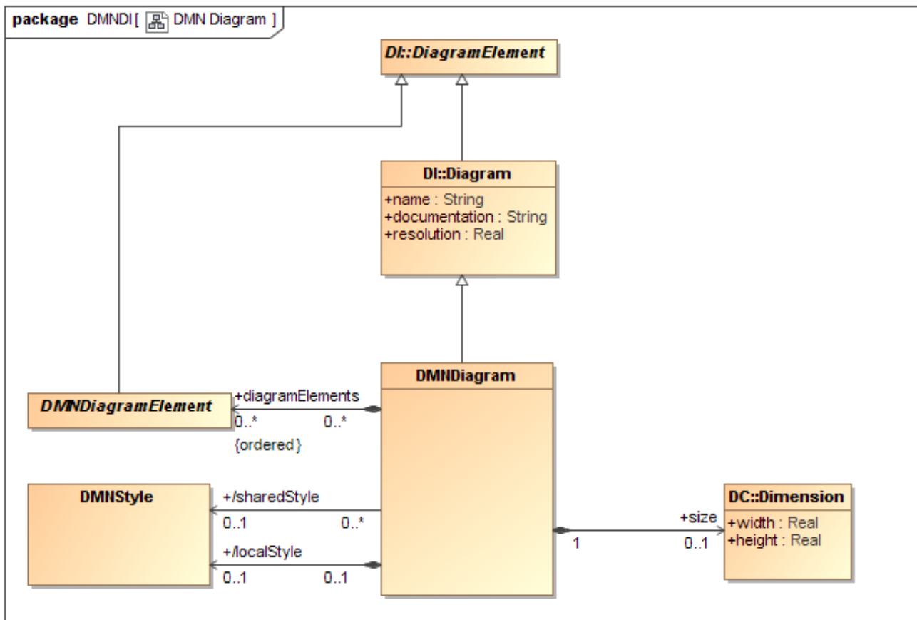
Figure 13.2: DMNDiagram
