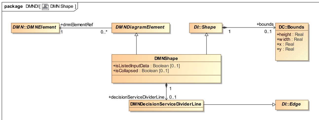
Figure 13.4: DMNShape
