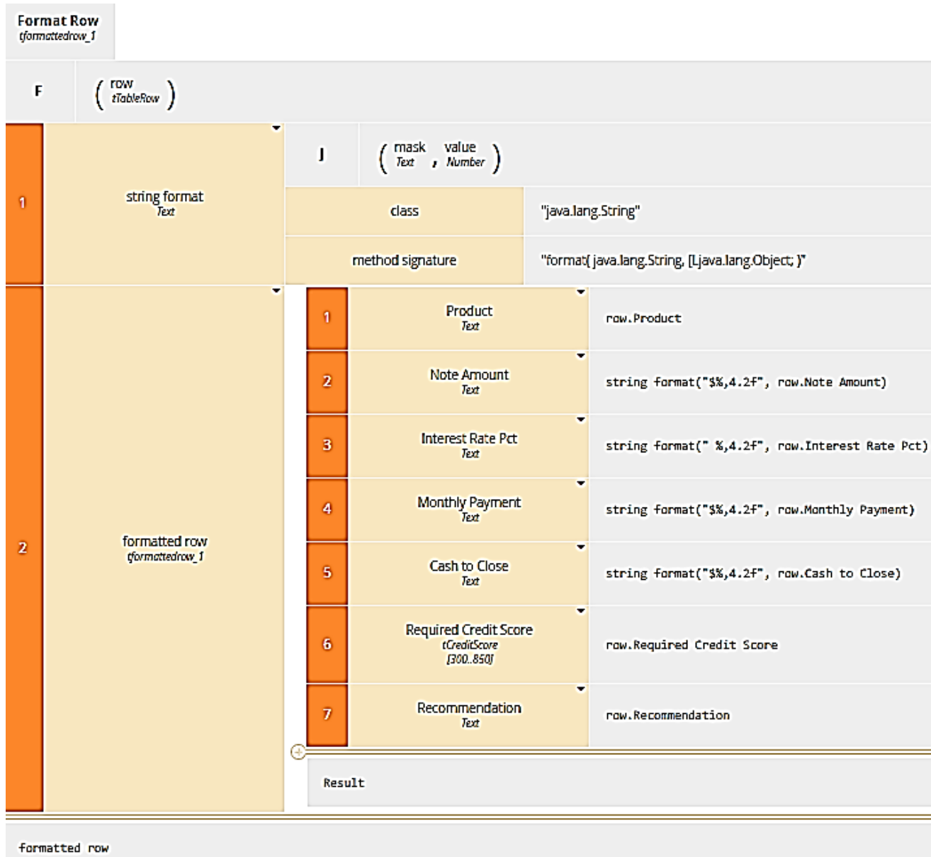
Figure 11.54: Format Row
