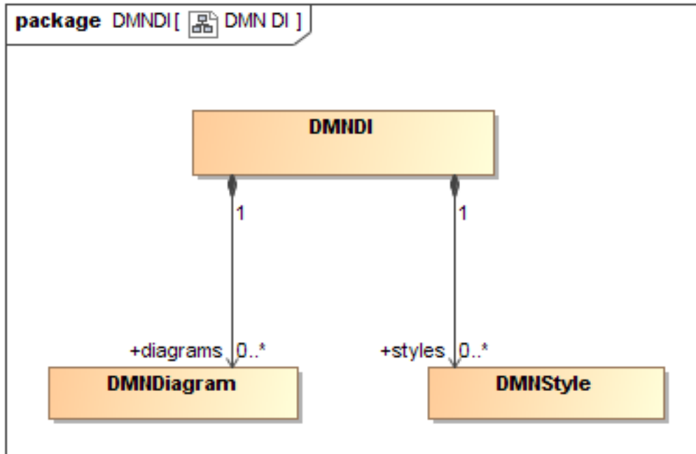
Figure 13.1: DMNDI
