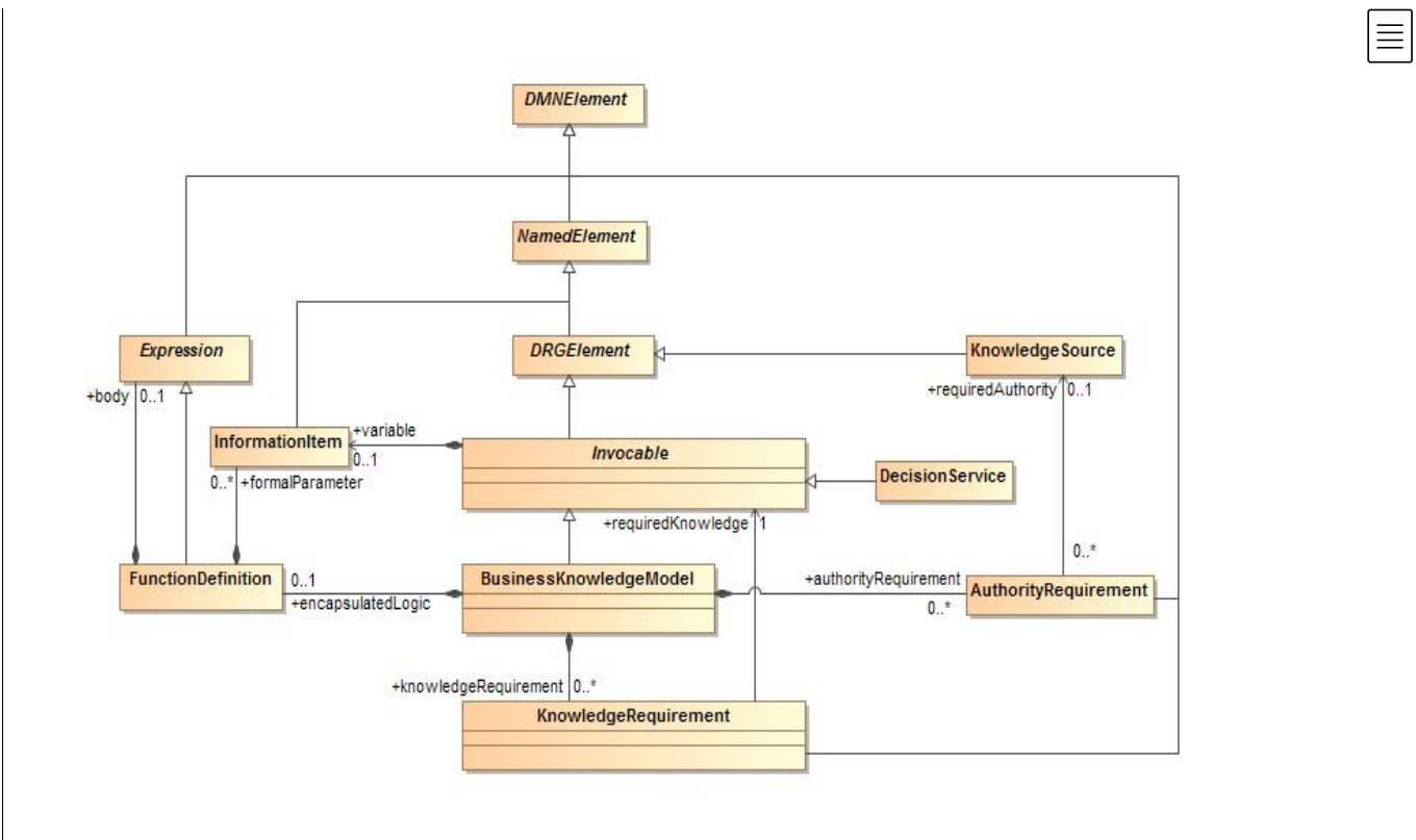
Figure 6.14: BusinessKnowledgeModel class diagram
