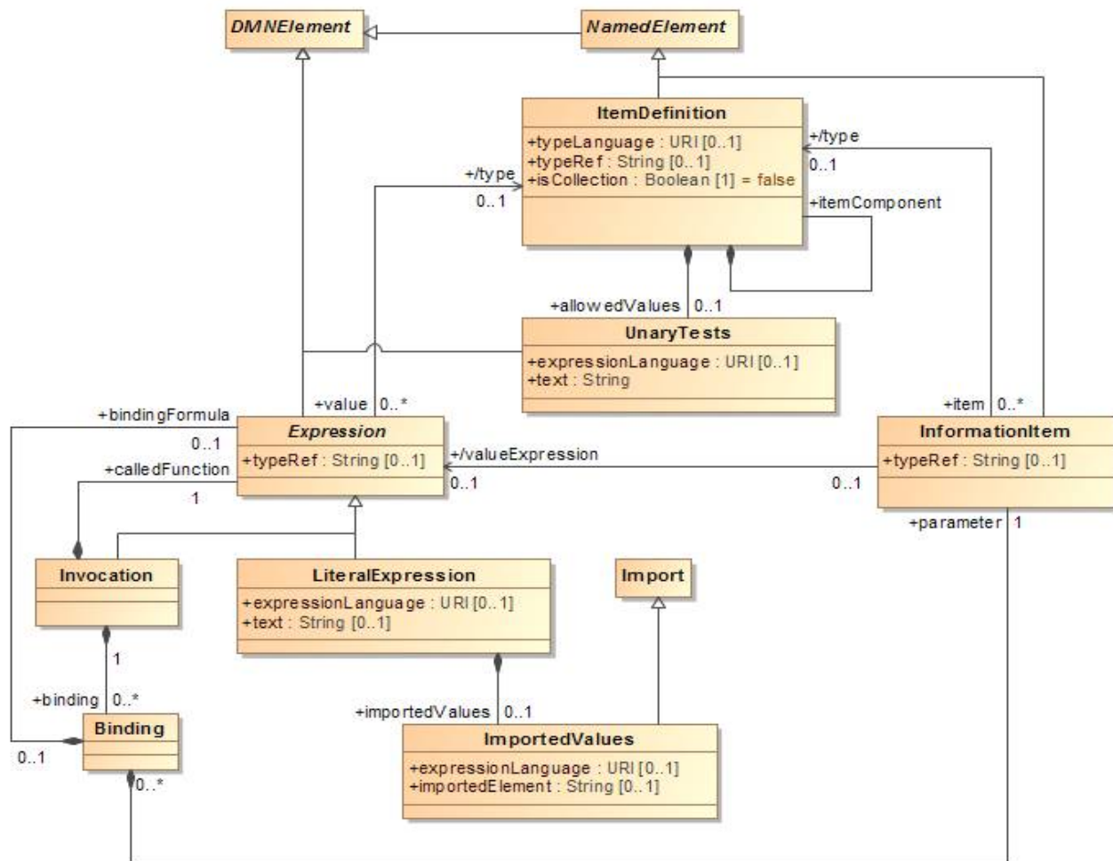
Figure 7.6: Expression class diagram
