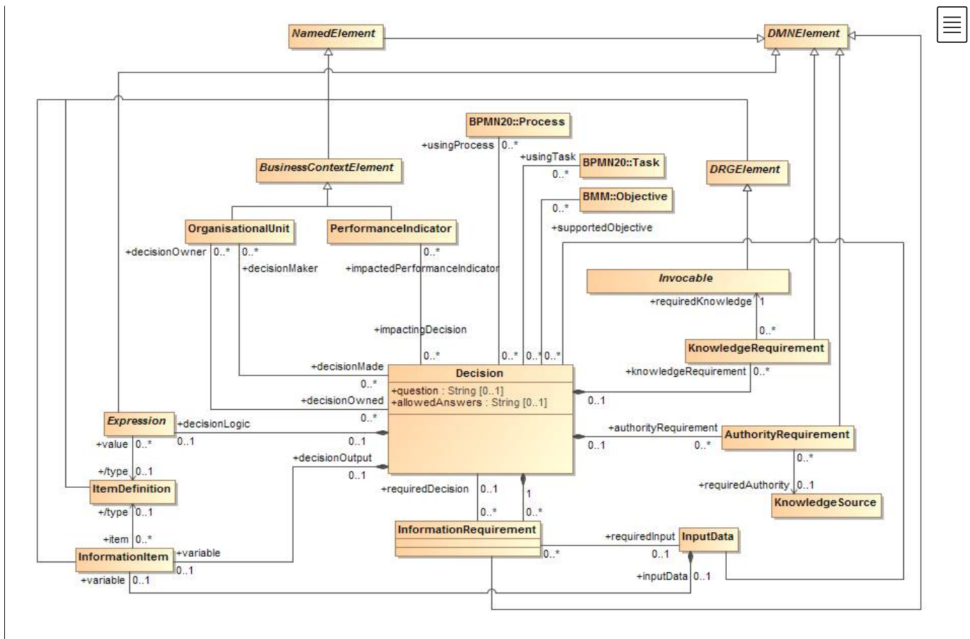
Figure 6.12: Decision Class Diagram
