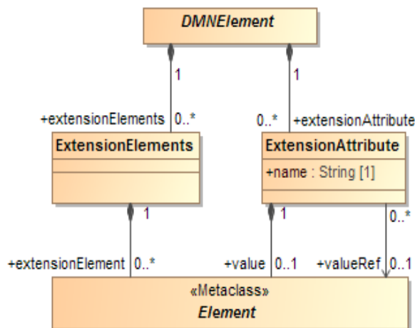
Figure 6.14 - Extensibility class diagram
