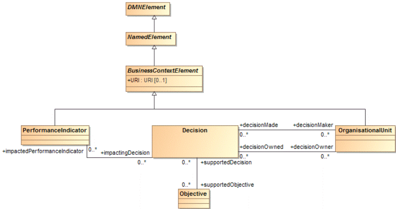
Figure 6.10 - BusinessContextElement class diagram
