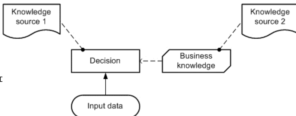
Figure 5.4 - Knowledge Sources
