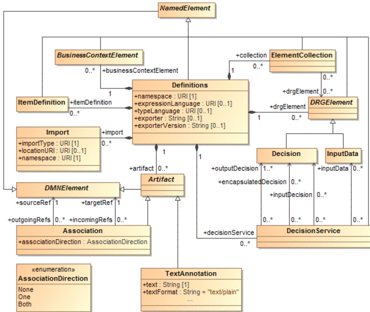
Figure 6.8 - Definitions Class Diagram
