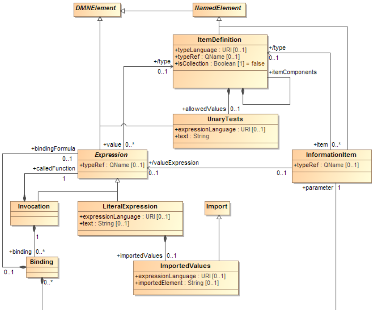
Figure 7.3 - Expression class diagram
