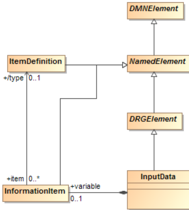
Figure 6.12 - InputData class diagram
