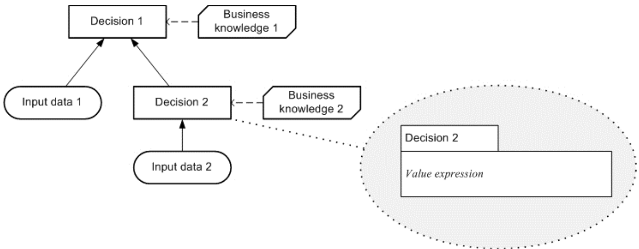
Figure 5.7 - Decision and corresponding value expression
