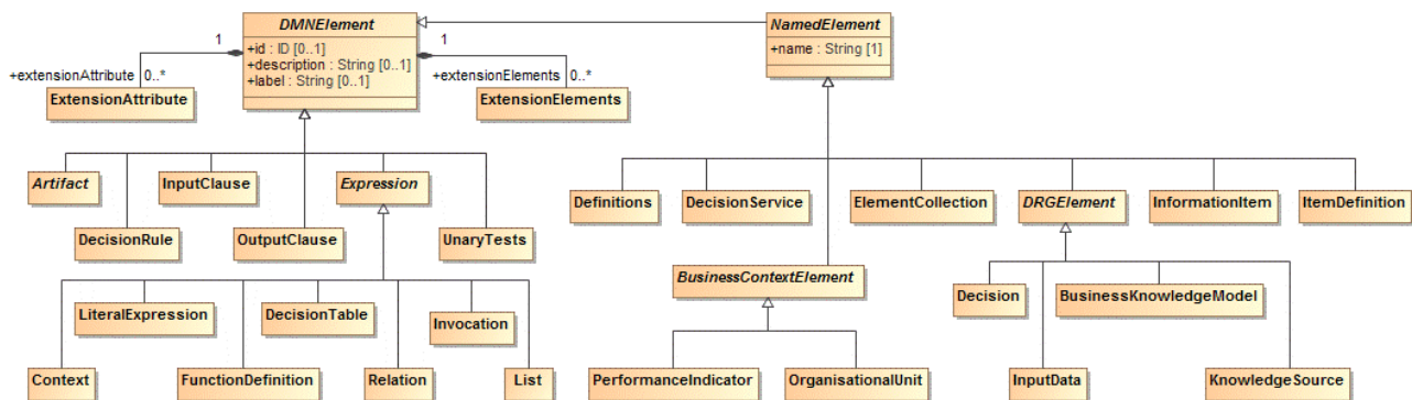
Figure 6.7 - DMNElement Class Diagram
