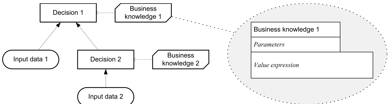
Figure 5.8 - Business knowledge model and corresponding value expression
