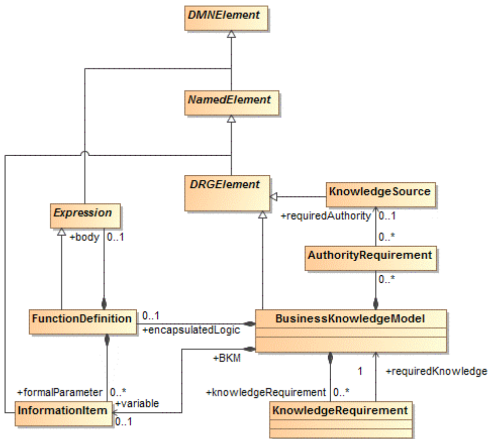
Figure 6.11 - BusinessKnowledgeModel class diagram
