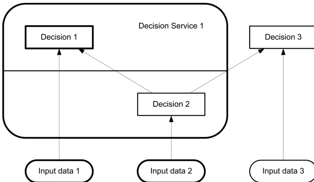
Figure 5.10 - A decision service
