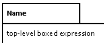
Figure 7.1 - Boxed expression
