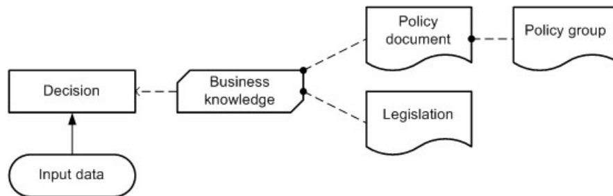
Figure 14: Knowledge Sources representing authorities
