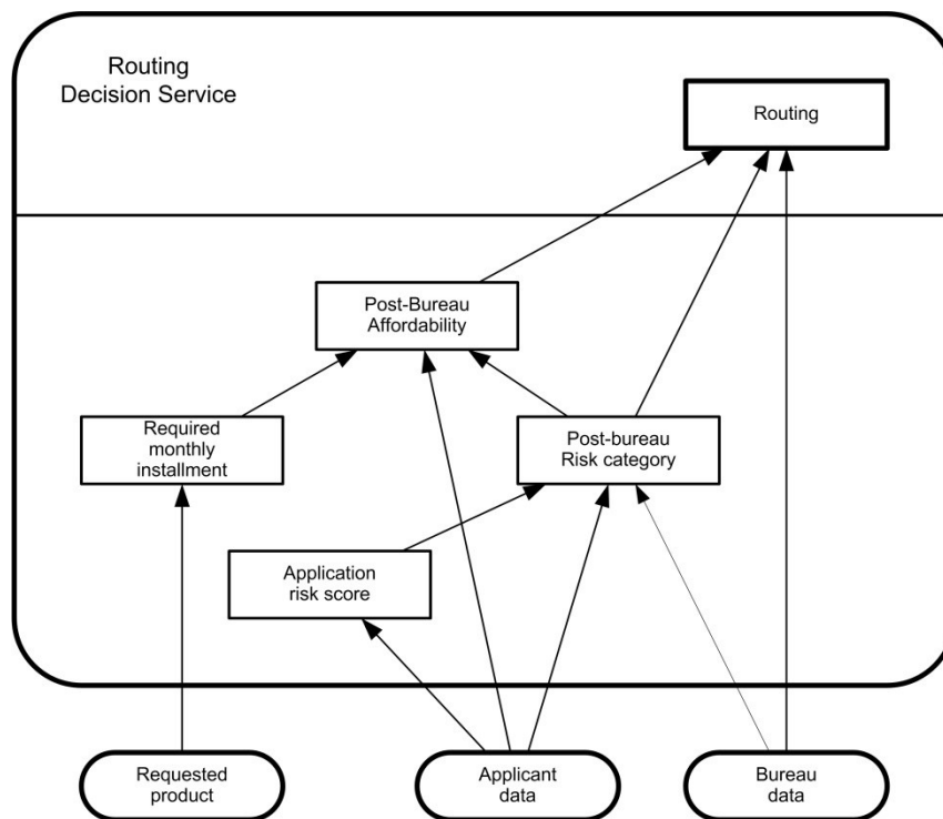
Figure 75: Routing Decision Service
