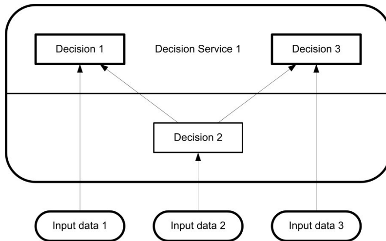
Figure 17: Decision Service notation
