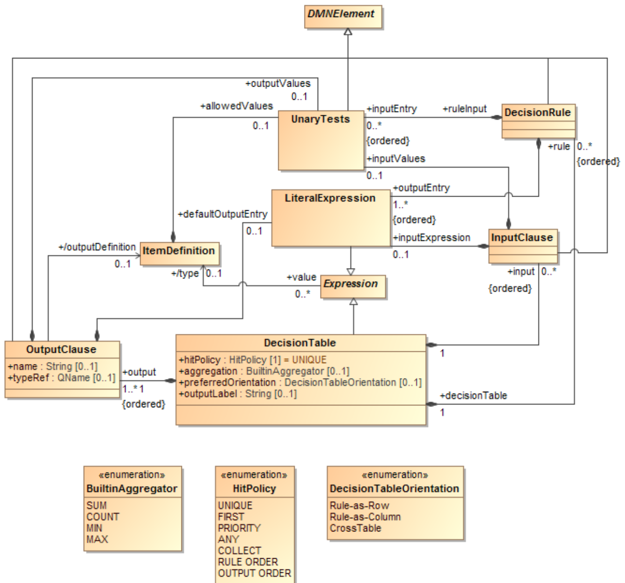
Figure 51: DecisionTable class diagram
