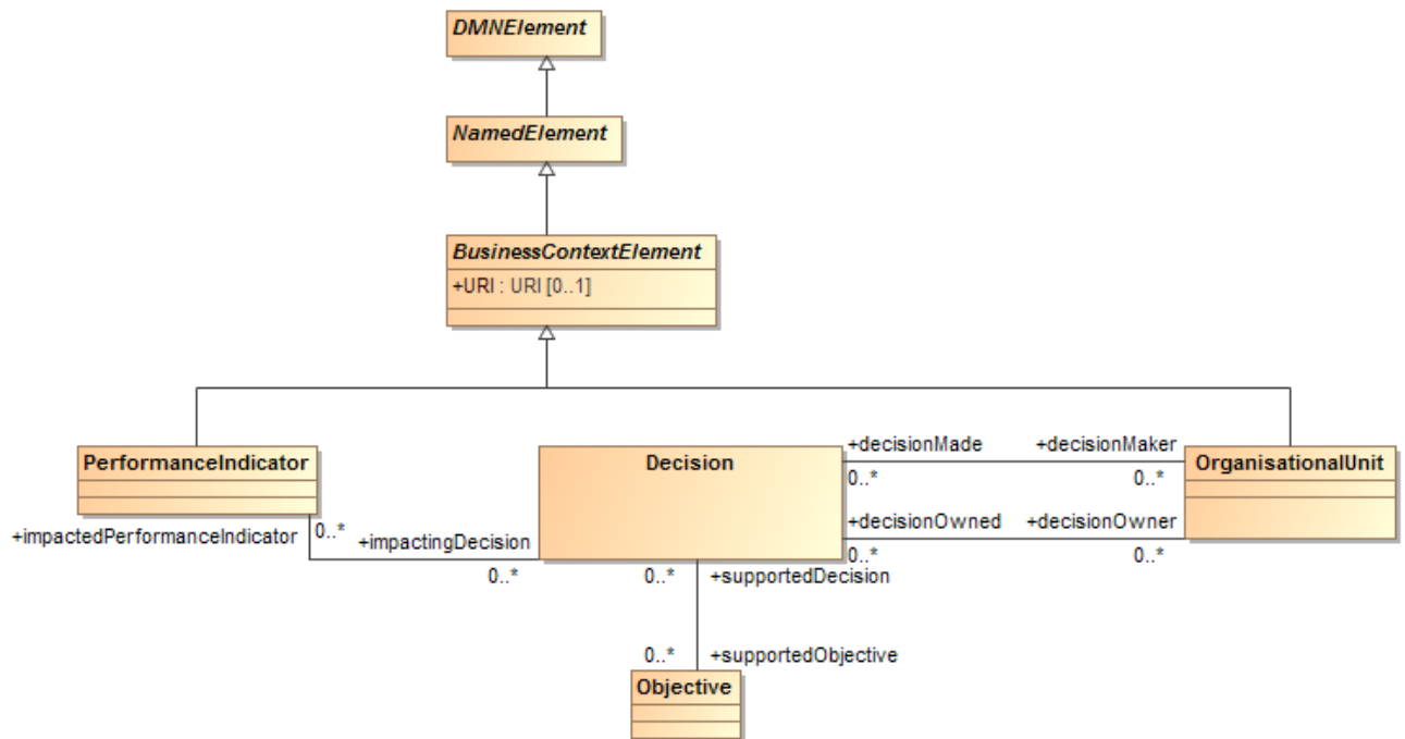
Figure 21: BusinessContextElement class diagram
