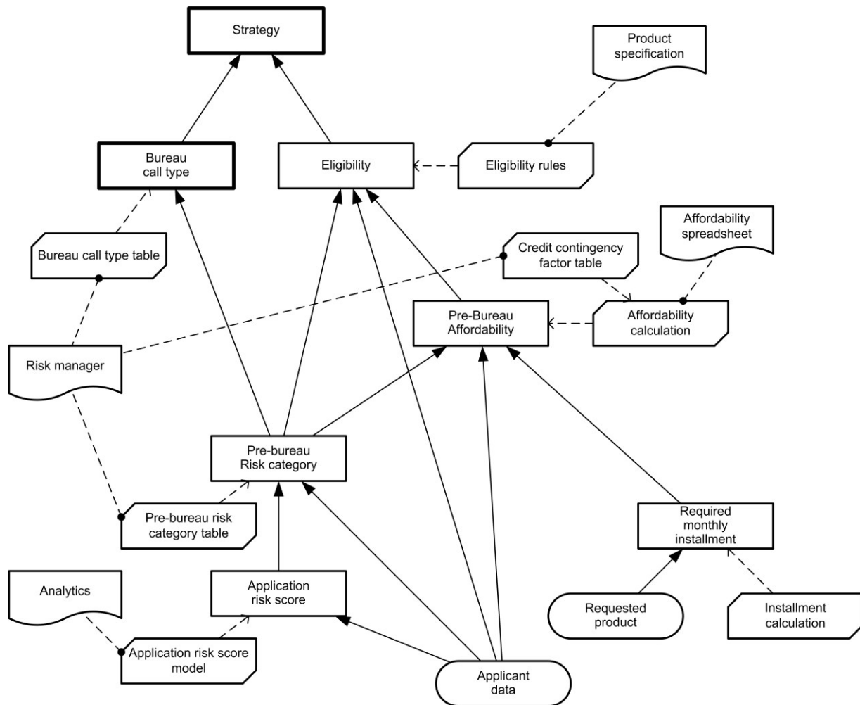
Figure 71: DRD for Decide bureau strategy decision point
