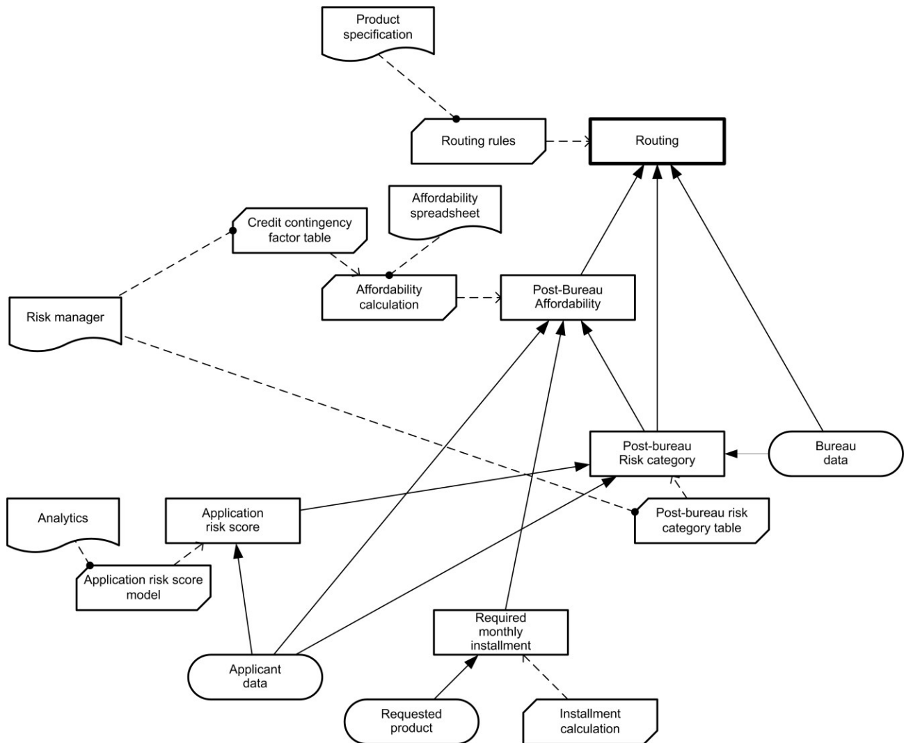
Figure 72: DRD for Decide routing decision point
