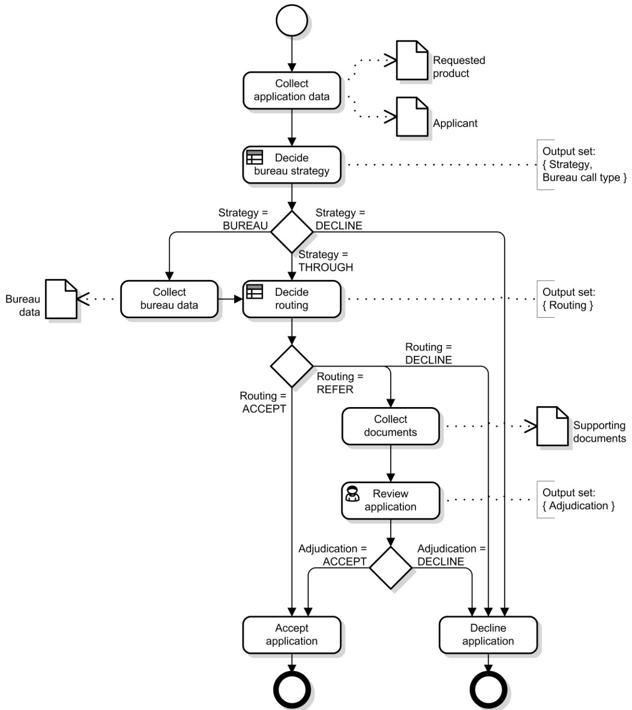
Figure 69: Example business process
