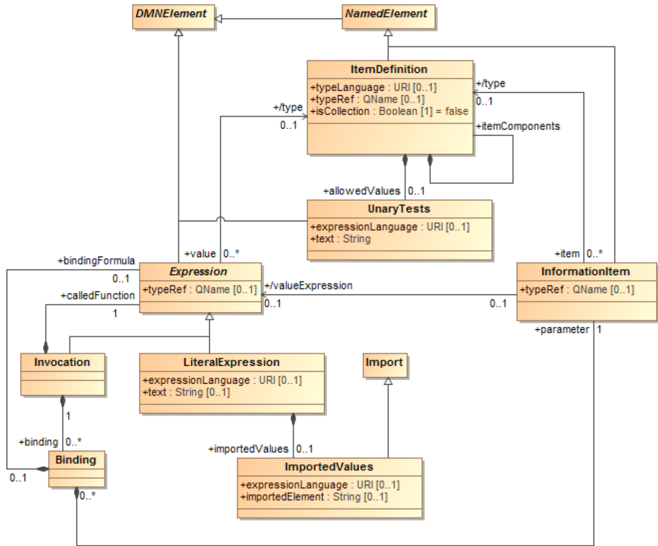
Figure 31: Expression class diagram
