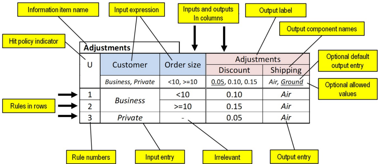
Figure 35: Decision table example (horizontal orientation, multiple output components)
