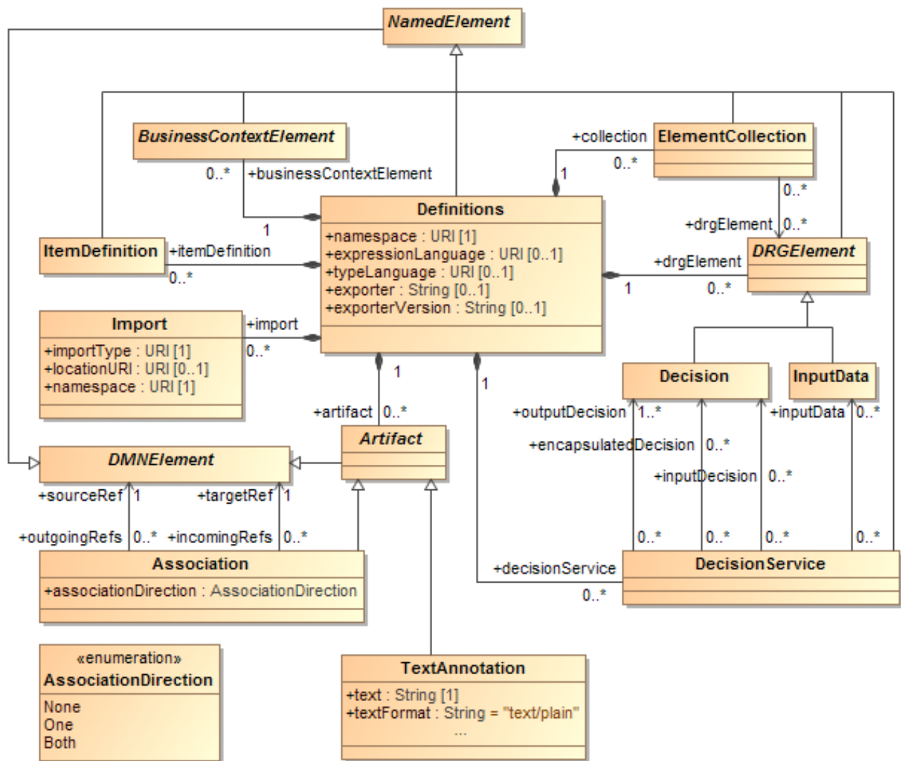
Figure 19: Definitions Class Diagram
