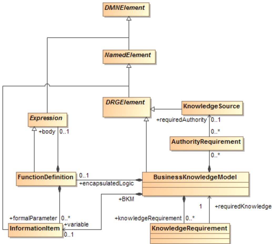
Figure 22: BusinessKnowledgeModel class diagram
