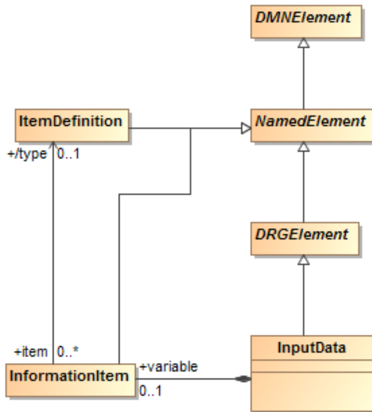
Figure 23: InputData class diagram
