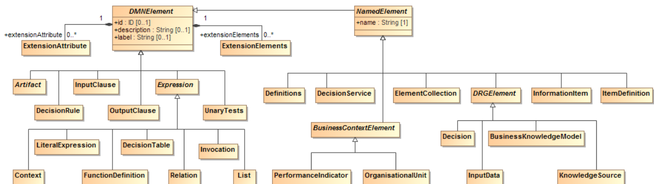
Figure 18: DMNElement Class Diagram
