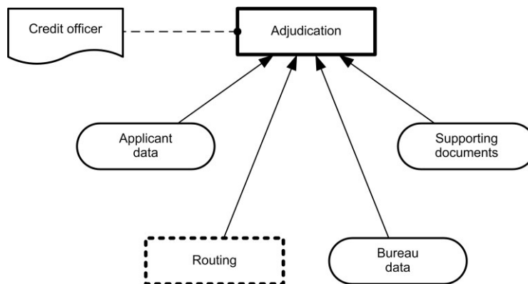
Figure 73: DRD for Review application decision point
