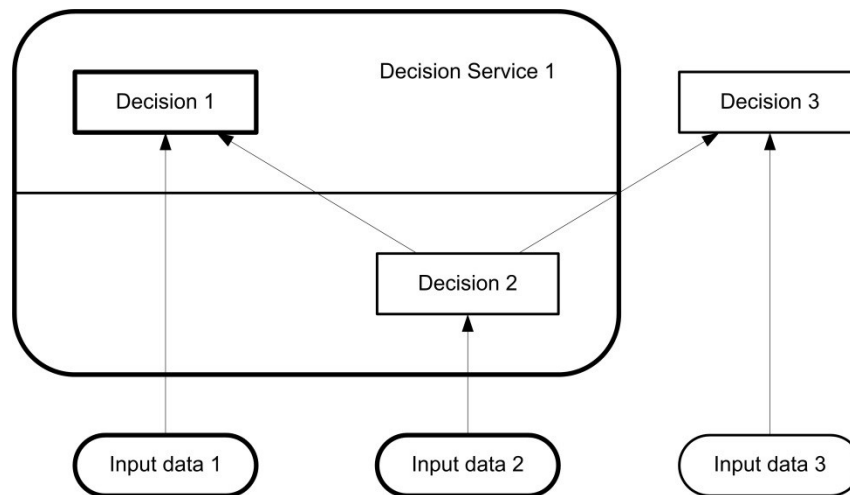
Figure 10: A decision service
