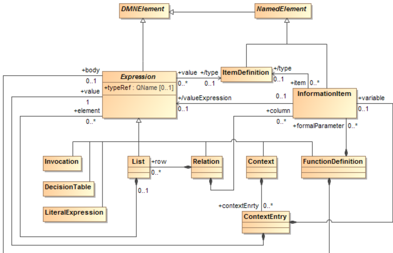
Figure 67: Expression class diagram
