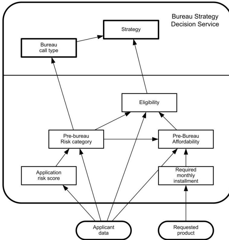
Figure 74: Bureau Strategy Decision Service
