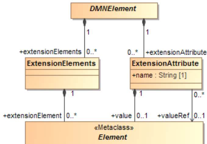
Figure 25: Extensibility class diagram
