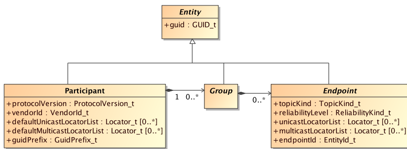
Figure 8.5 - RTPS Participant
